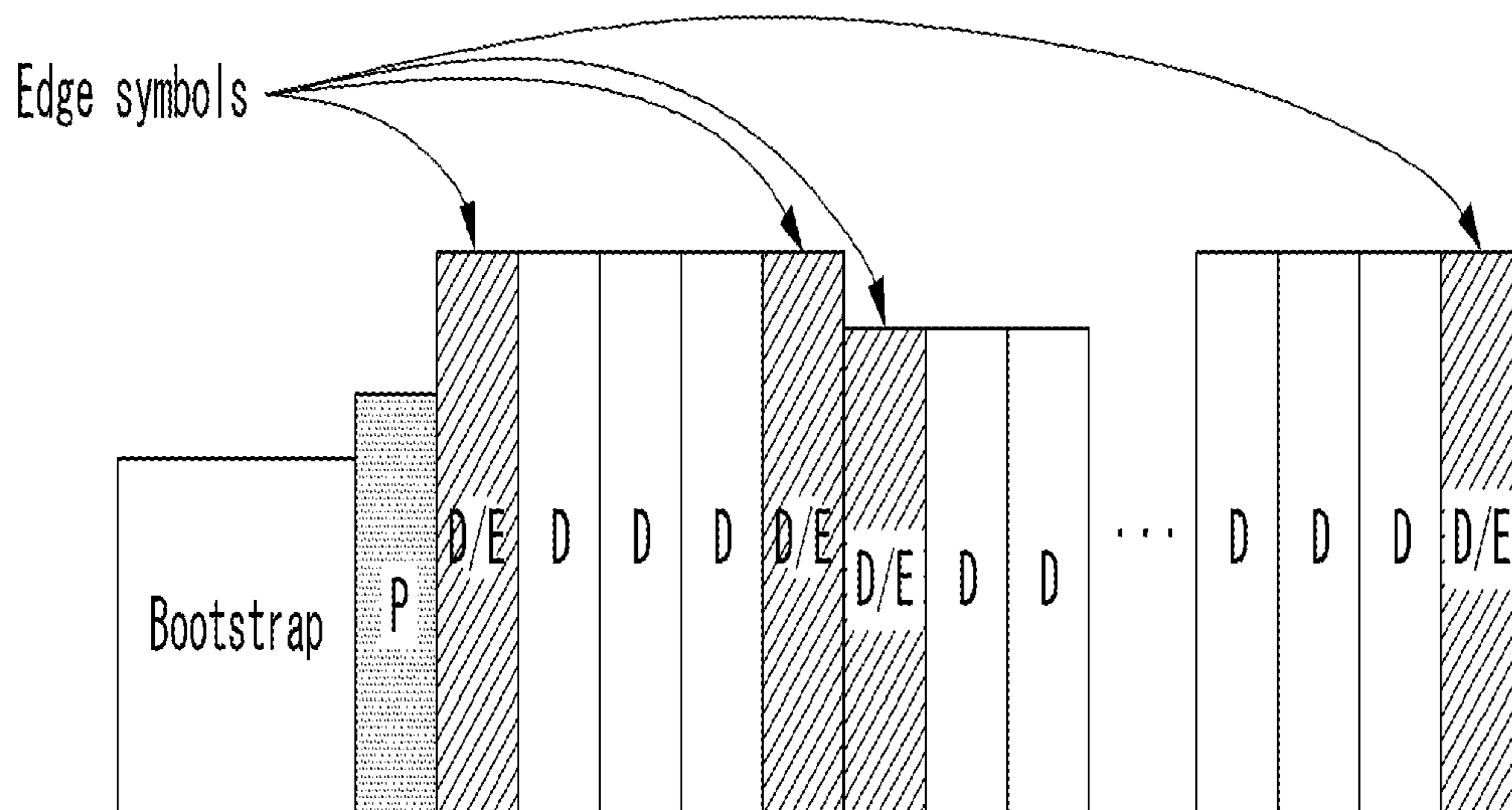
(b) Two edge symbols per sub-frame for a mixed FFT frame
