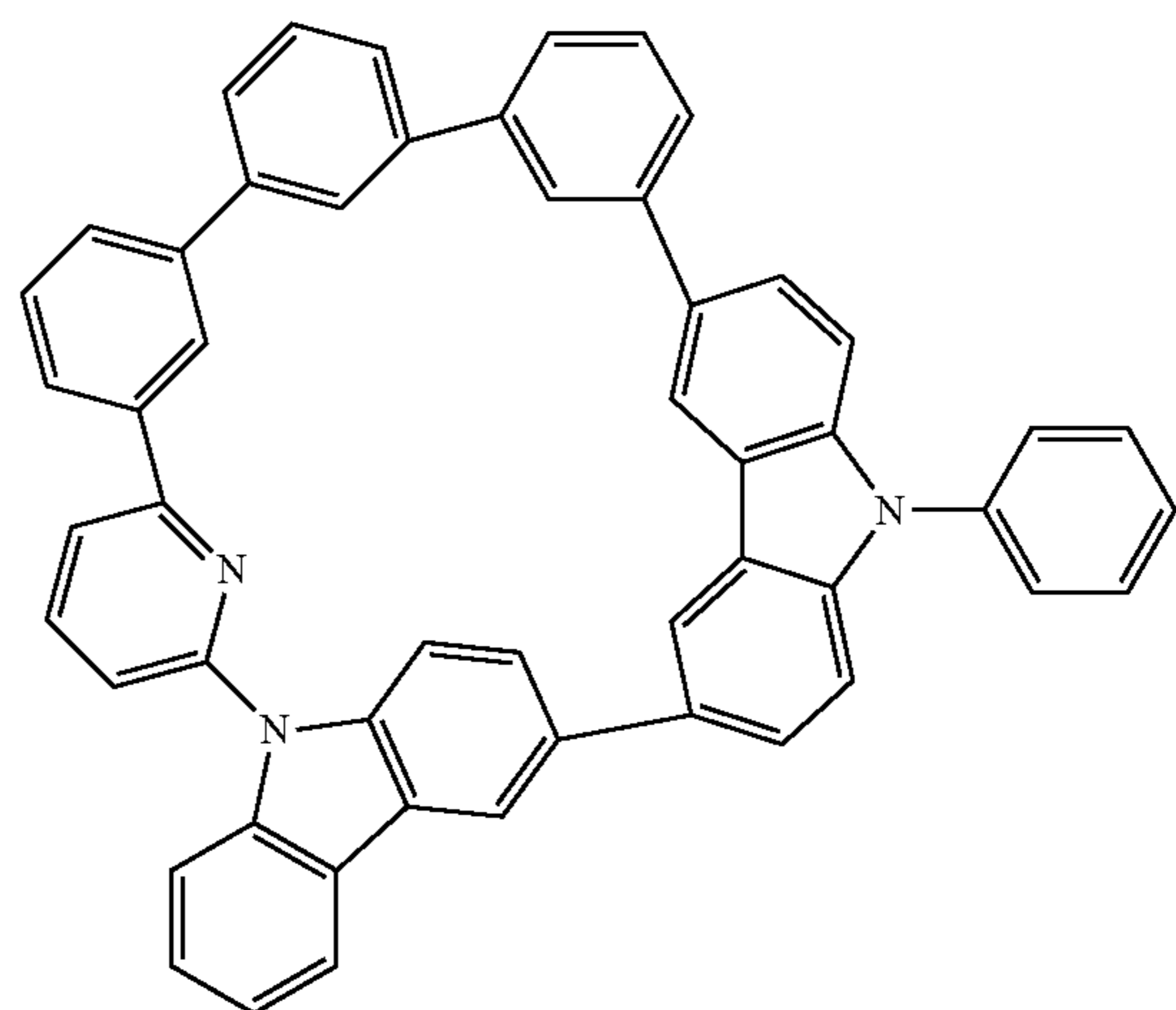
Compound 24
