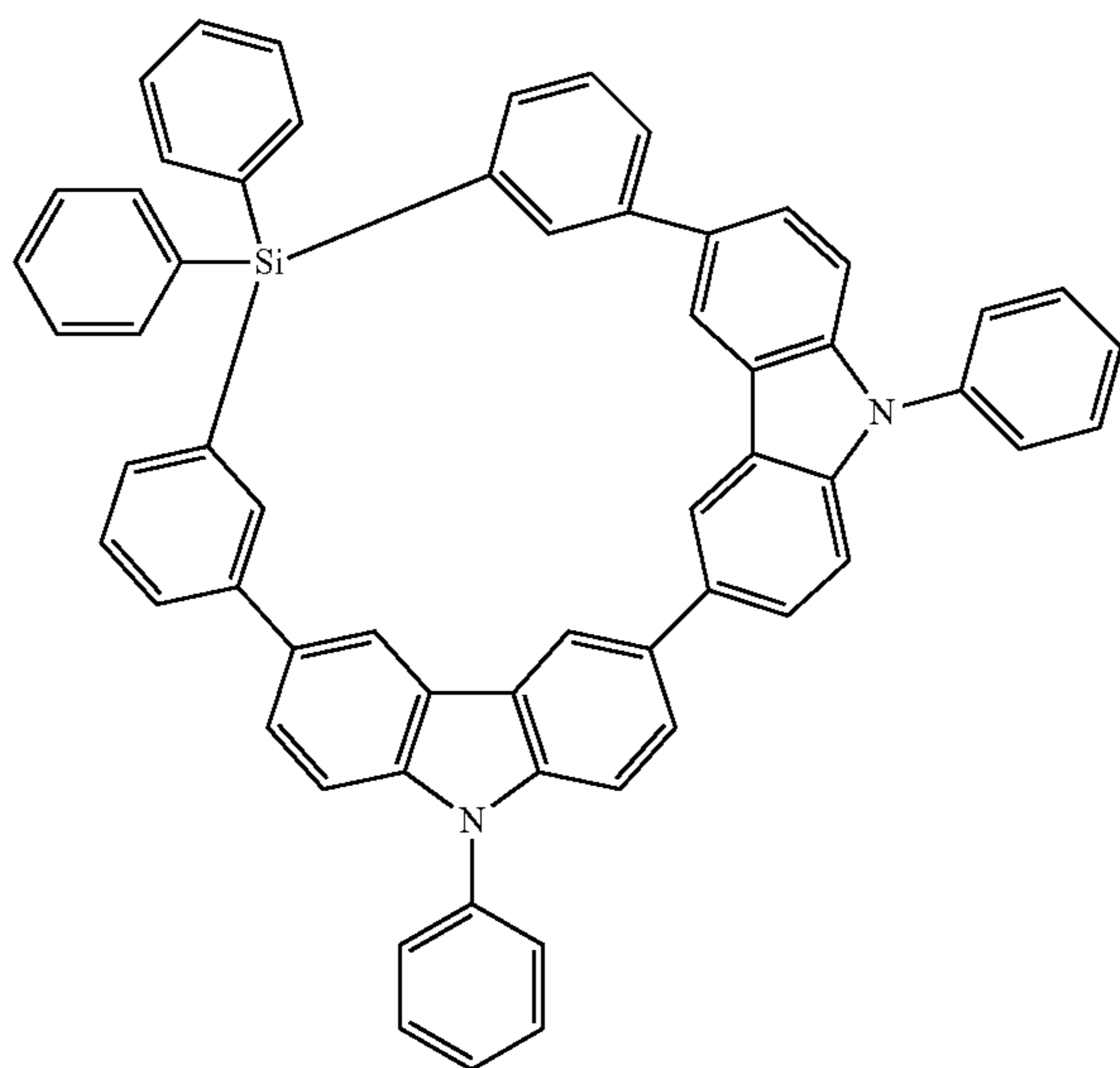
Compound 27
