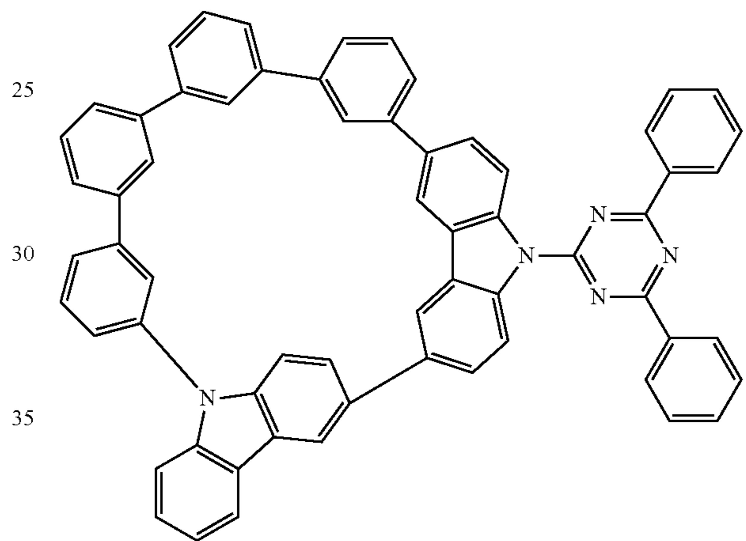
Compound 51
