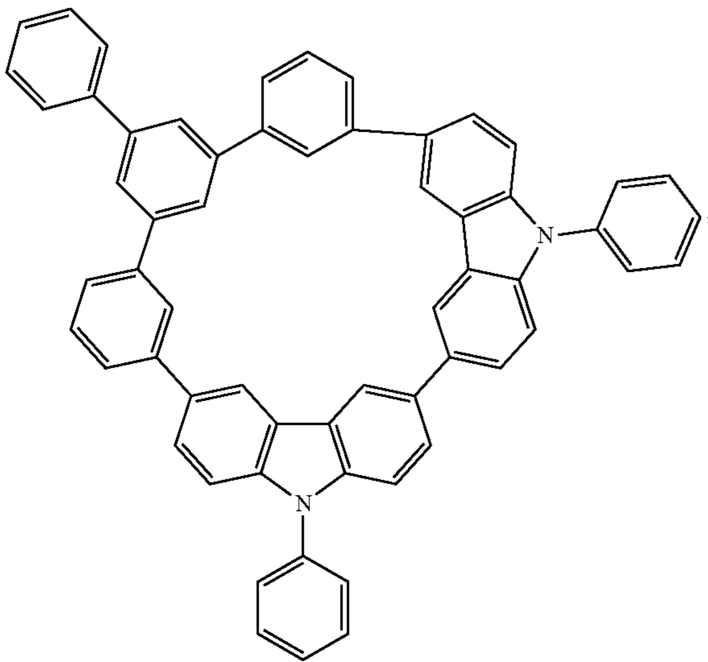
Compound 2
