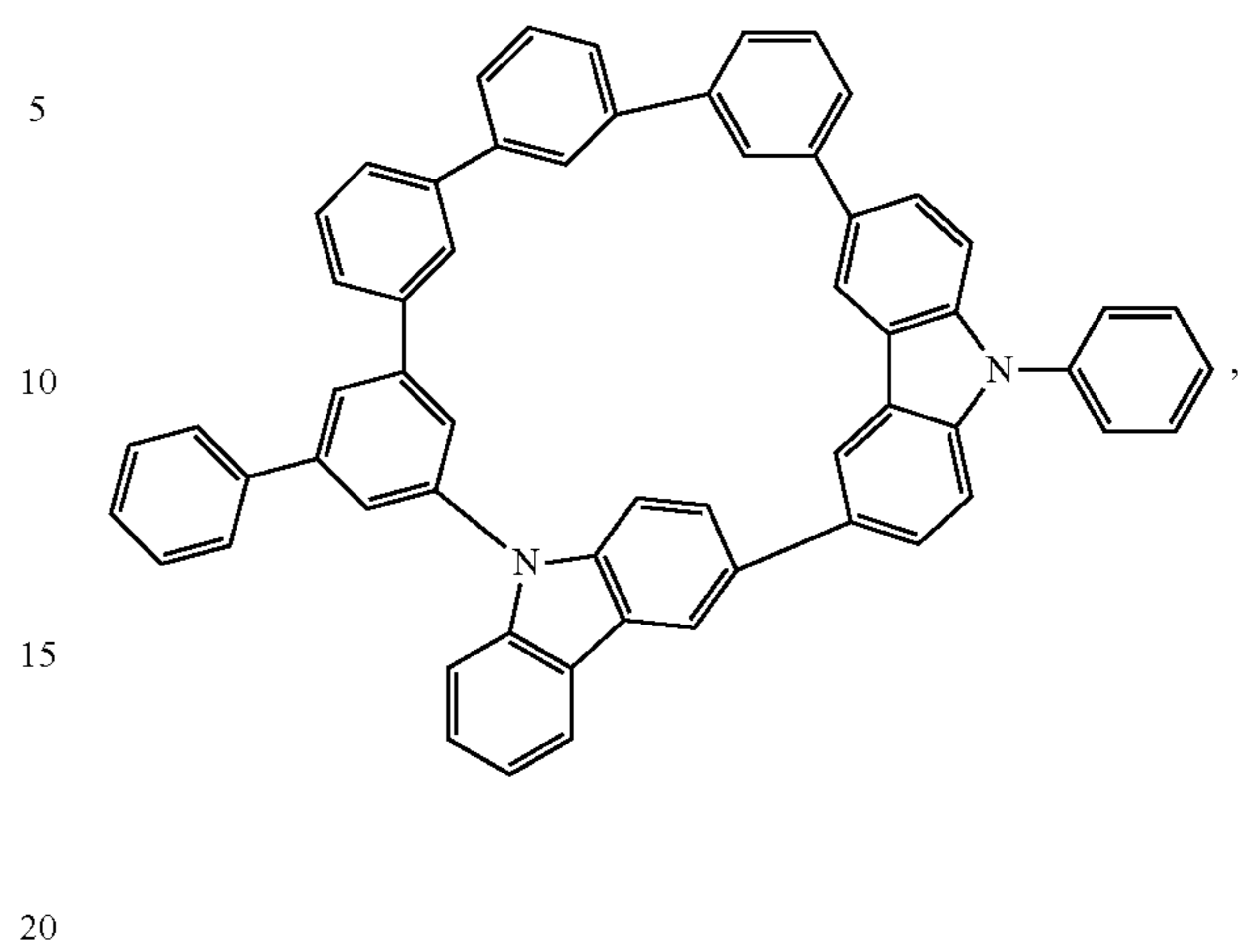
Compound 25
