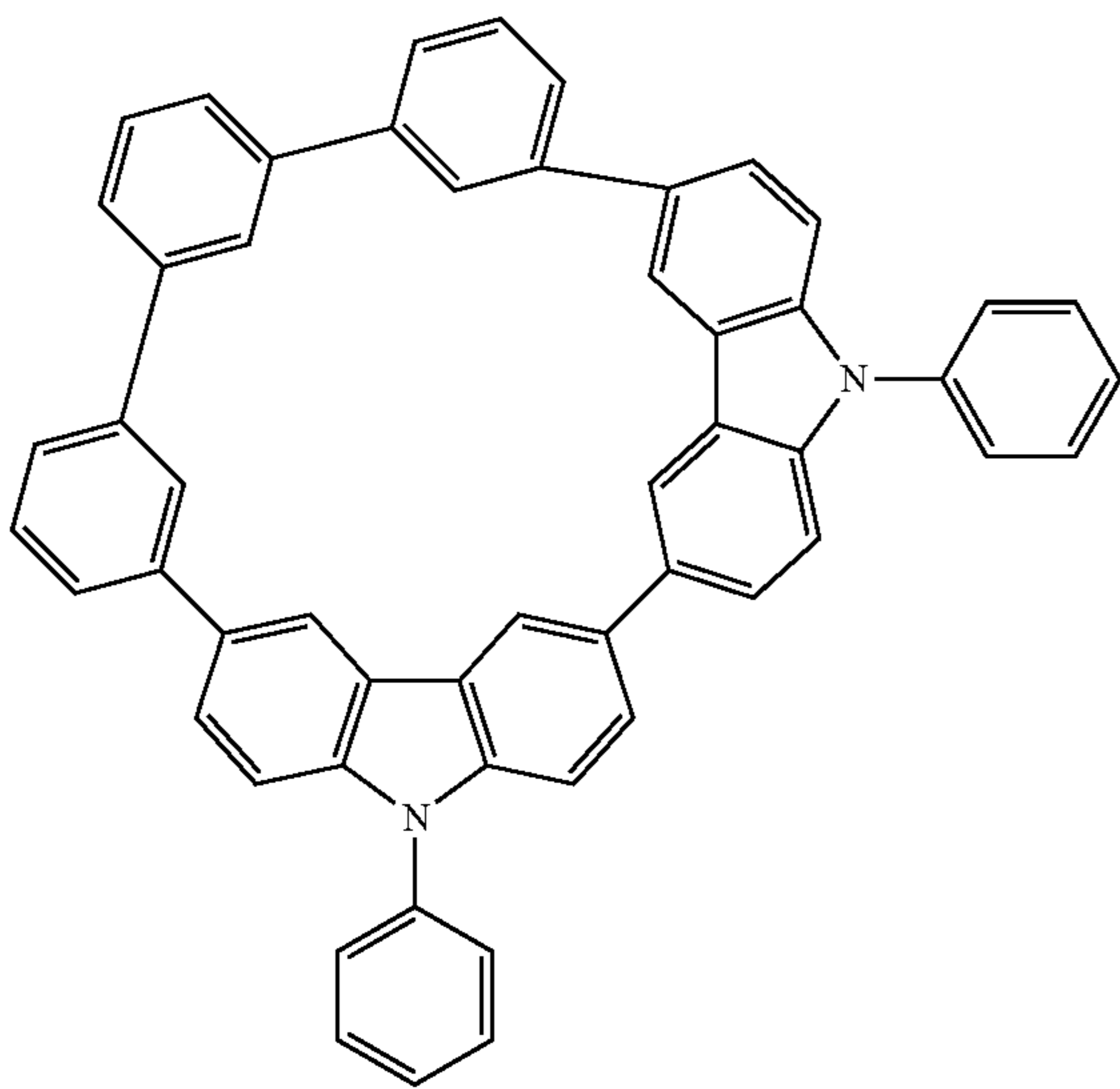
Compound 2
