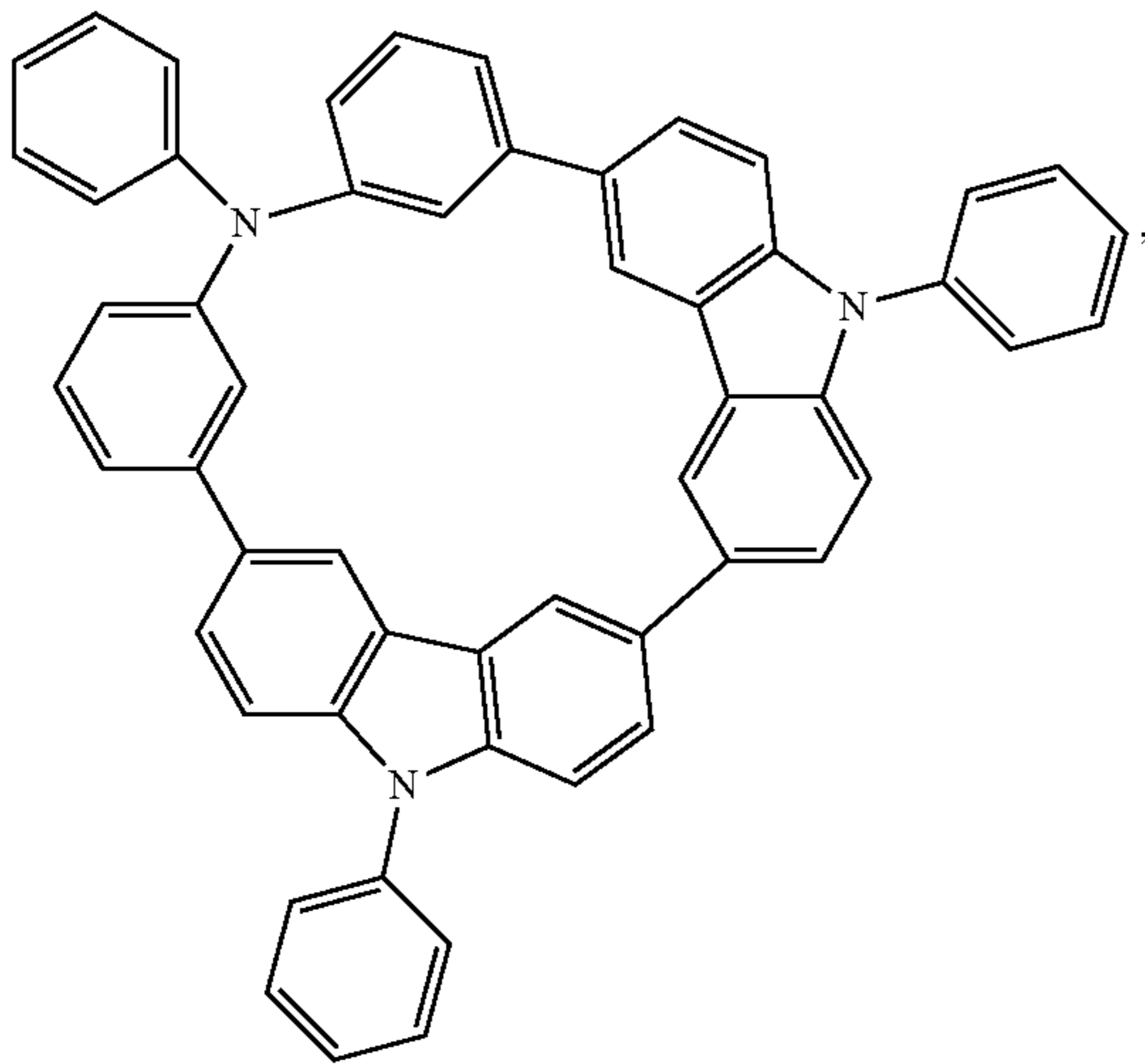
Compound 28
