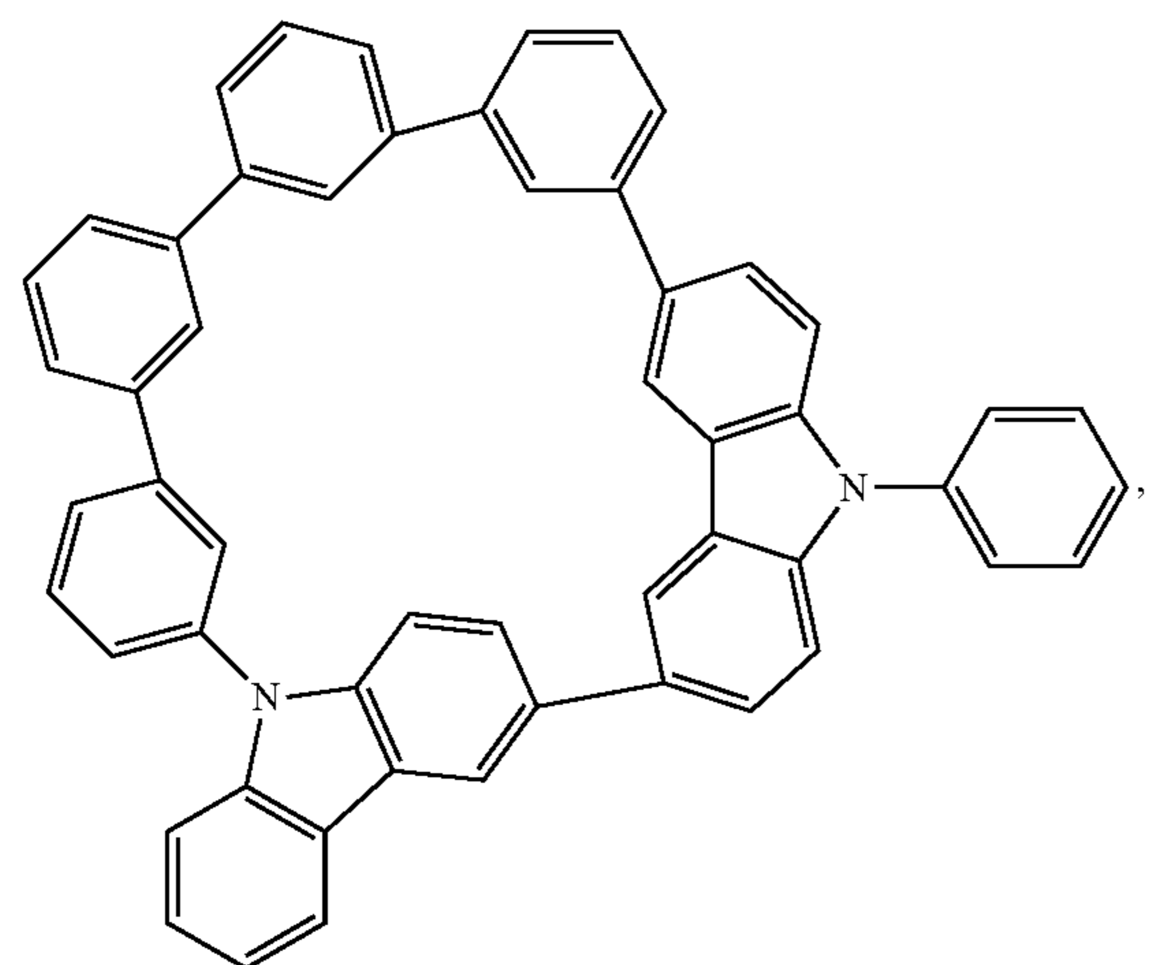
Compound 21
