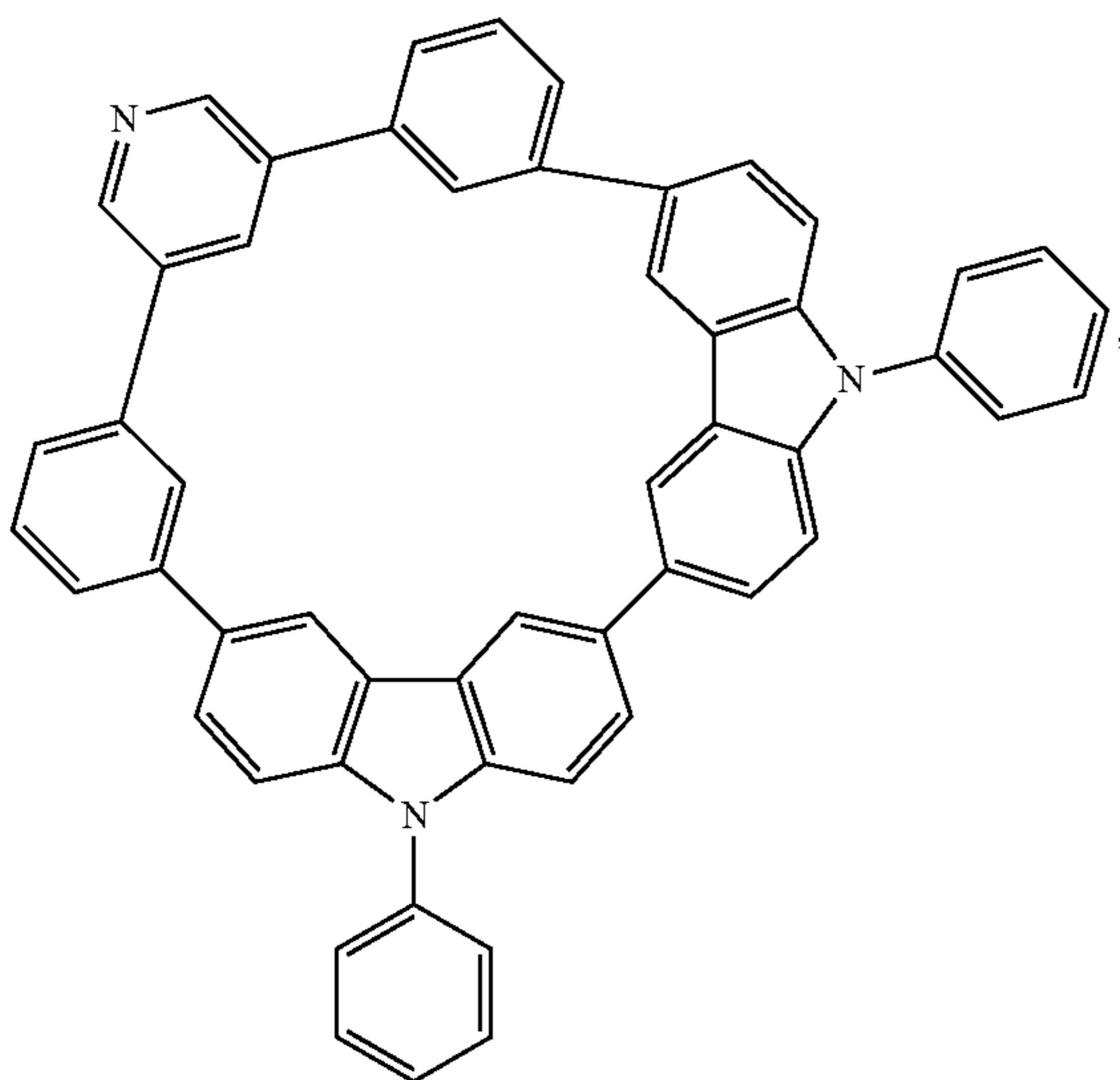
Compound 20
