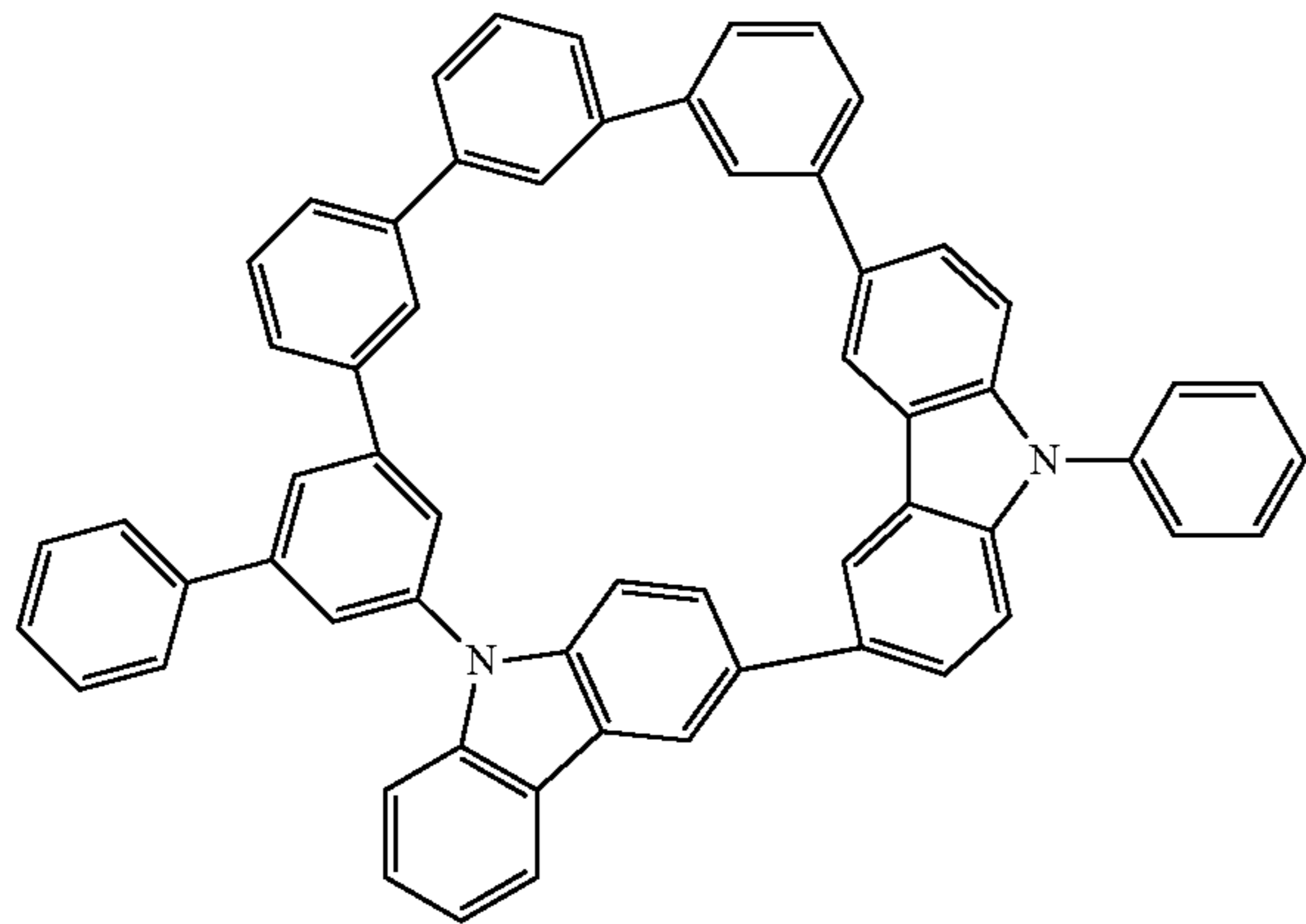
Compound 25
