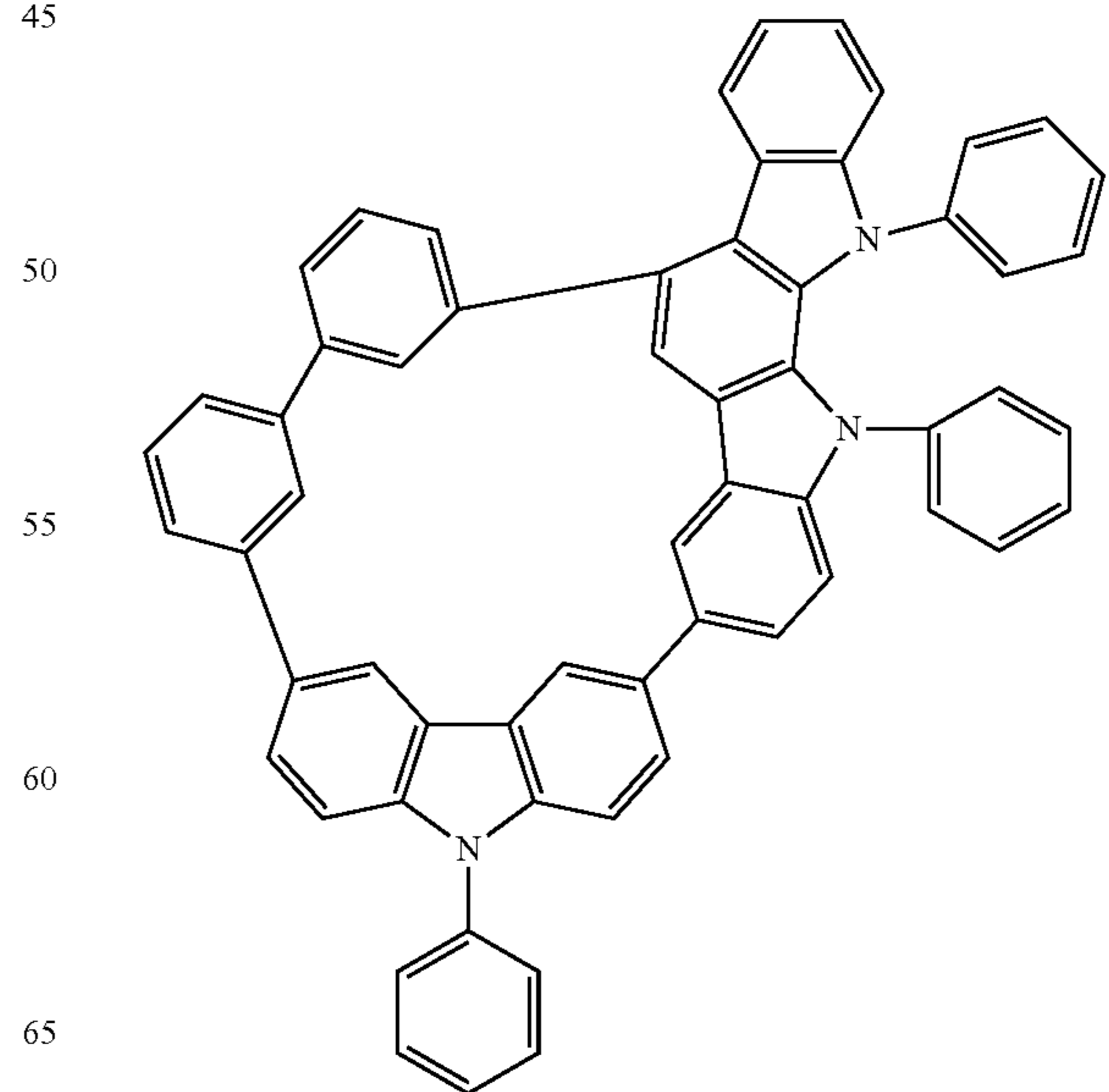
Compound 16
