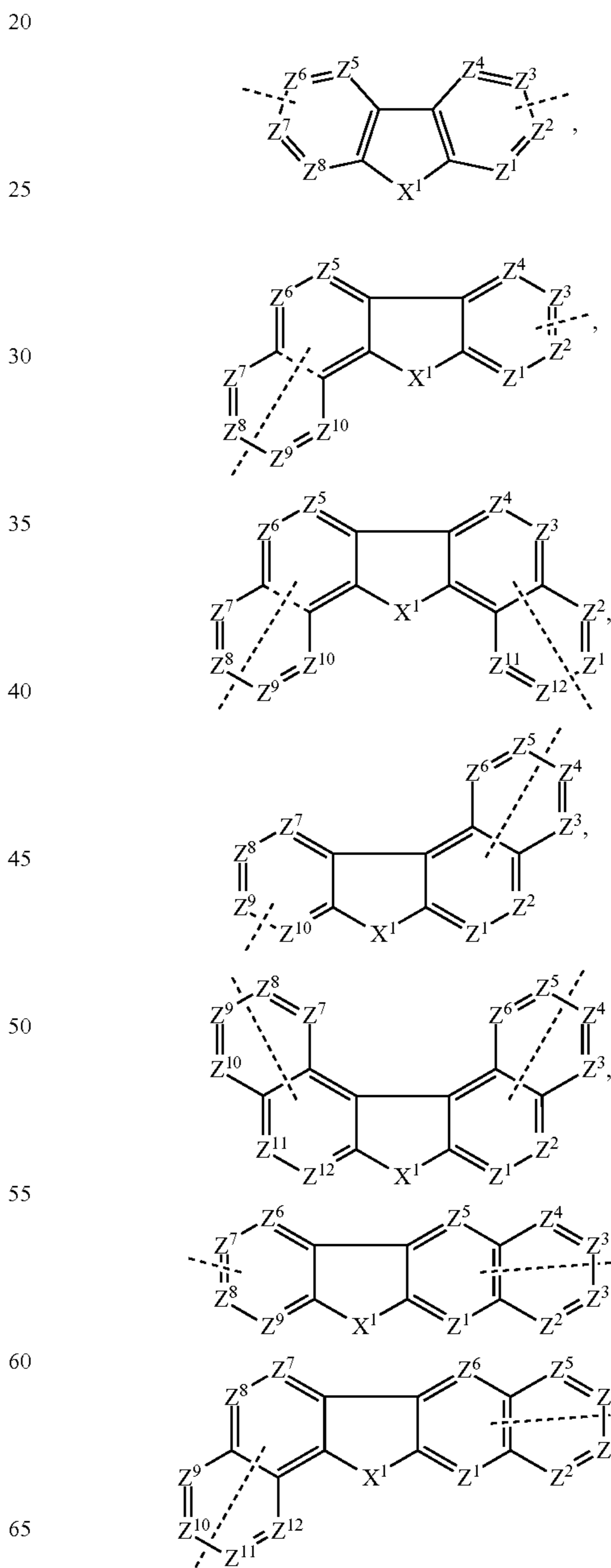
Formula I
