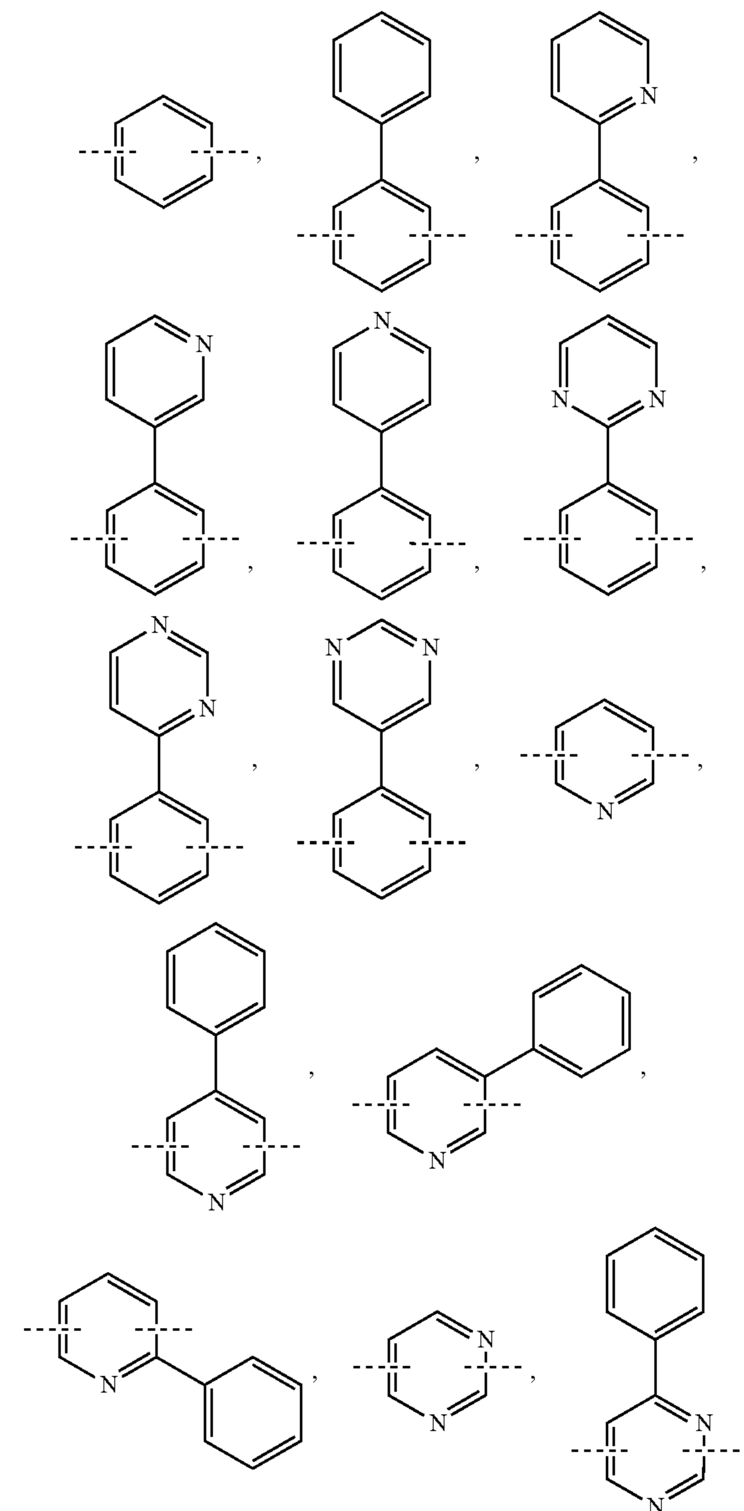
Formula I
