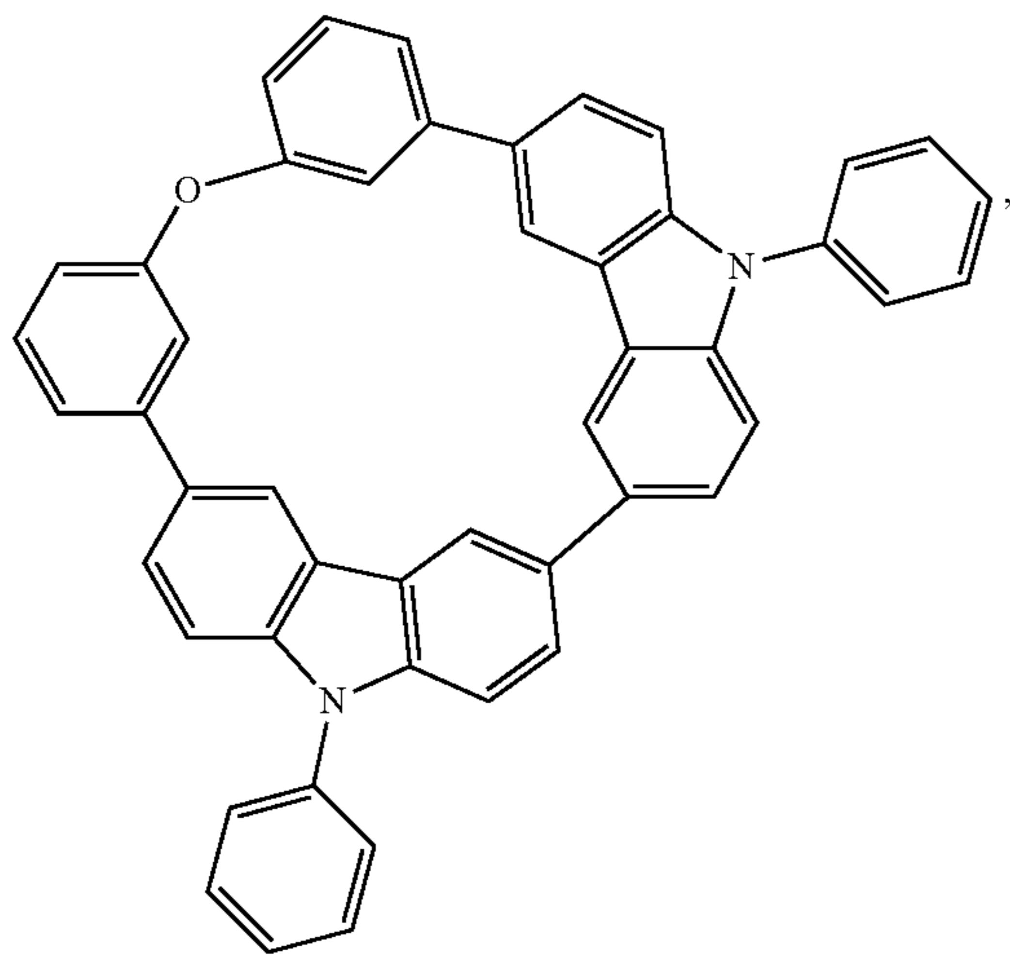
Compound 29
