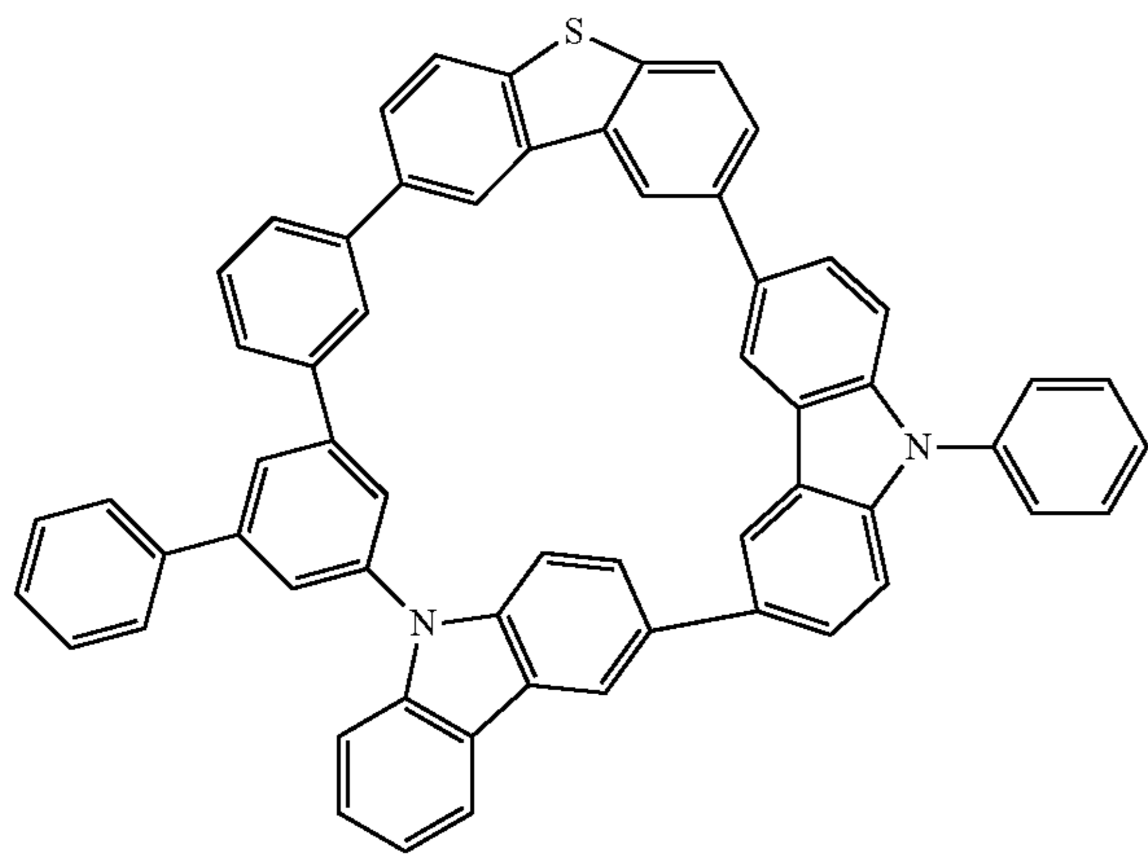
Compound 26
