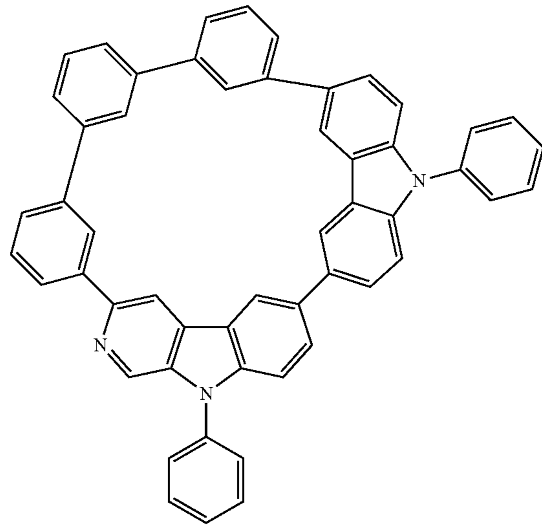
Compound 41
