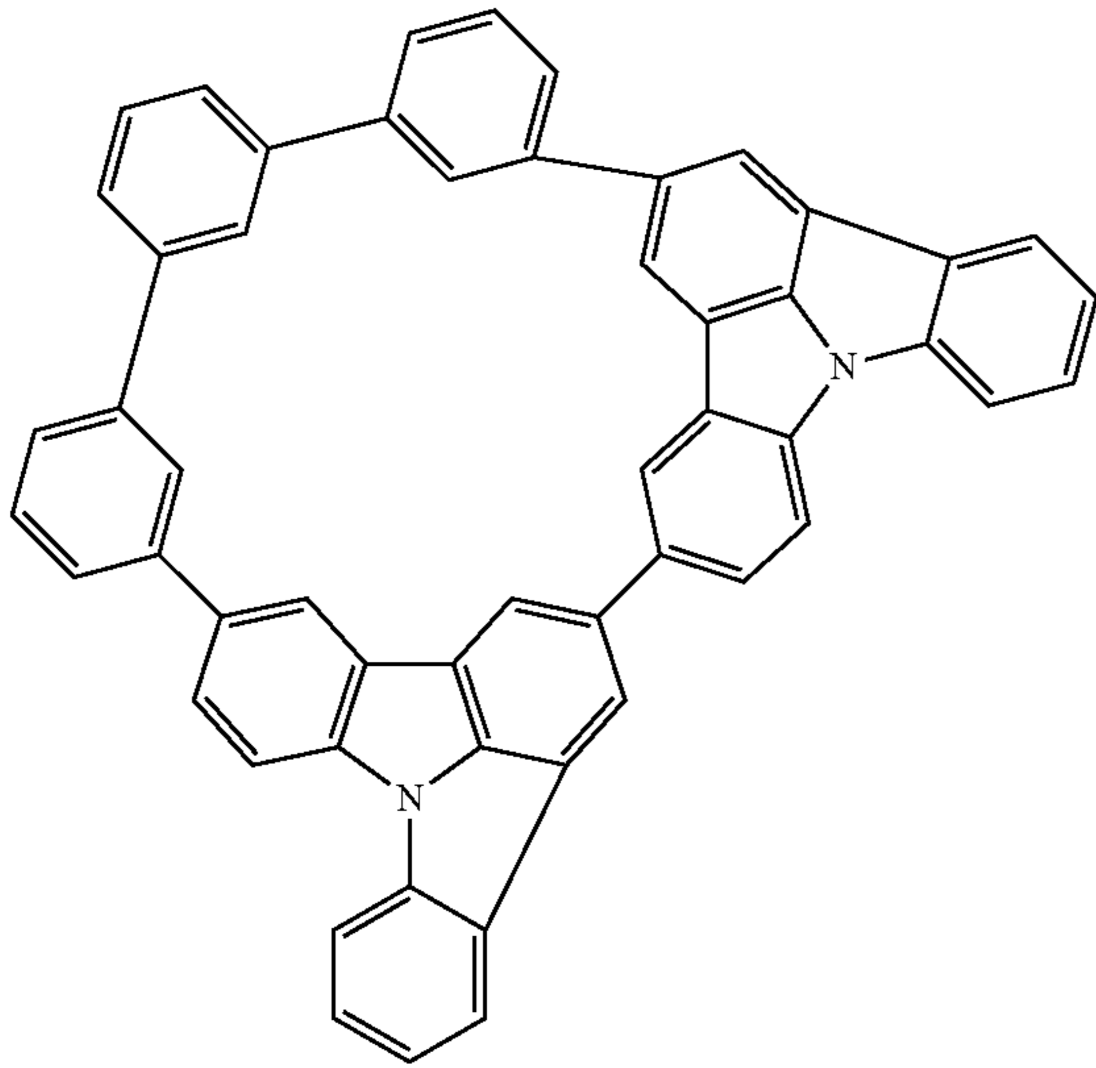
Compound 44
