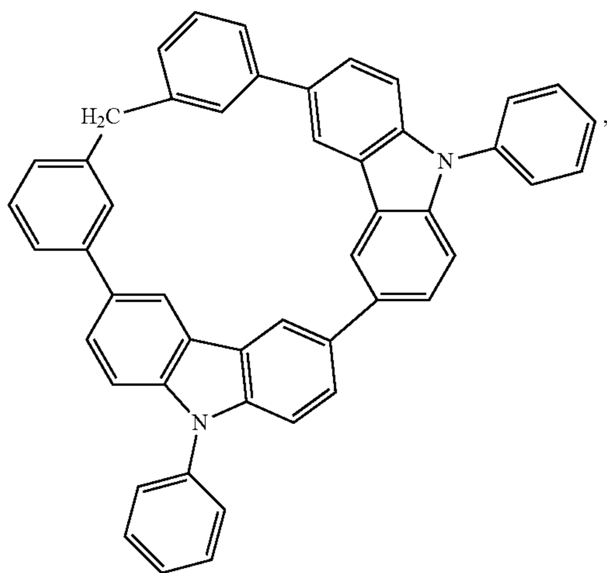
Compound 30
