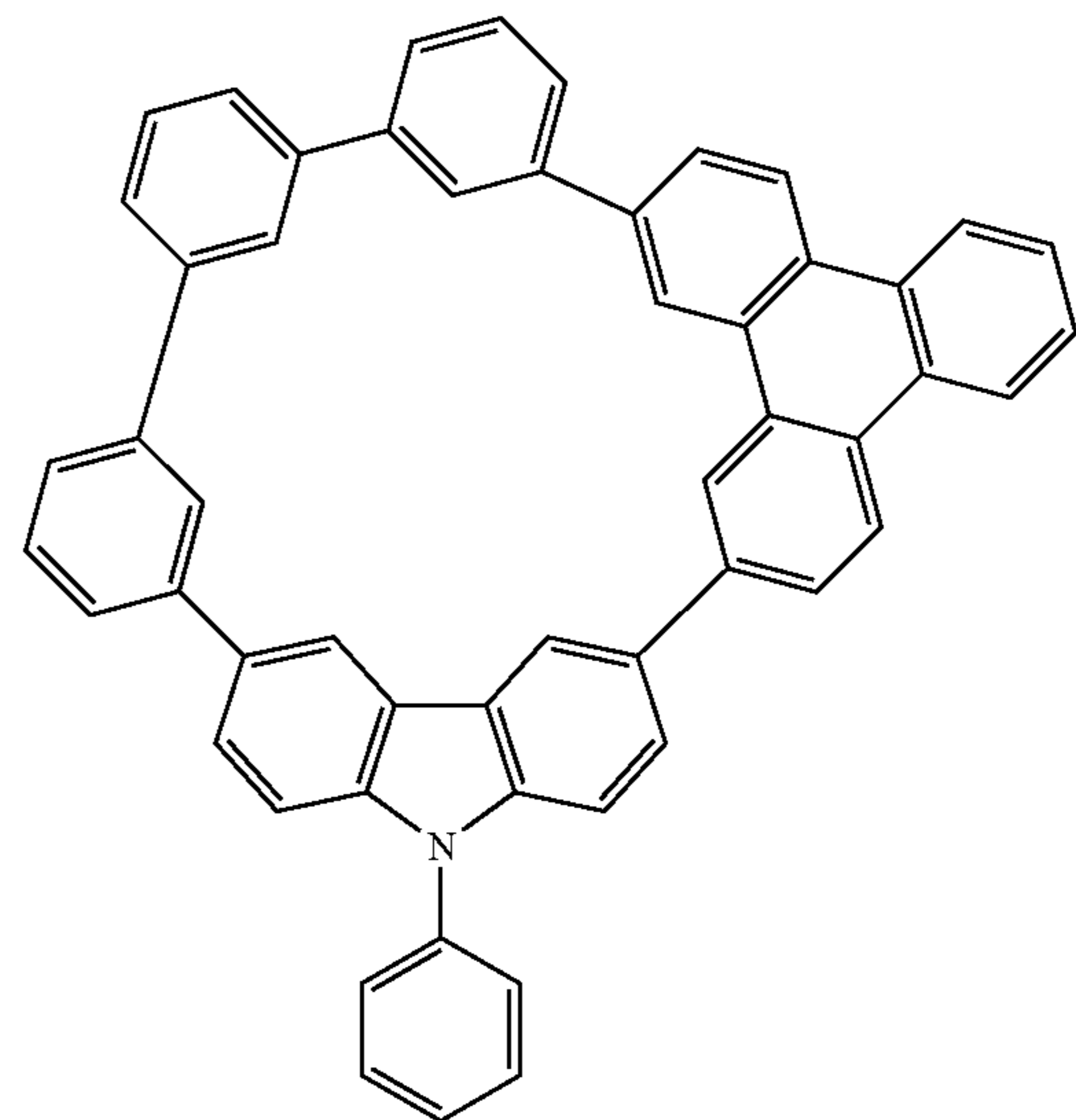
Compound 48
