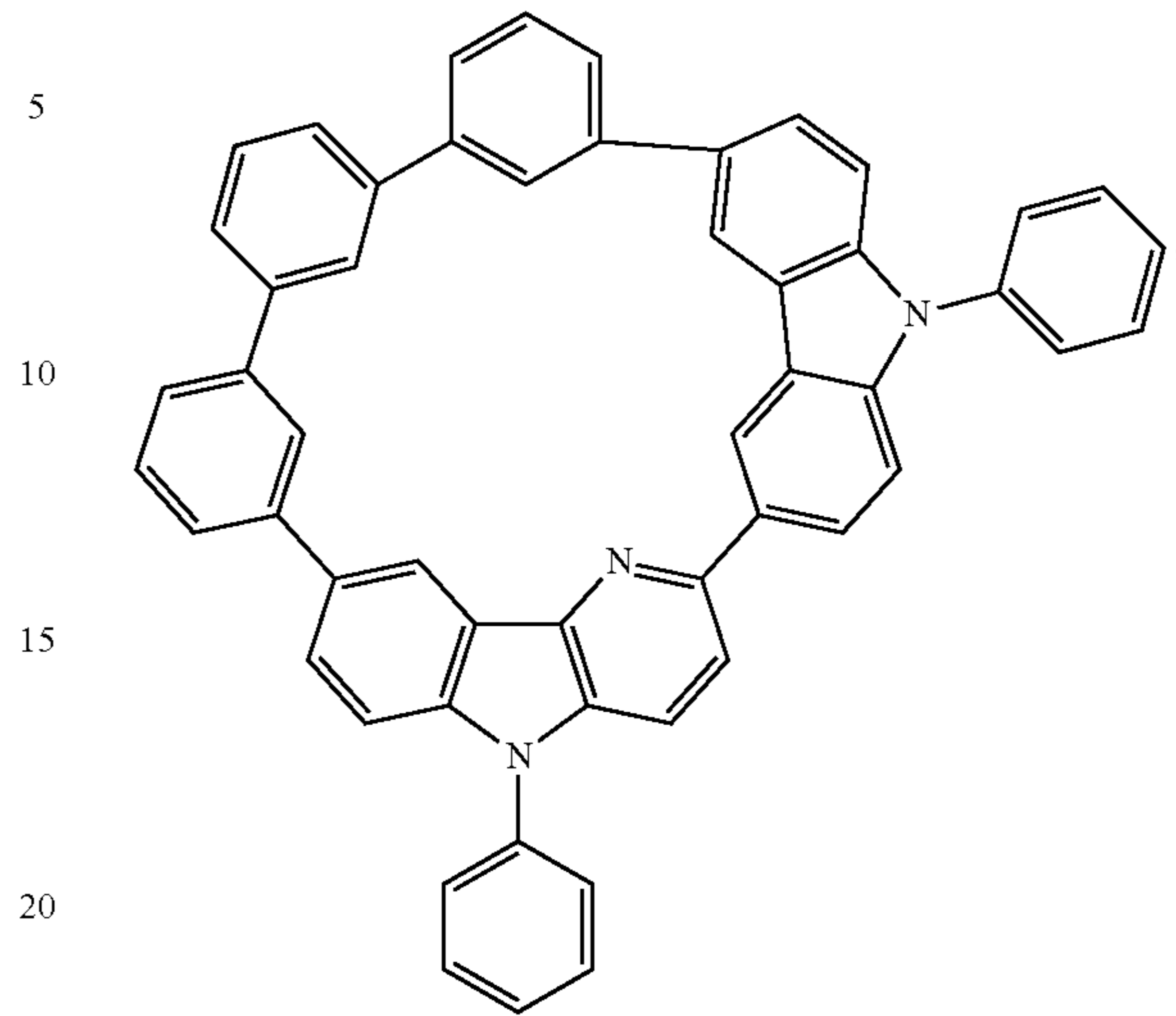
Compound 38
