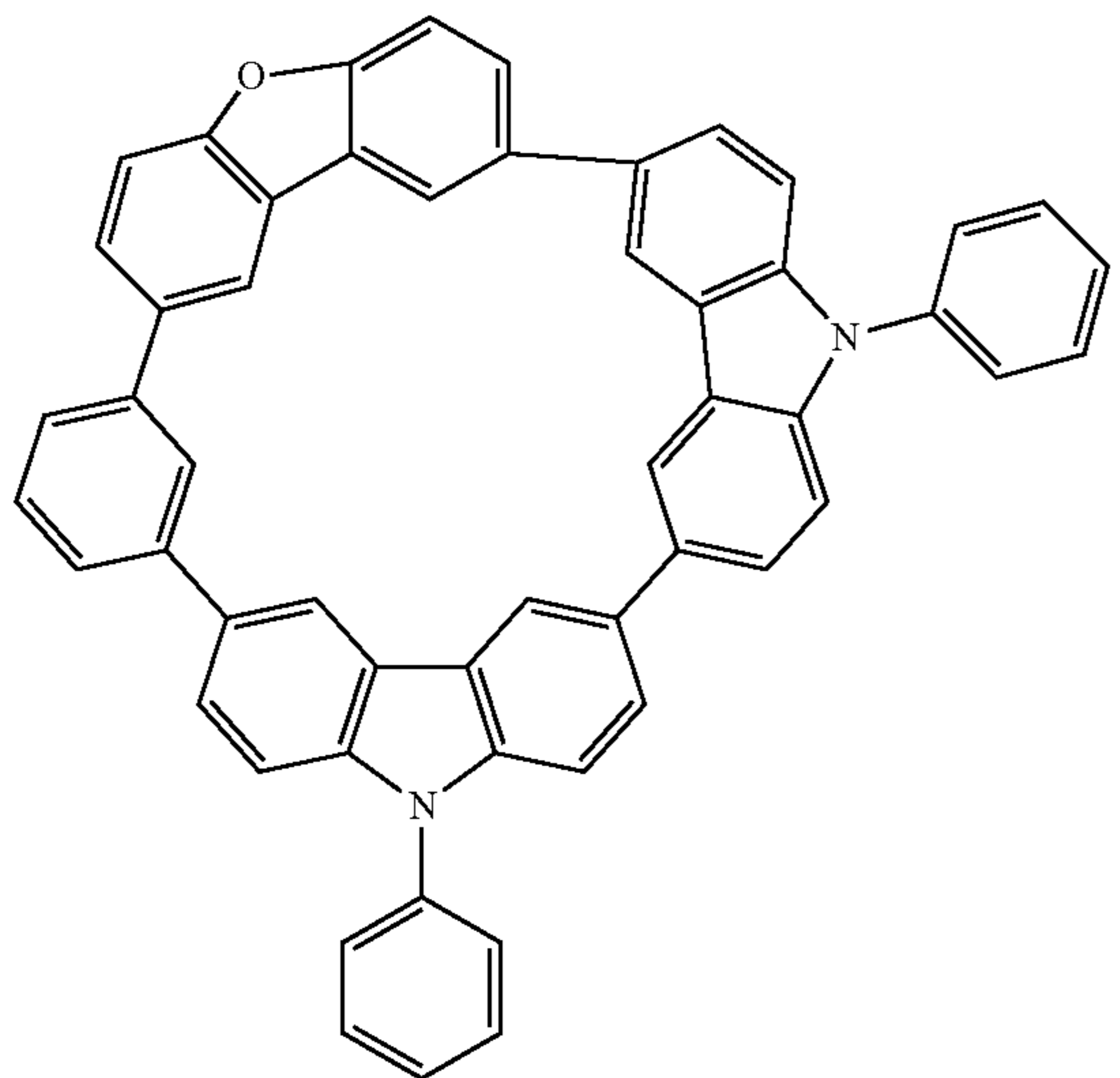
Compound 13
