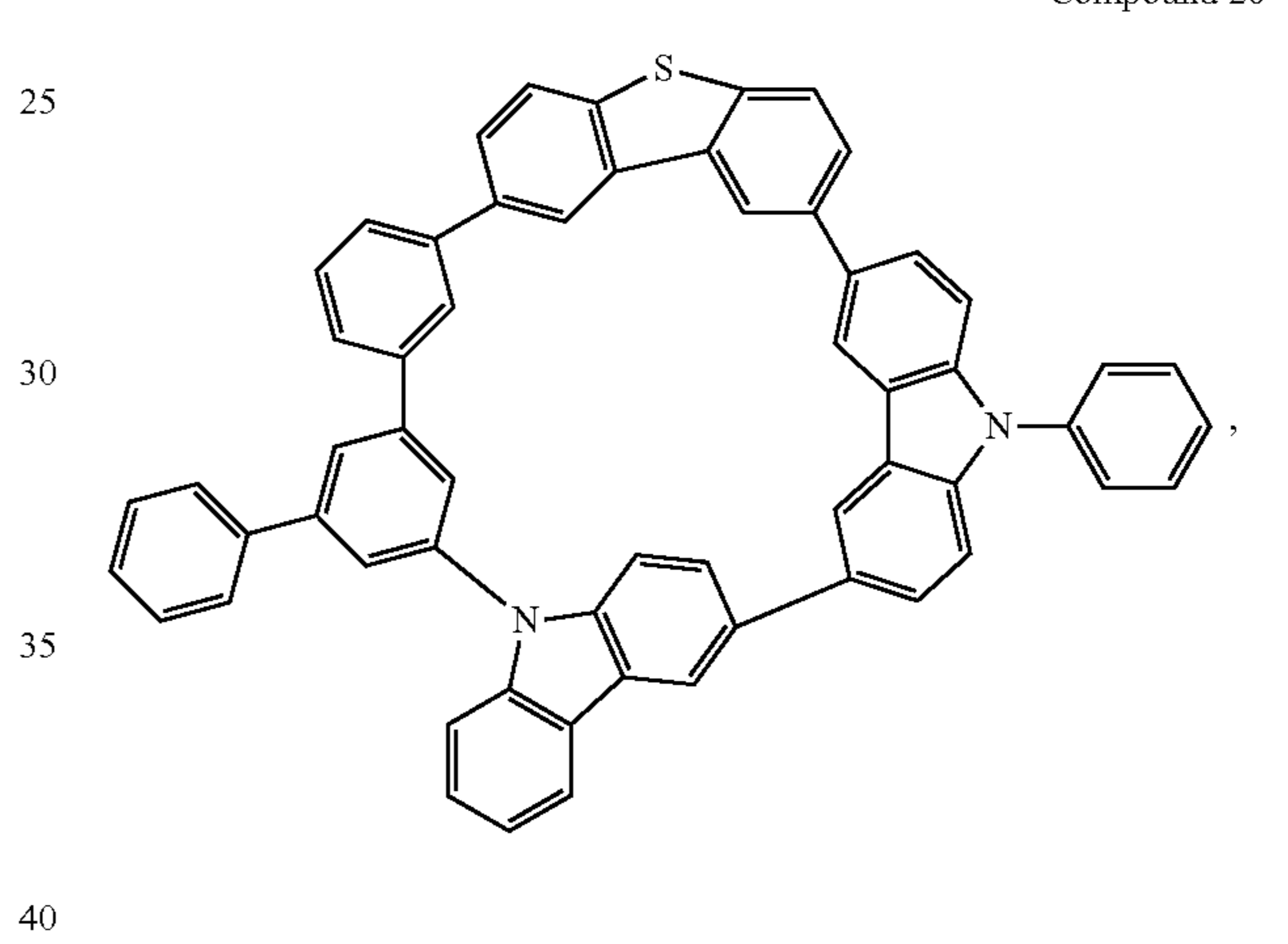
Compound 26
