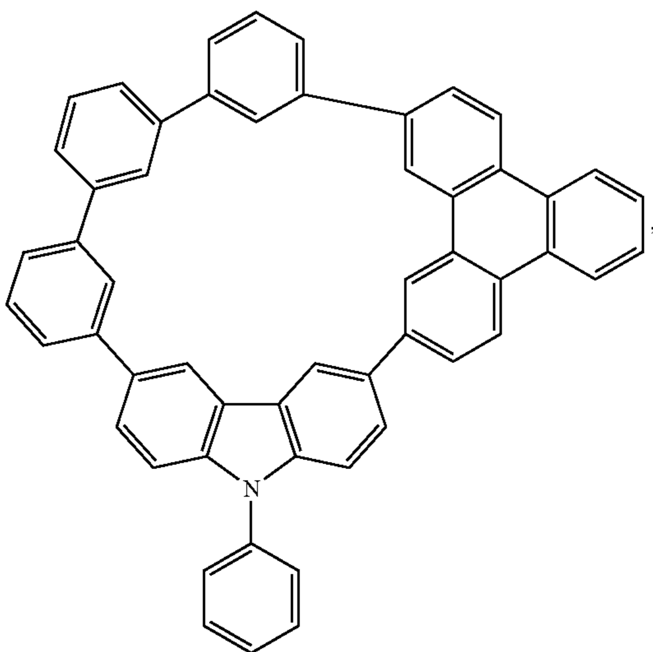
Compound 48
