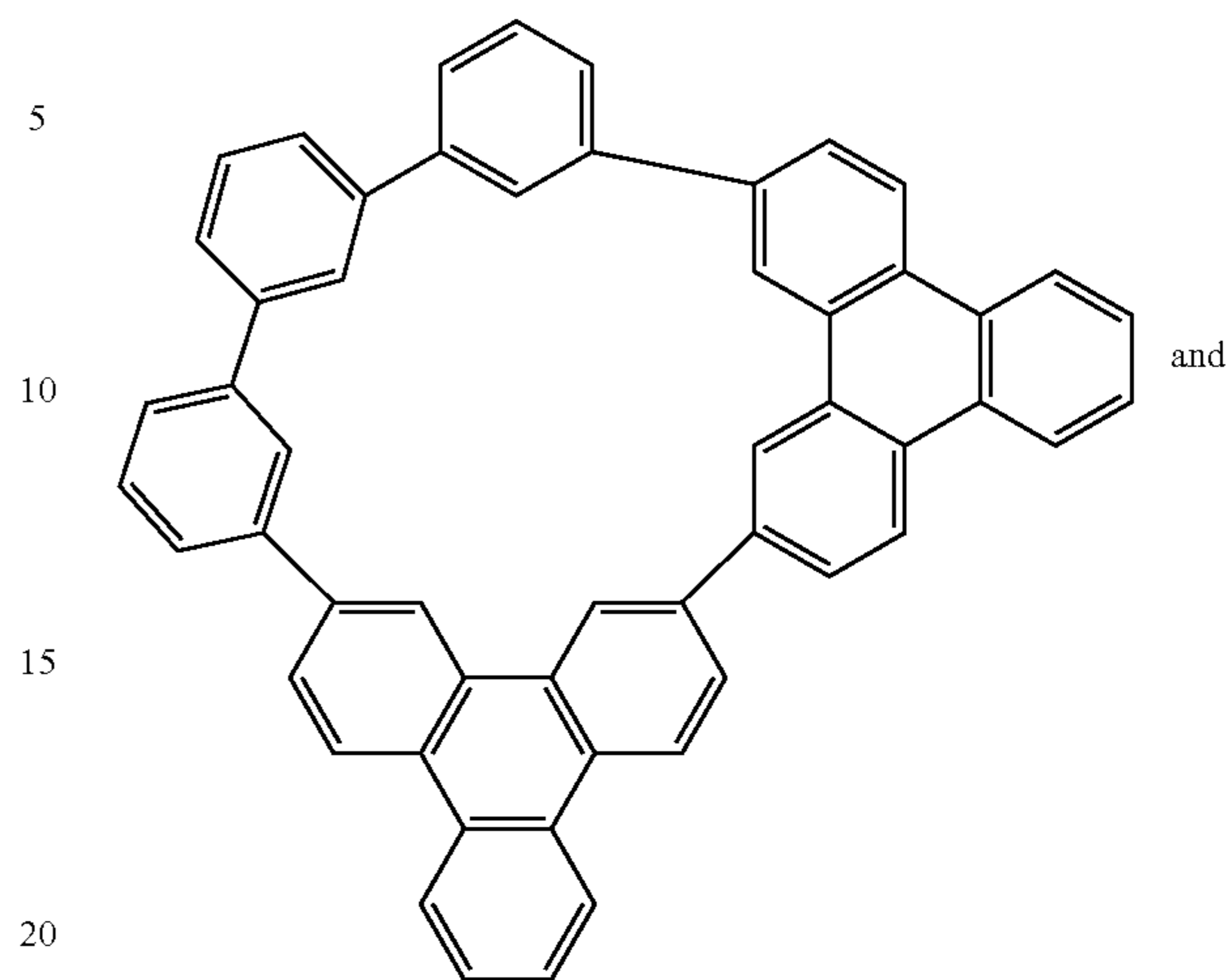
Compound 51
