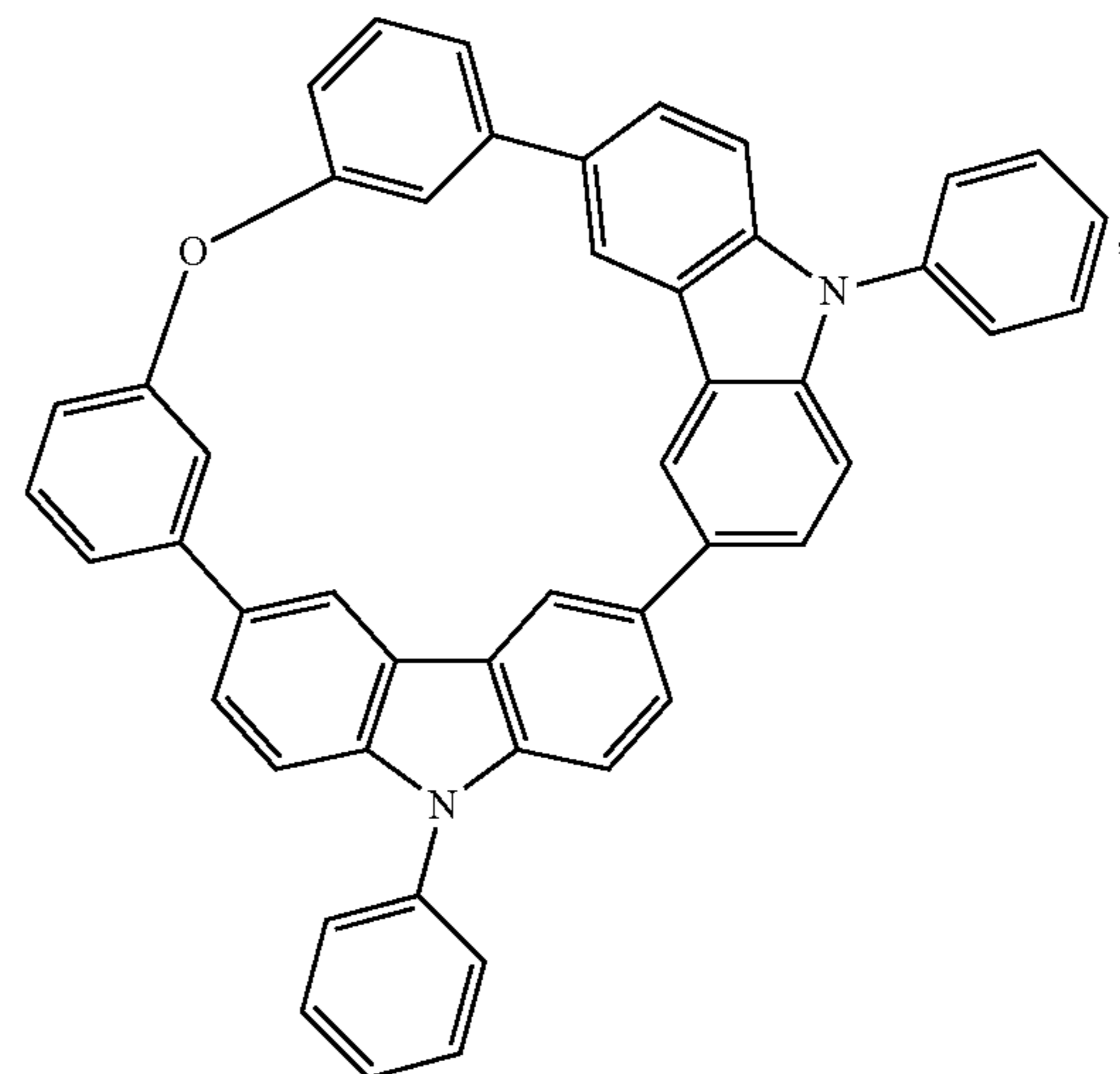
Compound 29
