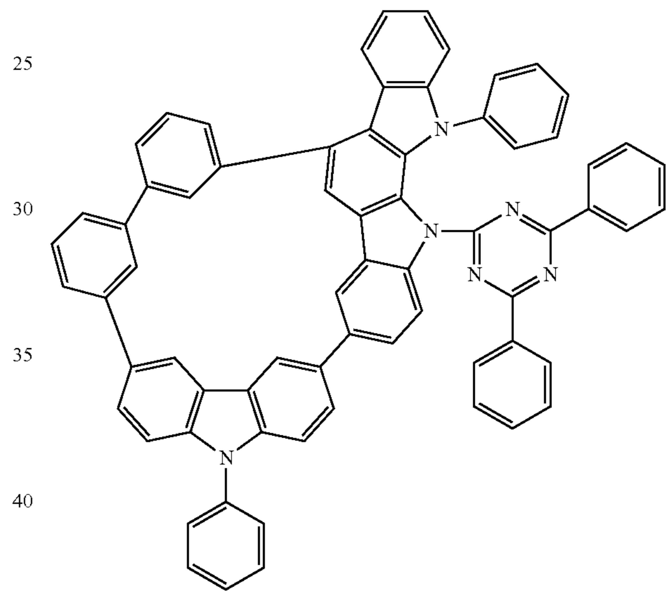
Compound 16
