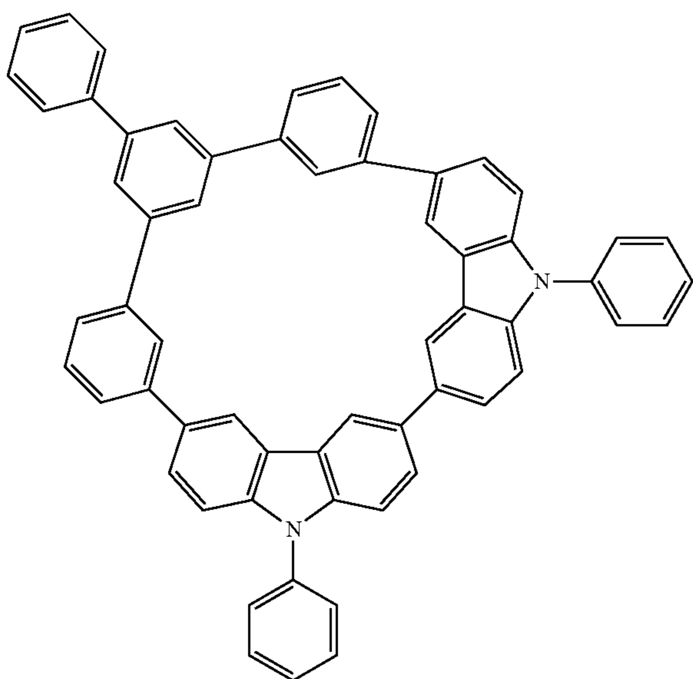
Compound 2
