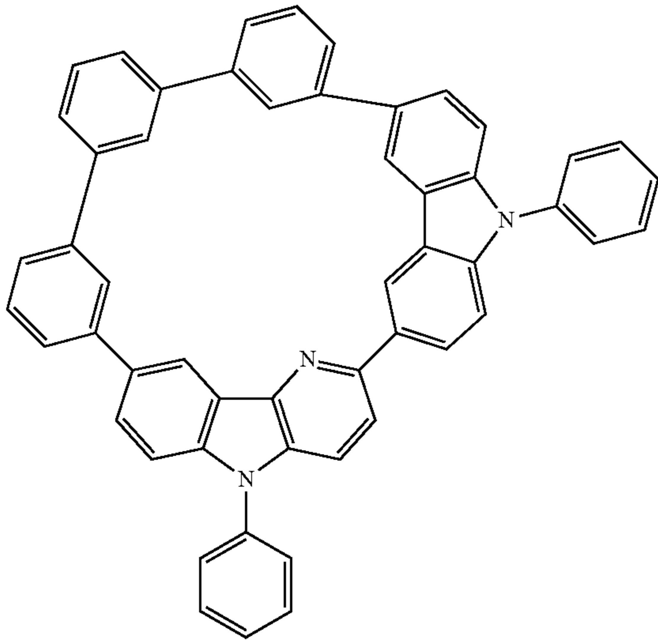
Compound 38
