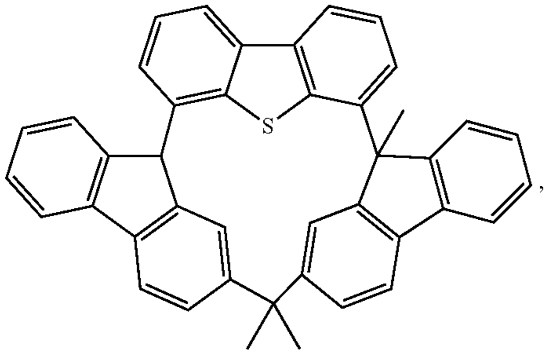
Compound 35
