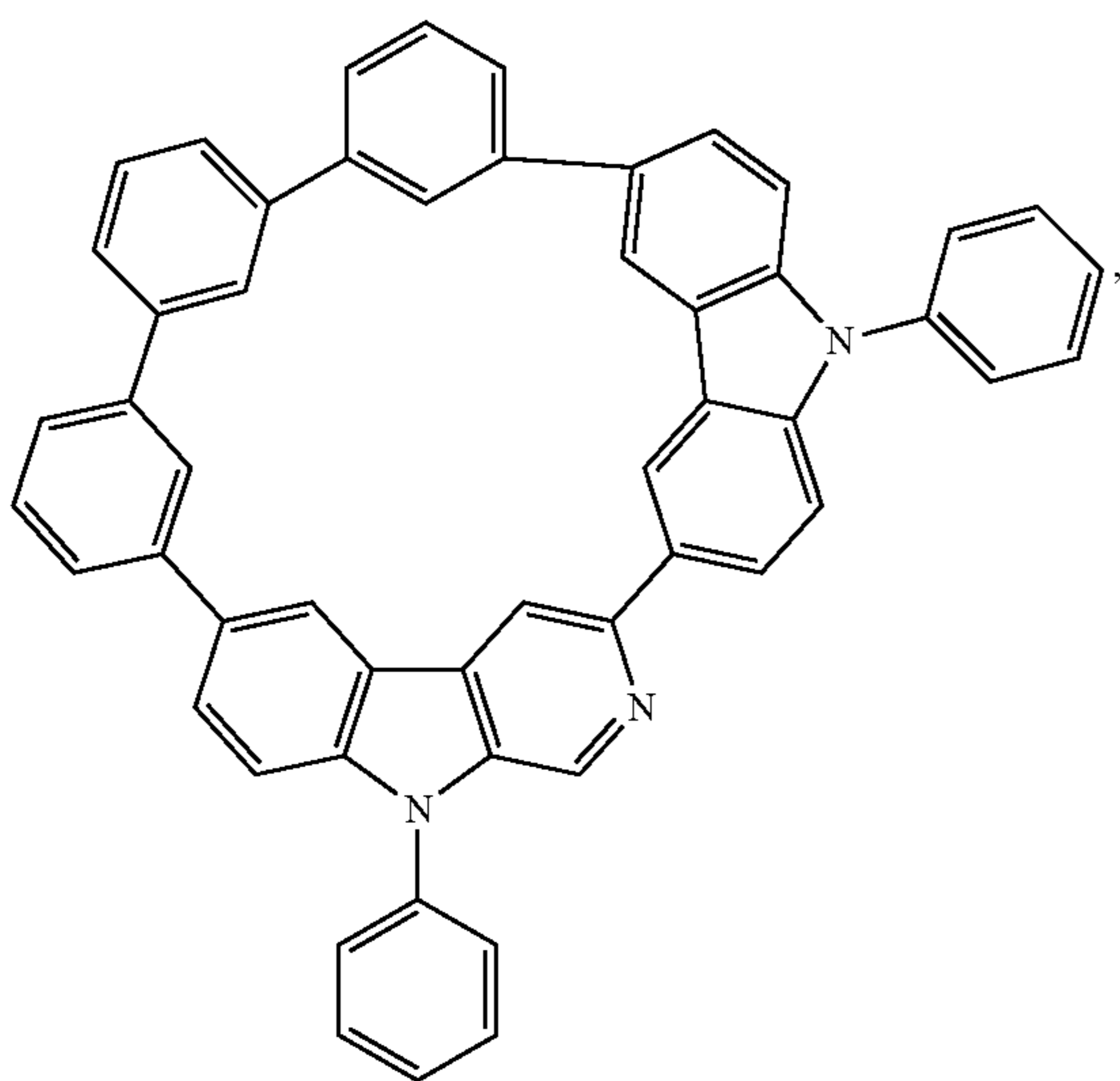
Compound 37
