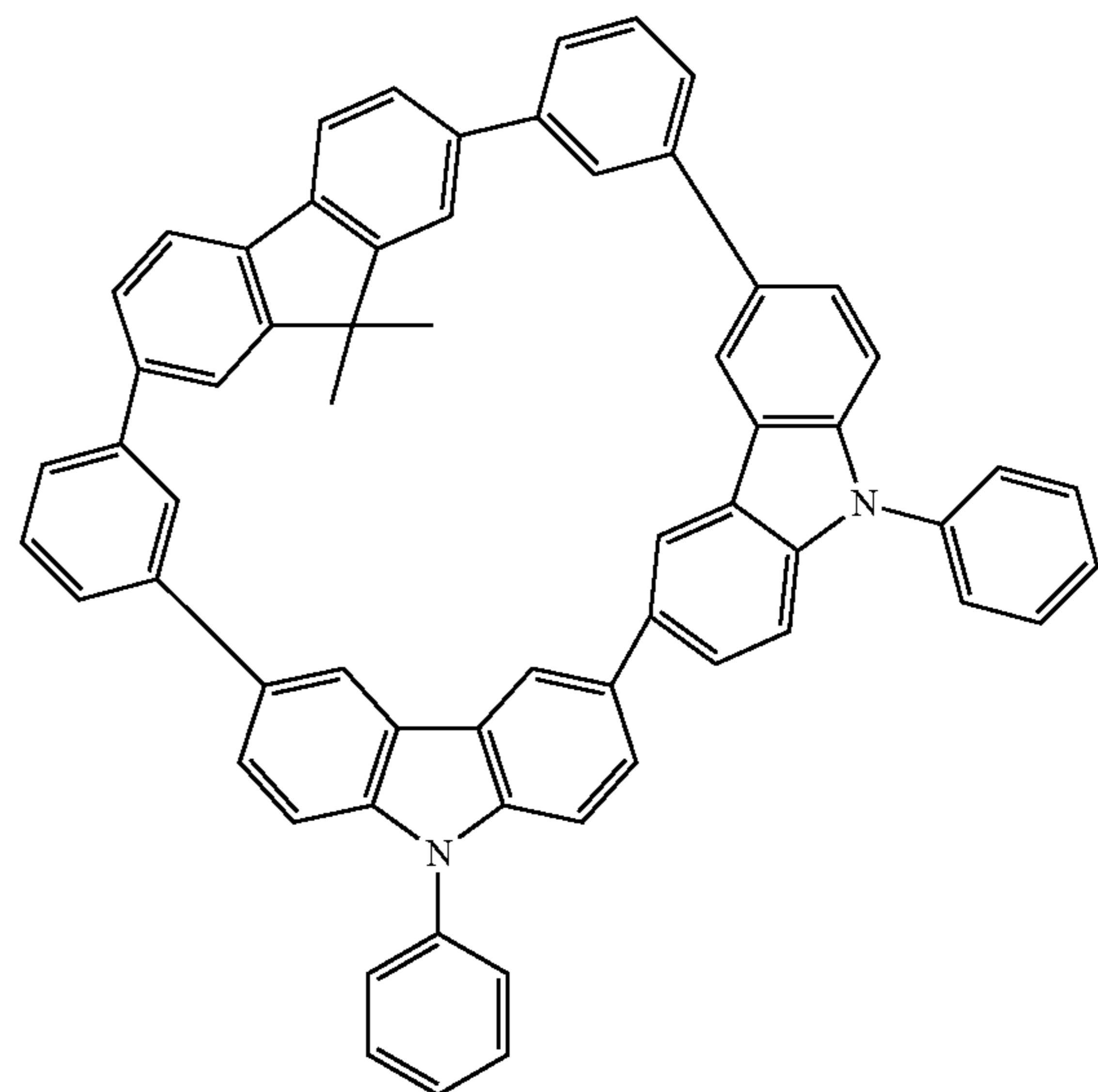
Compound 6
