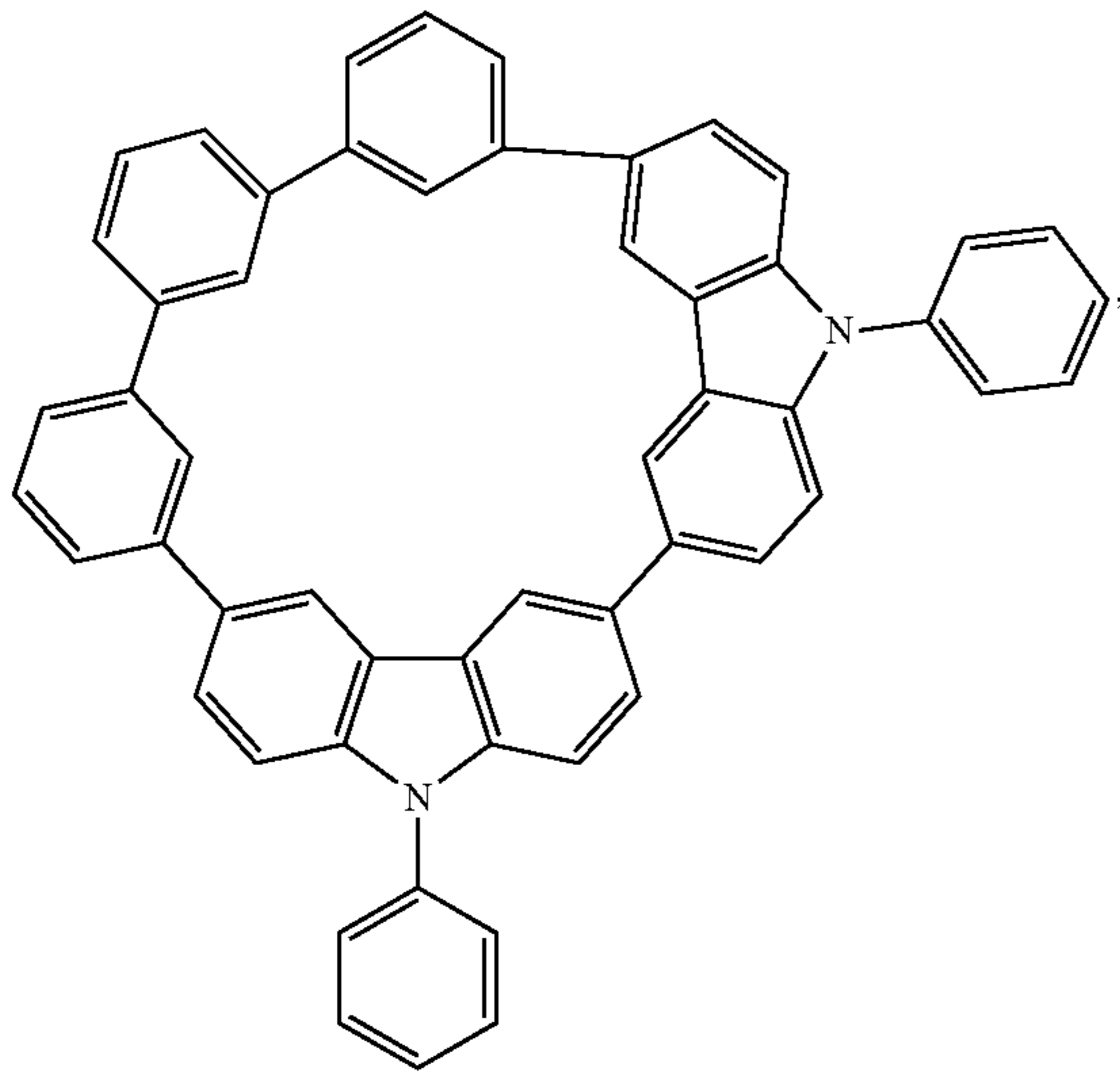
Compound 1
