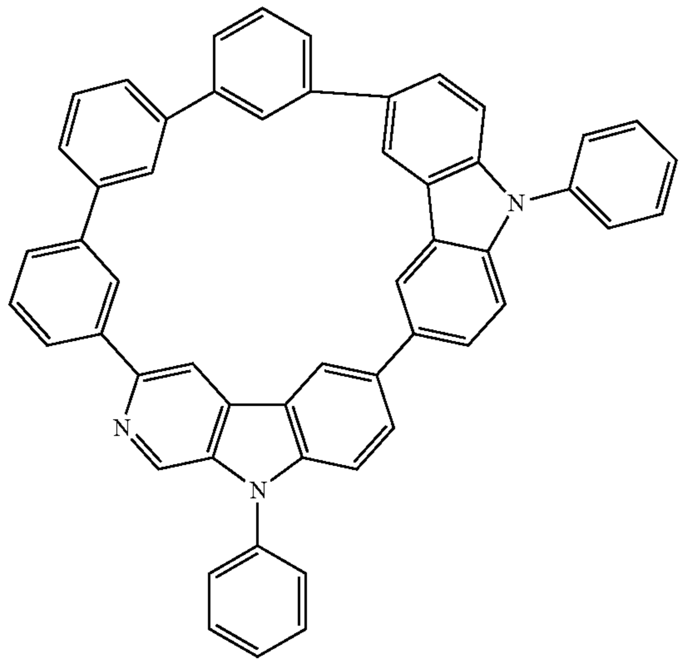
Compound 41
