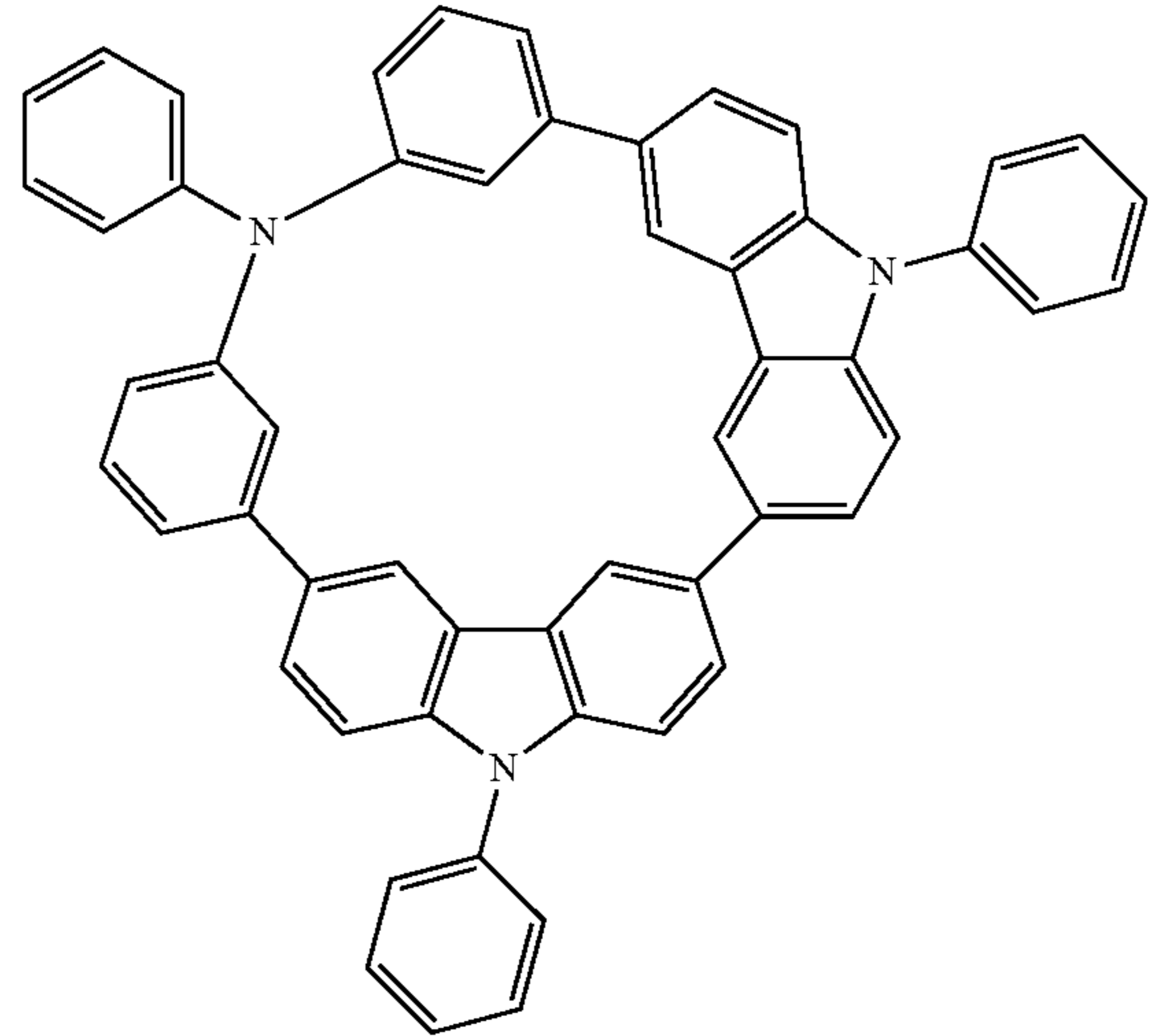
Compound 28
