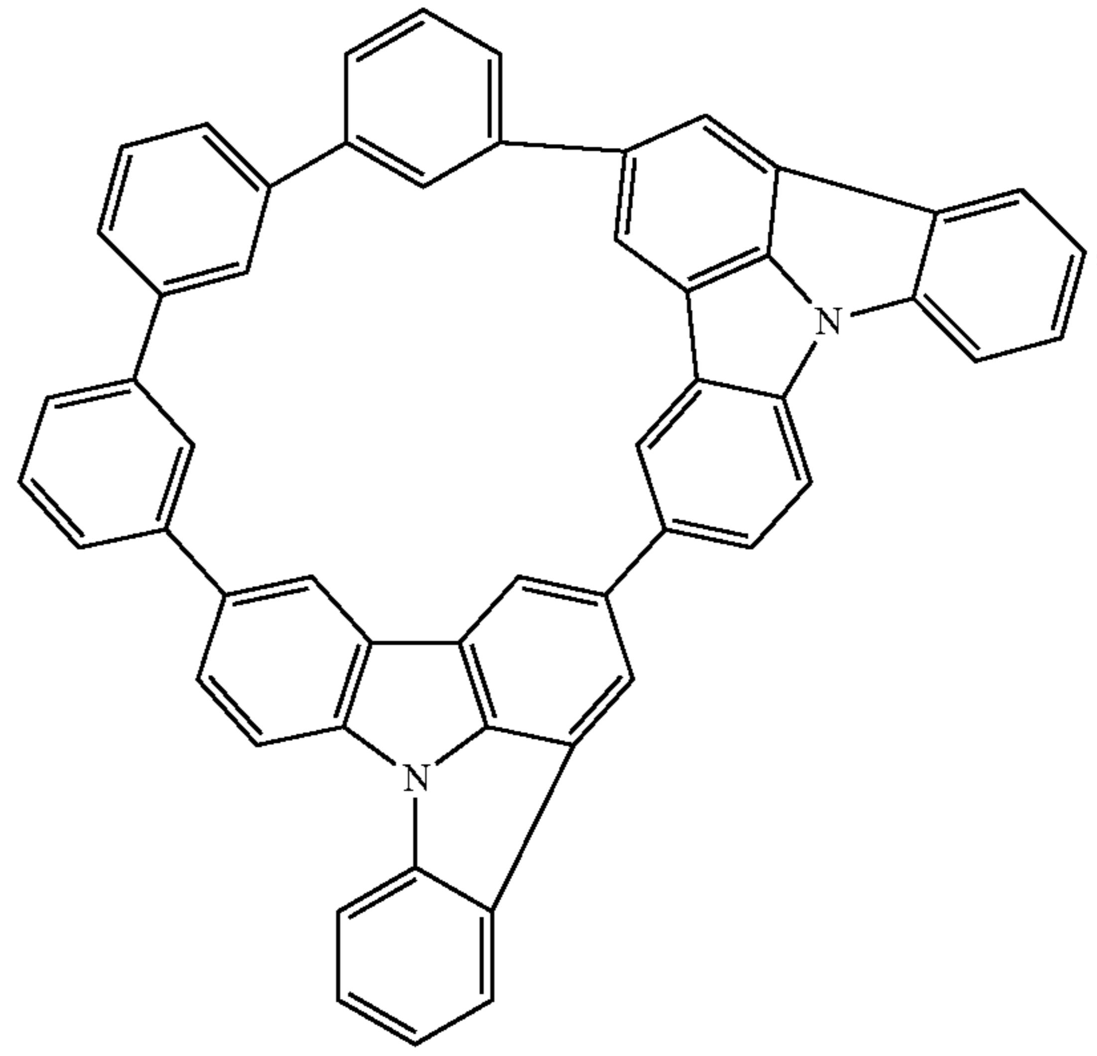
Compound 44
