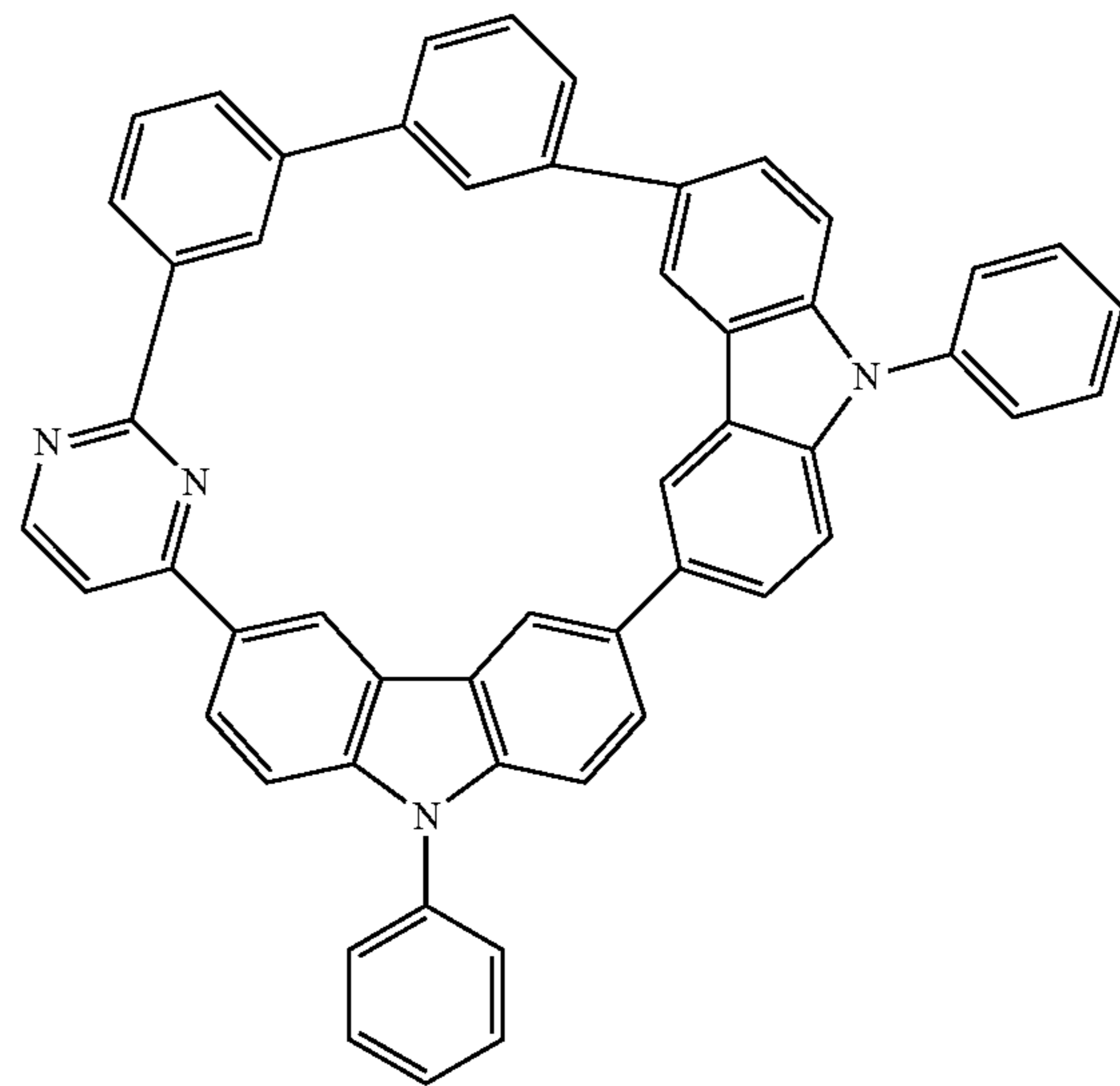
Compound 43
