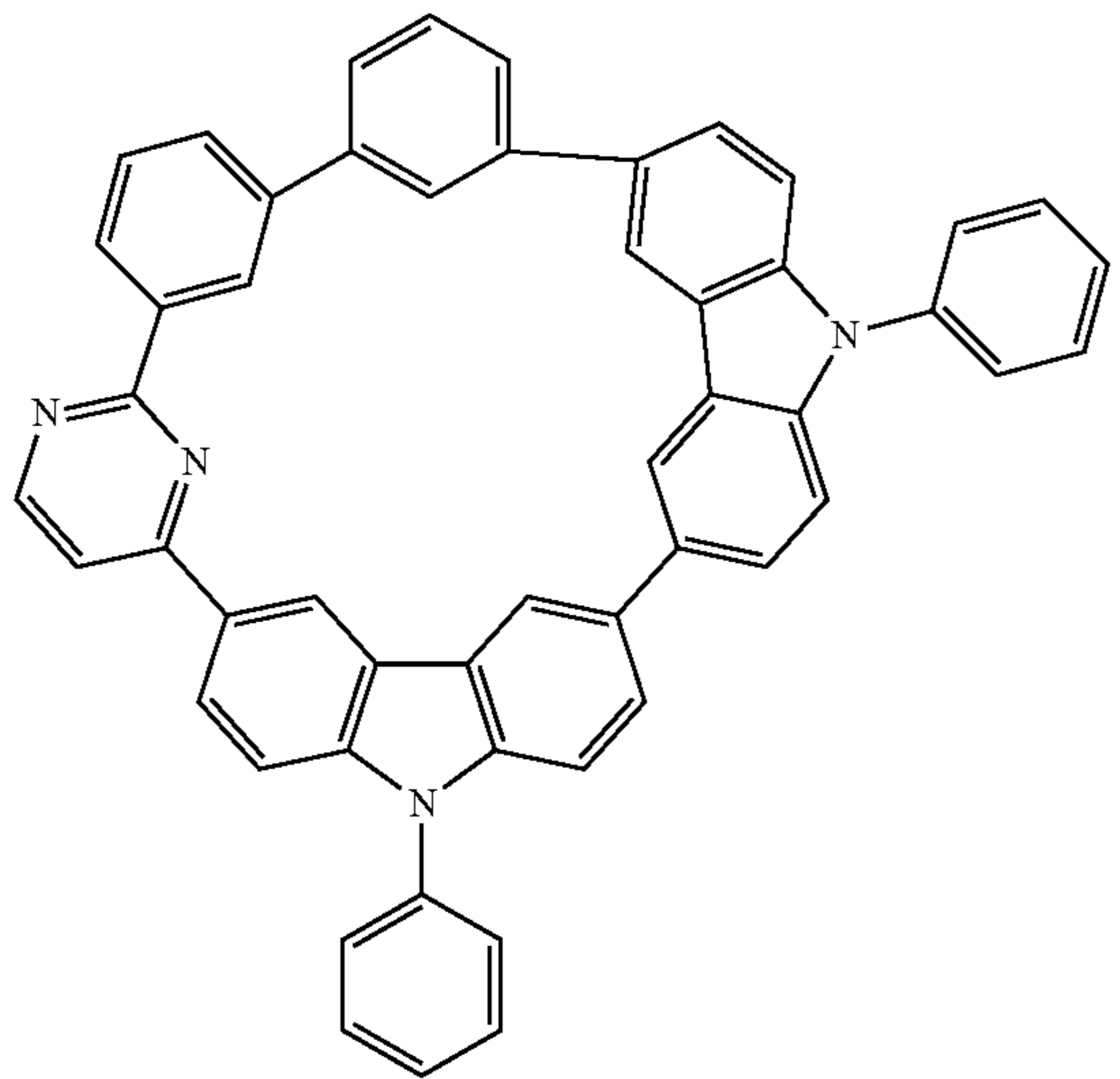
Compound 42
