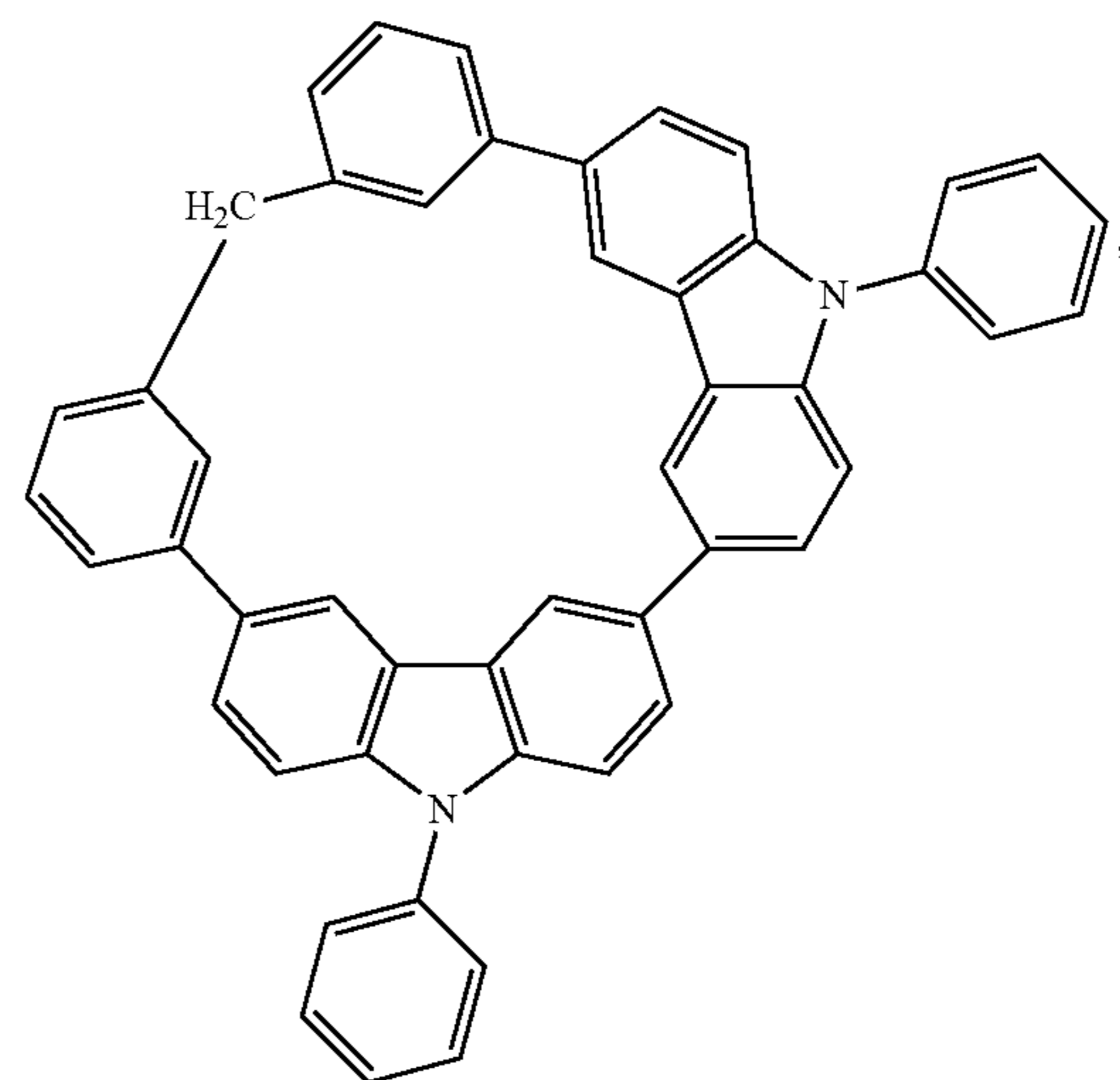
Compound 30
