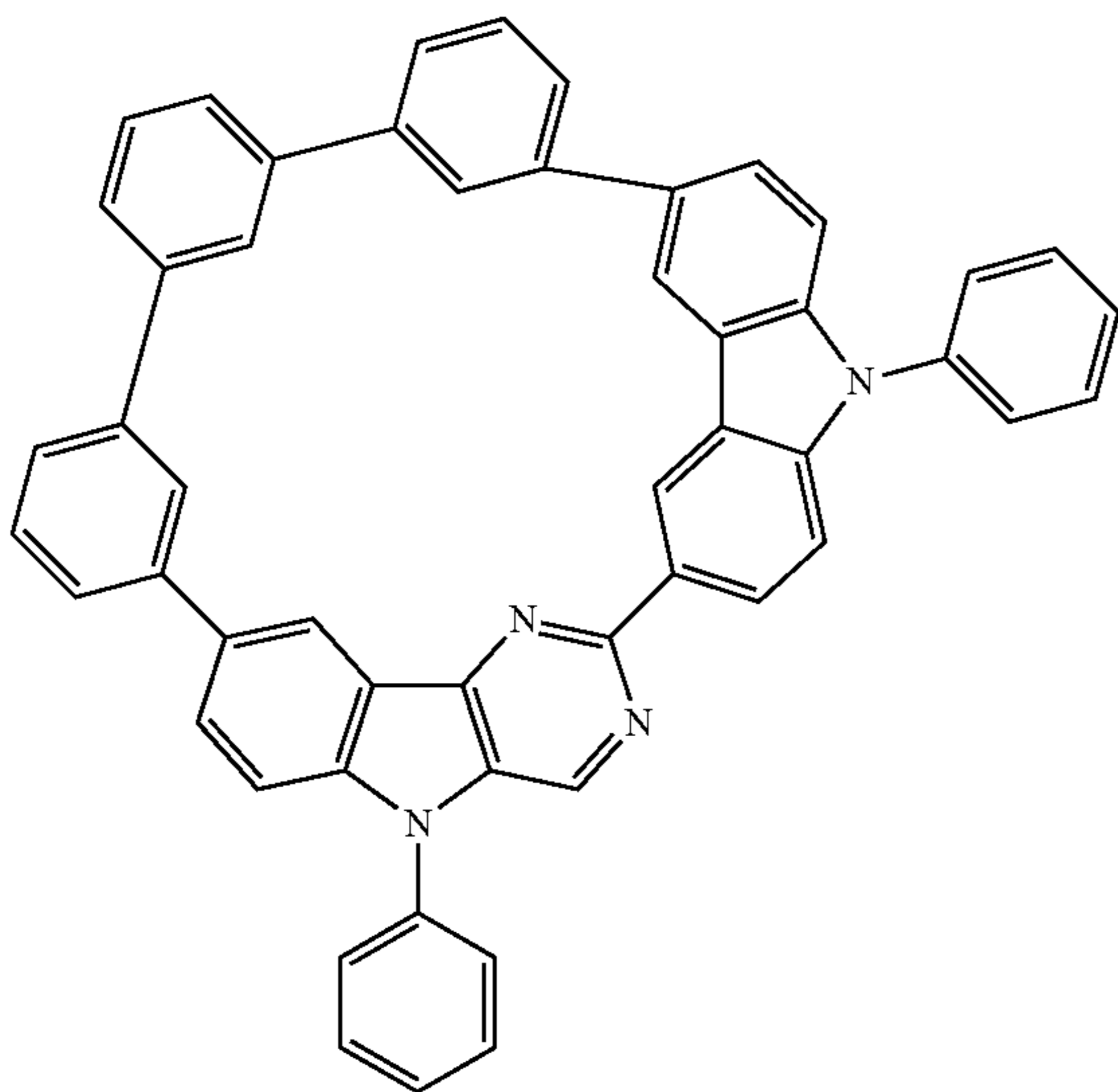
Compound 40
