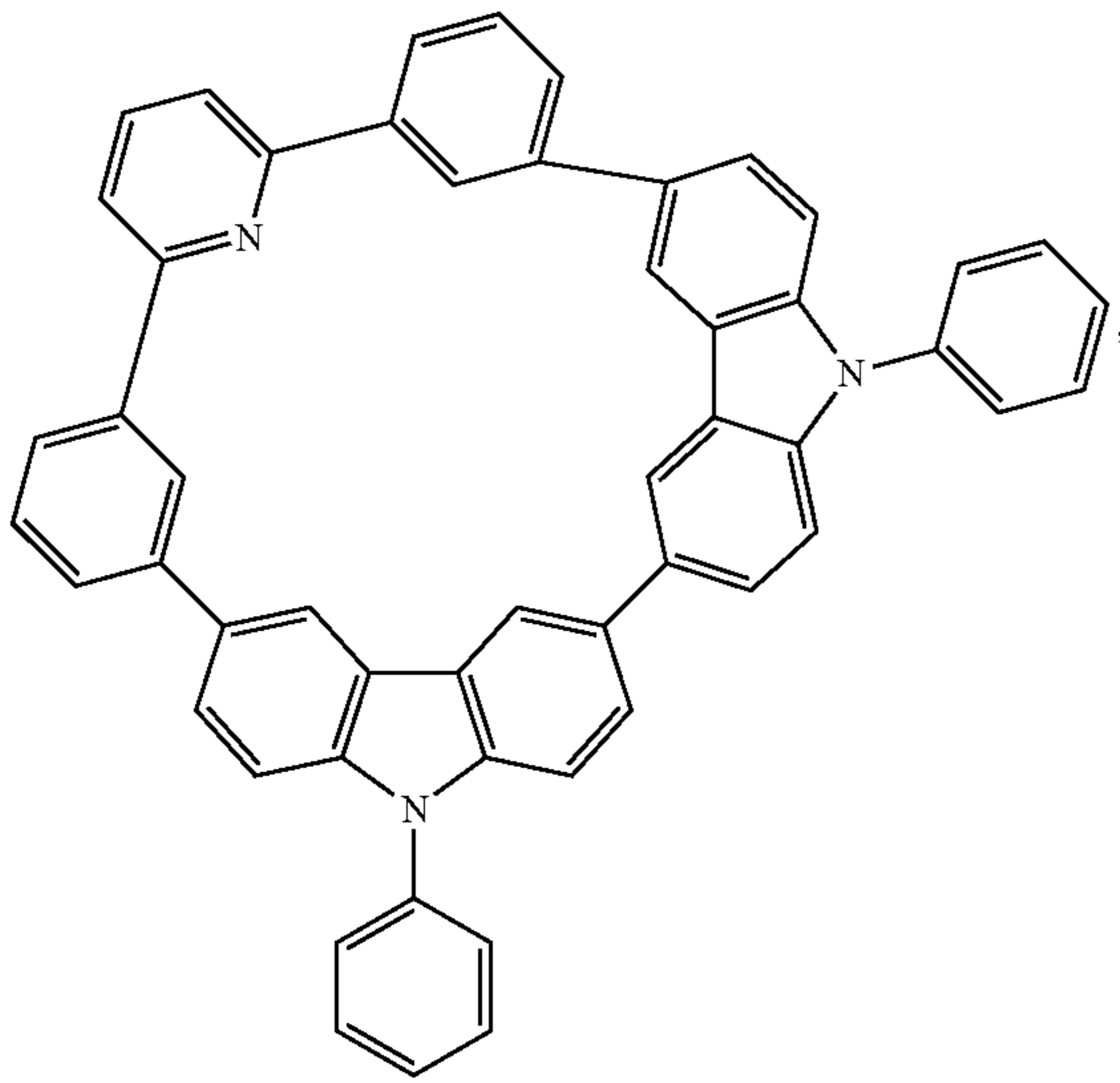
Compound 19
