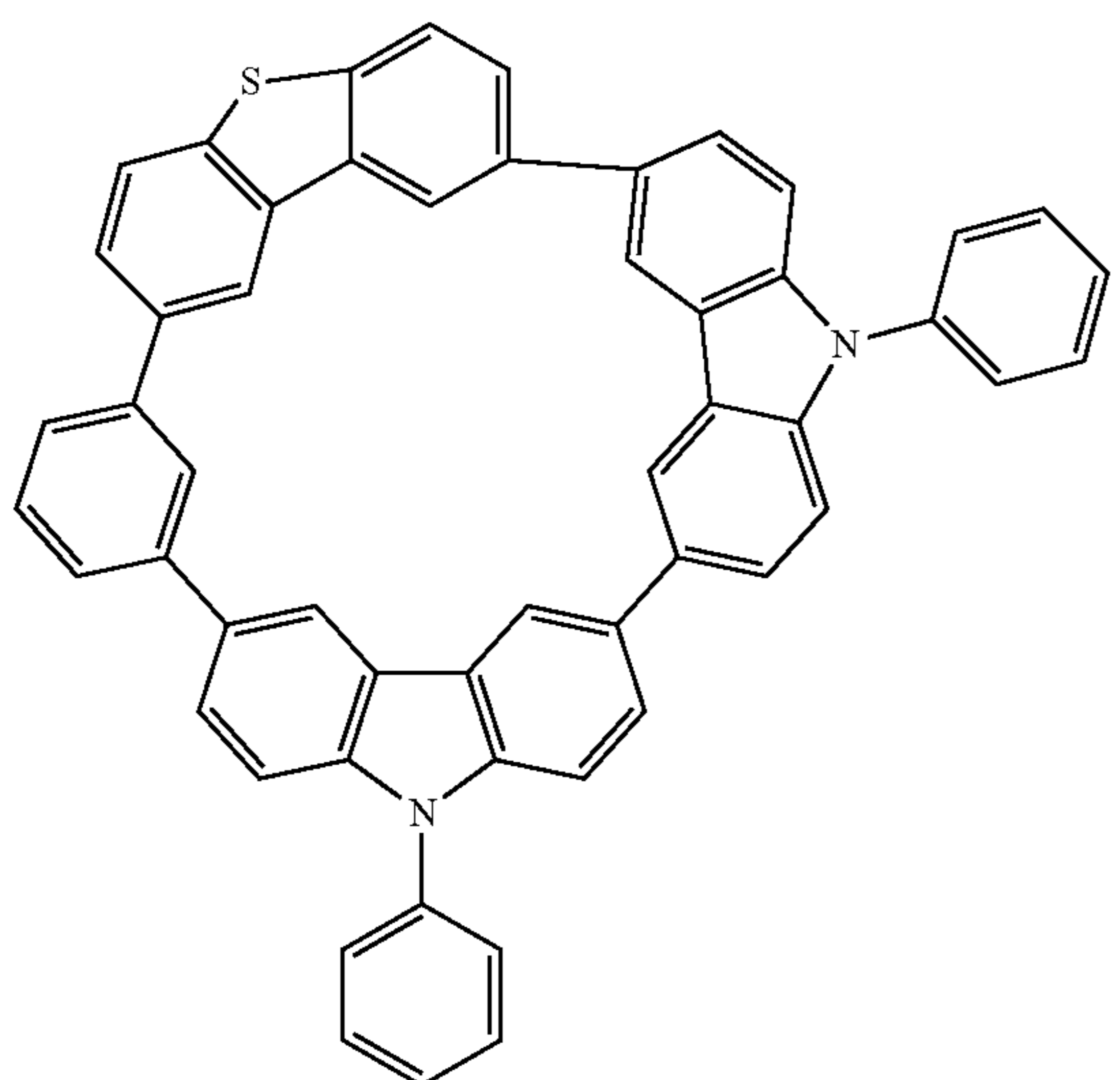
Compound 13
