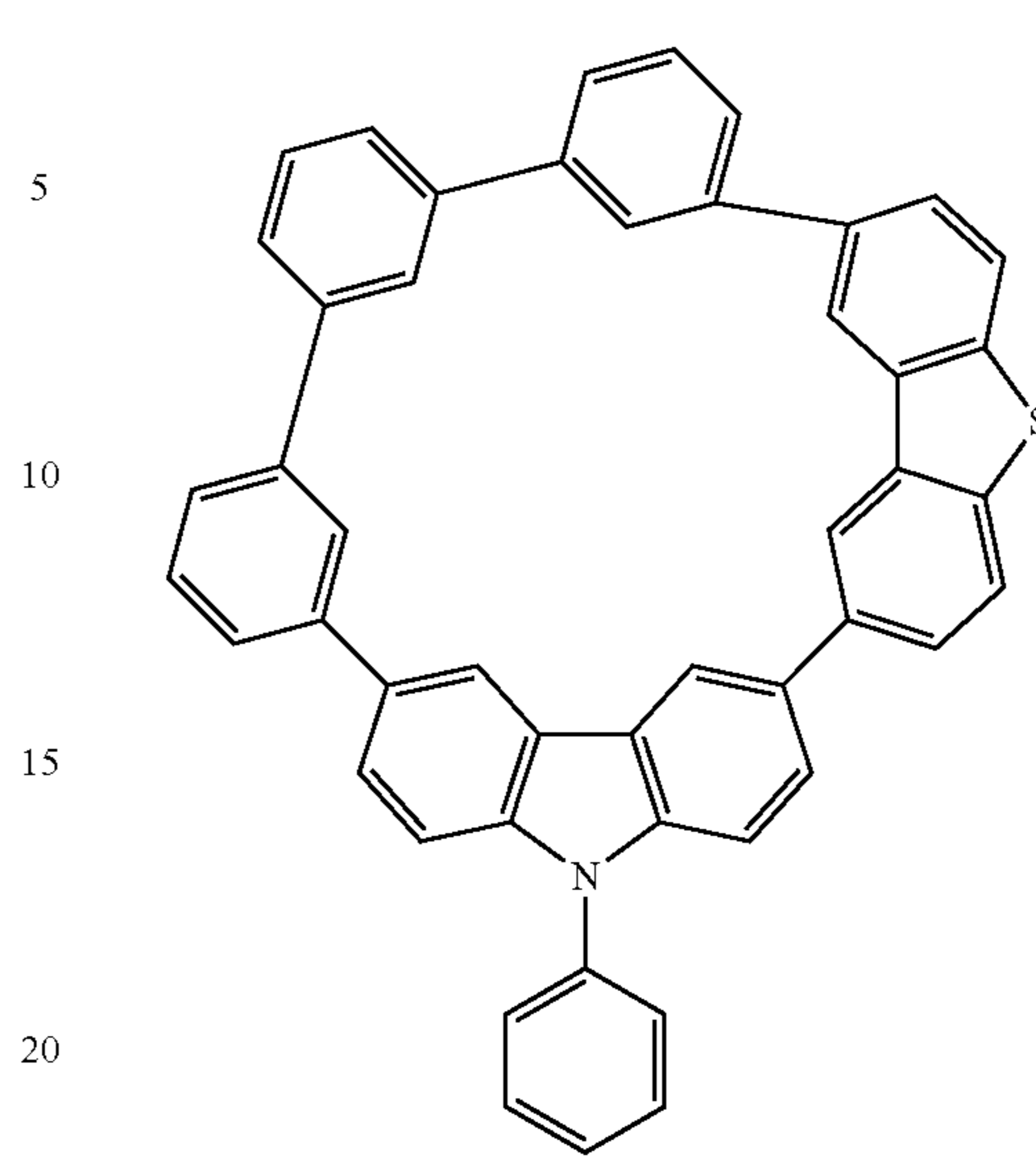
Compound 3
