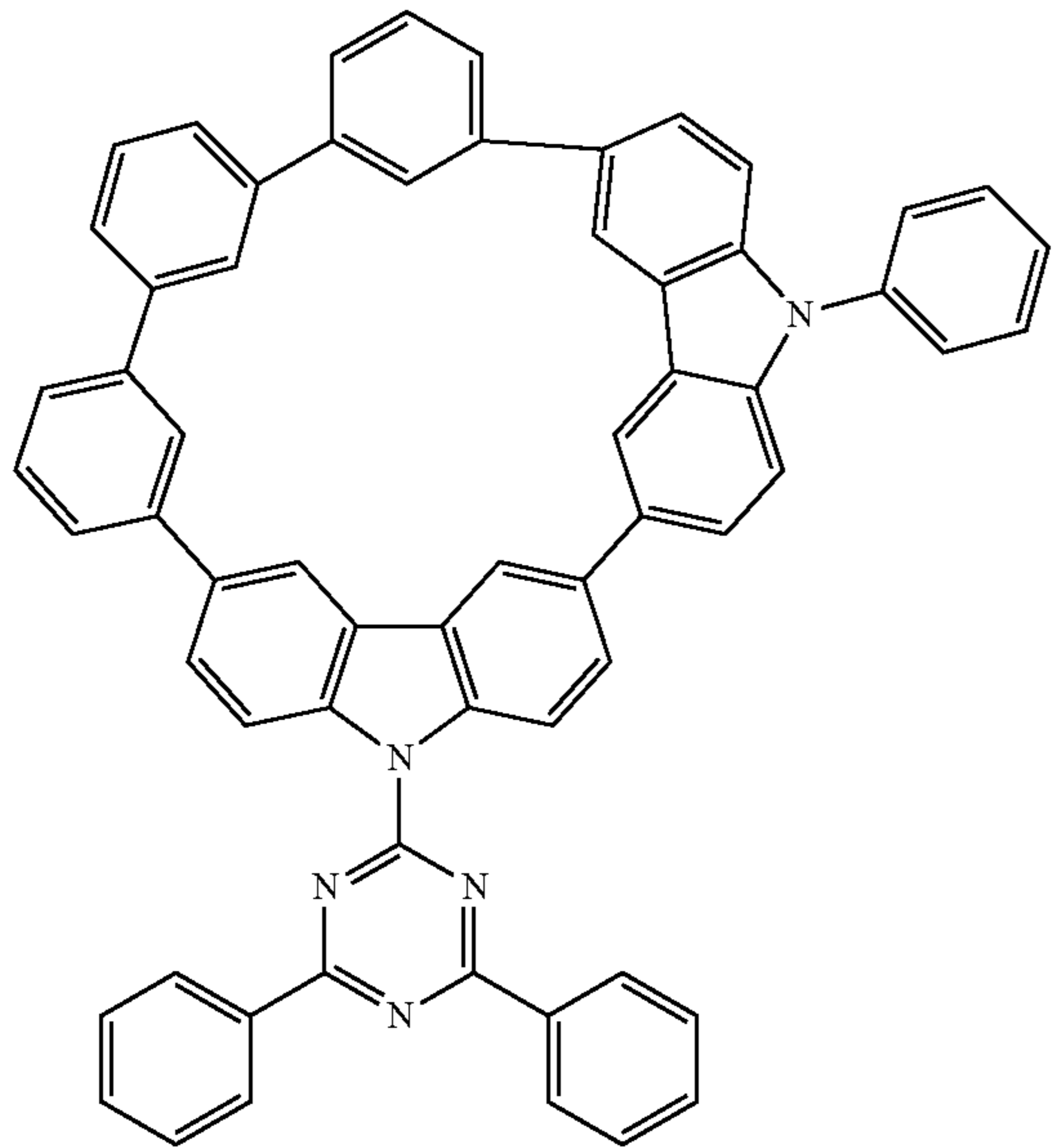
Compound 12
