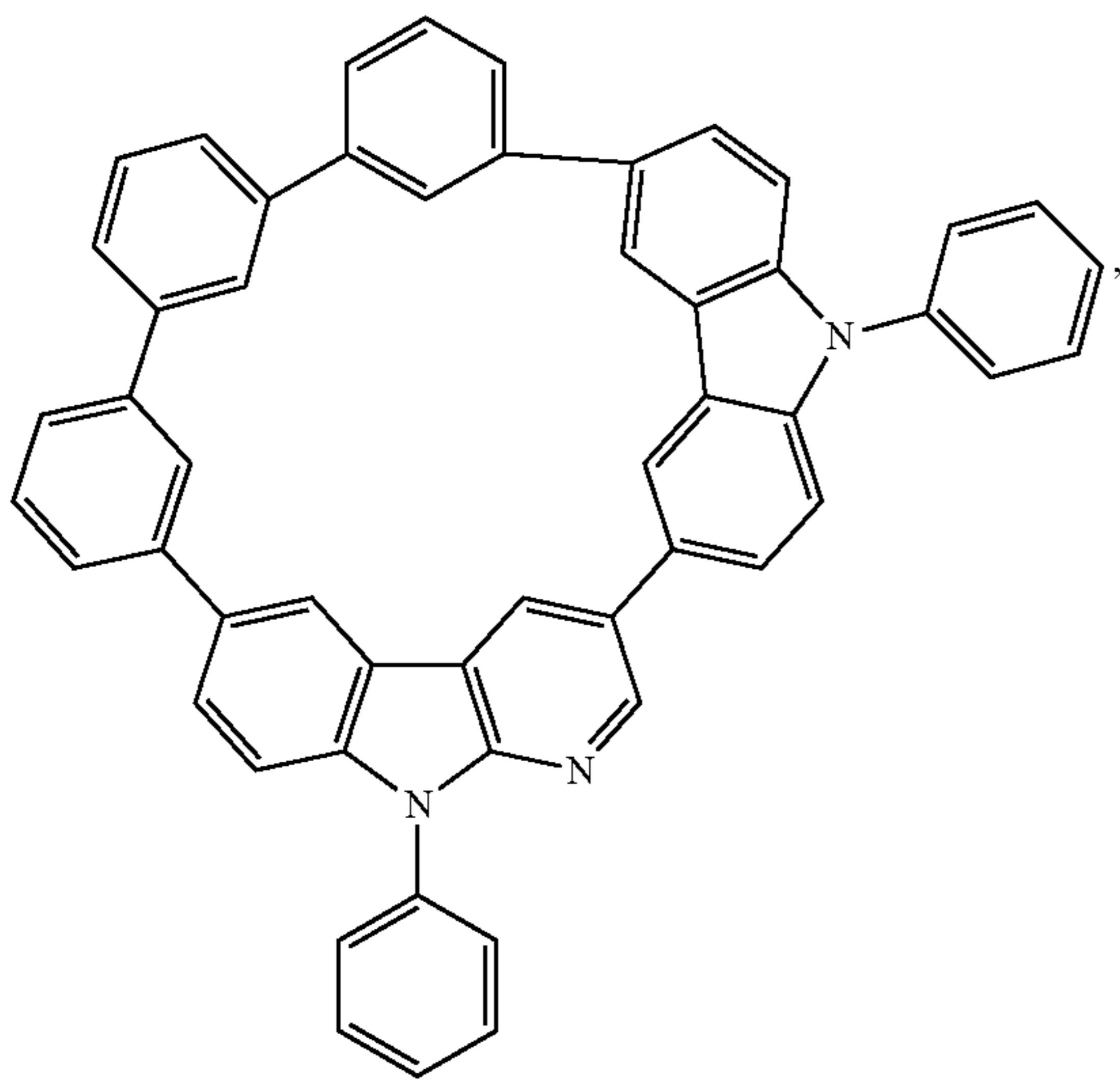
Compound 36
