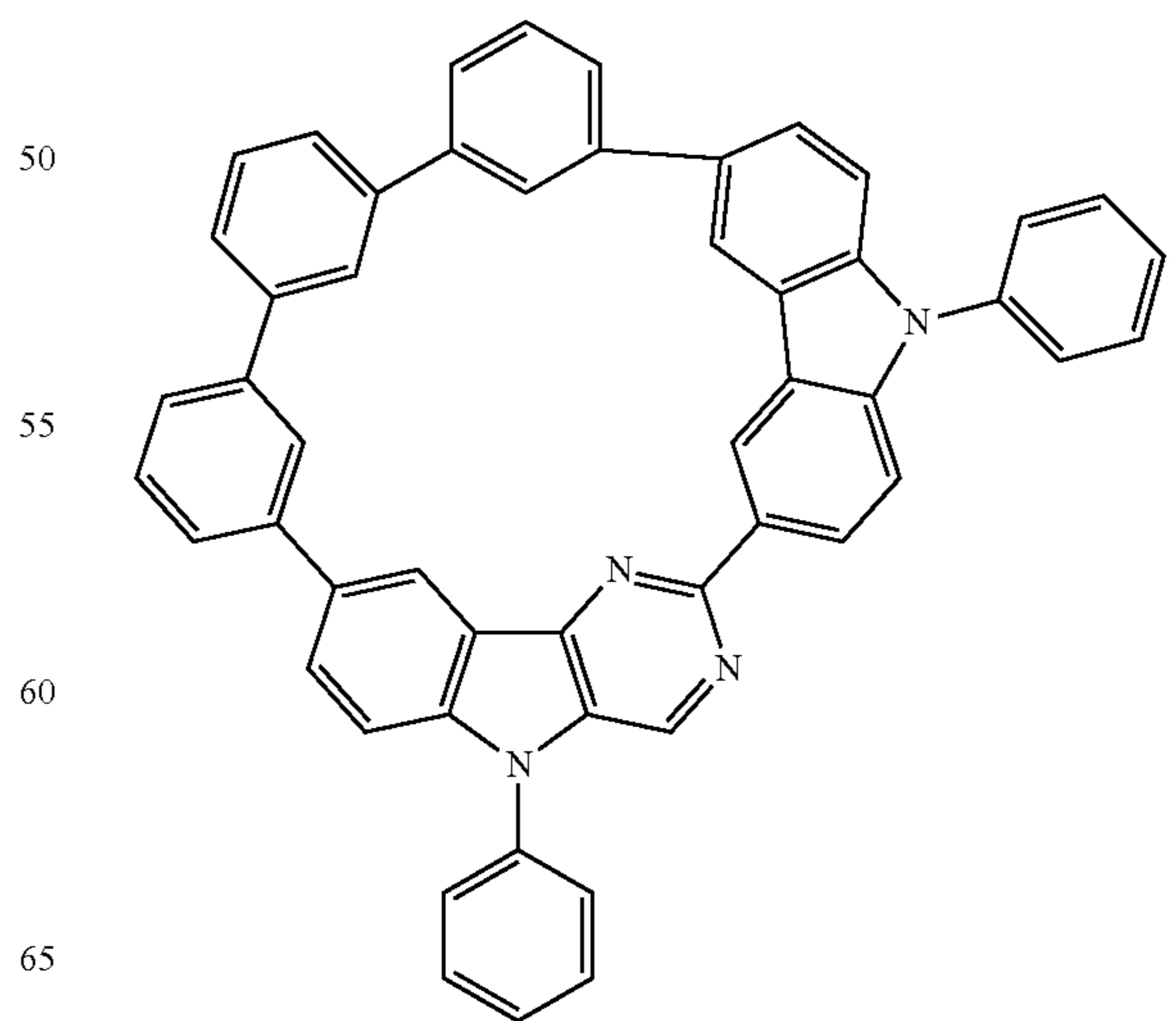
Compound 40
