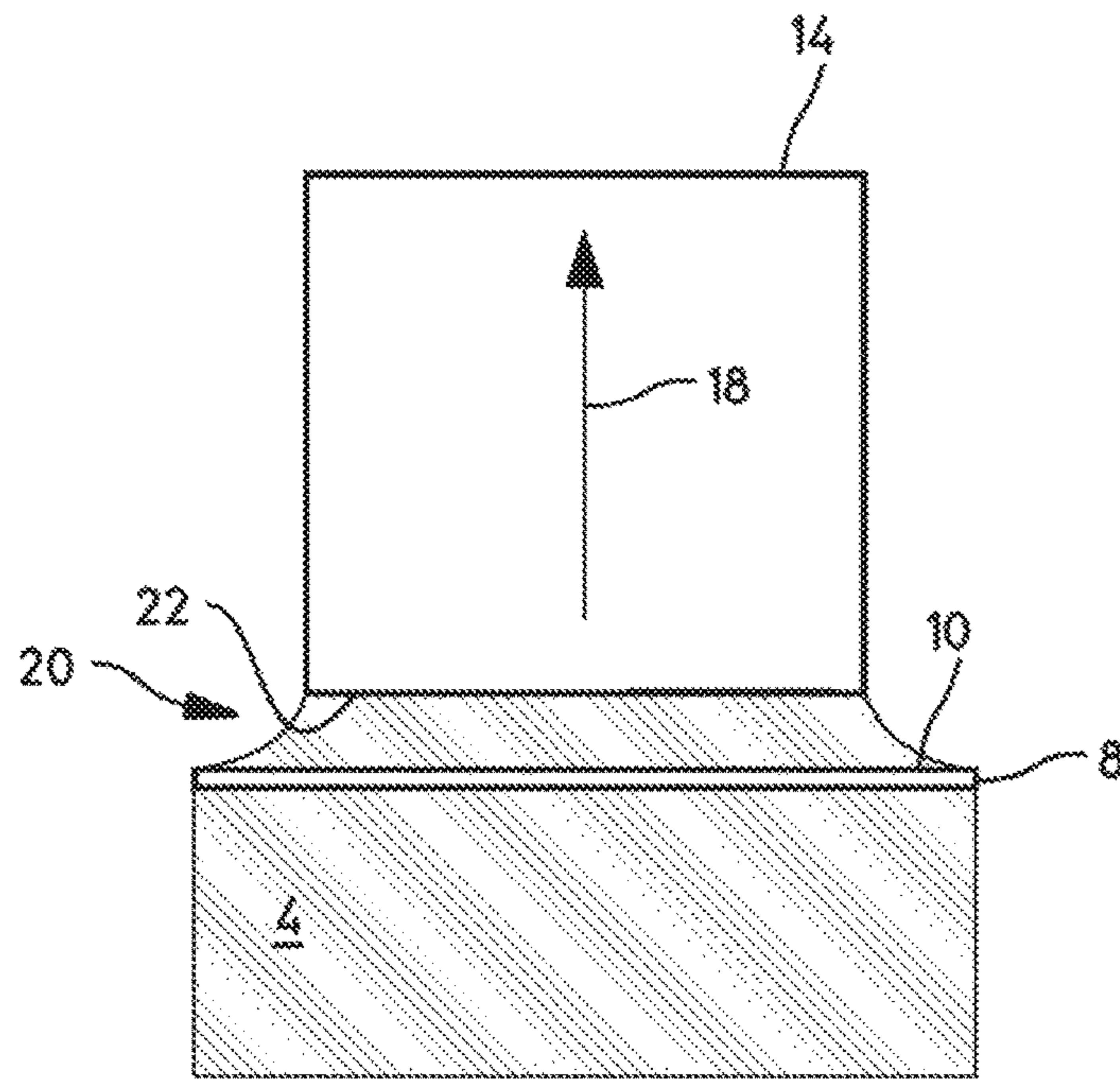
Fig. 1 PRIOR ART
