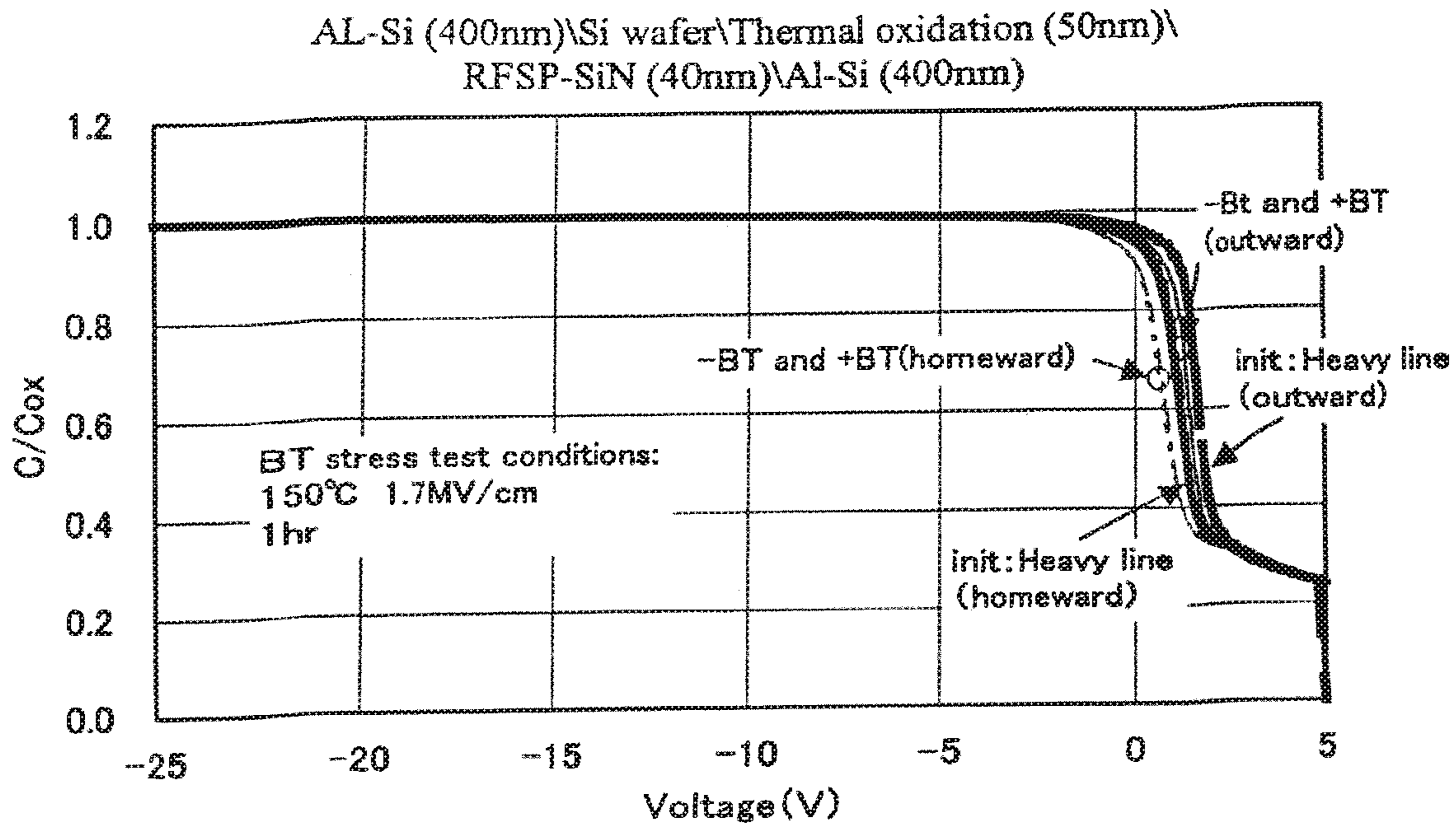
(A) C-V characteristics of MOS structure in case of not having Li diffusion source
