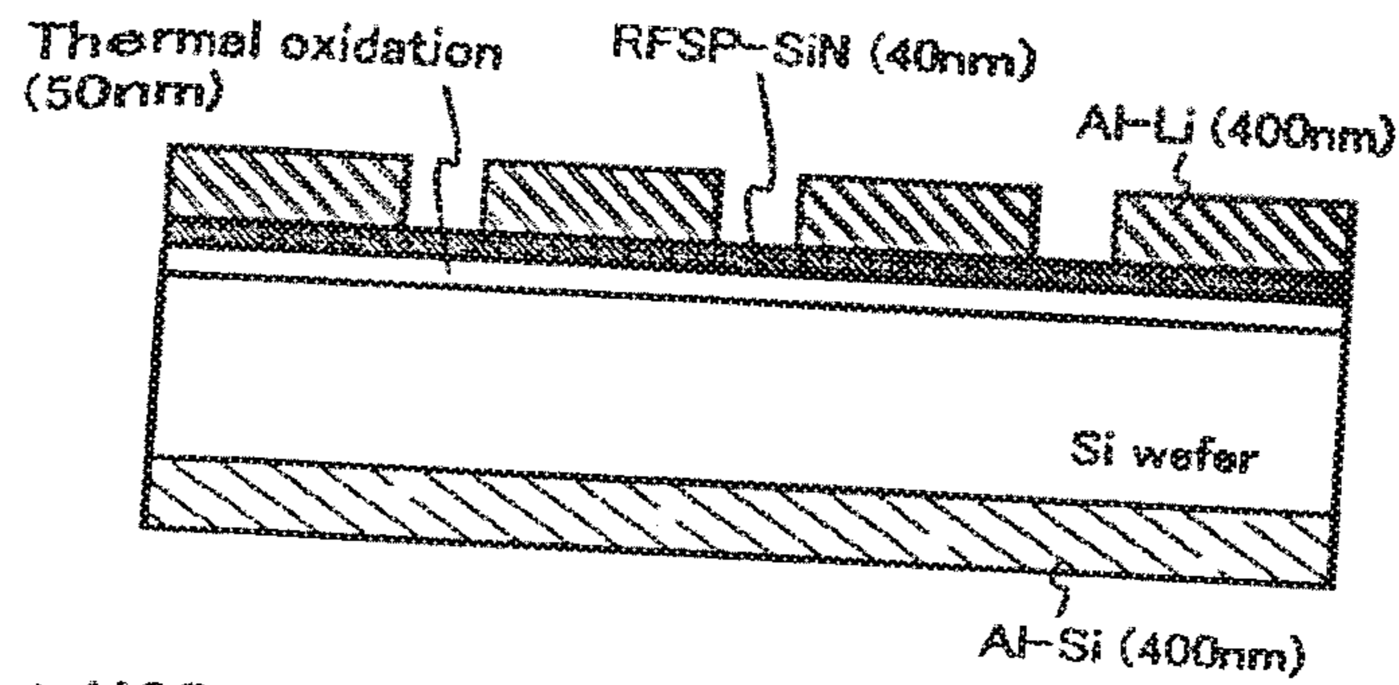
(B) MOS structure using RFSP-SiN film
