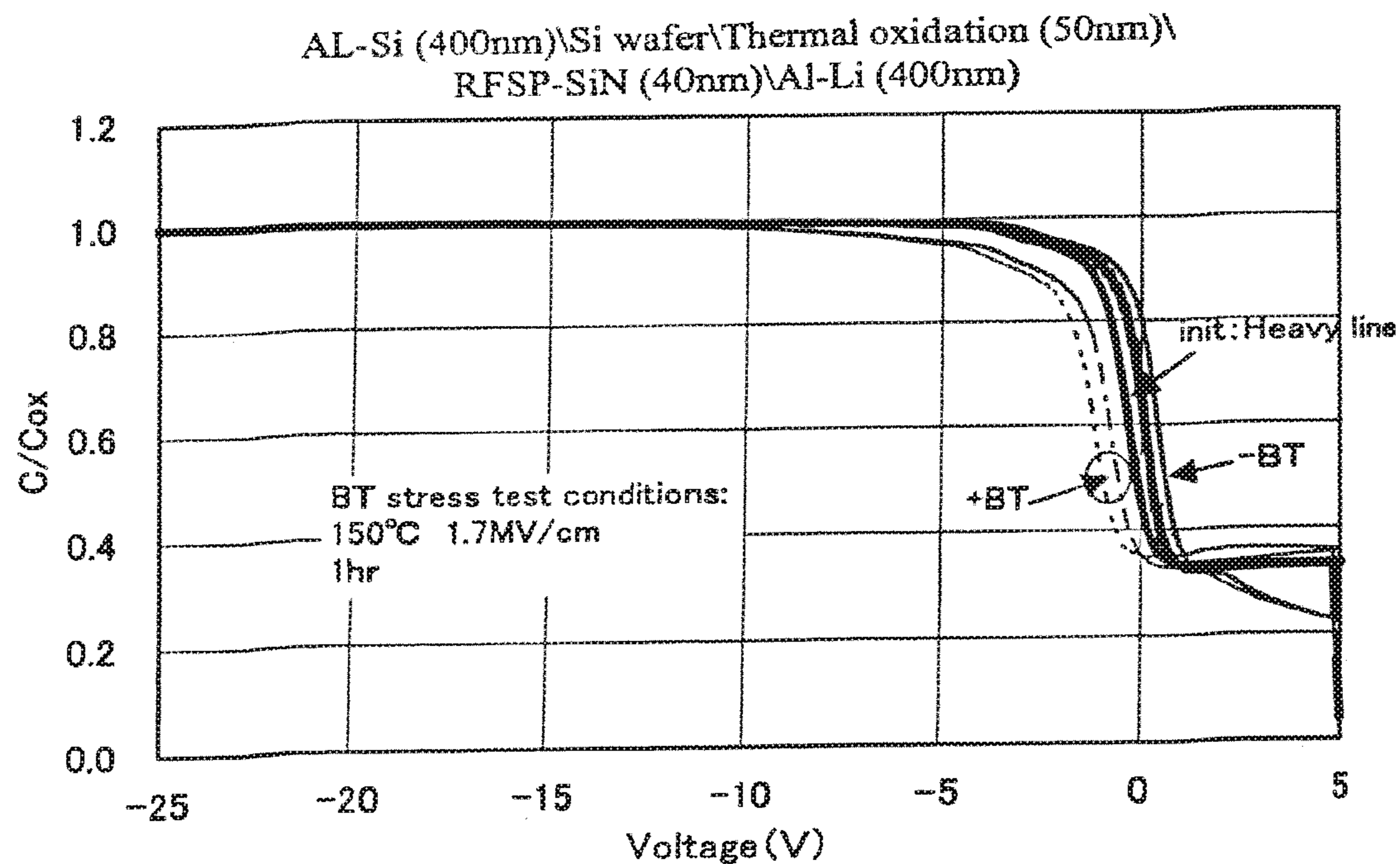
(B) C-V characteristics of MOS structure in case of having Li diffusion source
