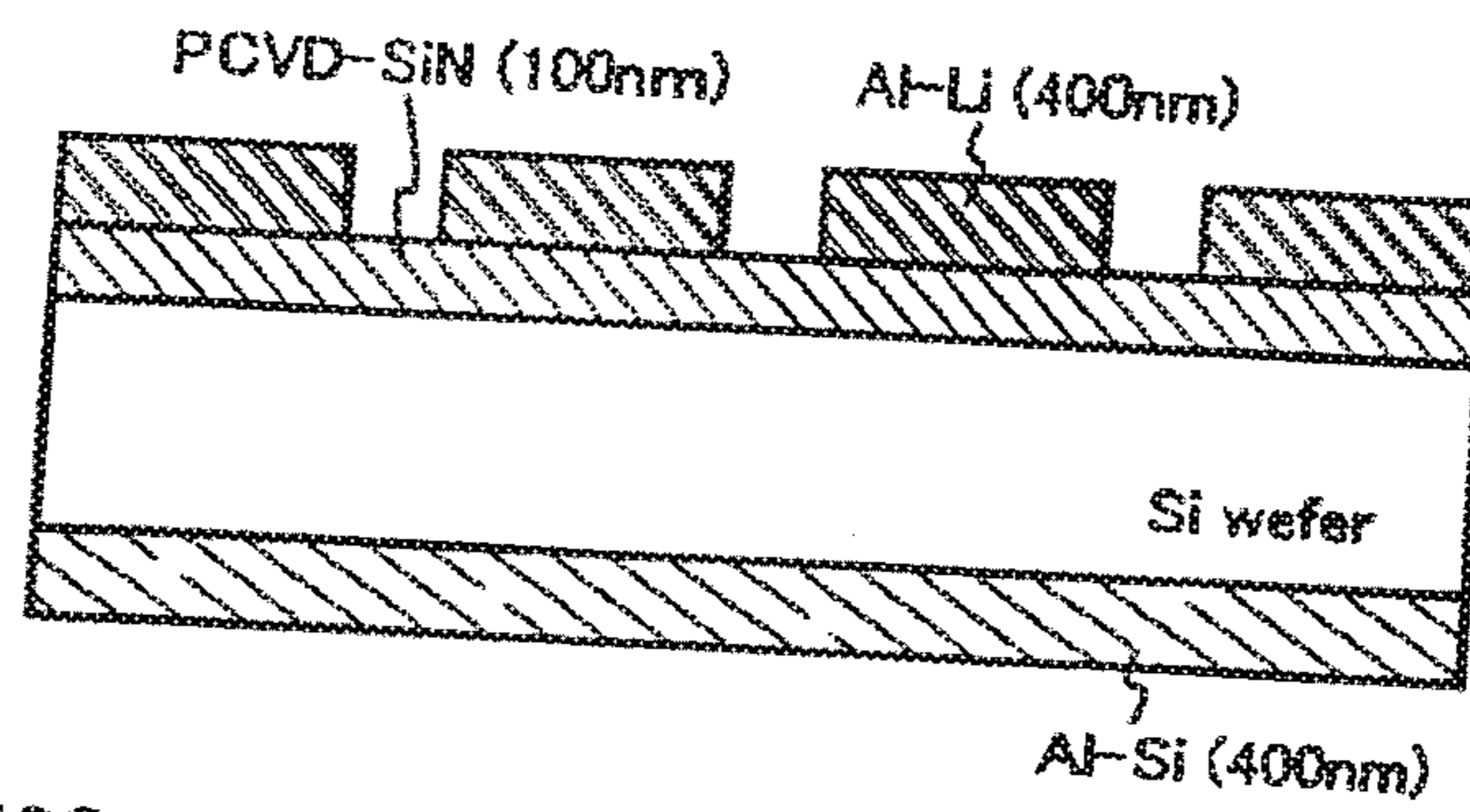
(A) MOS structure using PCVD-SiN film
