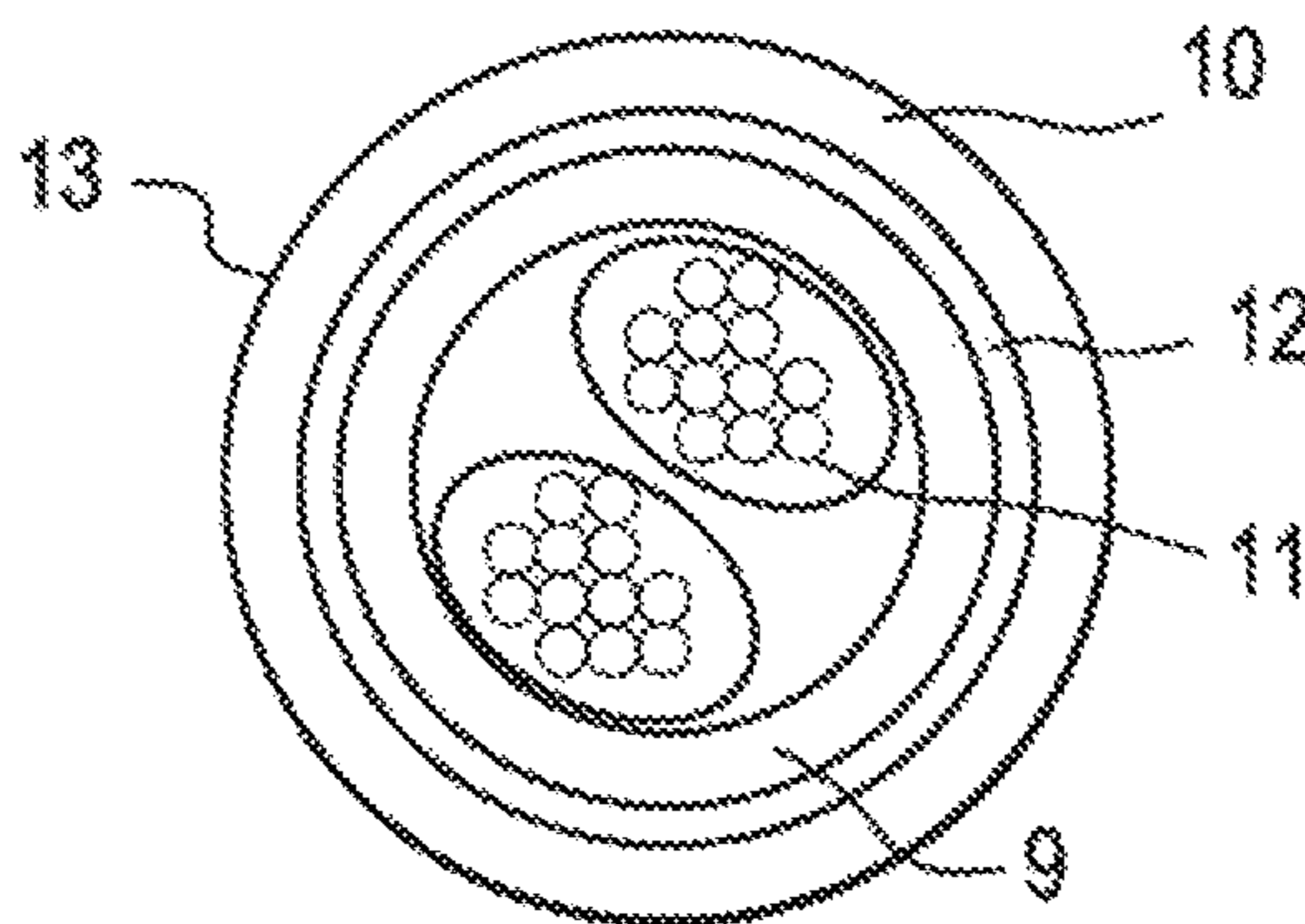
FIG. 3 RELATED ART
