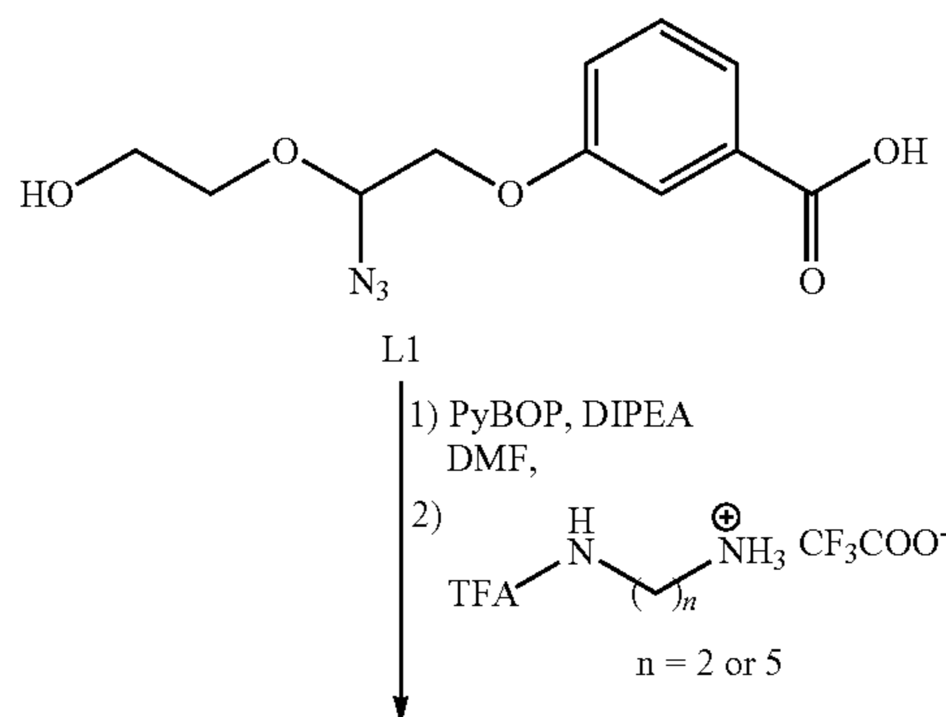
Scheme 1: Example of synthesis of two short pendant arm nucleotide triphosphate (pppT-sPA-Fl and pppT-sPA2-Fl, where Fl is a fluorophore)
