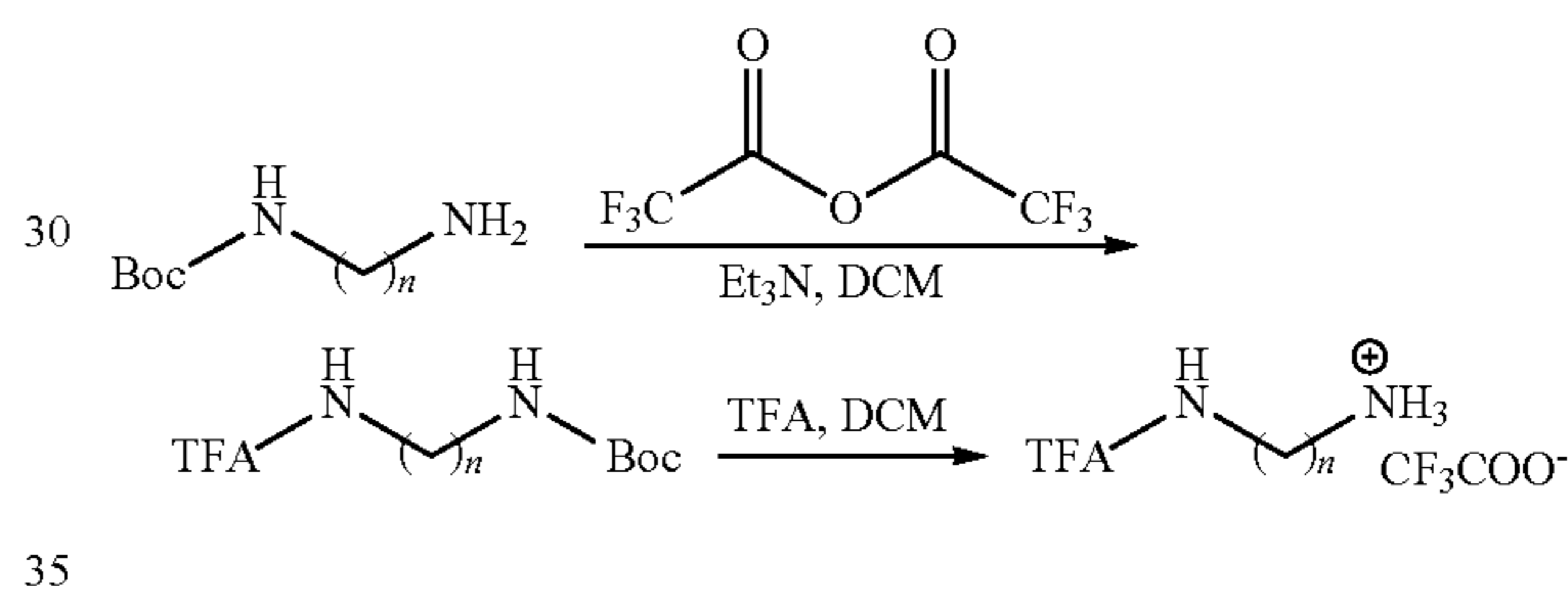
Scheme 2: General synthesis of \text{N} -trifluoroacetamido-diamine.
