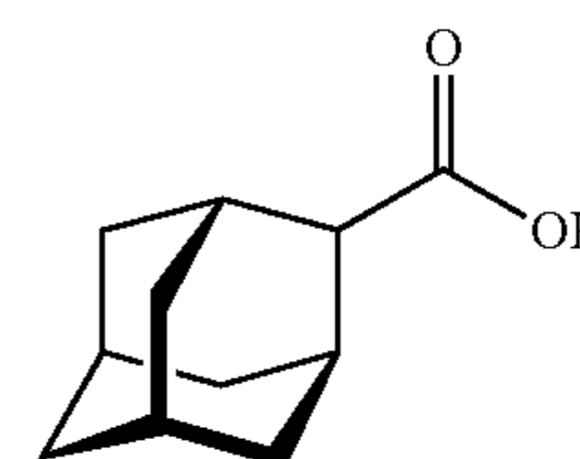
2-Adamantane Carboxylic Acid (23)
