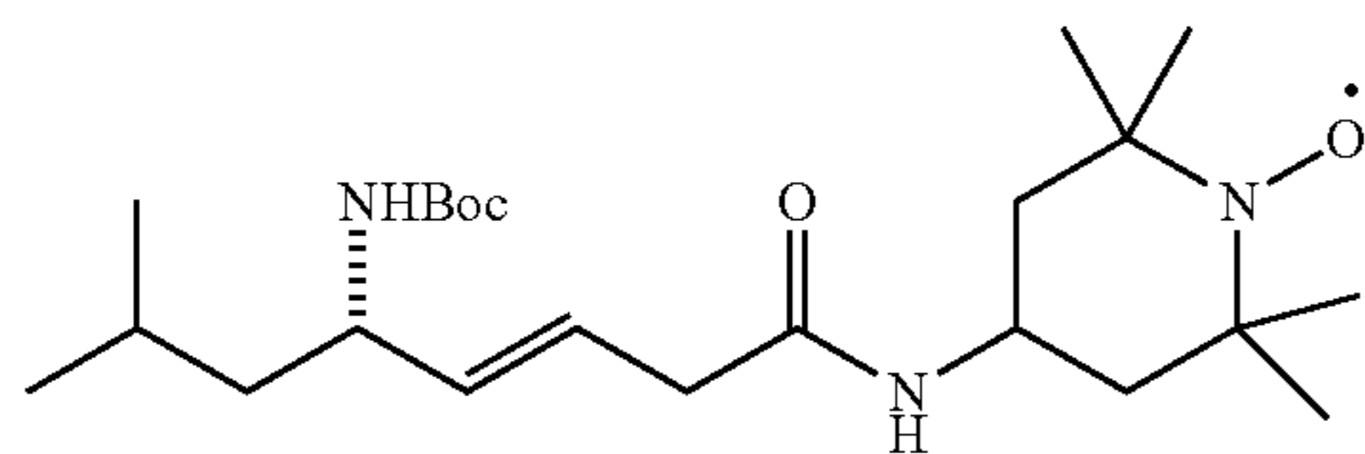
TEMPO-4-yl-(S,E)-5-(tert-butoxycarbonylamino)-7-methyloct-3-enamide (7)
