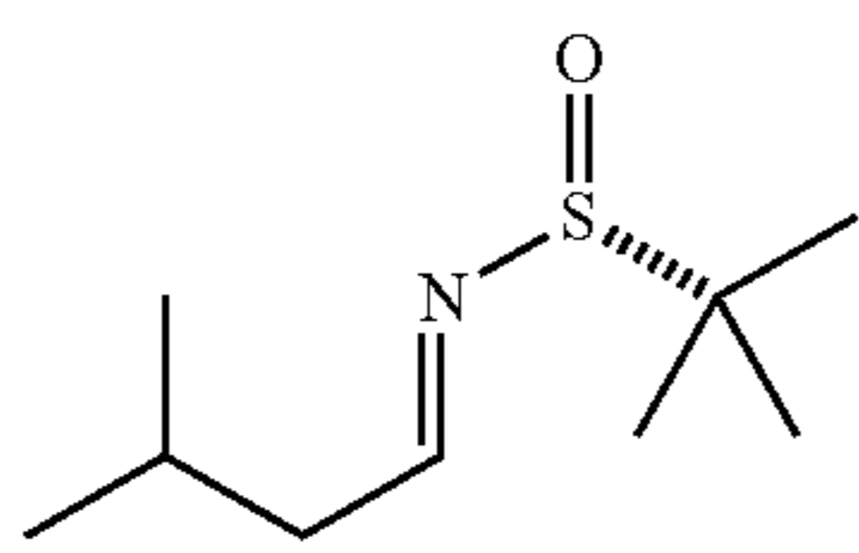
(R,E)-2-Methyl-N-(3-methylbutylidene)propane-2-sulfonamide (1)
