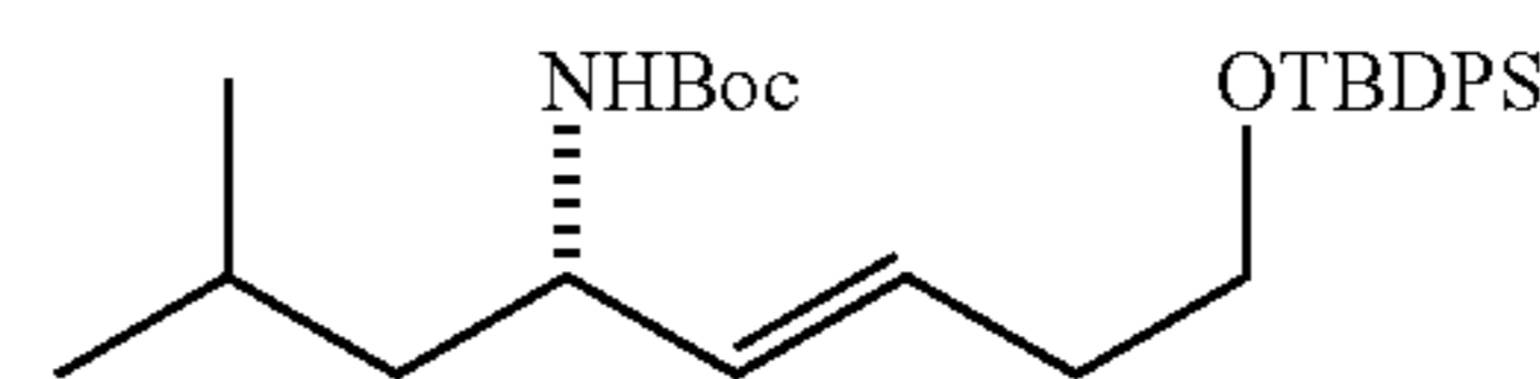
(S,E)-tert-Butyl 8-(tert-butyldiphenylsilyloxy)-2-methyloct-5-en-4-ylcarbamate (4)
