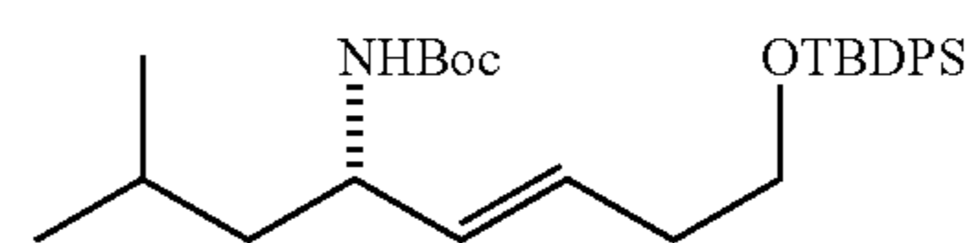
(S,E)-tert-Butyl 8-(tert-butyldiphenylsilyloxy)-2-methyloct-5-en-4-ylcarbamate (4)
