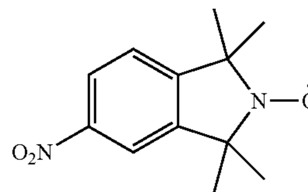
5-Nitro-1,1,3,3-tetramethylisoindolin-2-yloxy (19)
