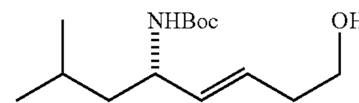
(S,E)-tert-Butyl 8-hydroxy-2-methyloct-5-en-4-ylcarbamate (5)
