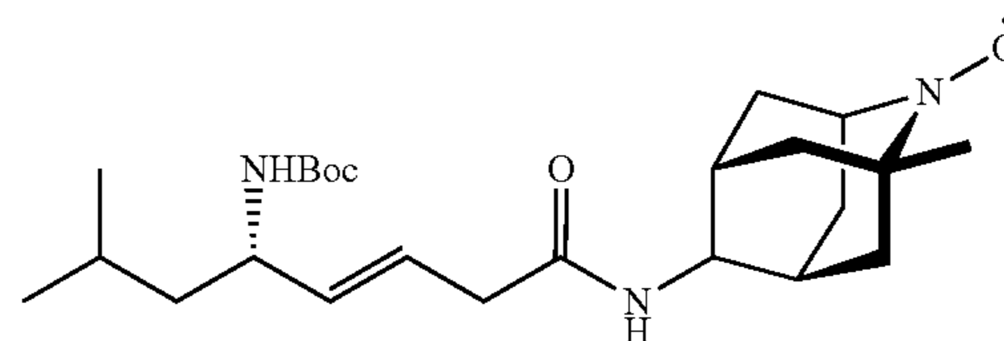
(1-Me-AZADO-6-yl)-(S,E)-5-(tert-butoxycarbo- nylamino)-7-methyloct-3-enamide (30)
