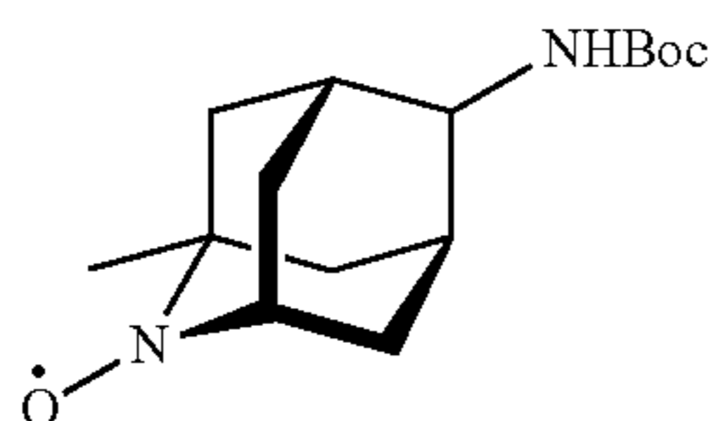
(1-Methyl-2-azaadamantane-N-oxyl-6-yl)-carbamic Acid Tert-Butyl Ester (29)
