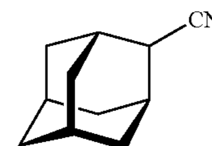
2-Adamantanecarbonitrile (tricyclo[3.3.1.1.3,7]decan-2-carbonitrile, 22)
