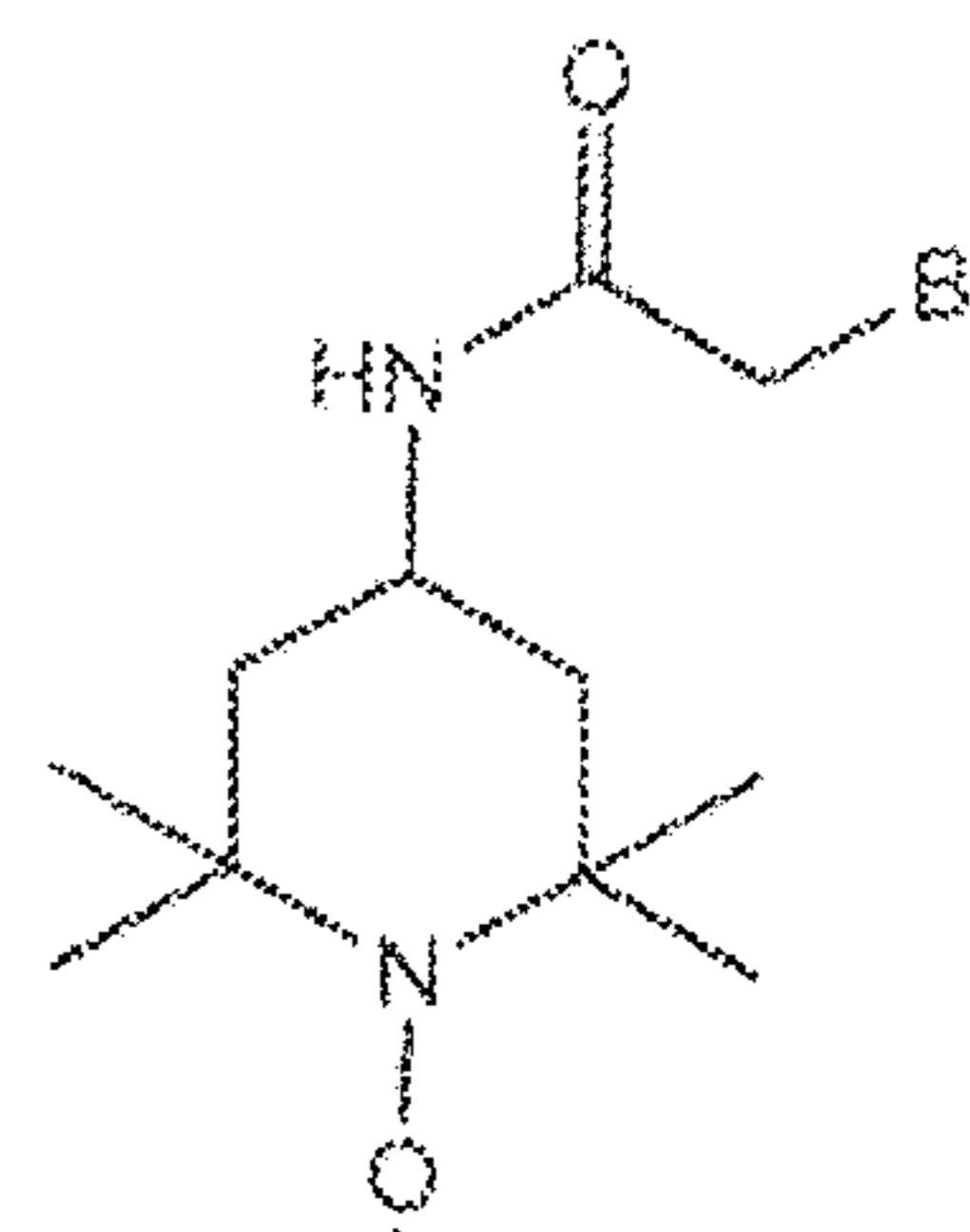
4-(2-Bromoacetamido)- TEMPO, LogP=1.9
