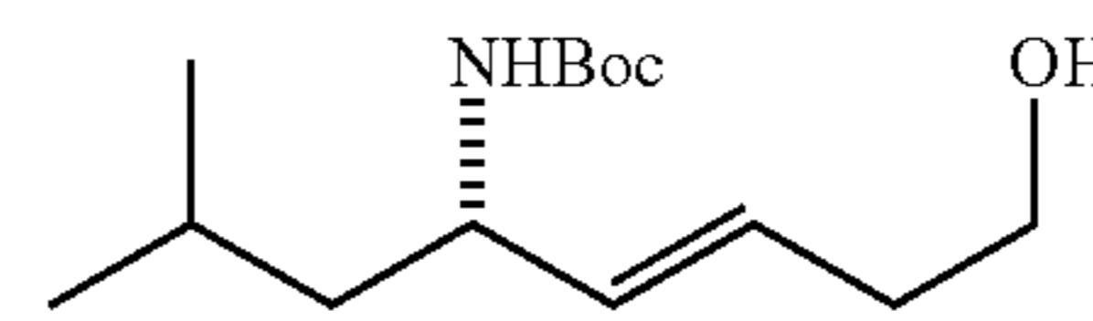
(S,E)-tert-Butyl 8-hydroxy-2-methyloct-5-en-4-ylcarbamate (5)
