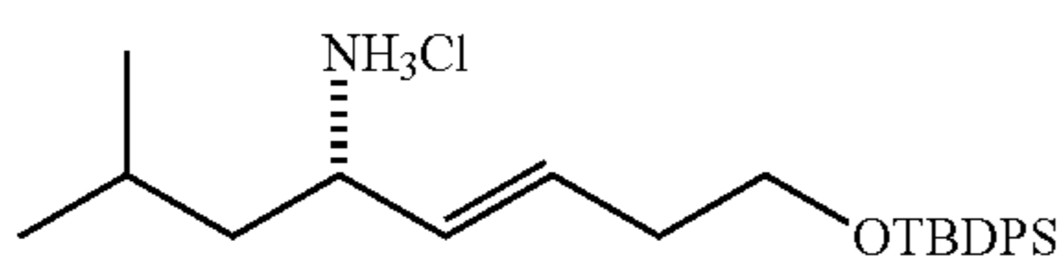
(S,E)-8-(tert-Butyldiphenylsilyloxy)-2-methyloct-5-en-4-amine hydrochloride (3)
