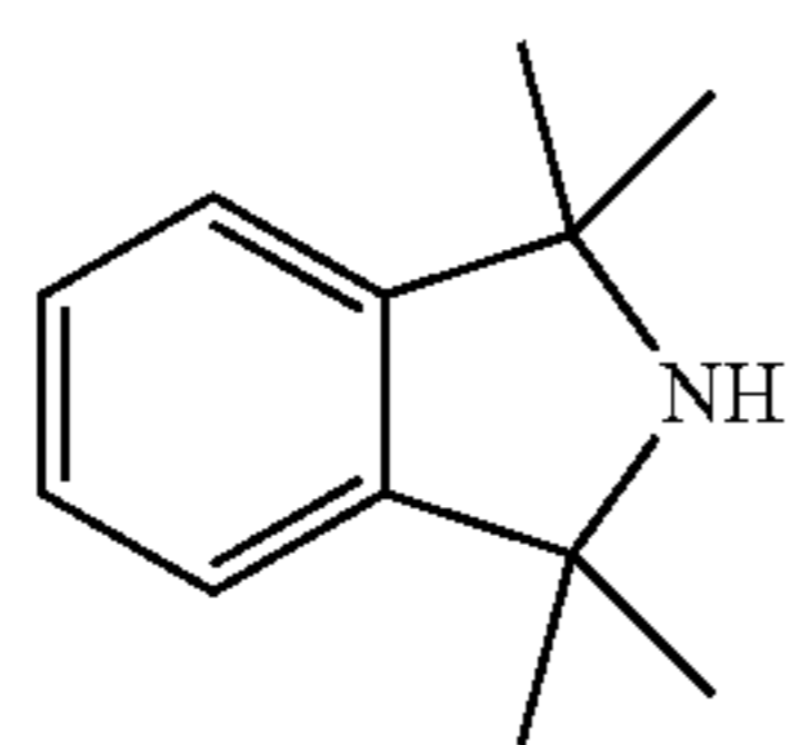
1,1,3,3-Tetramethylisoindoline (17)
