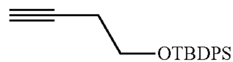
(But-3-ynoxy)(tert-butyl)diphenylsilane (2)
