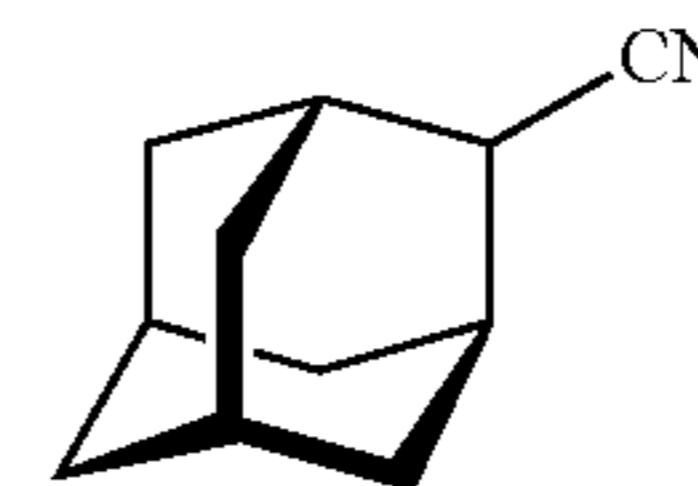
2-Adamantanecarbonitrile (tricyclo[3.3.1.1.3,7]decan-2-carbonitrile, 22)
