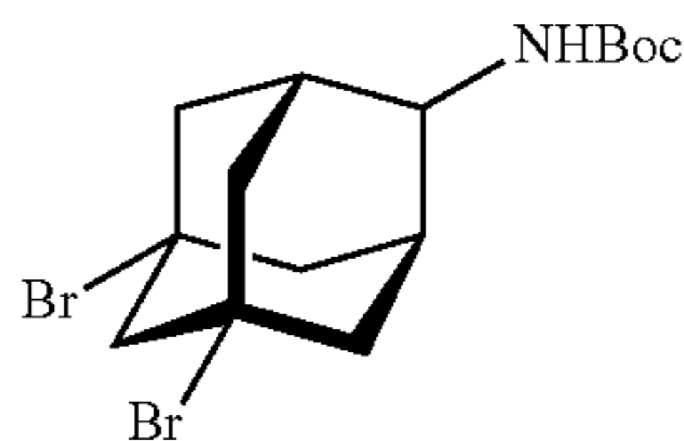
(5,7-Dibromo-adamantan-2-yl)-carbamic Acid Tert-Butyl Ester (25)
