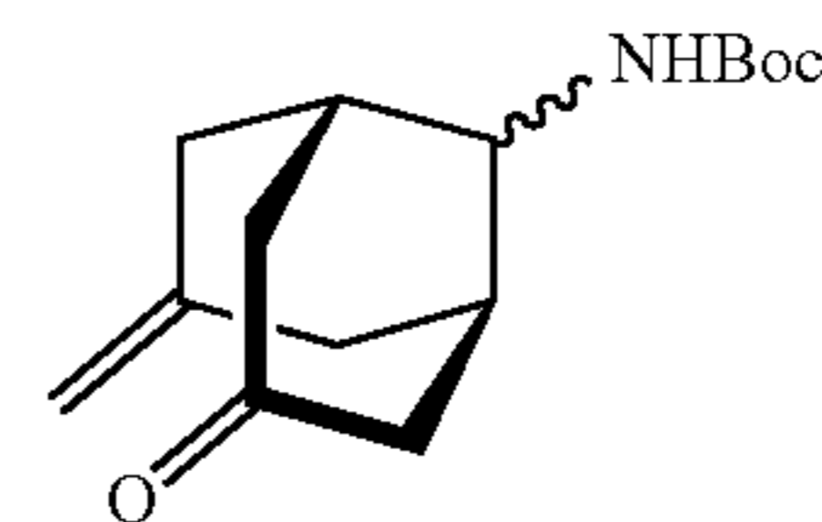
(7-Methylene-bicyclo[3.3.1]nonan-3-one-9-yl)-carbamic Acid Tert-Butyl Ester (26)
