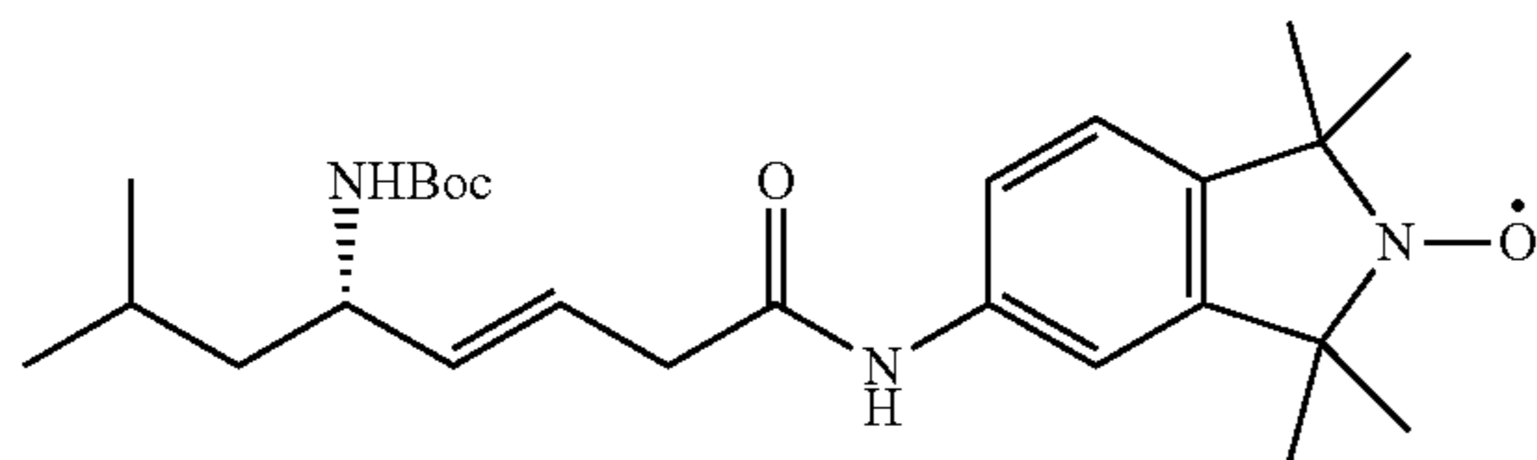
TMIO-5-yl-(S,E)-5-(tert-butoxycarbonylamino)-7-methyloct-3-enamide (20)
