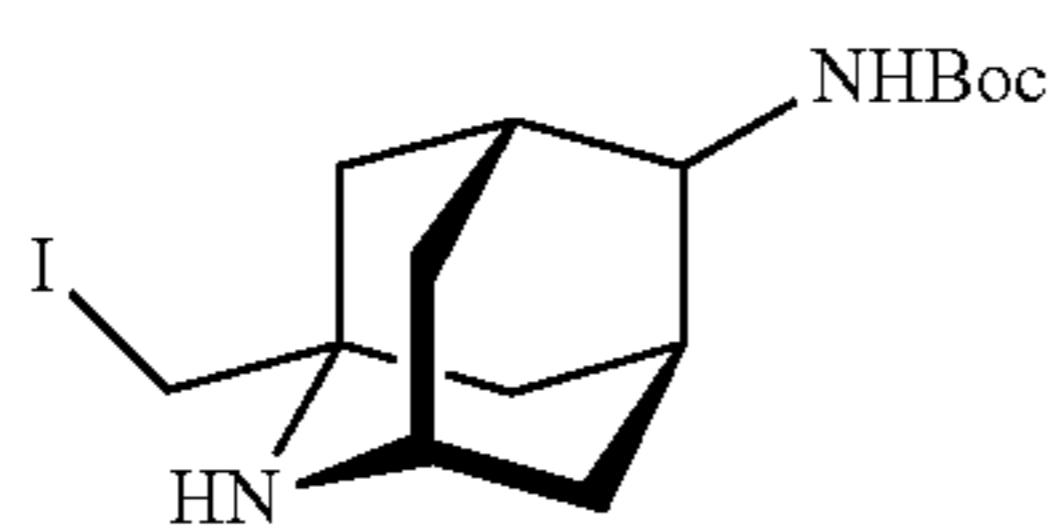
(1-Iodomethyl-2-azaadamantan-6-yl)-carbamic Acid Tert-Butyl Ester (28)
