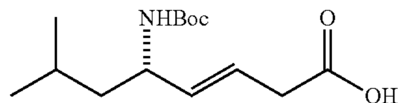
(S,E)-5-(tert-Butoxycarbonylamino)-7-methyloct-3-enoic acid (6)
