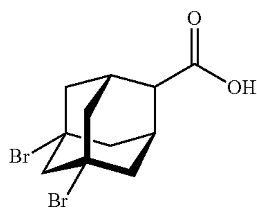
5,7-Dibromo-2-adamantane Carboxylic Acid (24)
