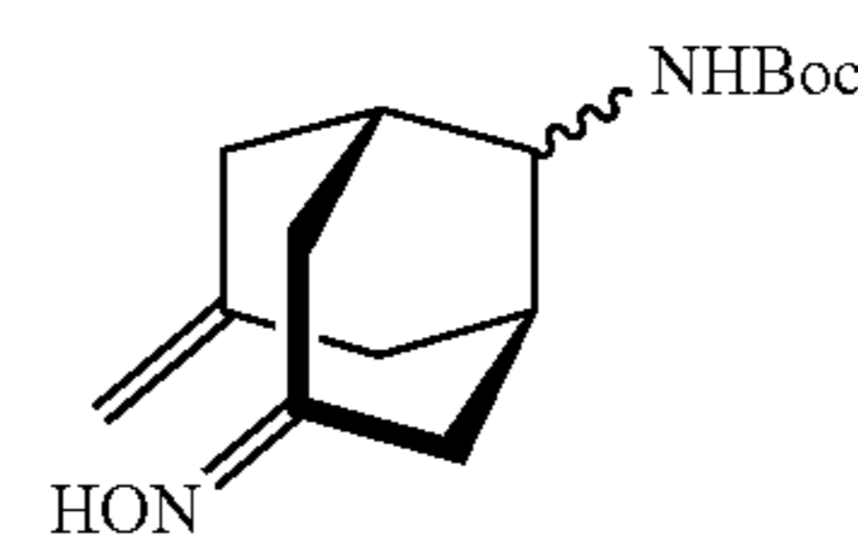
(7-Methylene-bicyclo[3.3.1]nonan-3-one oxime-9-yl)-carbamic Acid Tert-Butyl Ester (27)
