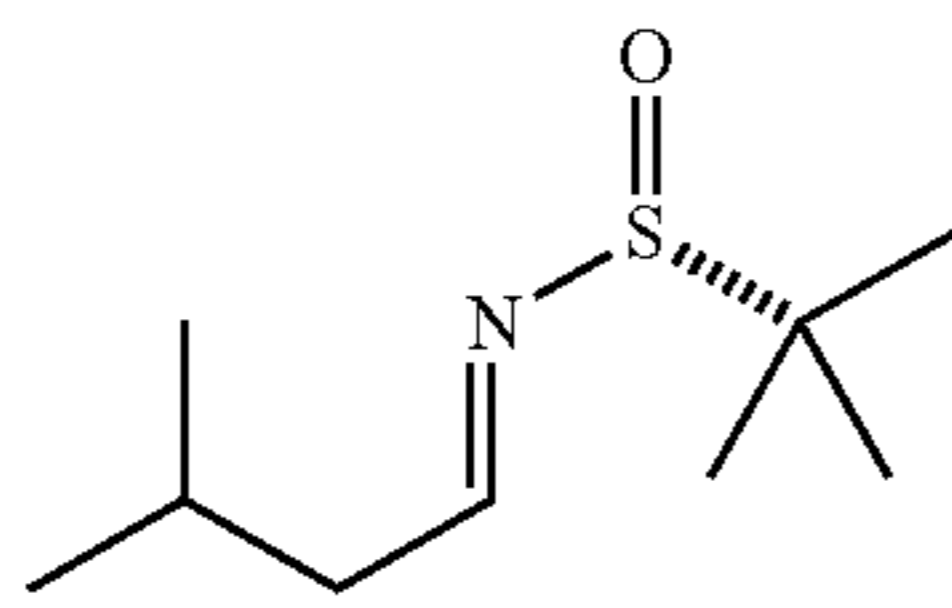
(R,E)-2-Methyl-N-(3-methylbutylidene)propane-2-sulfonamide (1)
