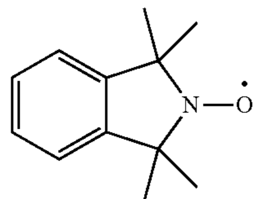
1,1,3,3-Tetramethylisoindolin-2-yloxy (18)
