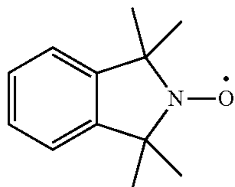
1,1,3,3-Tetramethylisoindolin-2-yloxy (18)
