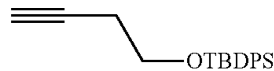
(But-3-ynoxy)(tert-butyl)diphenylsilane (2)
