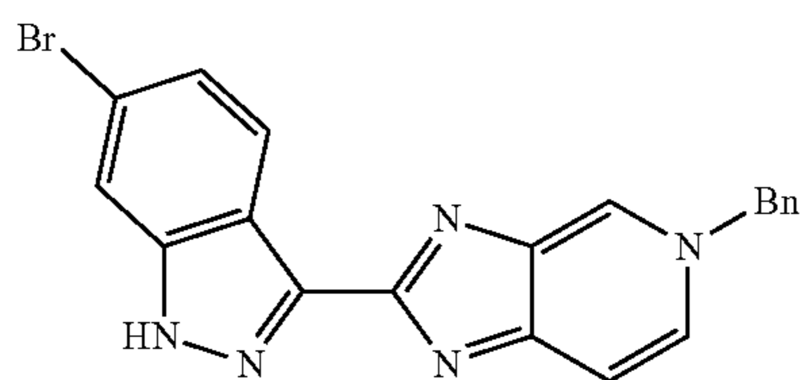
(a) 5-Benzyl-2-(6-bromo-1H-indazol-3-yl)-5H-imidazo[4,5-c]pyridine
