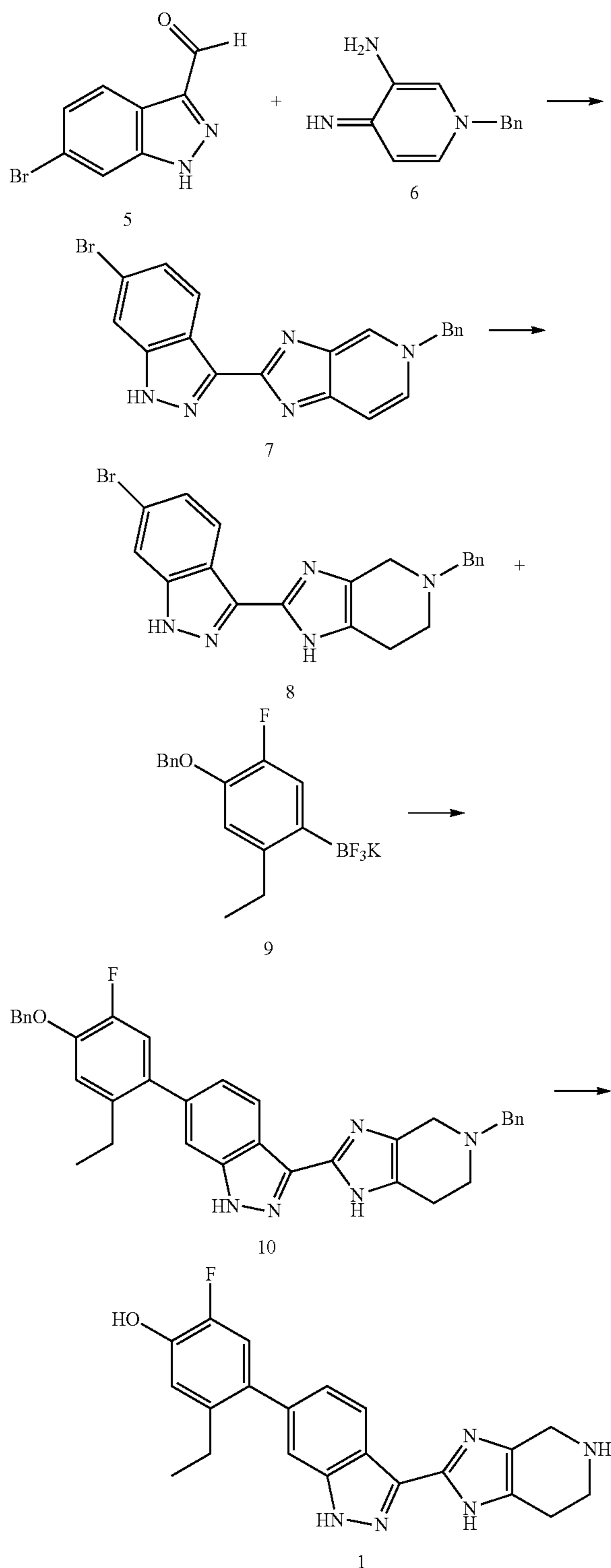
Scheme 2
