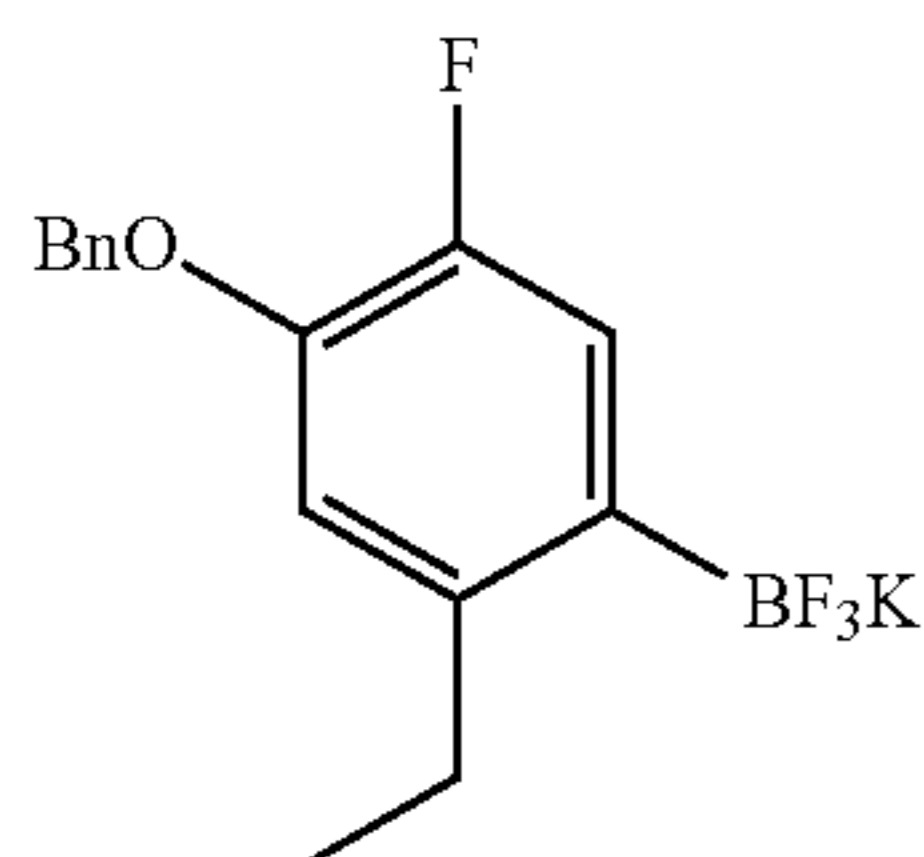
(a) 2-(4-(Benzyloxy)-2-ethyl-5-fluorophenyl)-4,4,5,5-tetramethyl-1,3,2-dioxaborolane
