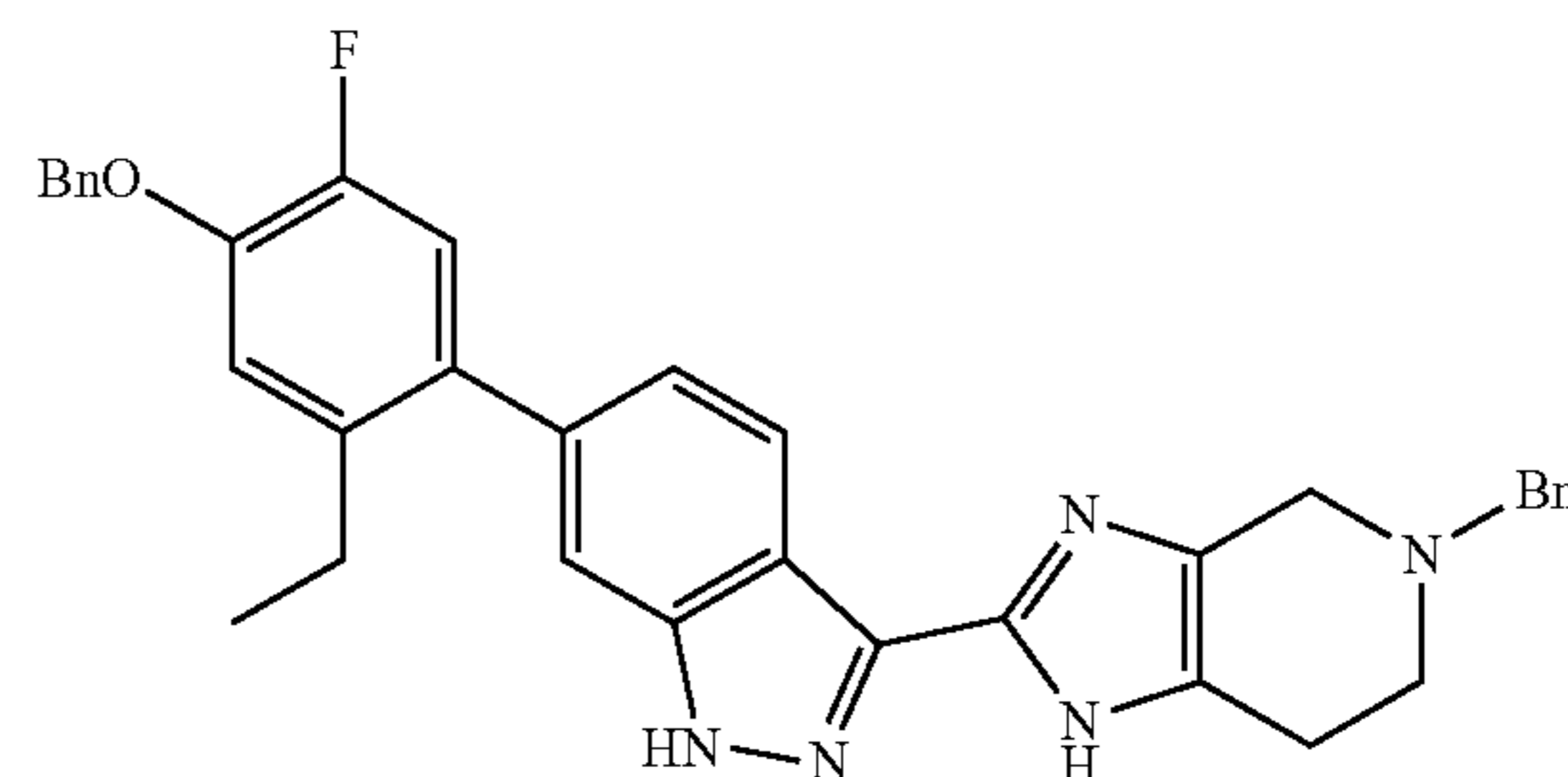
(a) 5-Benzyl-2-(6-(4-(benzyloxy)-2-ethyl-5-fluorophenyl)-1H-indazol-3-yl)-4,5,6,7-tetrahydro-1H-imidazo[4,5-c]pyridine
