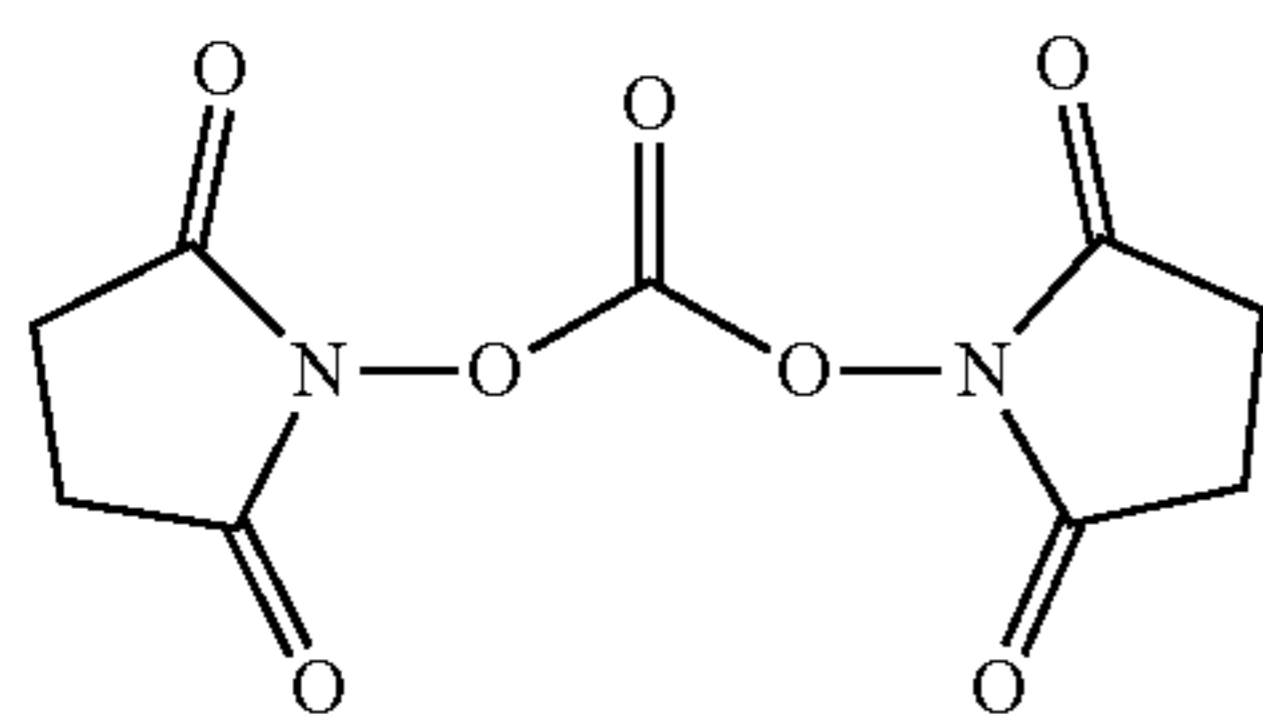
N,N'-Disuccinimidyl Carbonate (DSC)
