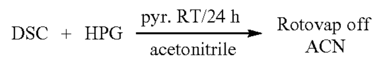
N,N'-Disuccinimidyl Carbonate (DSC)
