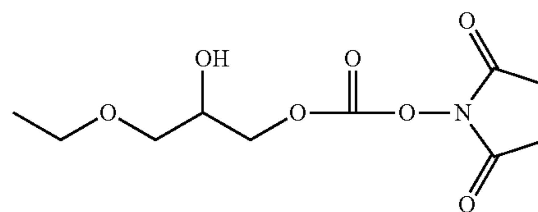
HPG-Succinimidyl Carbonate White solid, soluble in EtOH/PBS
