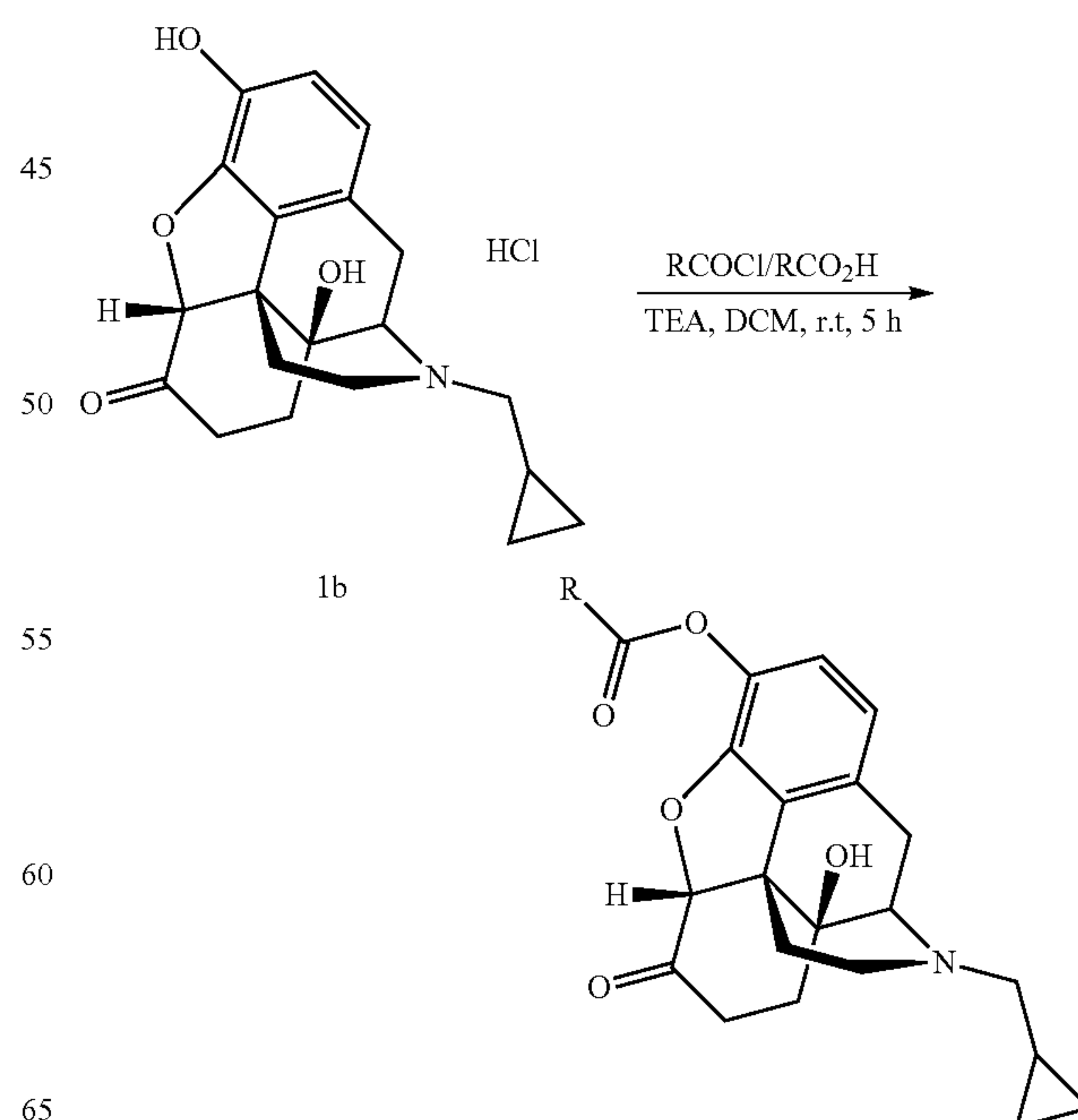
Scheme 2
