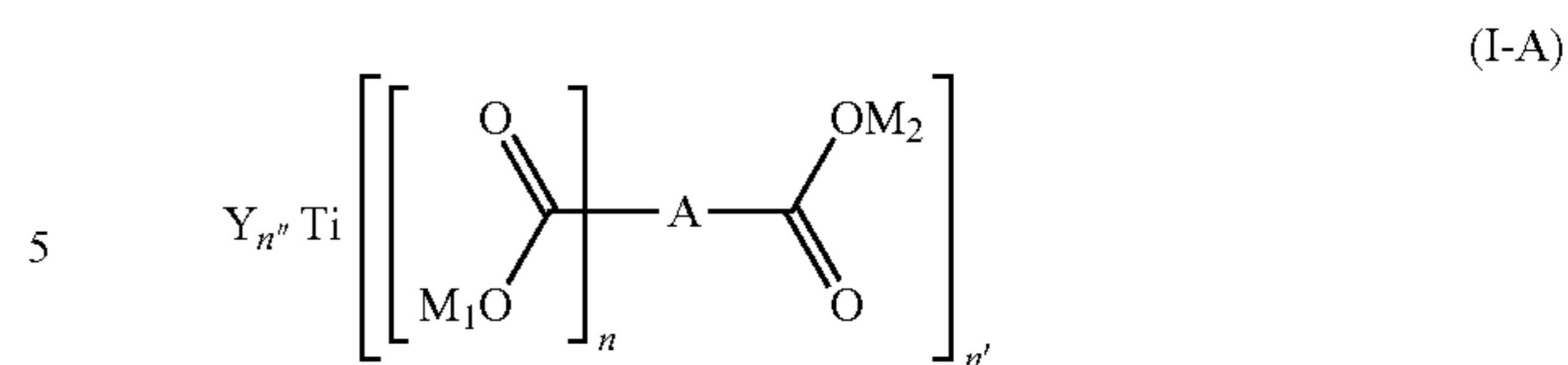
Basic Yellow 87
