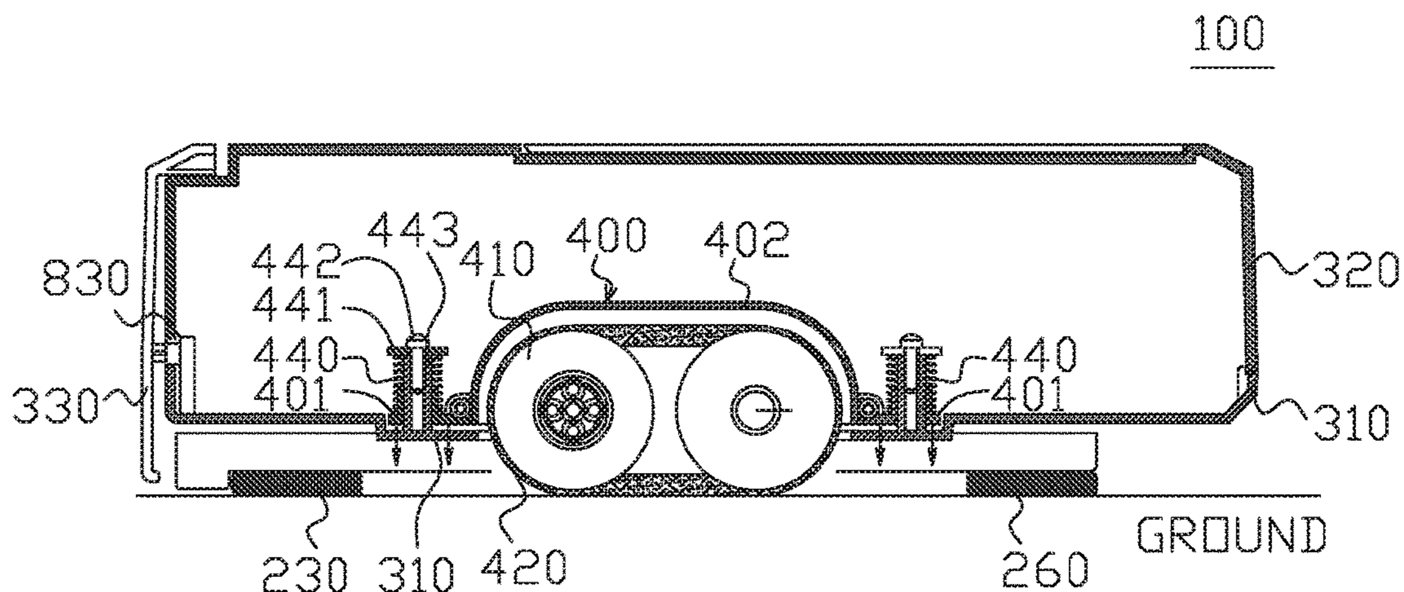
SECTION "C"-"C" FIG. 5
