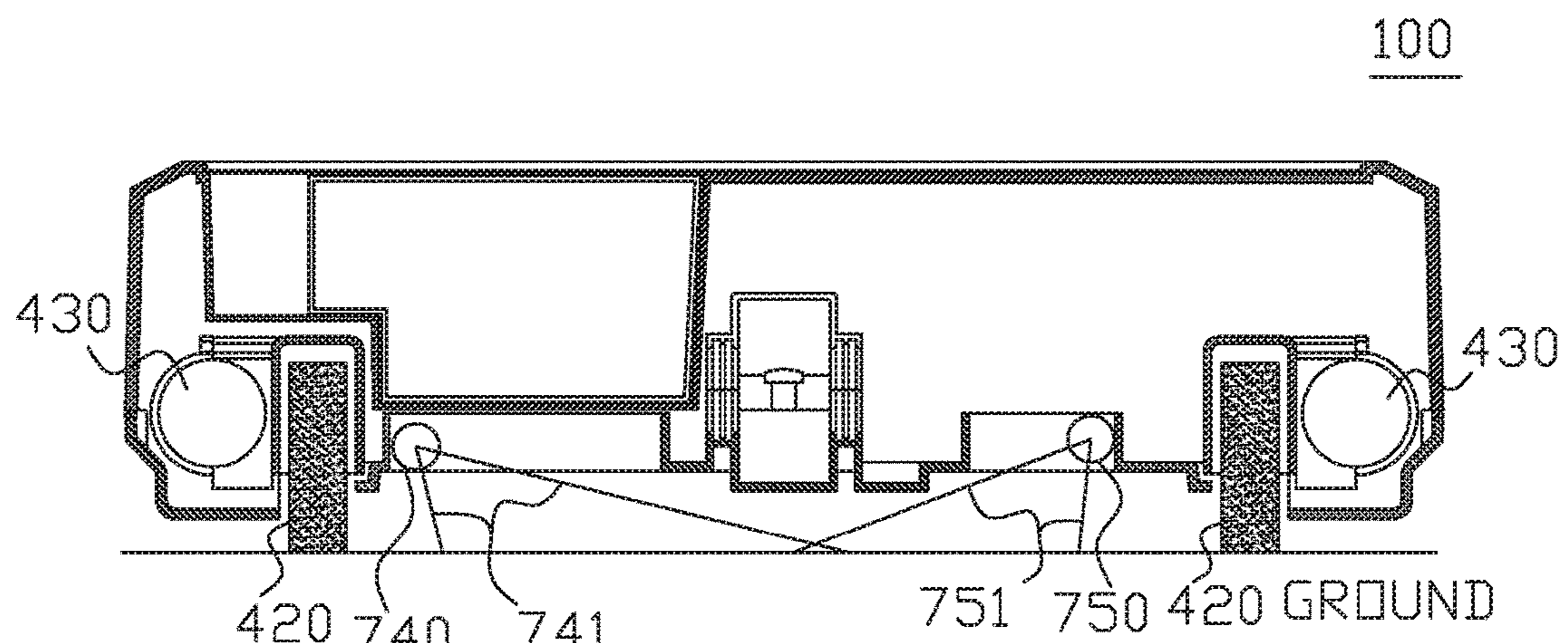
SECTION "K"-"K" FIG. 6
