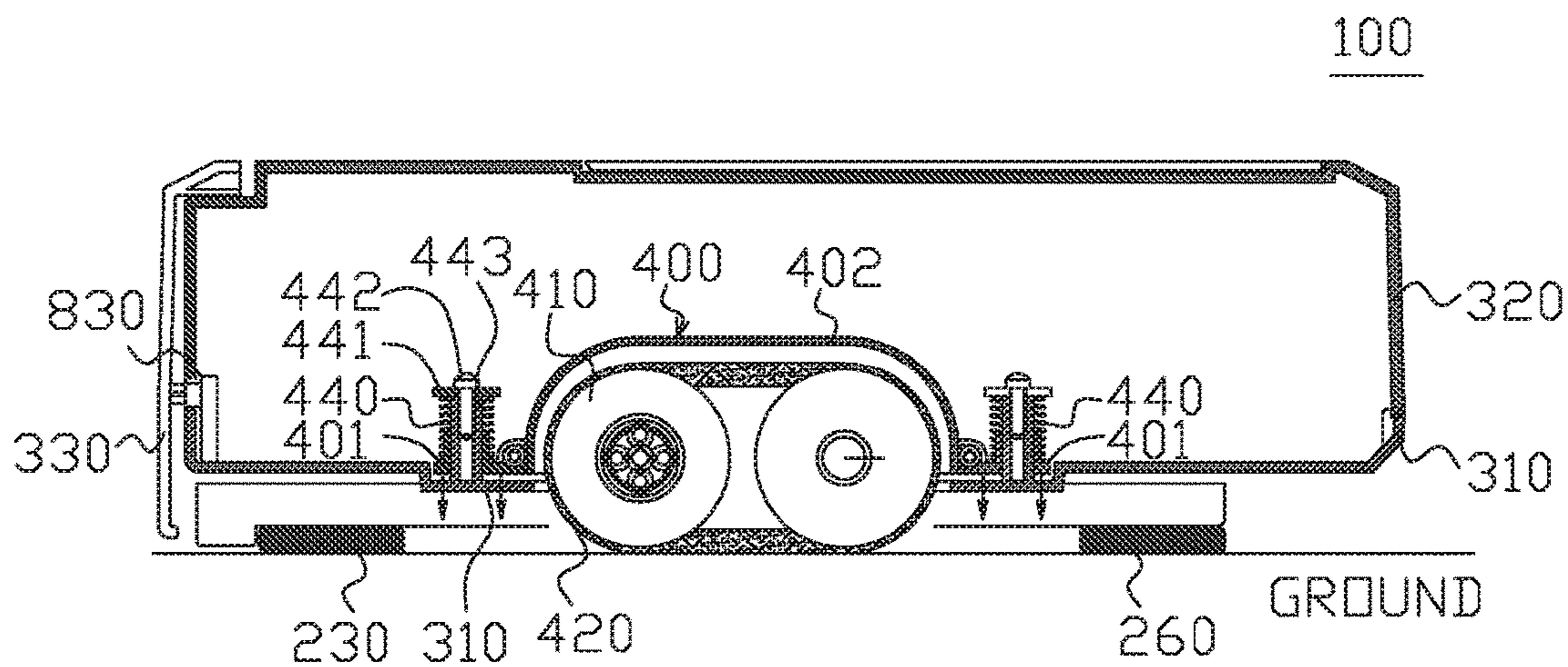
SECTION "C"-"C" FIG. 5
