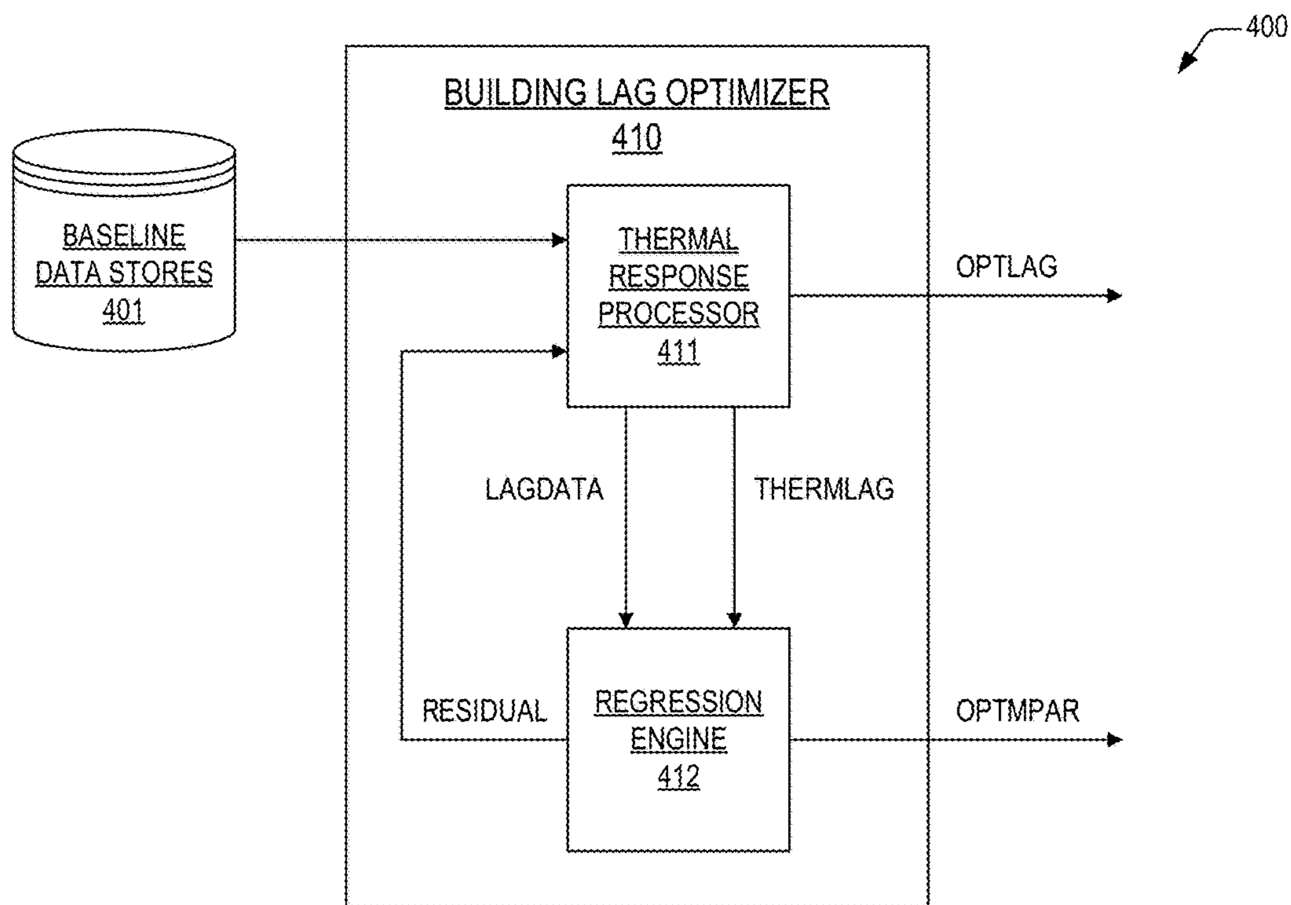
FINE-GRAINED BASELINE ENERGY DATA WEATHER NORMALIZATION APPARATUS
