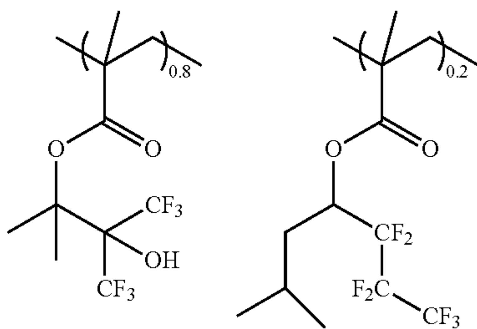
Water-repellent polymer 2 M w = 9,300 M w /M n = 1.87
