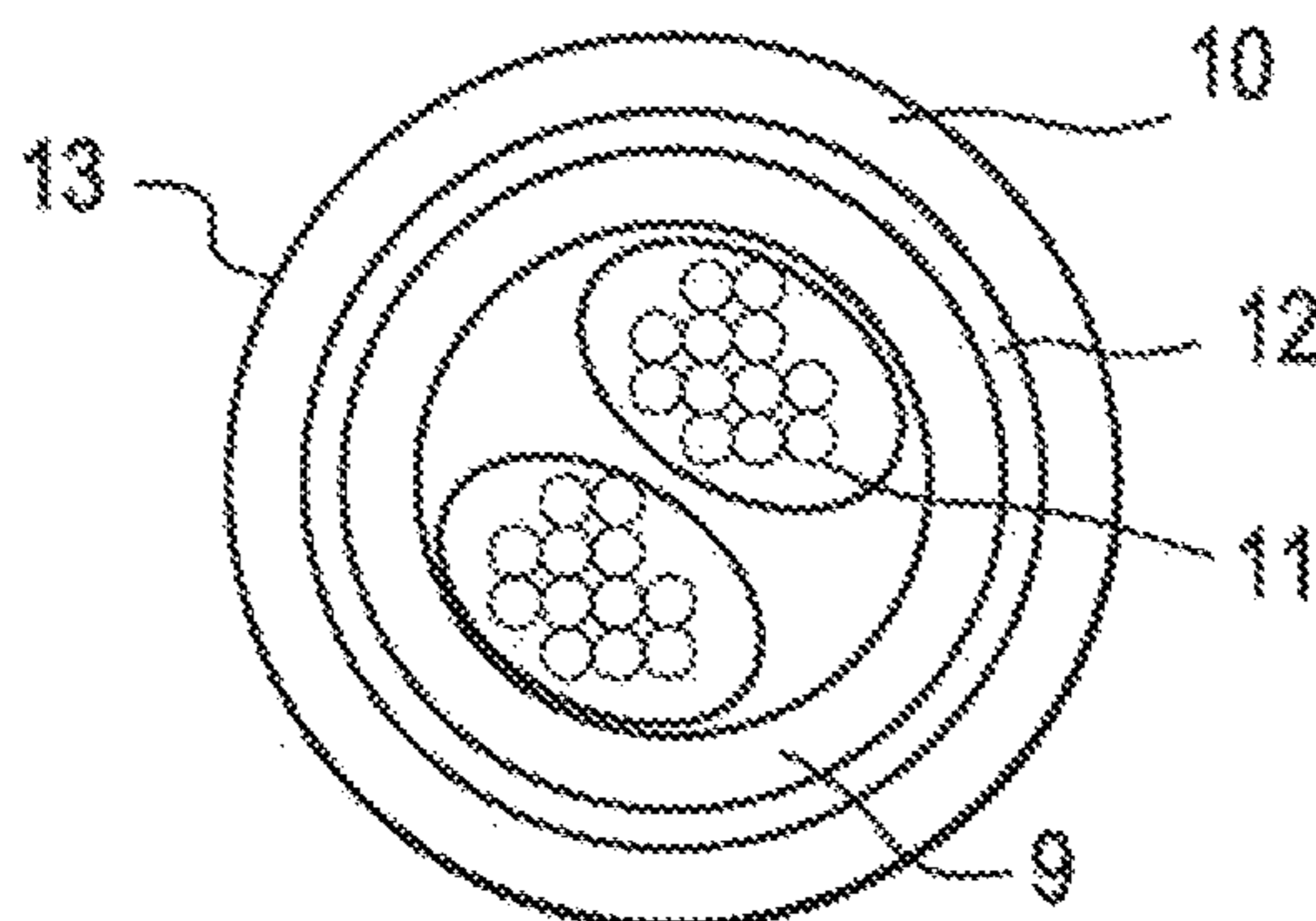
FIG. 3 RELATED ART
