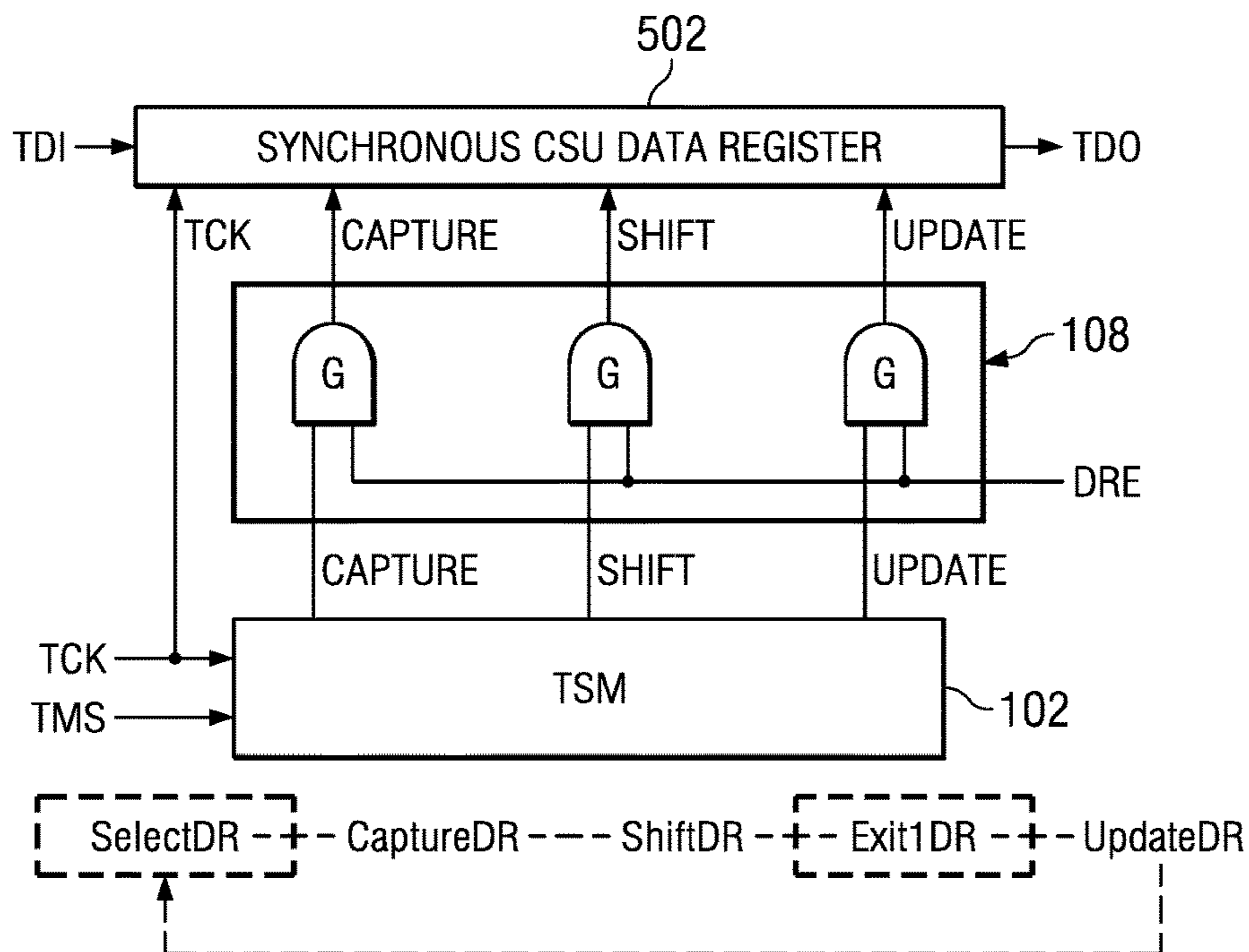
FIG. 5 (PRIOR ART)
