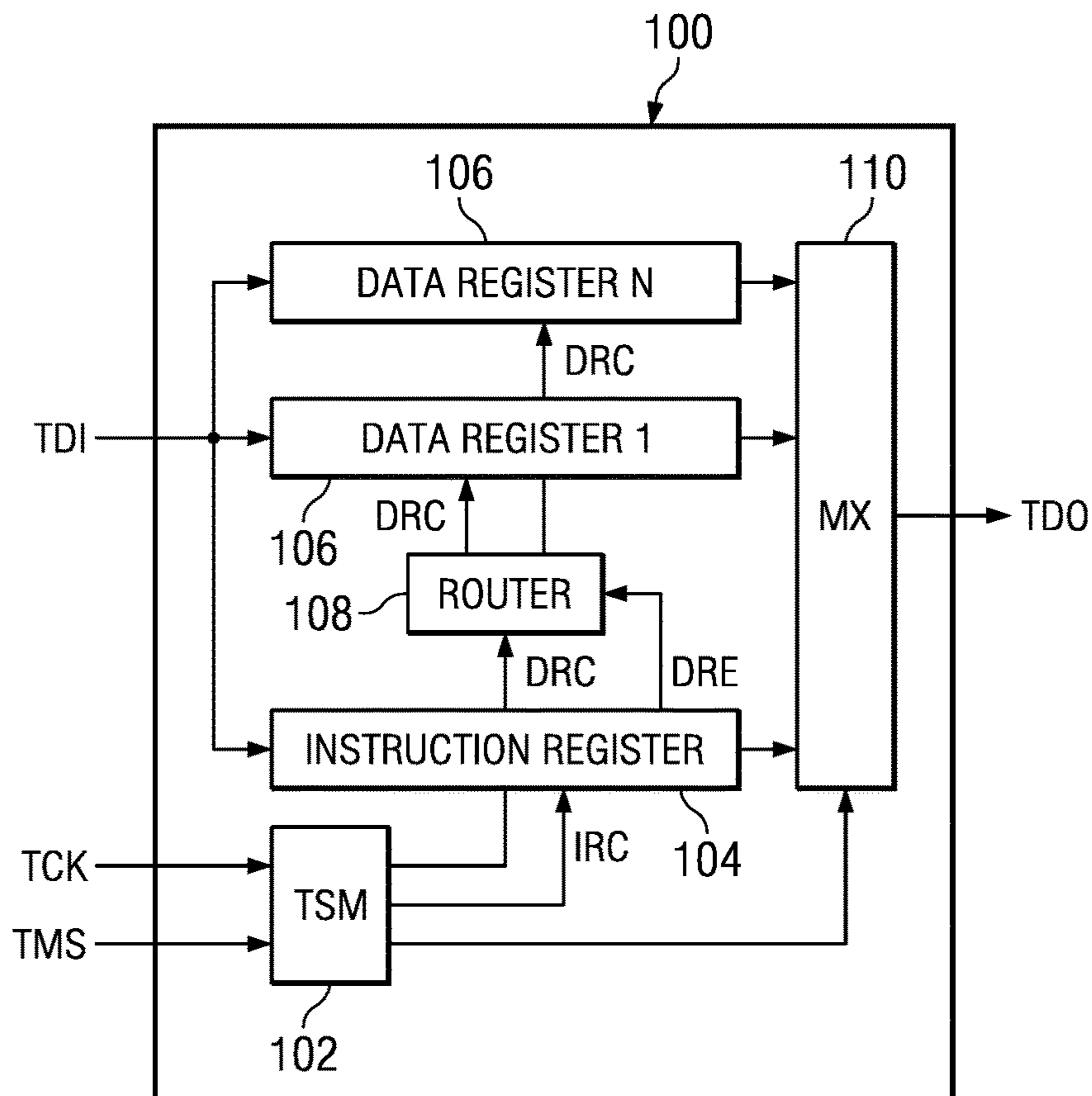
FIG. 1 (PRIOR ART)
