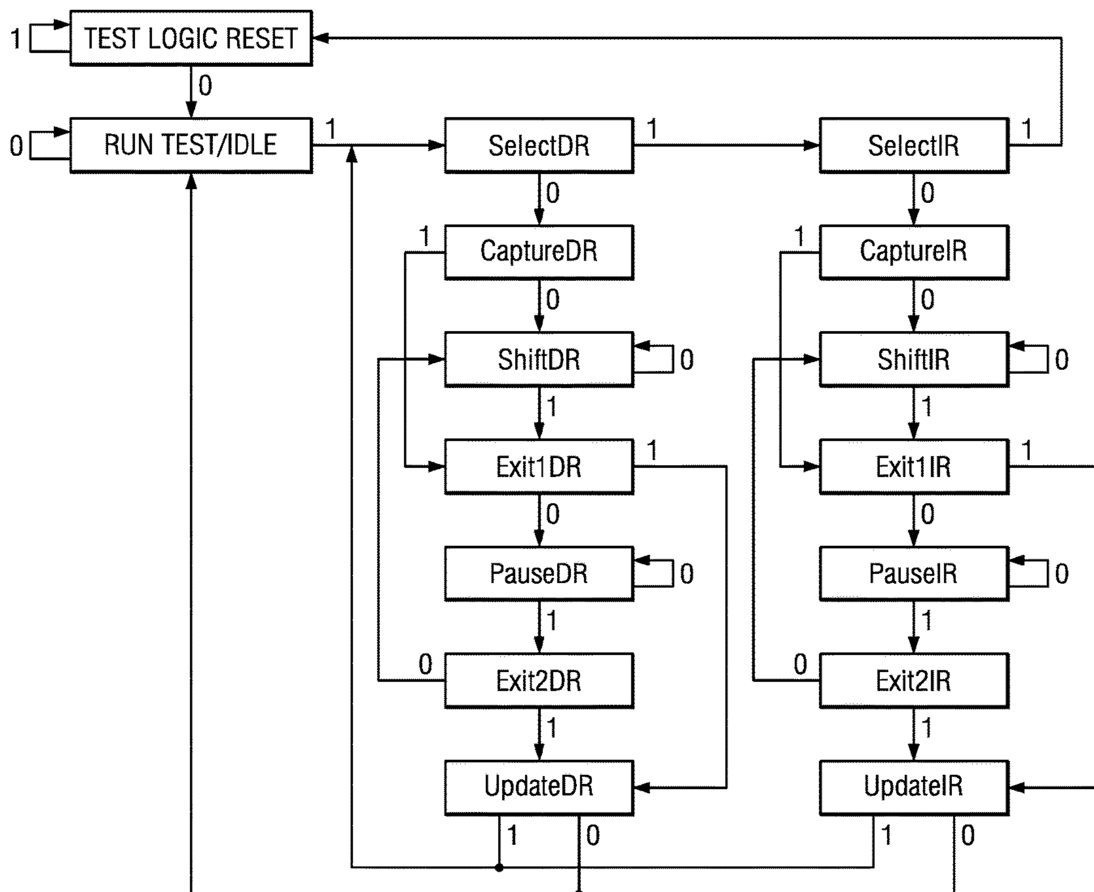
FIG. 3 (PRIOR ART)
