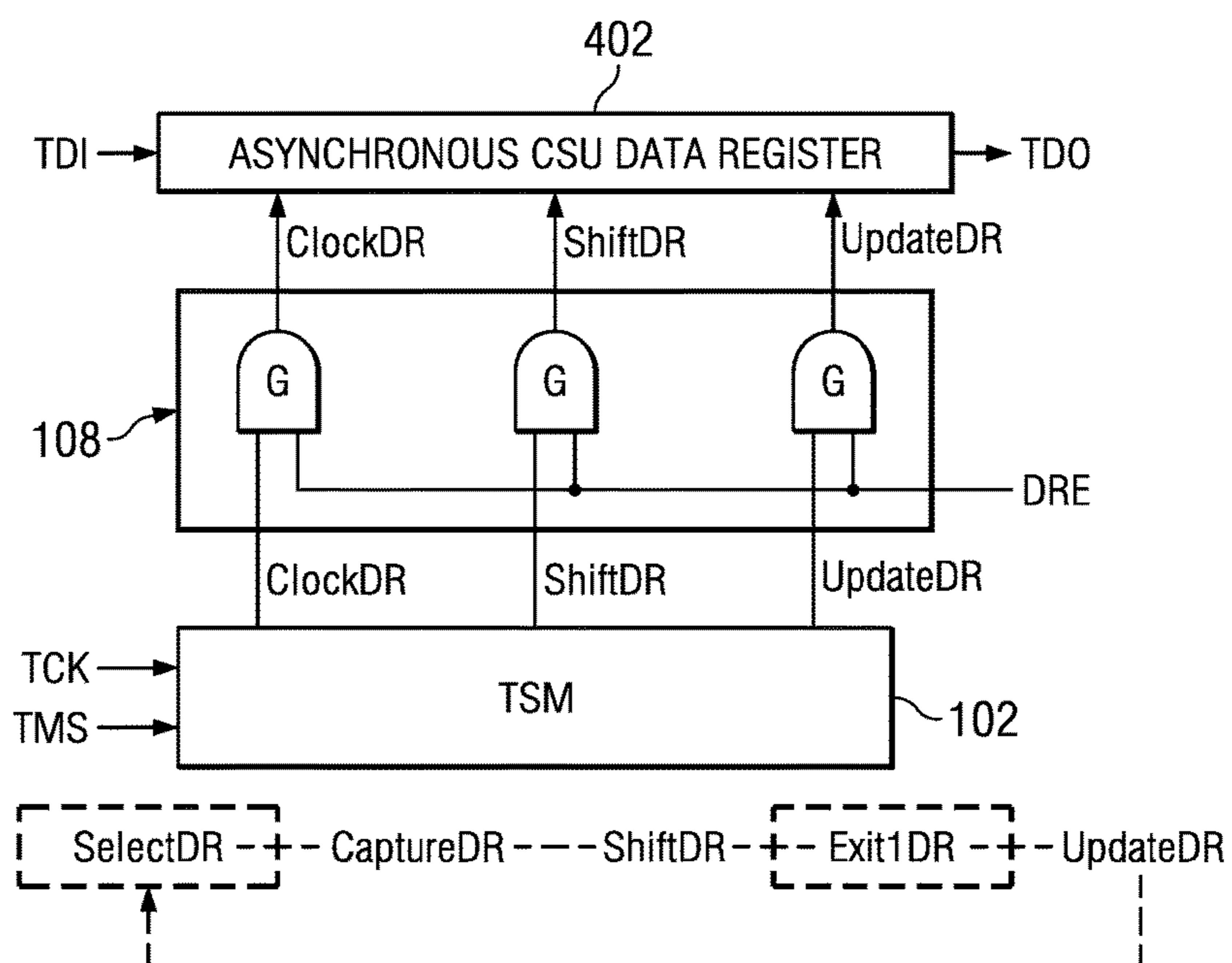
FIG. 4 (PRIOR ART)
