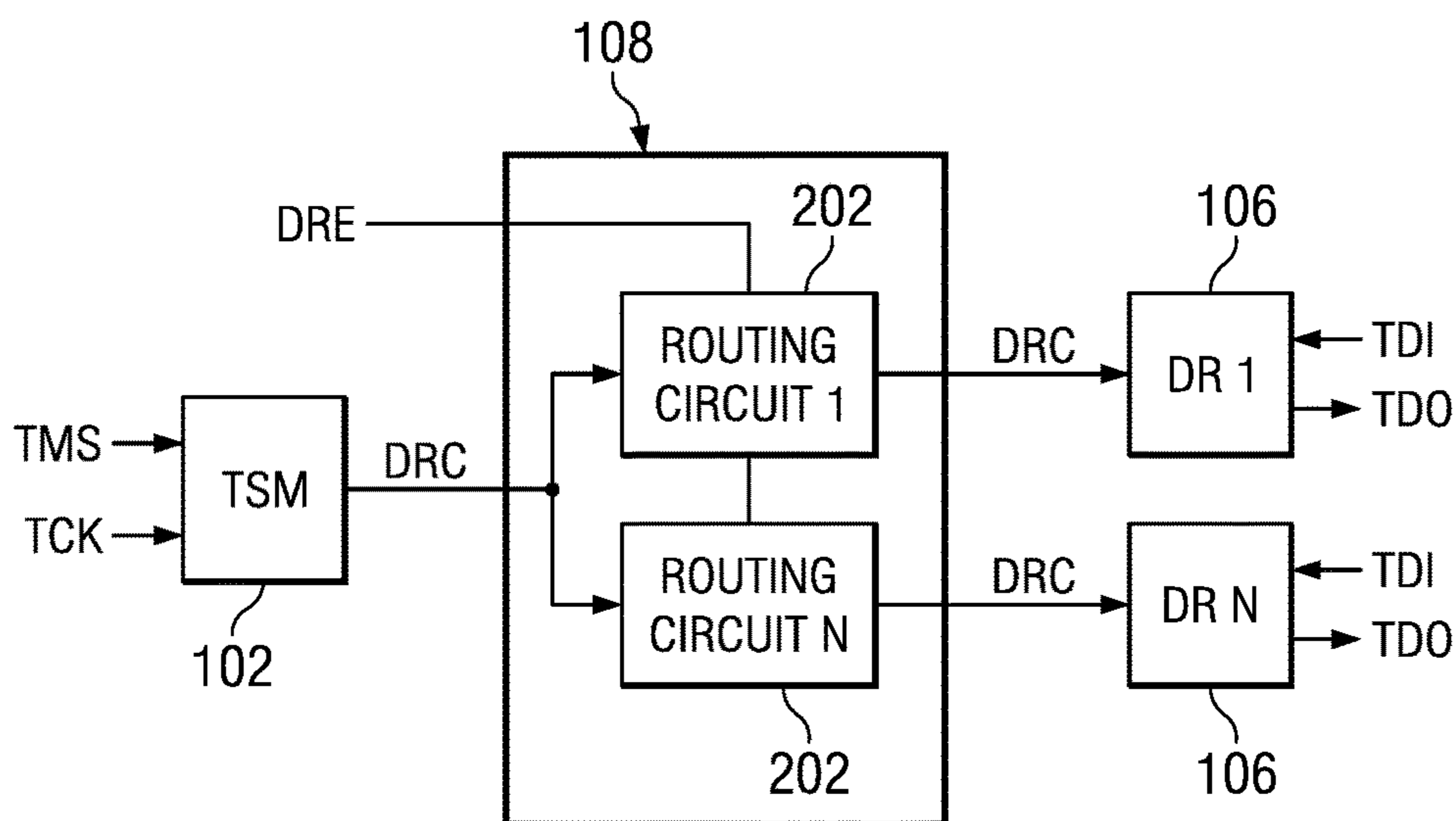
FIG. 2 (PRIOR ART)
