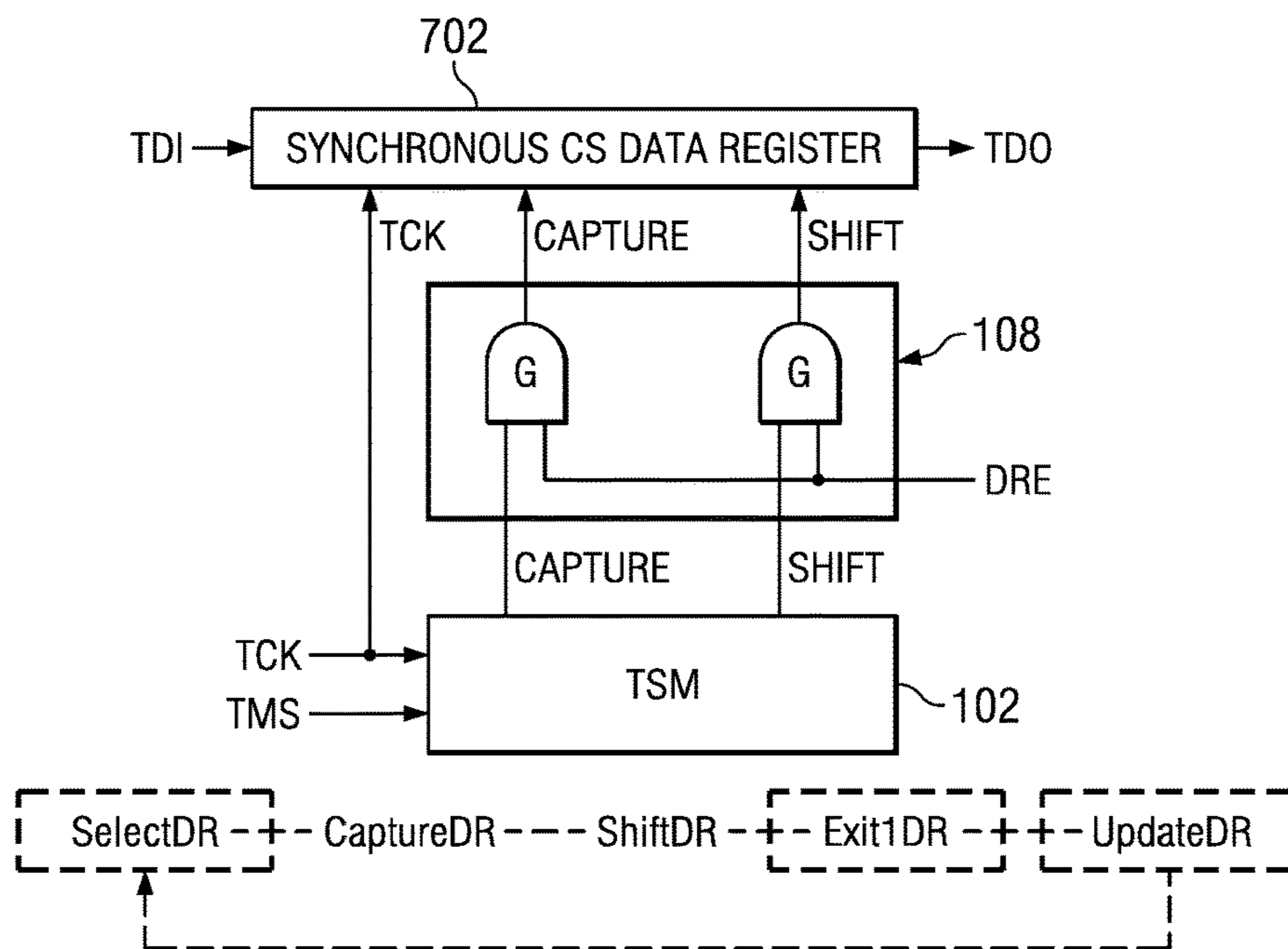
FIG. 7 (PRIOR ART)
