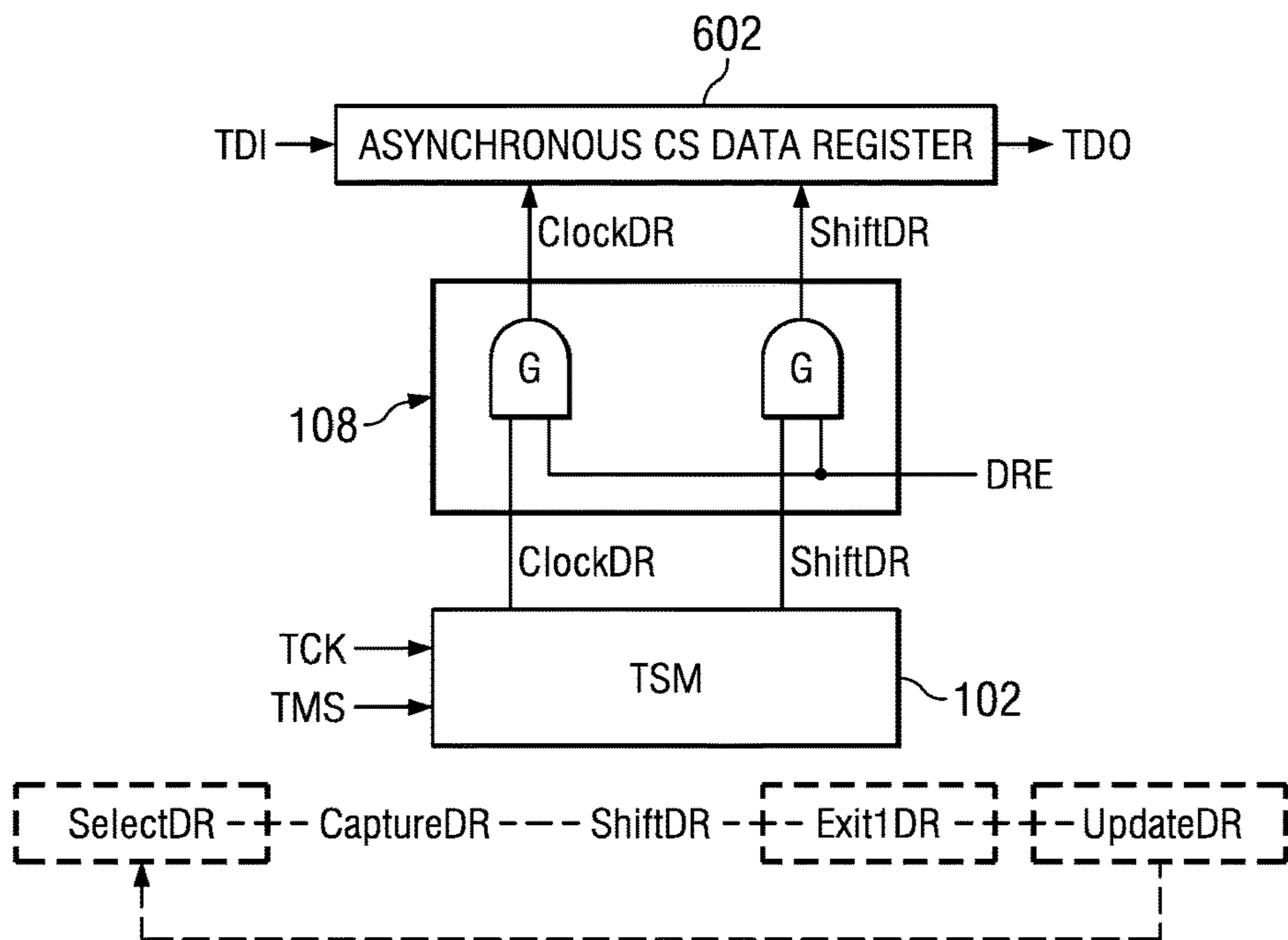
FIG. 6 (PRIOR ART)
