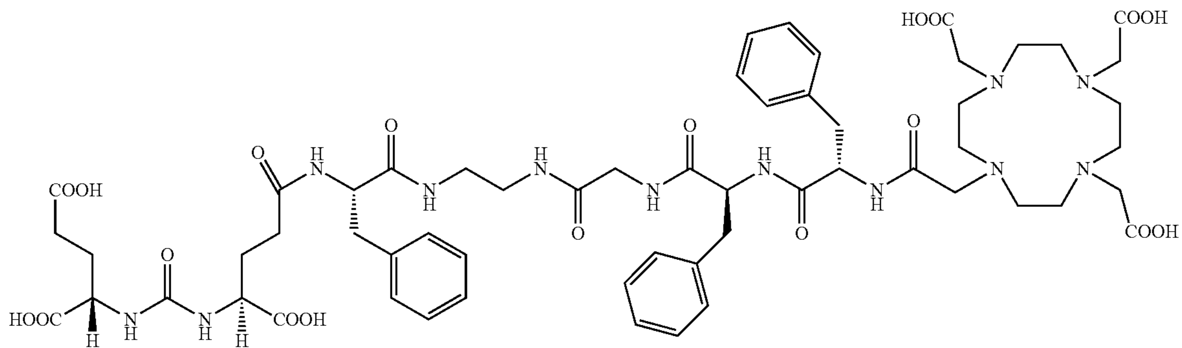
DOTA conjugate capable of chelating for example 64 Cu, 65 Cu, and the like
