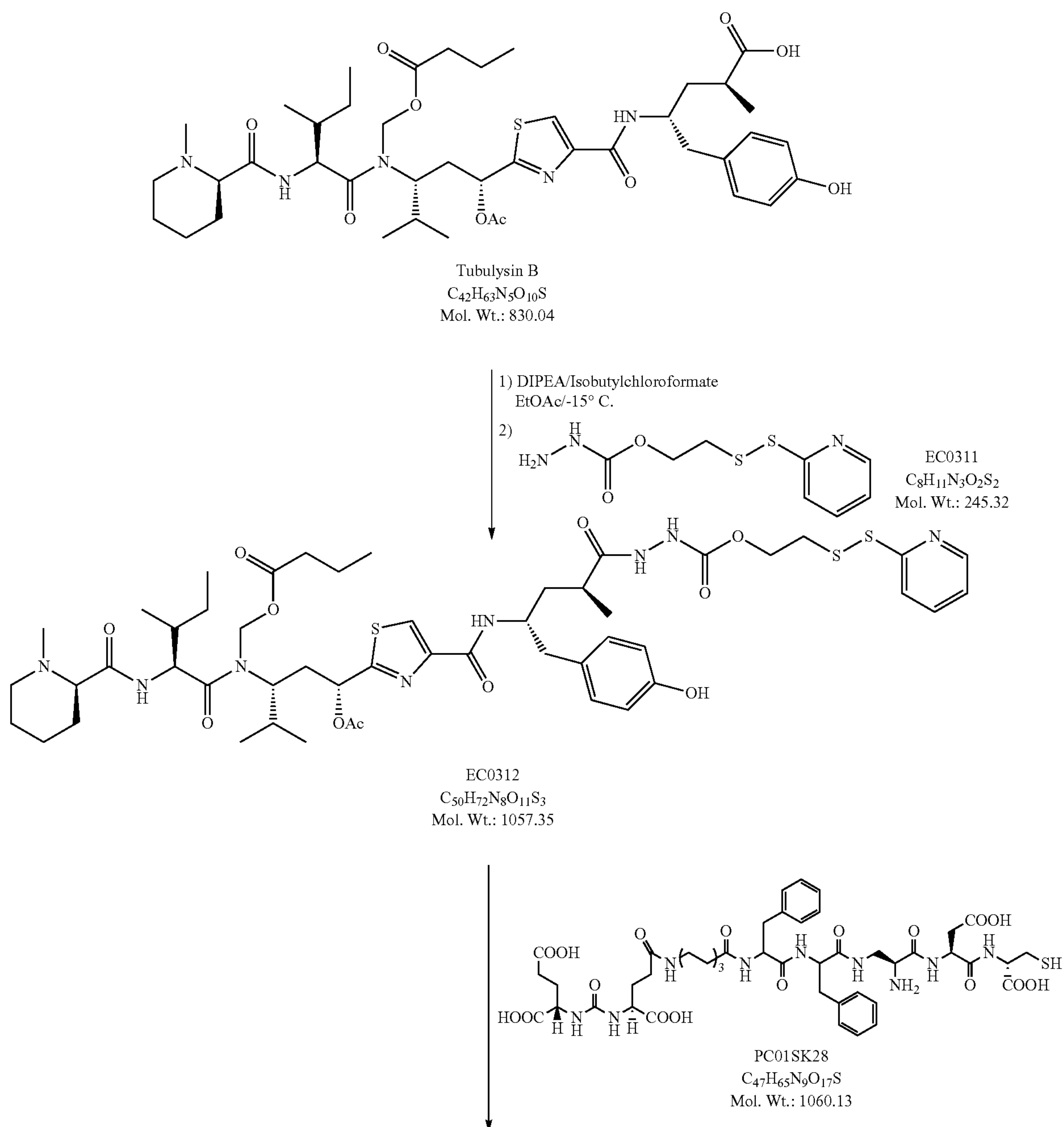
Scheme 6.4
