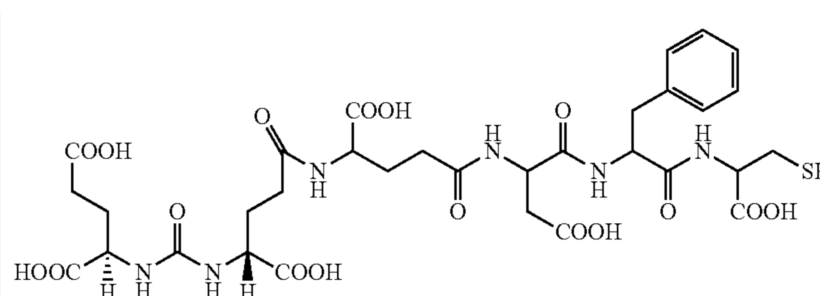
PC01SK68 C_{32}H_{42}N_6O_{17}S Mol. Wt.: 814.77
