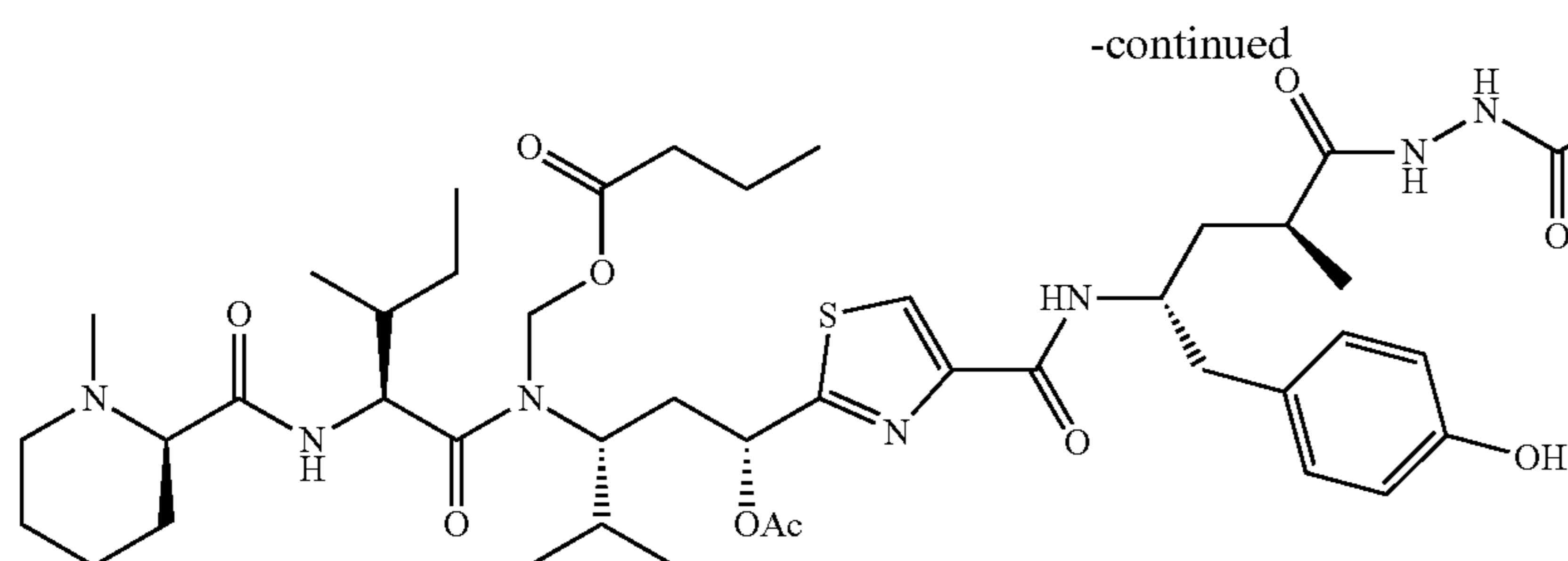
EC0312 C_{50}H_{72}N_8O_{11}S_3 Mol. Wt.: 1057.35
