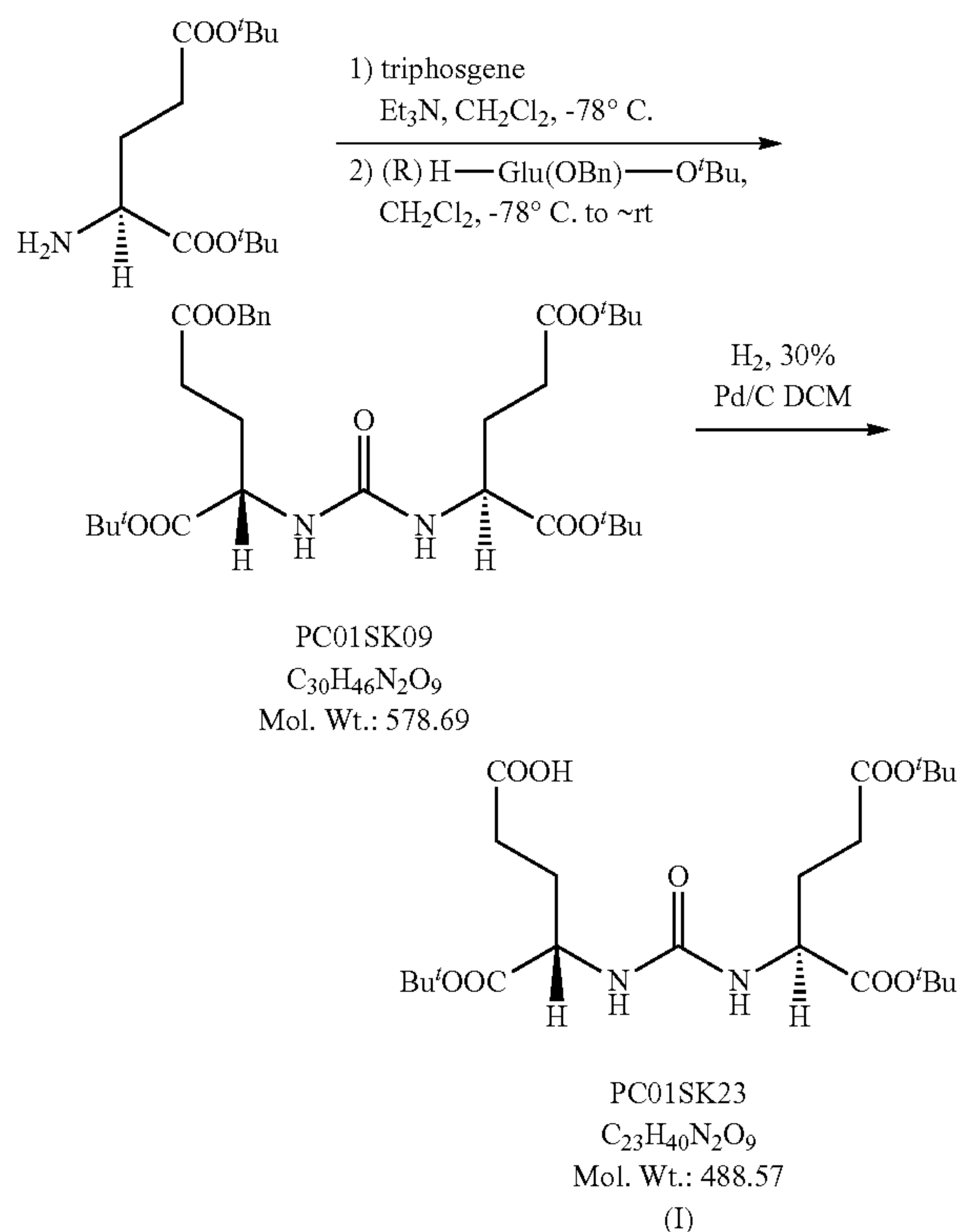
Scheme 2.1
