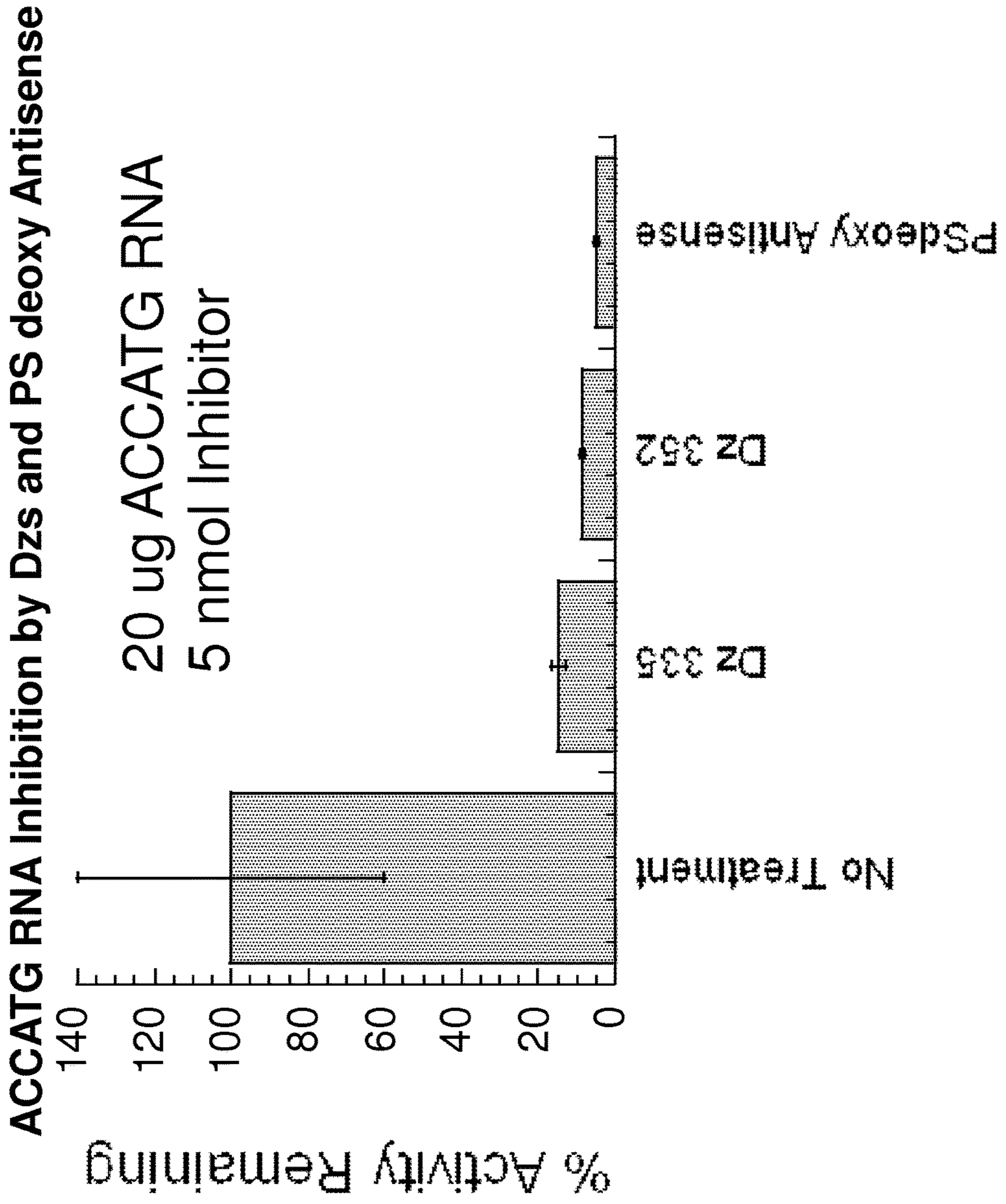
Figure 5B The DNazymes Dz 335 and Dz 352 as well as the antisense molecule Psdeoxy inhibit translation of ACCATG RNA (same as ACC RNA) by binding to the HCV IRES
