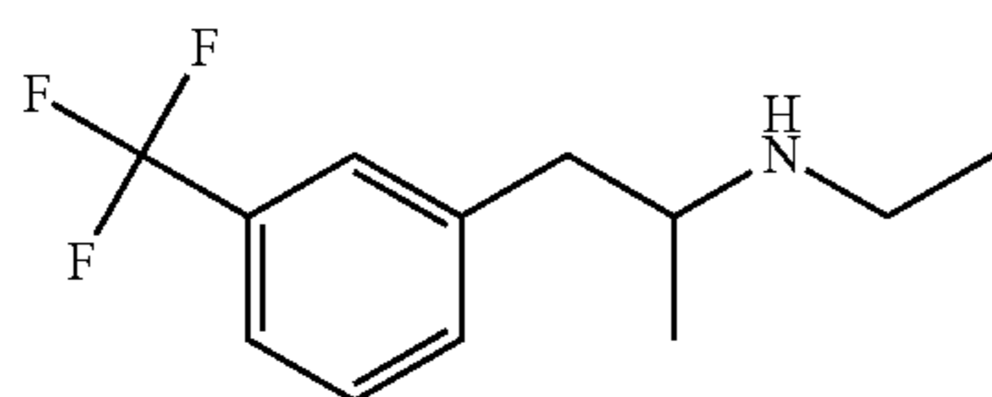
(R,S)—N-ethyl-1-[3-(trifluoromethyl)phenyl]propan-2-amine
