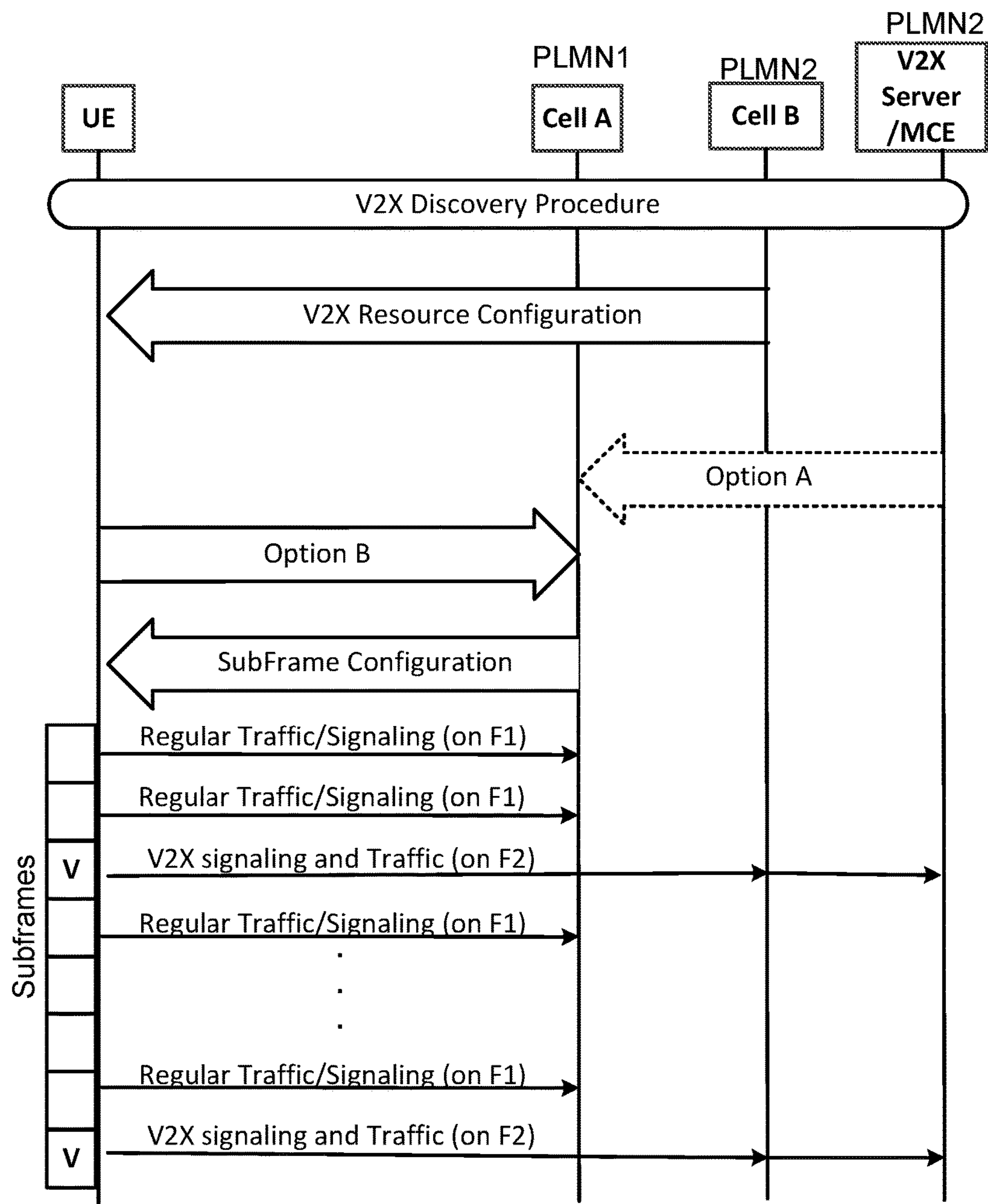
Time/Subframe Multiplexing Between F1 and F2 Option B: V2X interest indication Option A: Inter-PLMN management signaling, V2X resource configuration and timing
