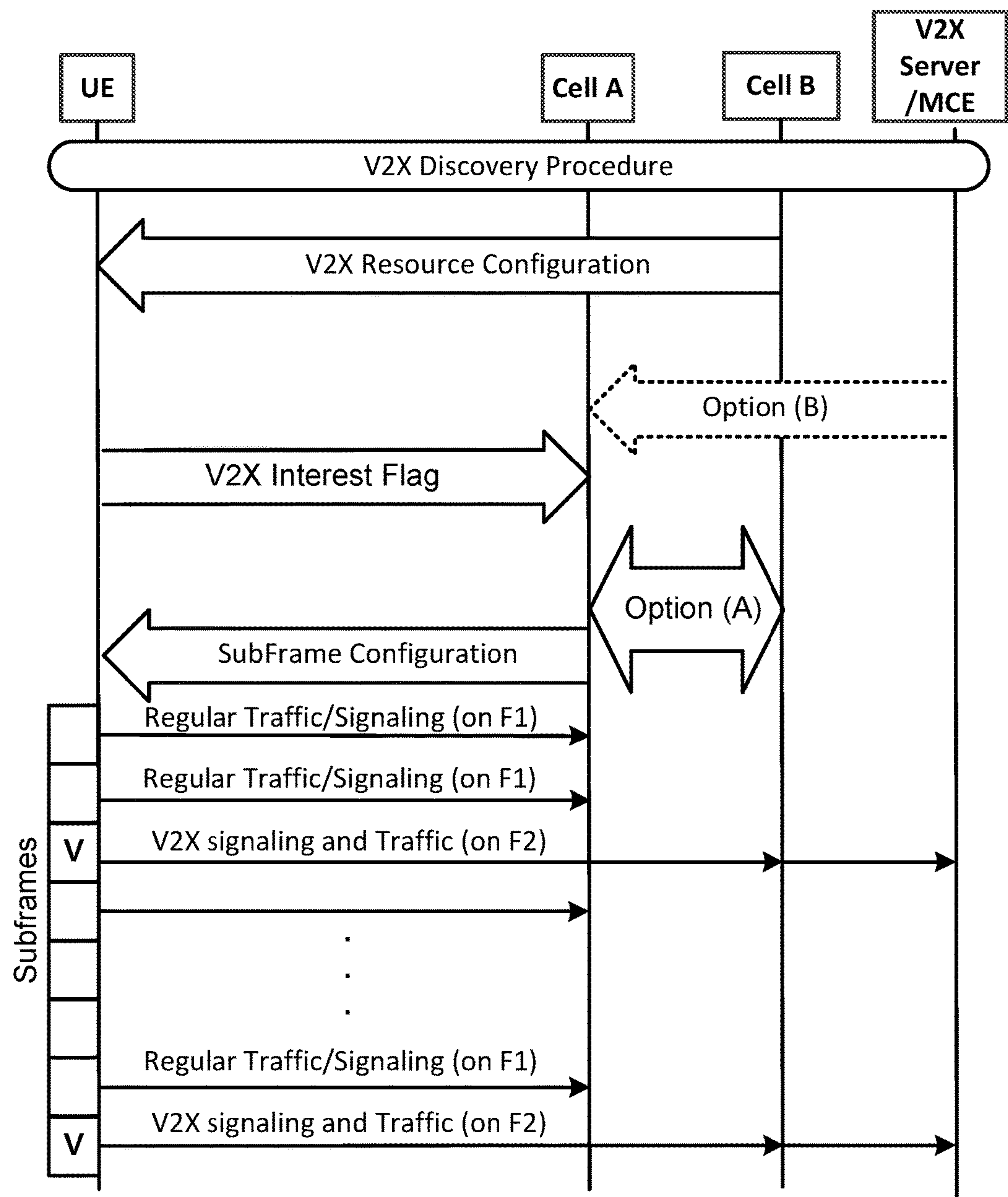
Time/Subframe Multiplexing Between F1 and F2 Option B: Core network Signaling V2X Resource Configuration and Timing Option A: Inter-Cell V2X Configuration Exchange
