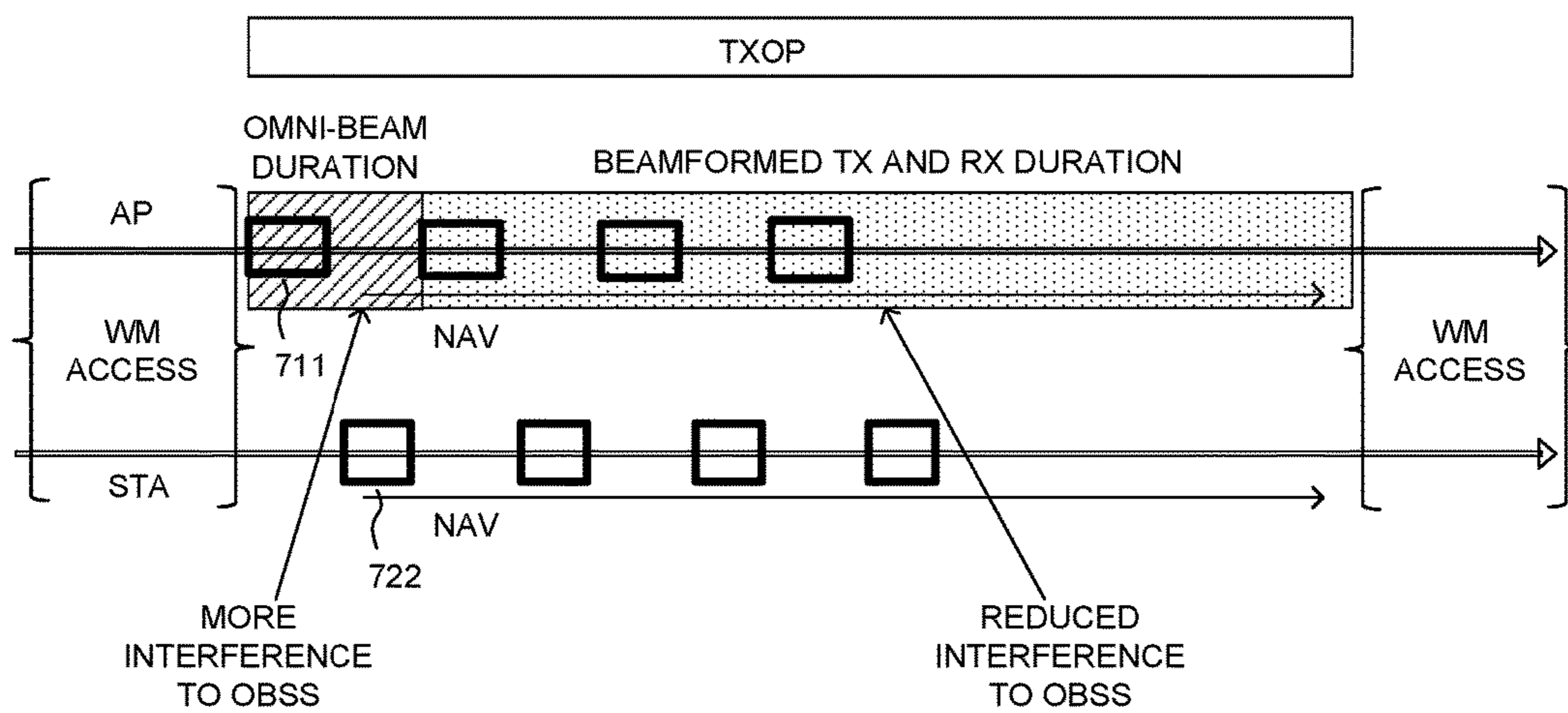
TXOP-BASED BEAMFORMED FRAME EXCHANGE
