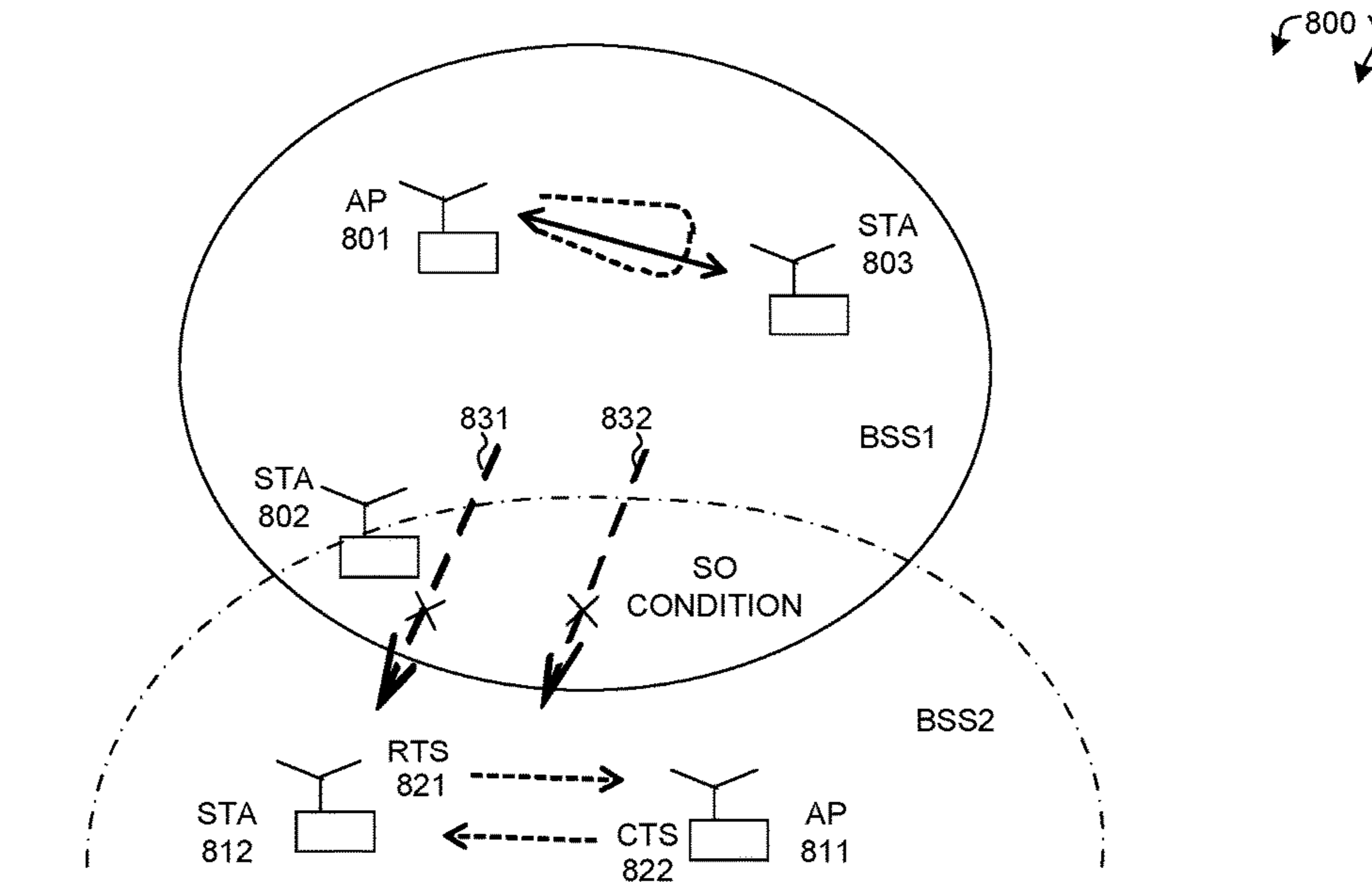
TXOP-BASED BEAMFORMED AND SO FRAME EXCHANGE
