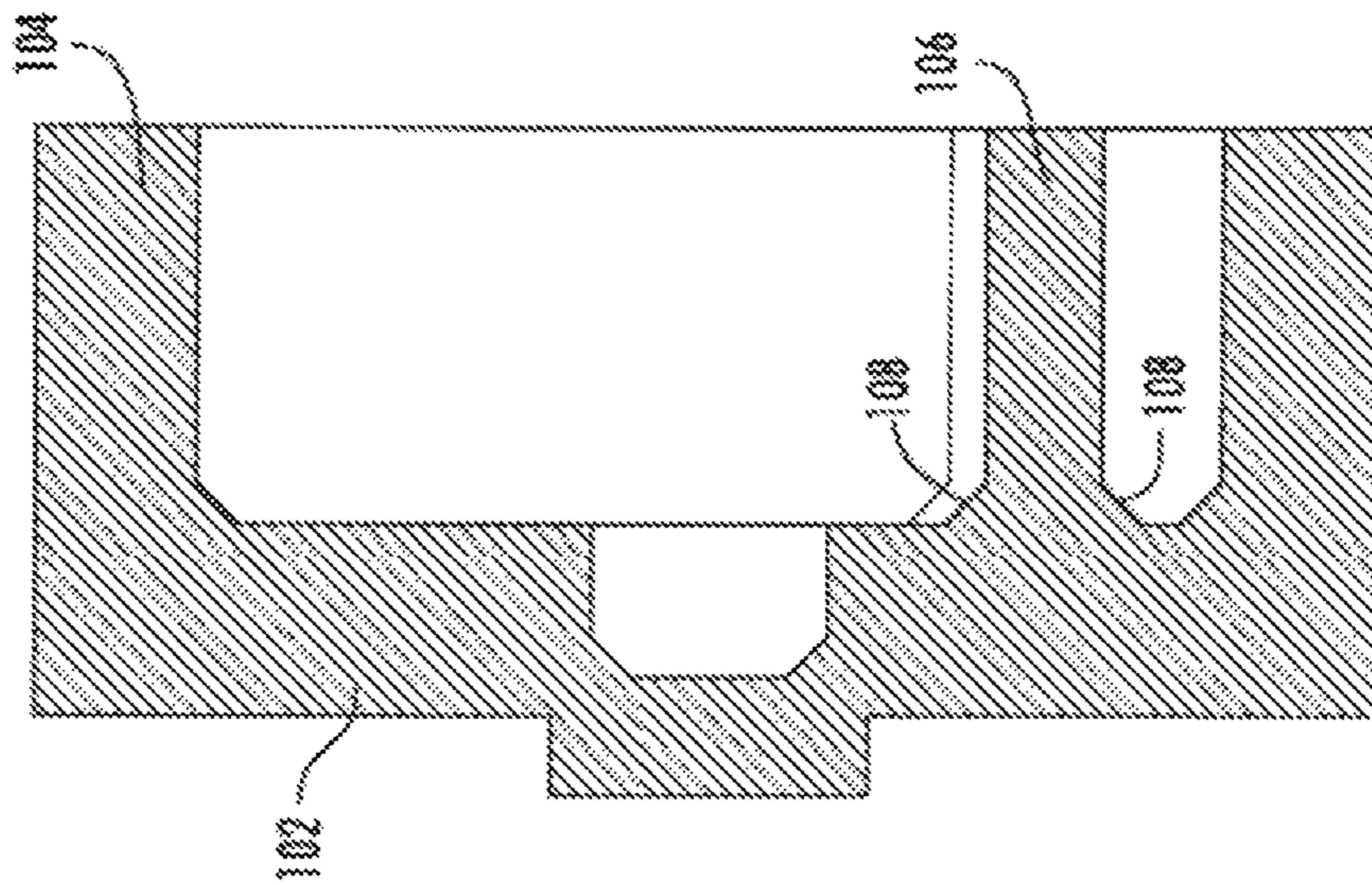
FIG. 4 (PRIOR ART)
