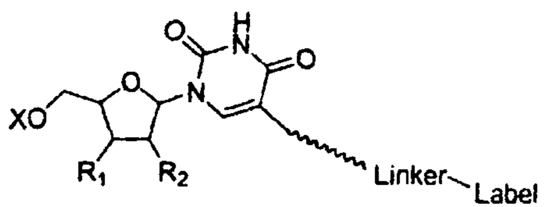
Uridine C5-linker
