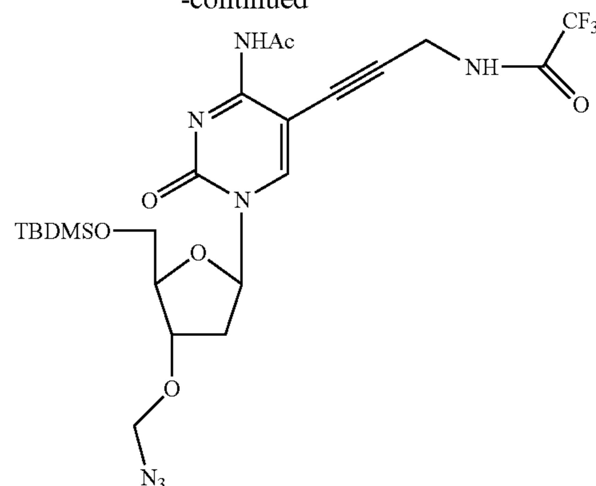
4-N-Acetyl-3'-O-(azidomethyl)-5'-O-(tert-butyldimethylsilyl)-5-[3-(2,2,2-trifluoroacetamide)-prop-1-ynyl]-2'-deoxycytidine (10)
