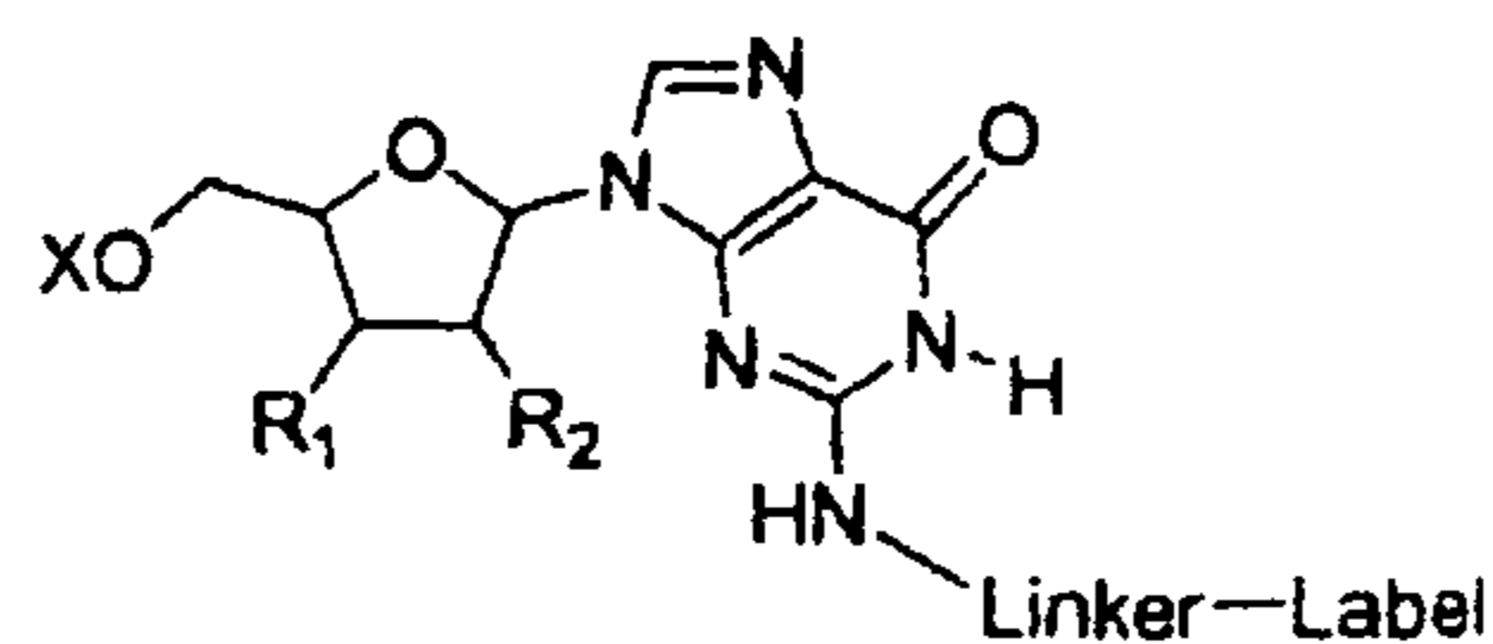
Guanosine N2-linker
