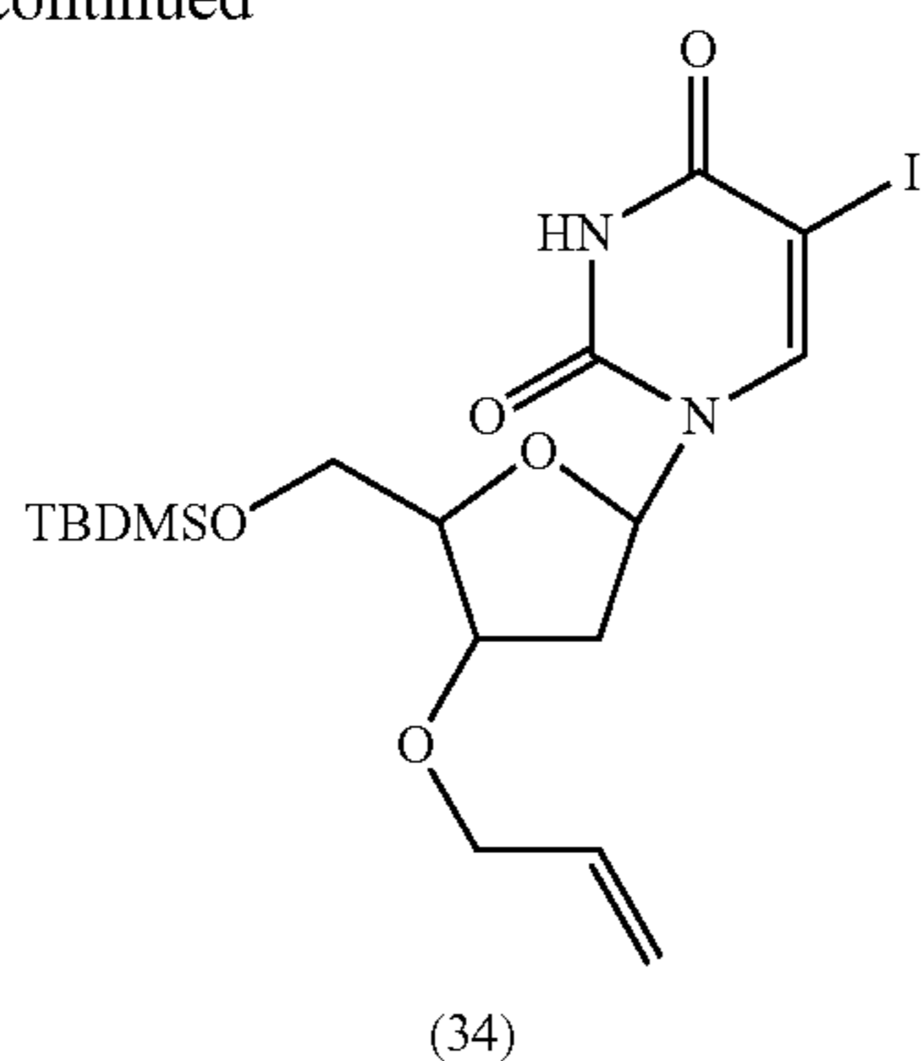
3'-O-Allyl-5'-O-t-butyldimethylsilyl-5-iodo-2'-deoxyuridine (34)
