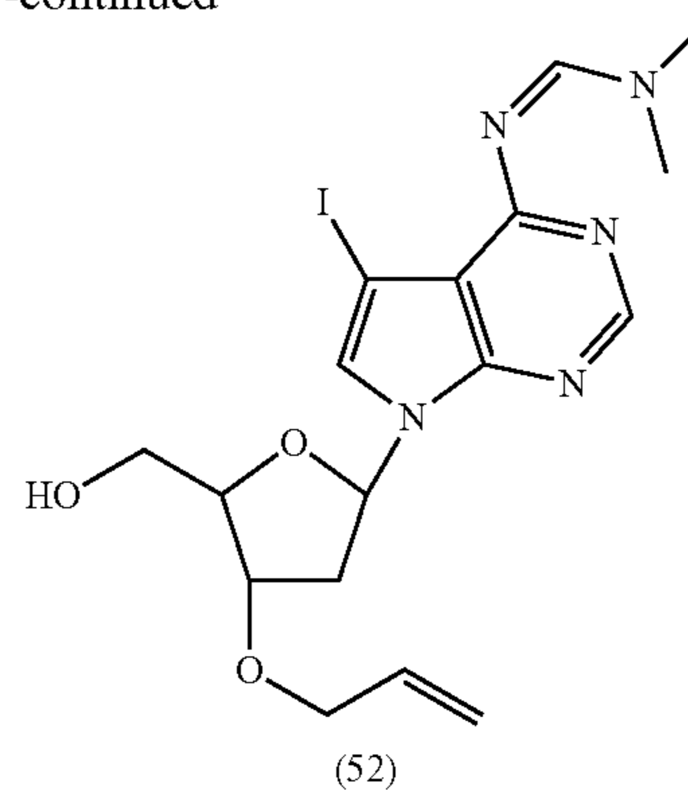
3'-O-Allyl-7-deaza-6-N,N-dimethylformadine-7-iodo-2'-deoxyadenosine (52)
