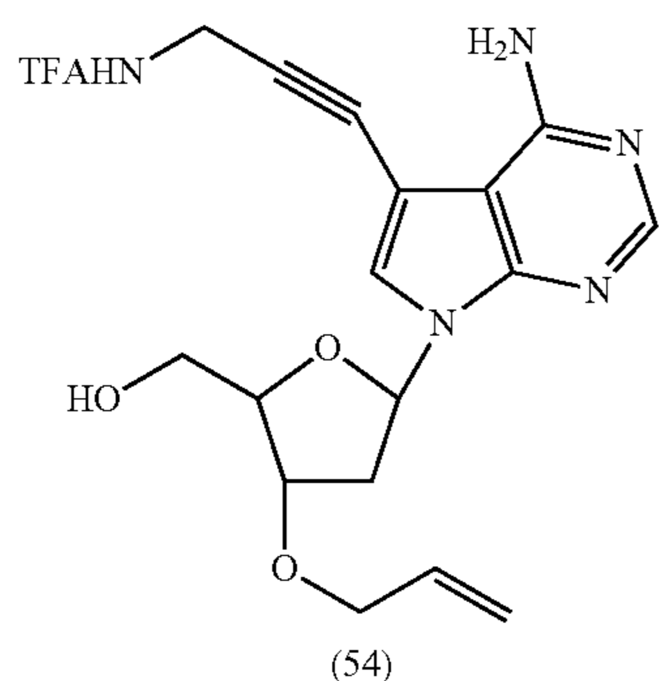
3'-O-Allyl-7-deaza-7-[3-(2,2,2-trifluoroacetamide)]-2'-deoxyadenosine (54)
