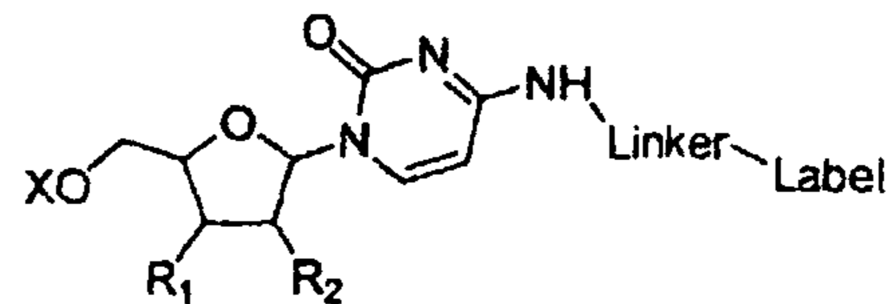
Cytidine N4-linker
