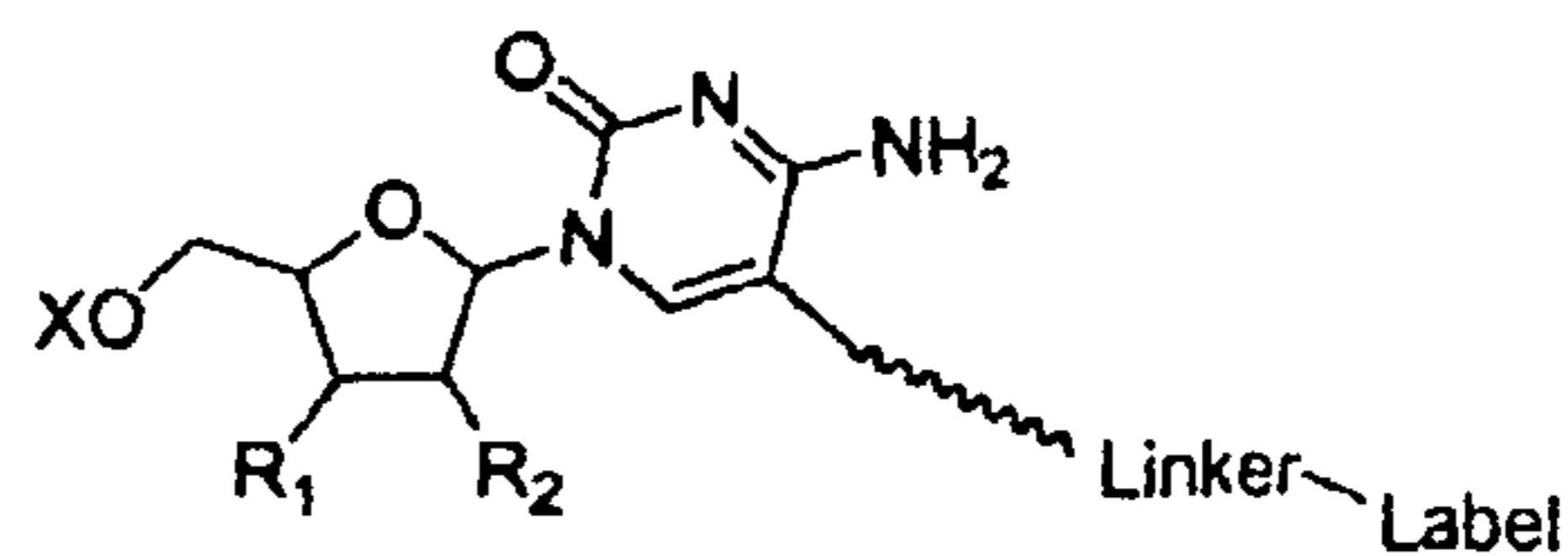
Cytidine C5-linker
