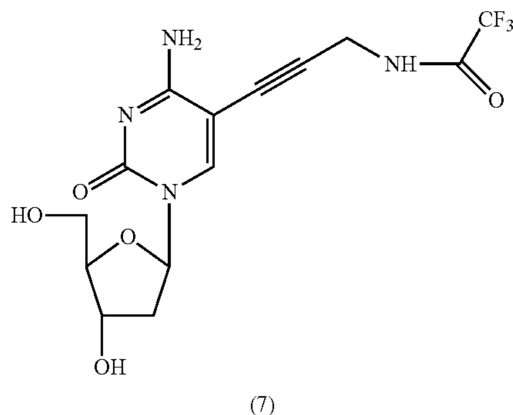
5-[3-(2,2,2-Trifluoroacetamido)-prop-1-ynyl]-2'-deoxycytidine (7)
