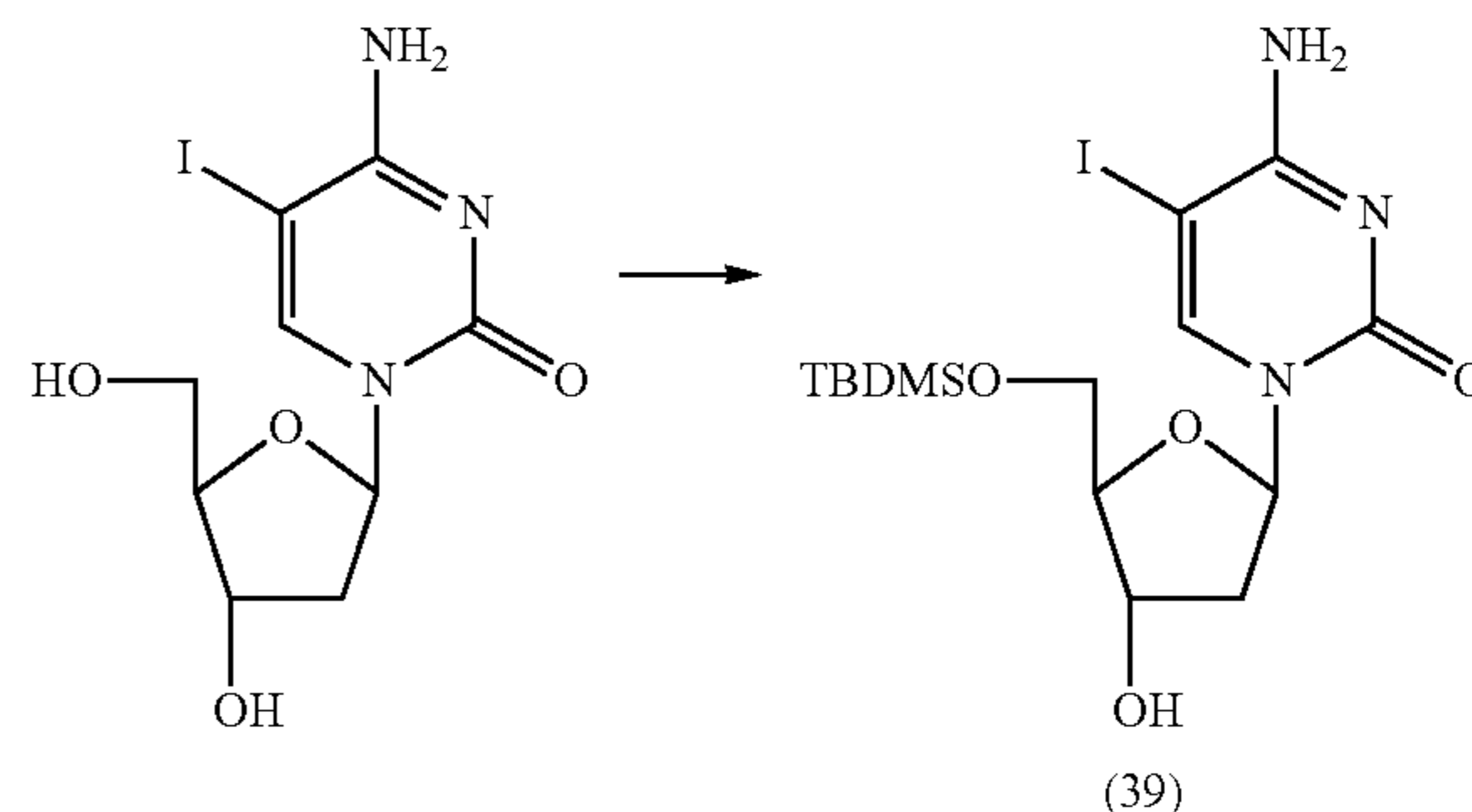
5'-O-(tert-Butyldimethylsilyl)-5-iodo-2'-deoxycytidine (39)
