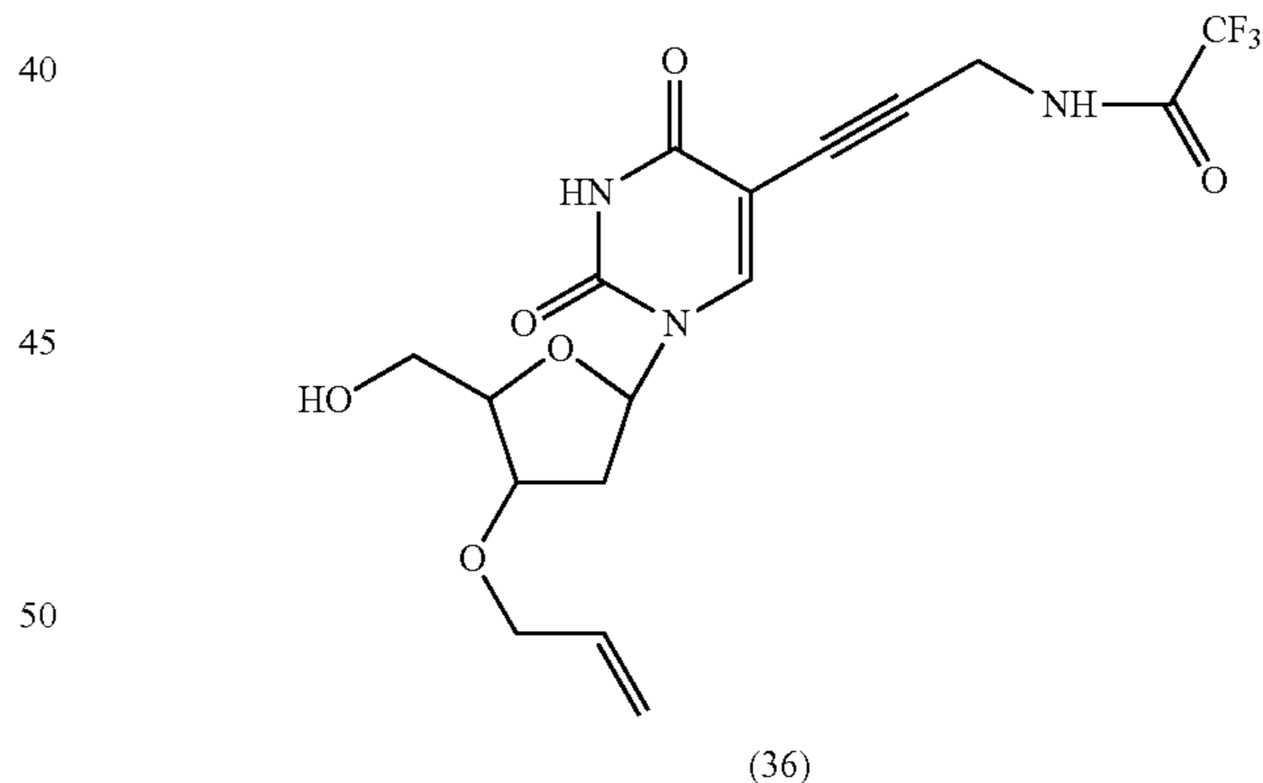
3'-O-Allyl-5-[3-(2,2,2-trifluoroacetamido)-prop-1-ynyl]-2'-deoxyuridine
