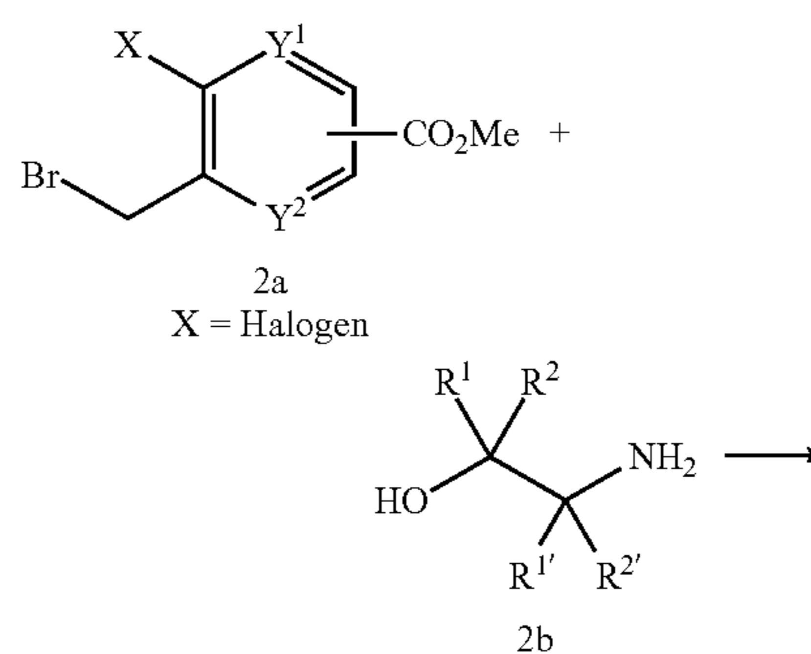
Scheme 1. General synthesis of ethers, thioethers, or sulfones described in the disclosure.
