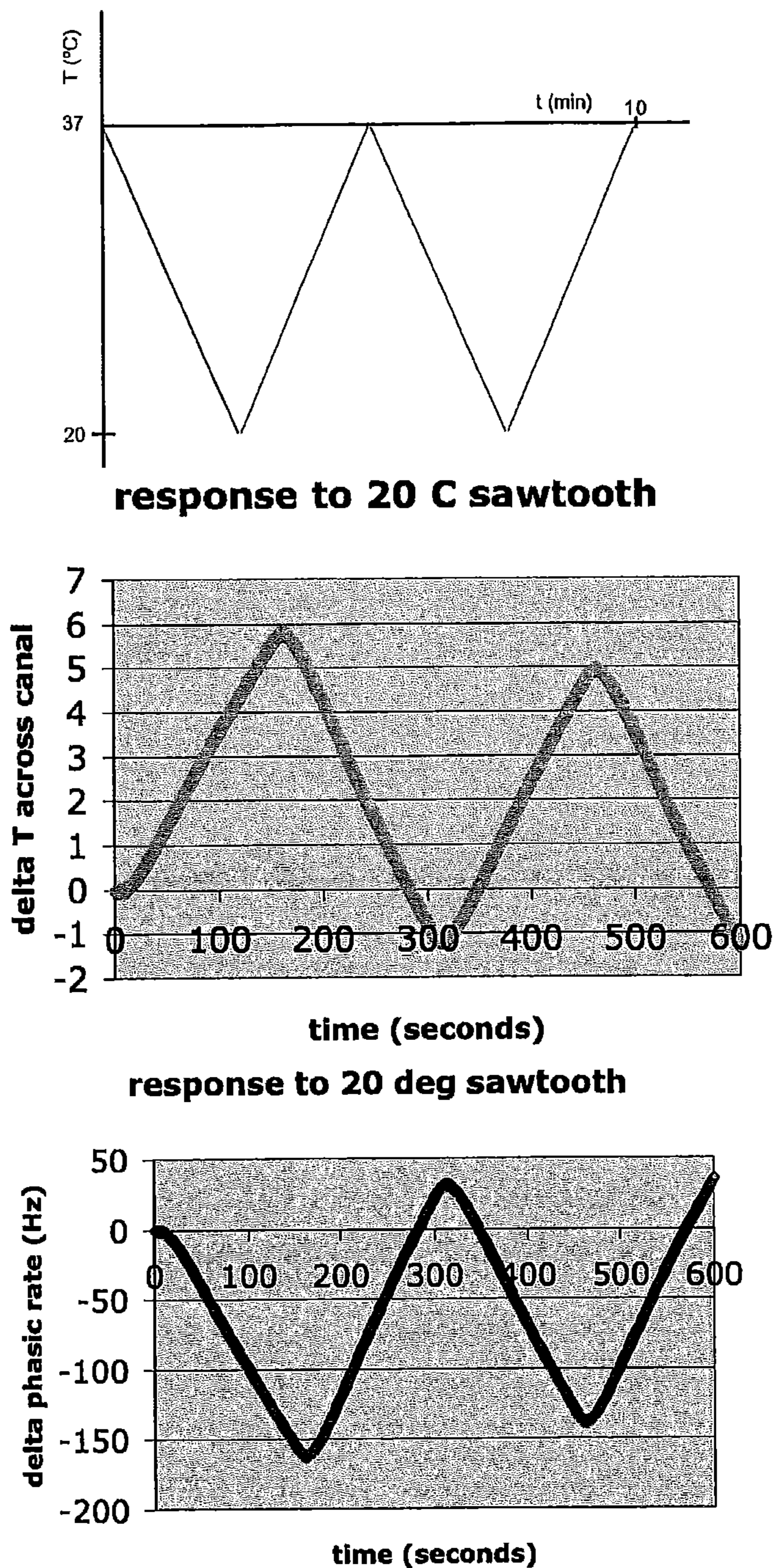
Figure 28. Two consecutive sawtooth waveforms (20 °C) over 10 minutes.
