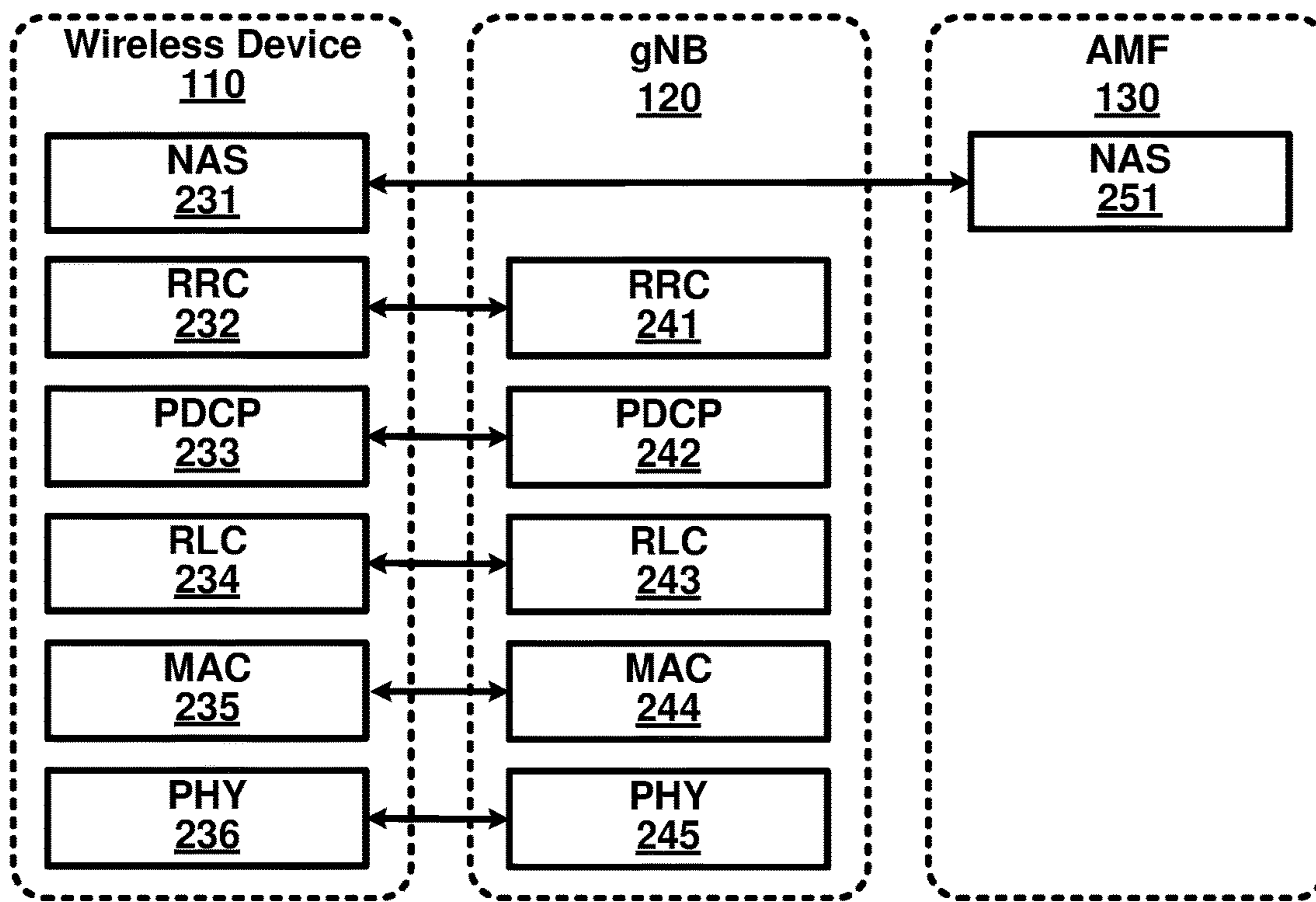
Control Plane Protocol Stack
