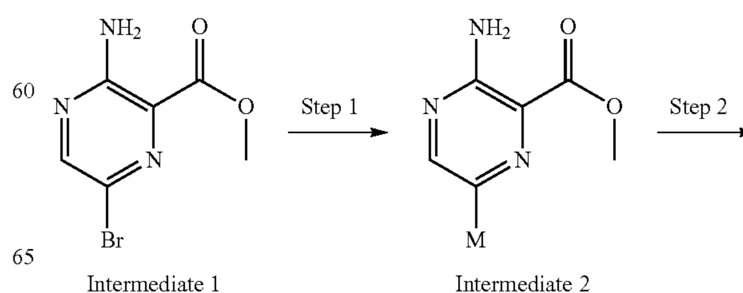
Scheme 1
