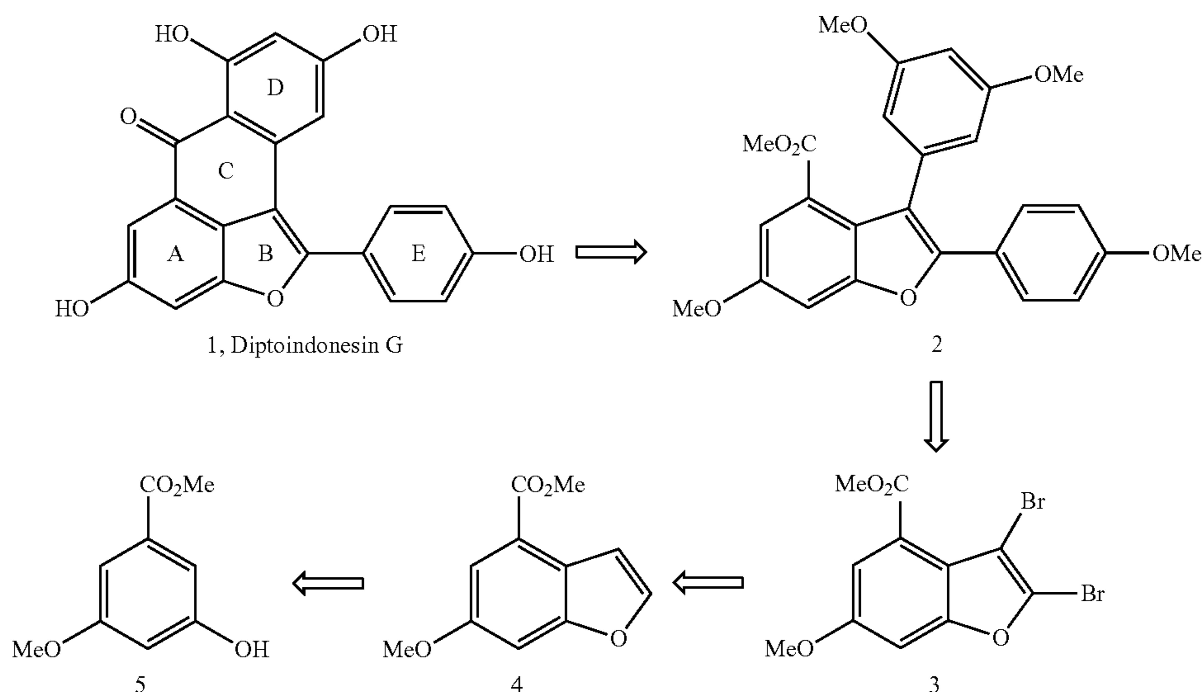
Scheme 1: Retrosynthetic Analysis of Dip G
