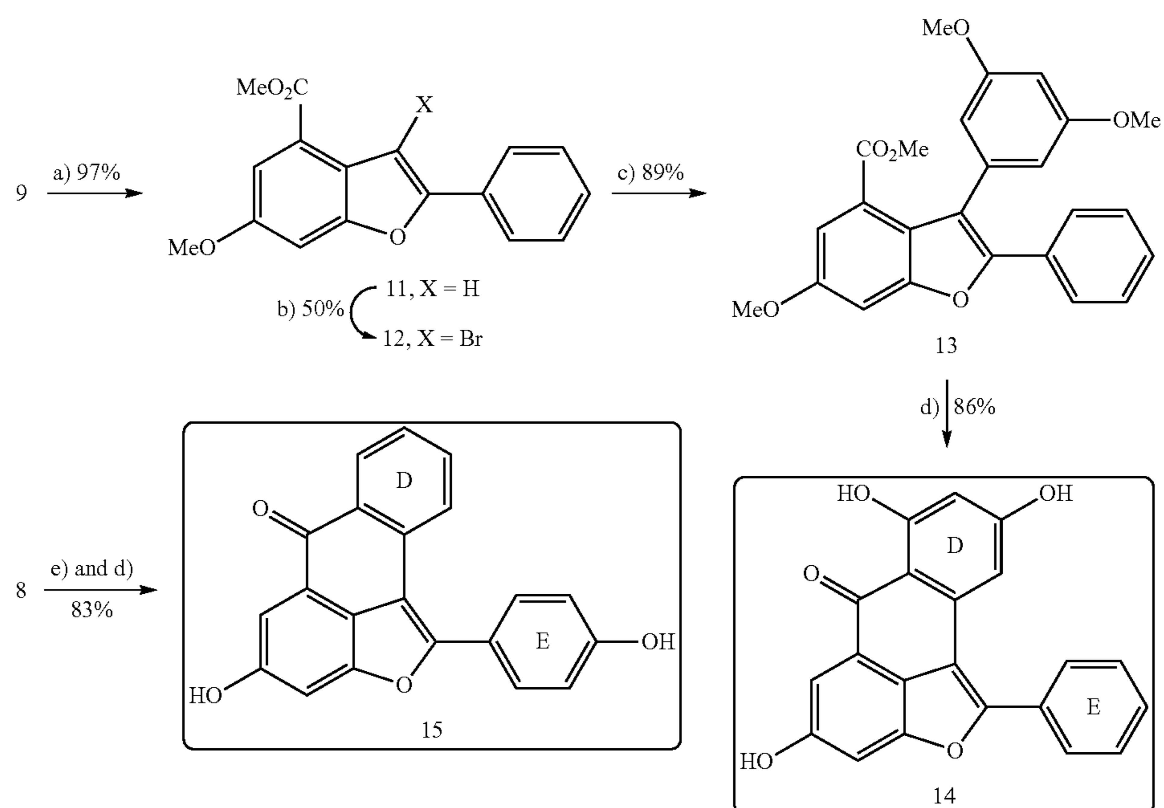
Scheme 4: Synthesis of Dip G Analogs
