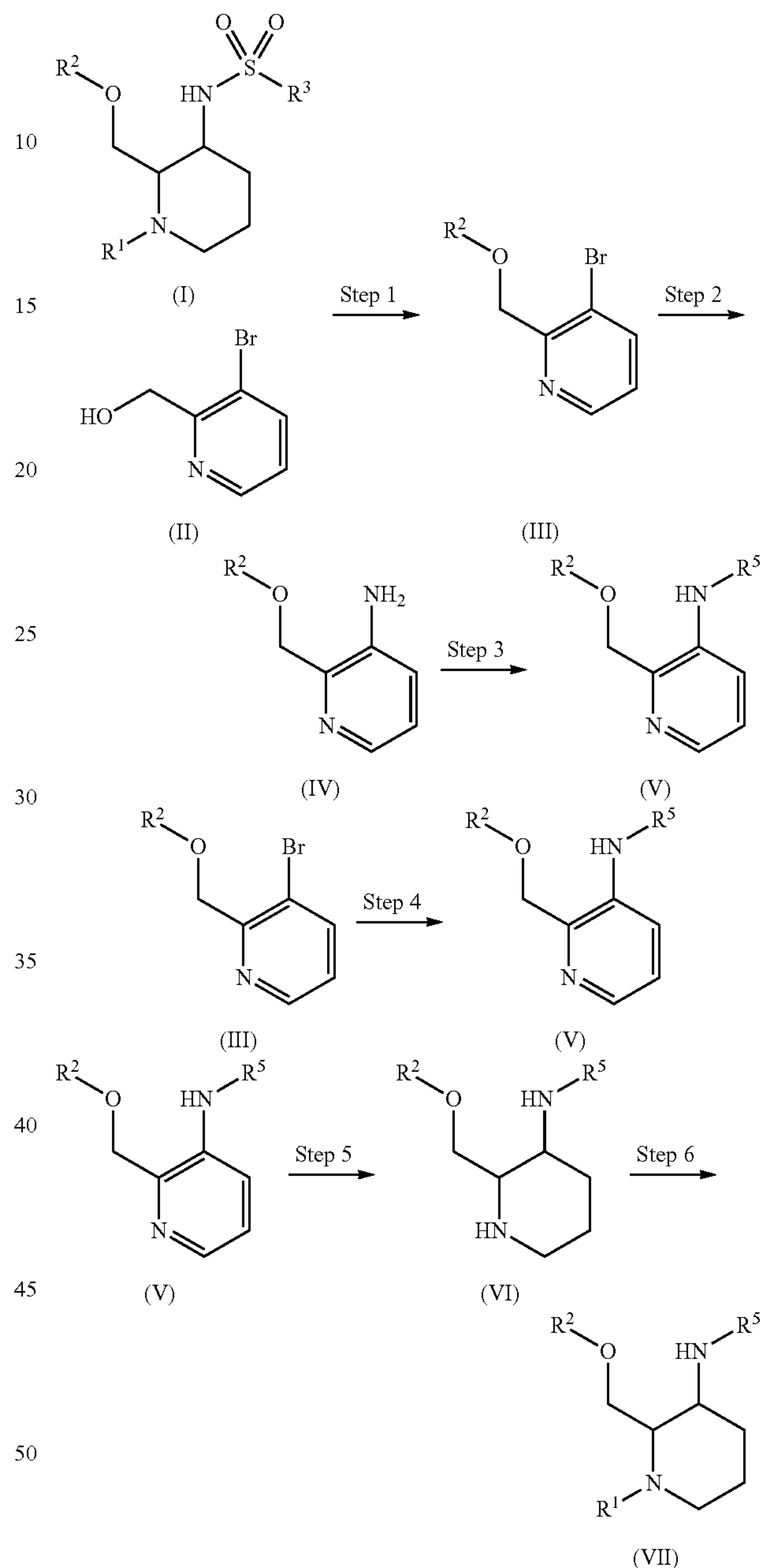
(Scheme 1)
