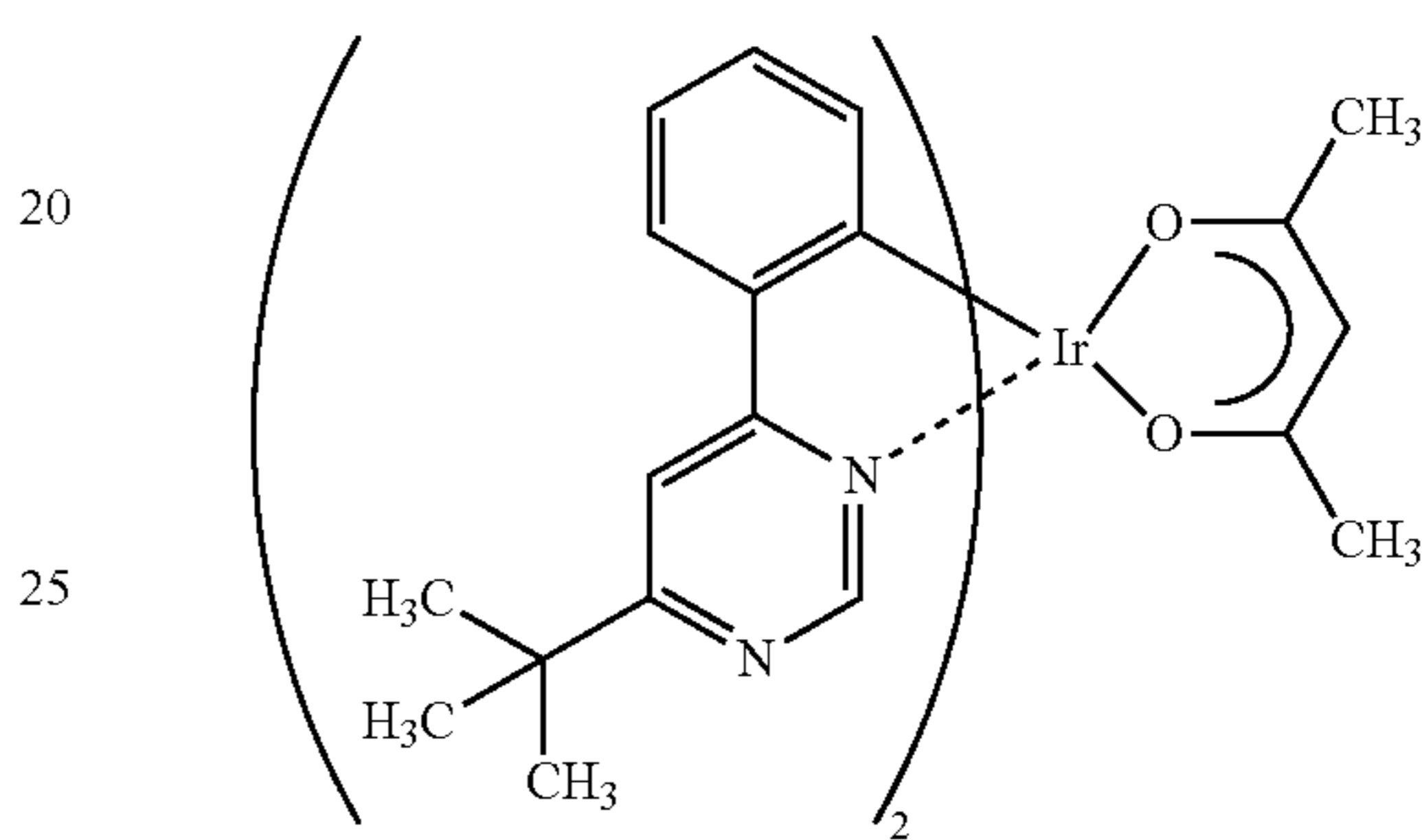
Ir(tBuppm) 2 (acac)
