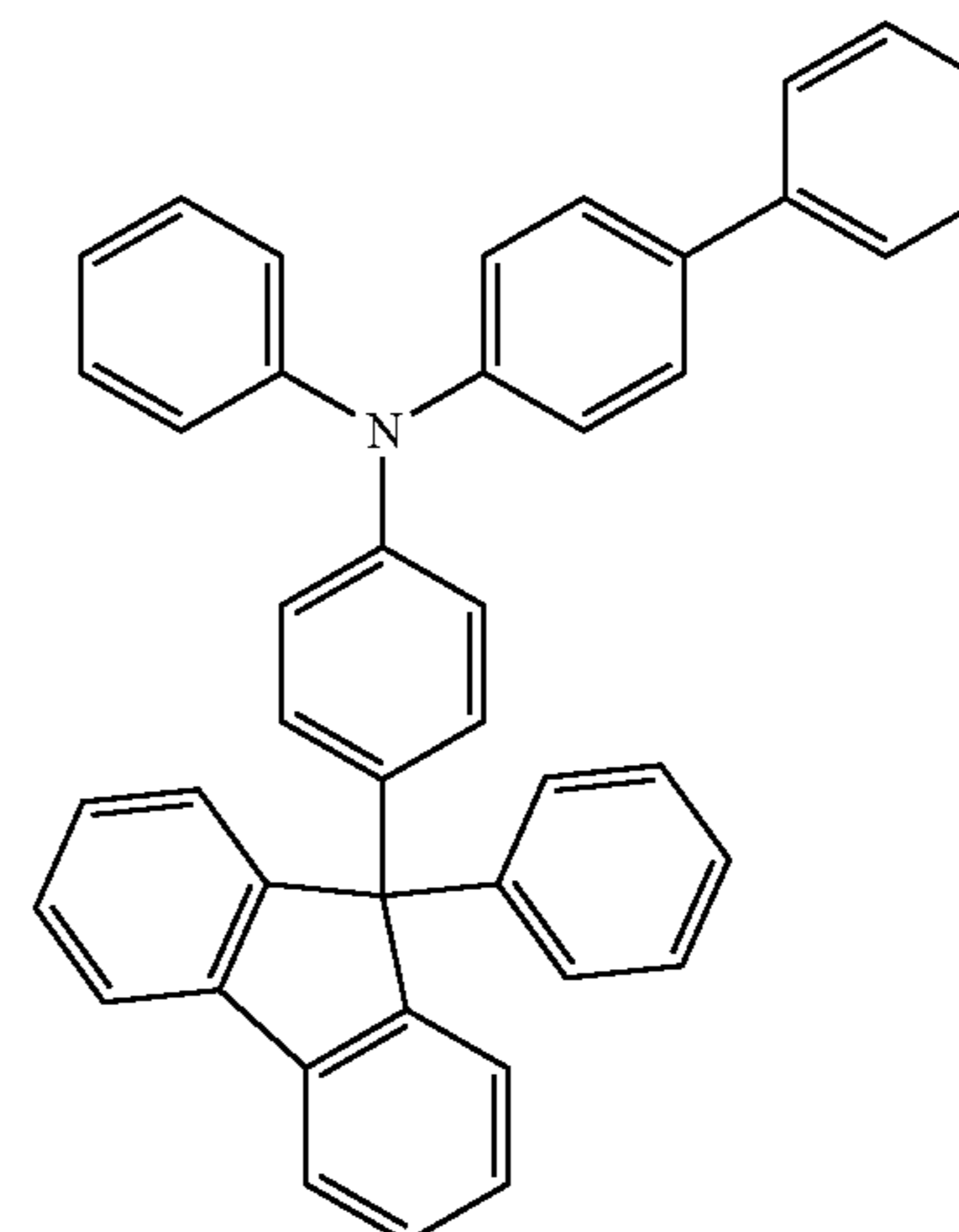
BPAFLP
