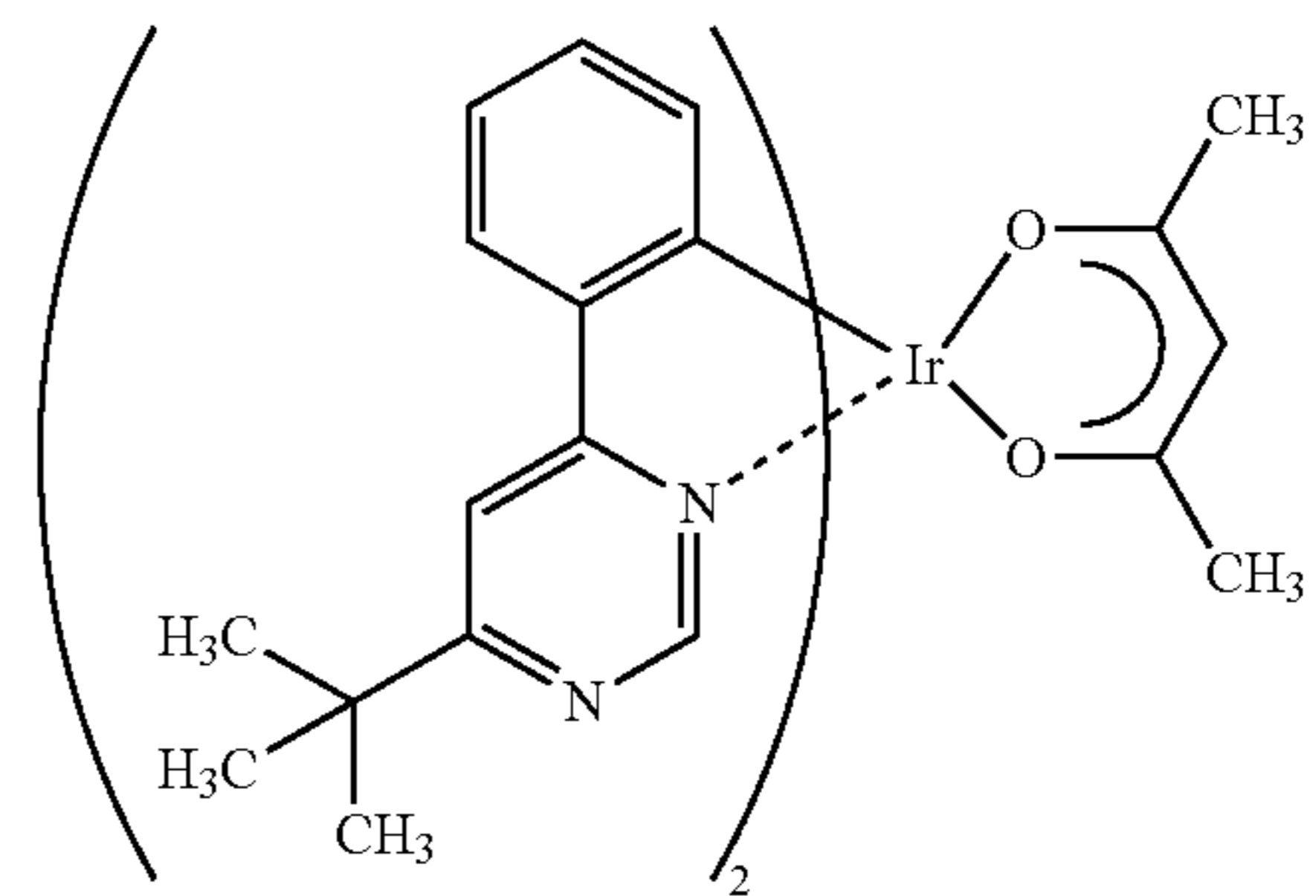
Ir(tBuppm) 2 (acac)
