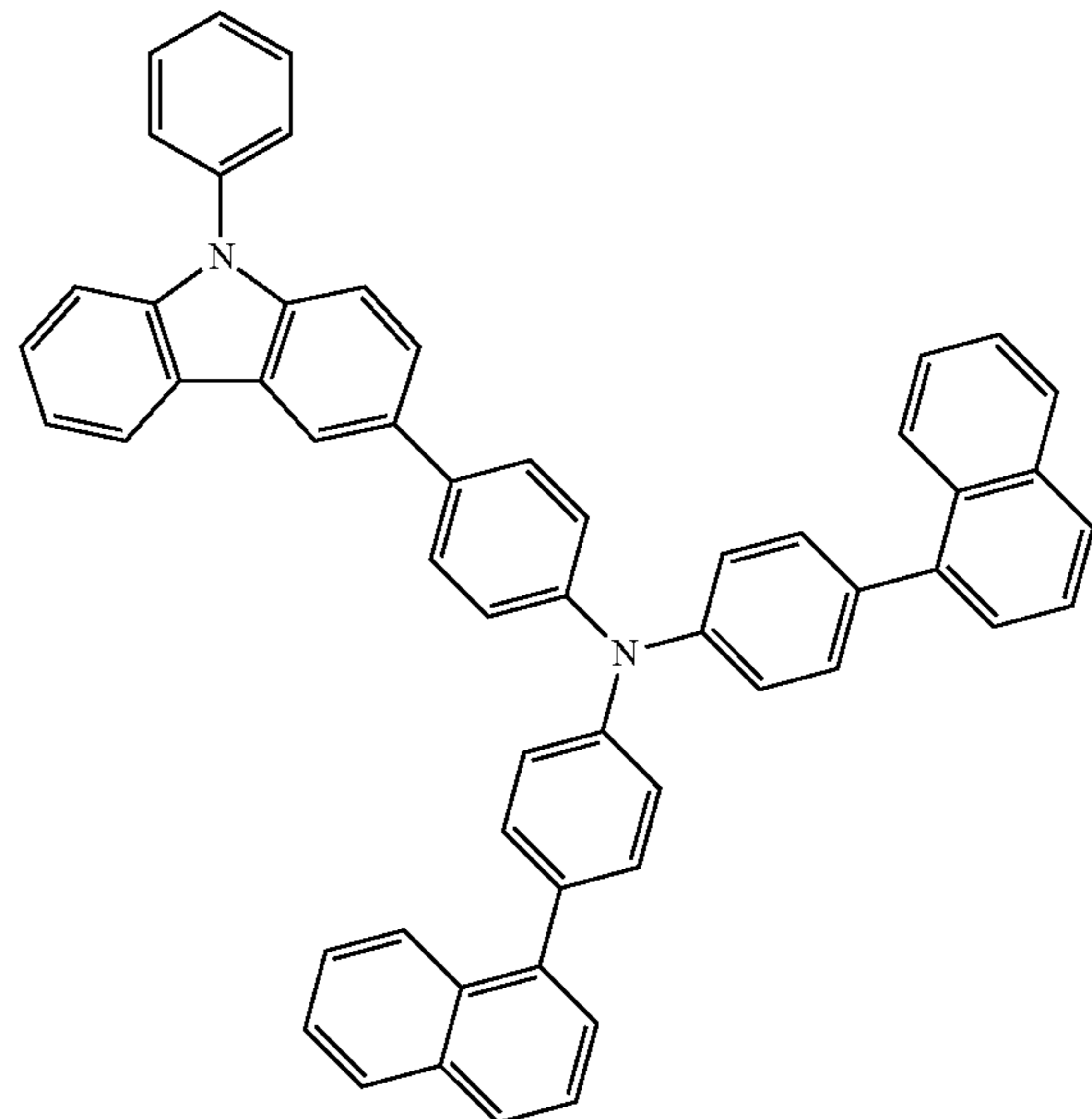
PCBNBB
