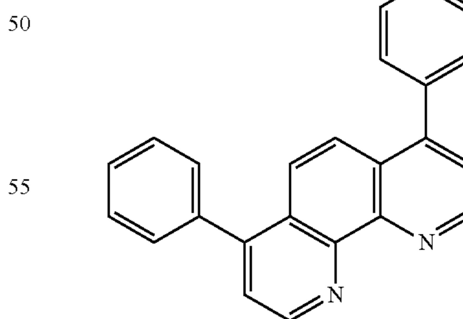
BPhen
