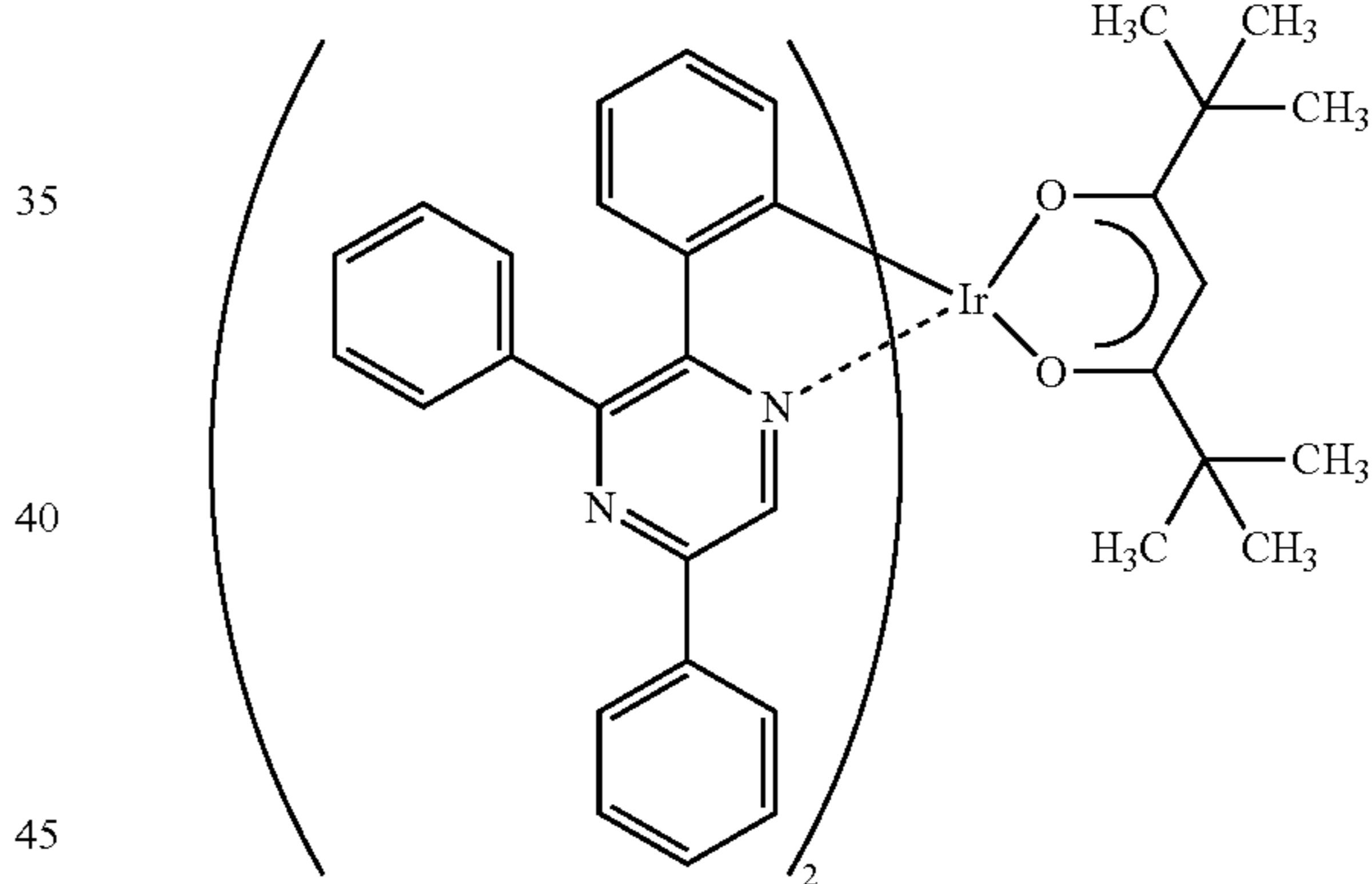
Ir(tppr) 2 (dpm)
