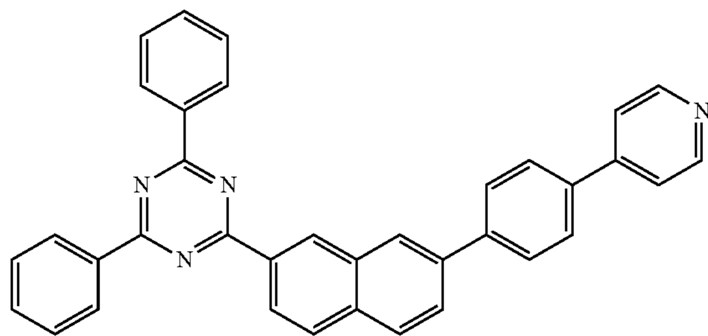
[formula 5-1-3]
