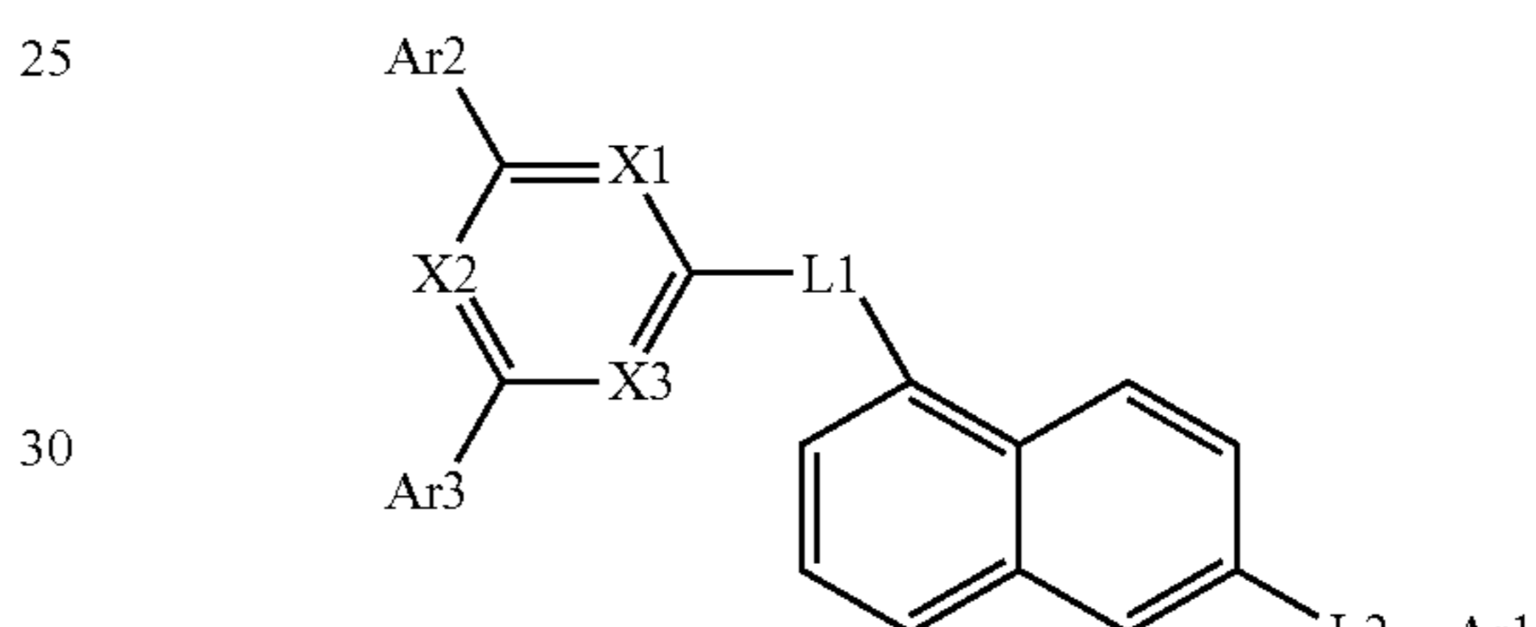
[Chemical Formula 1-8]
