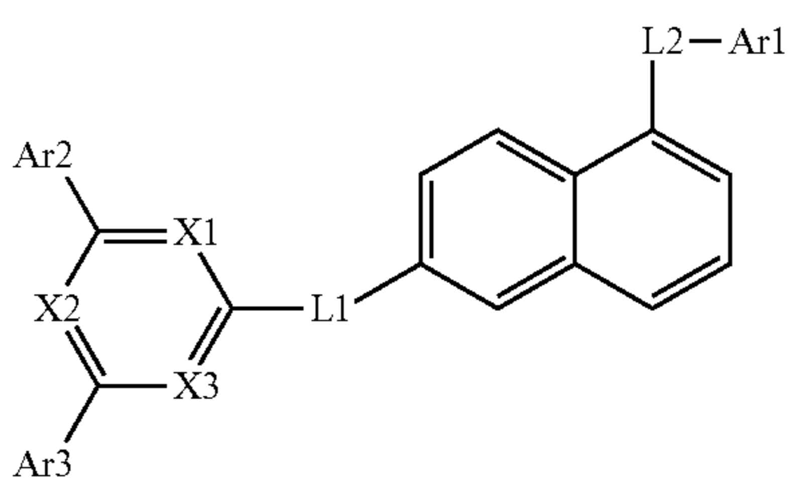
[Chemical Formula 1-4]
