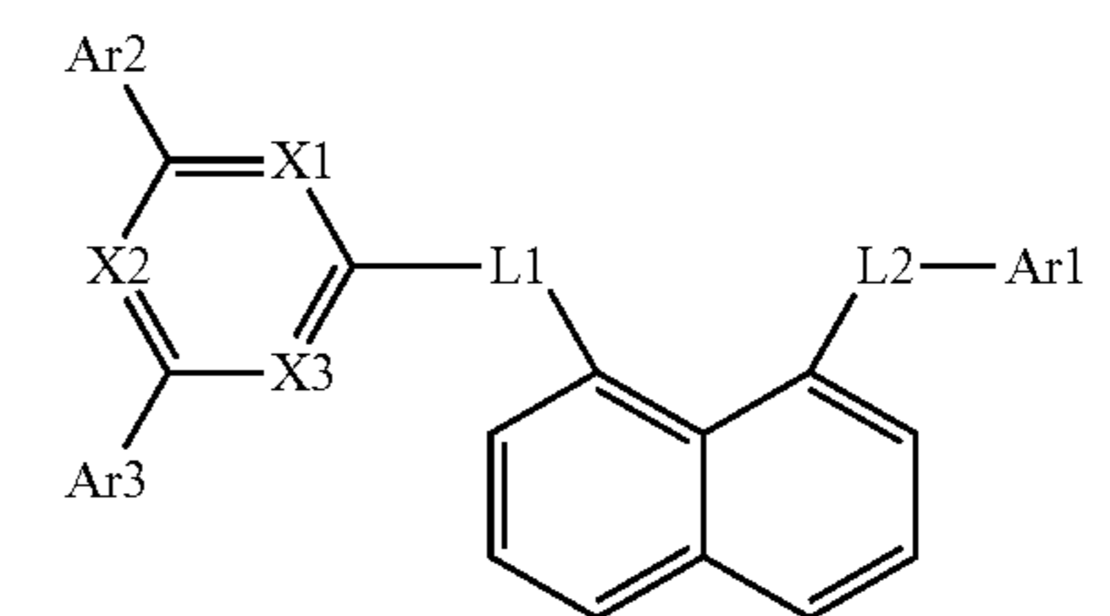
[Chemical Formula 1-6]
