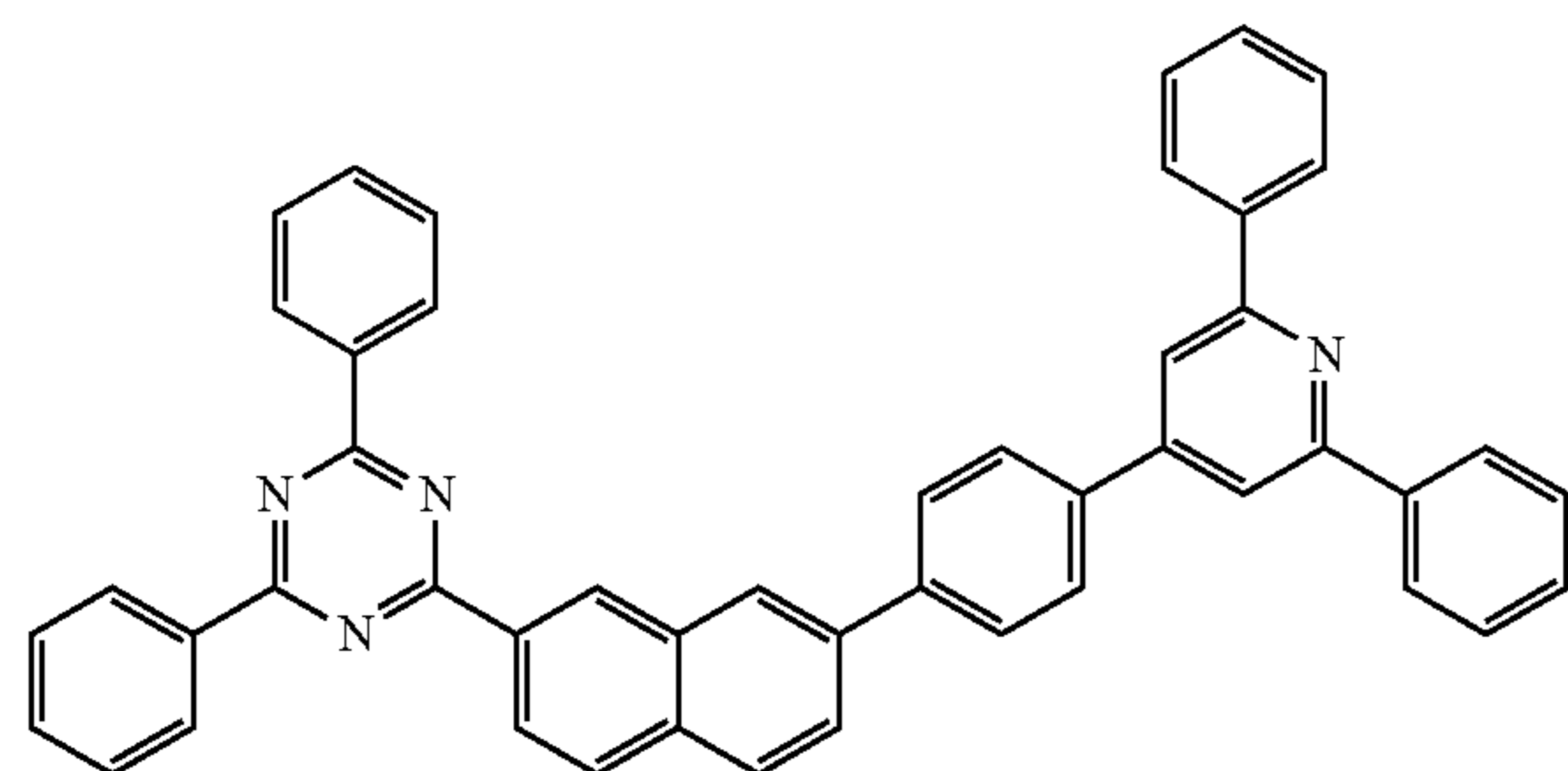
[formula 5-1-4]
