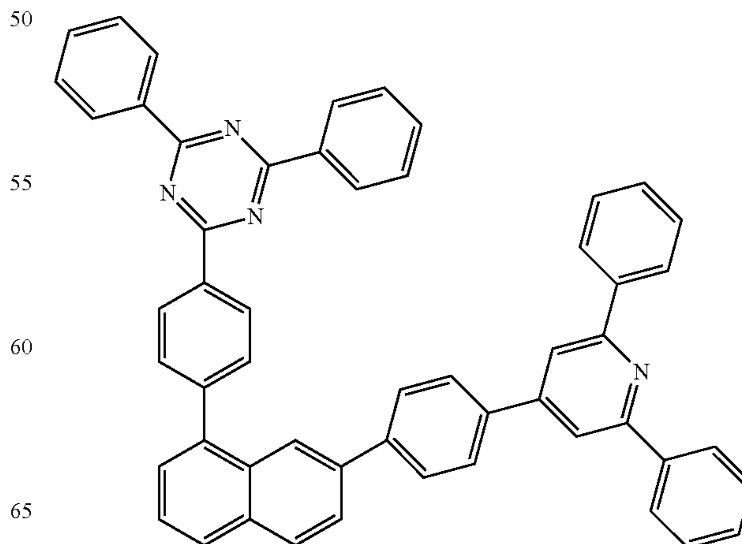
[formula 2-6-3]
