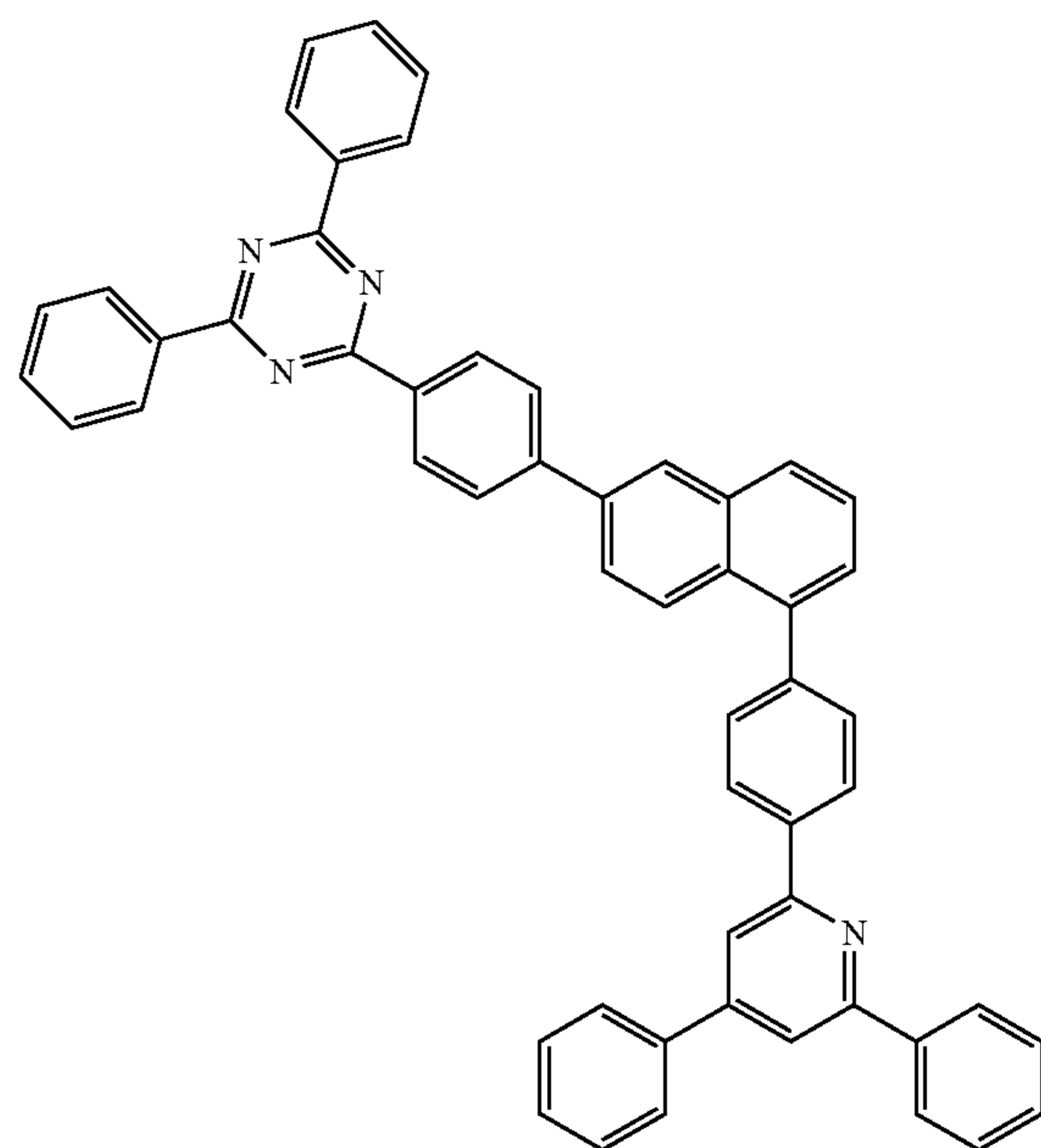
[formula 2-3-1]
