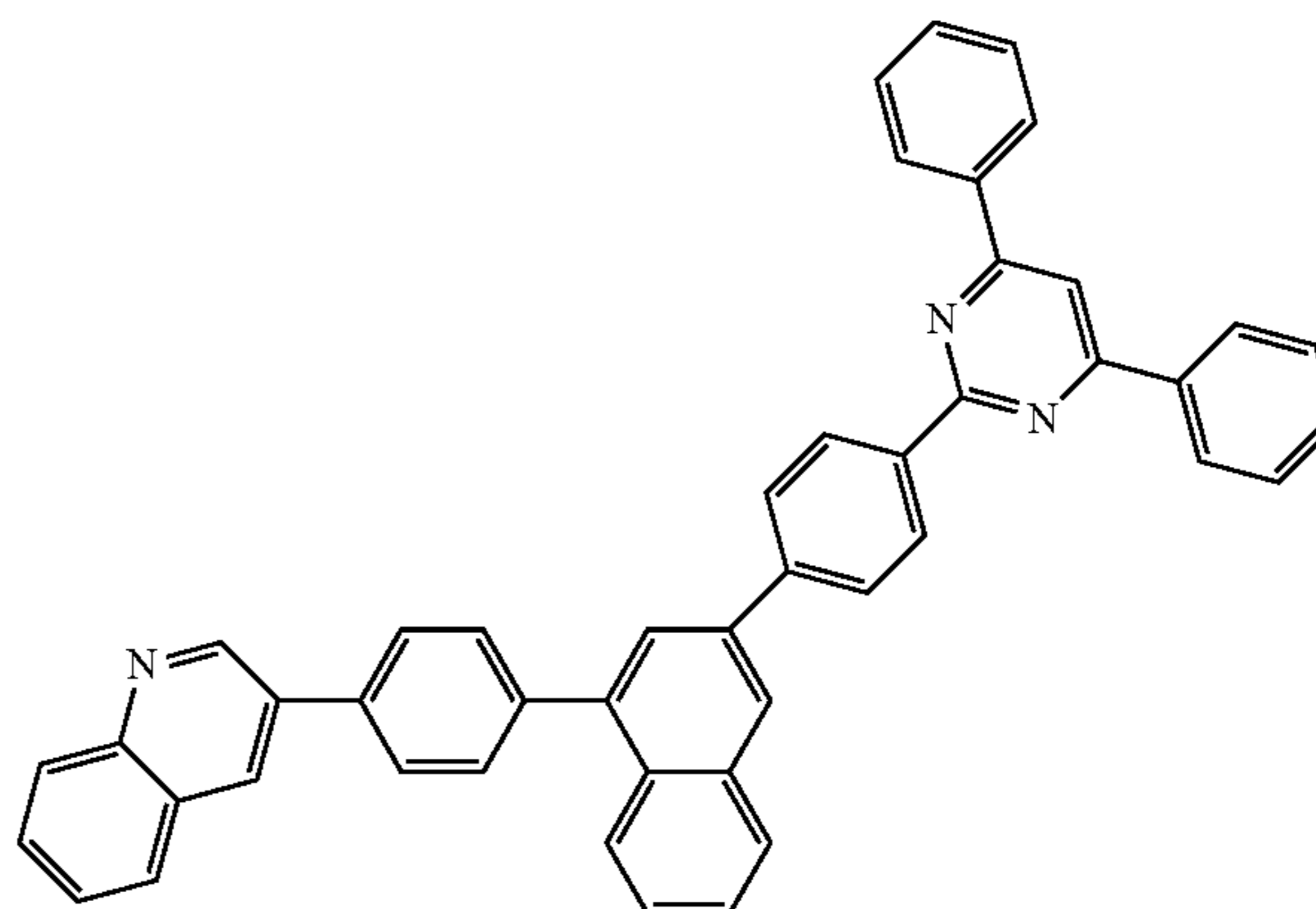
[formula 3-10-6]
