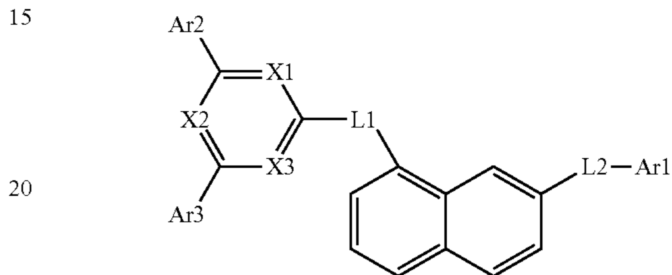
[Chemical Formula 1-7]
