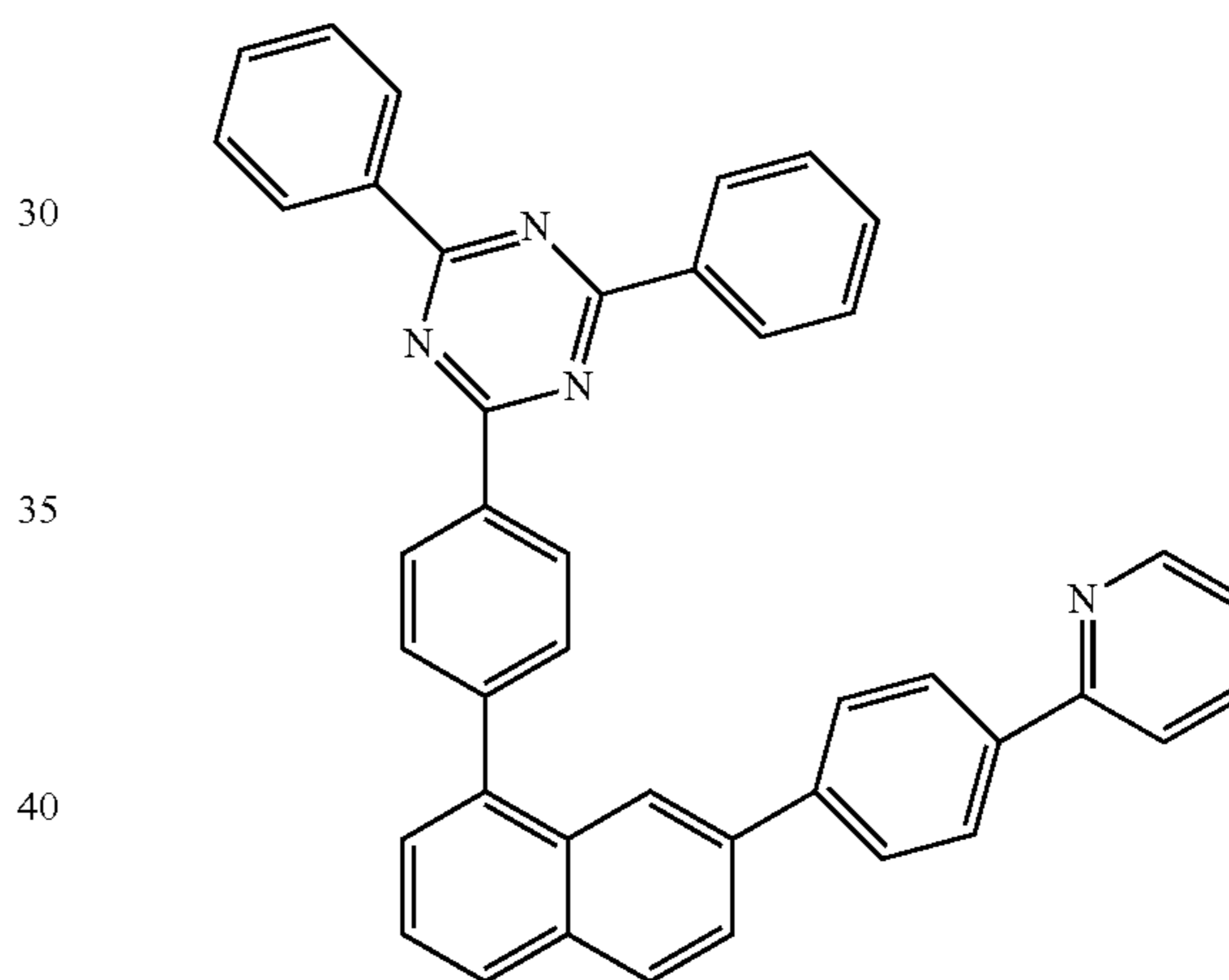
[formula 2-6-2]
