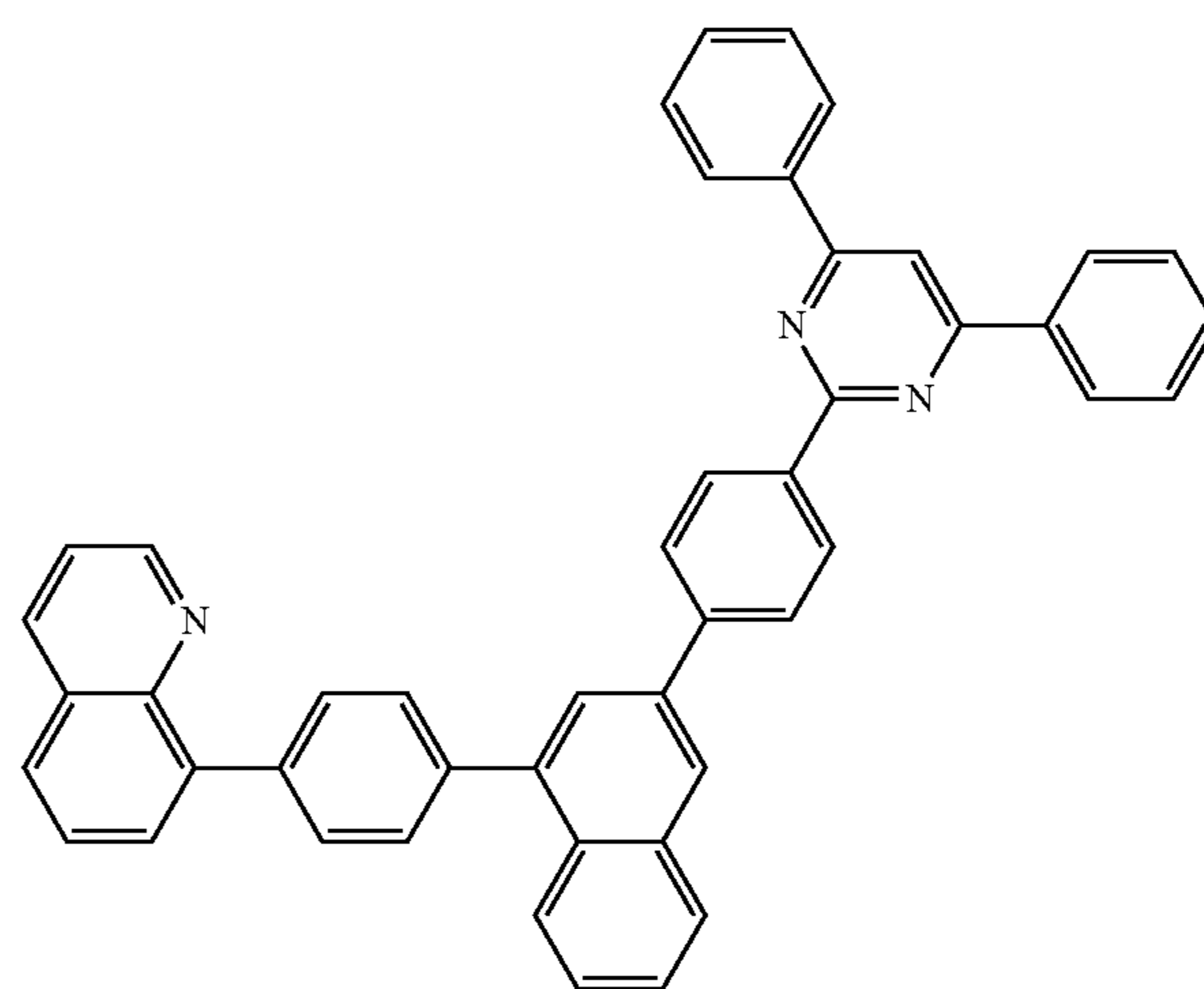
[formula 3-10-5]
