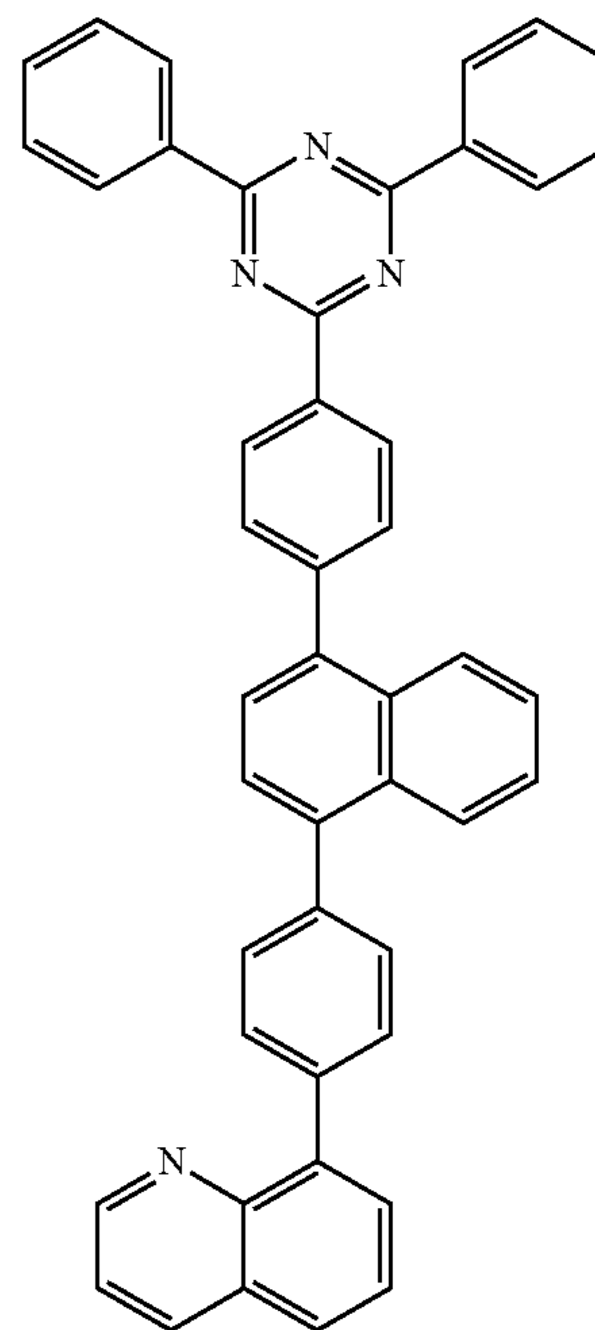
[Chemical Formula 3-12-1]
