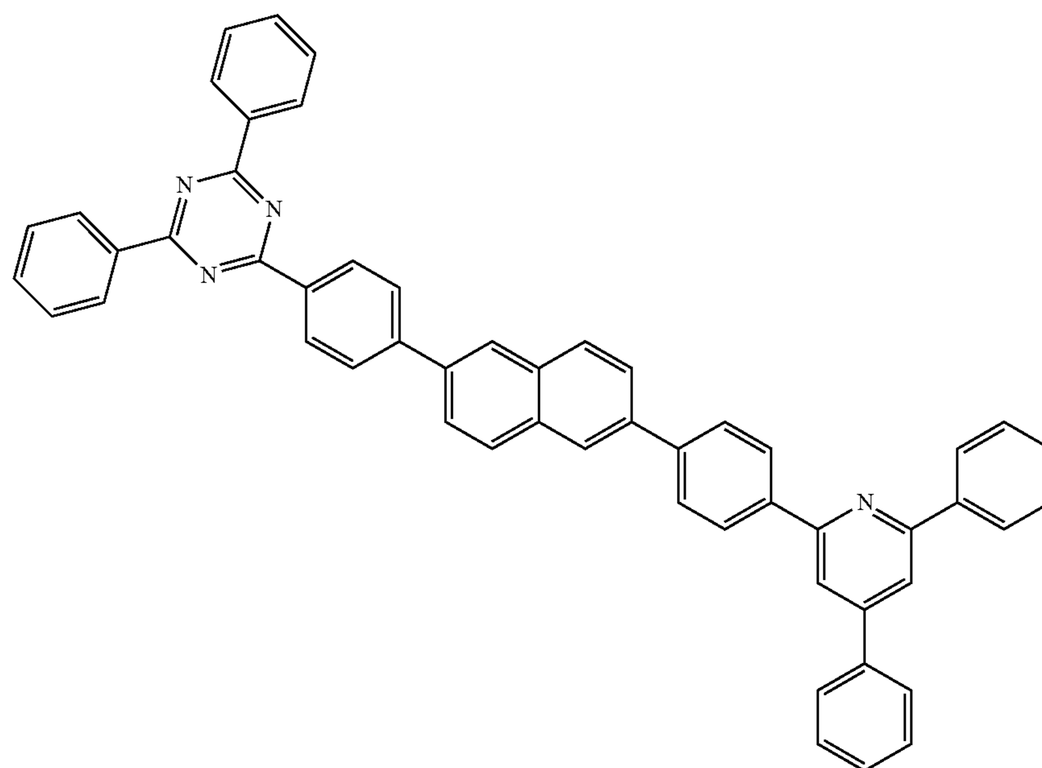
[Chemical Formula 2-4-1]
