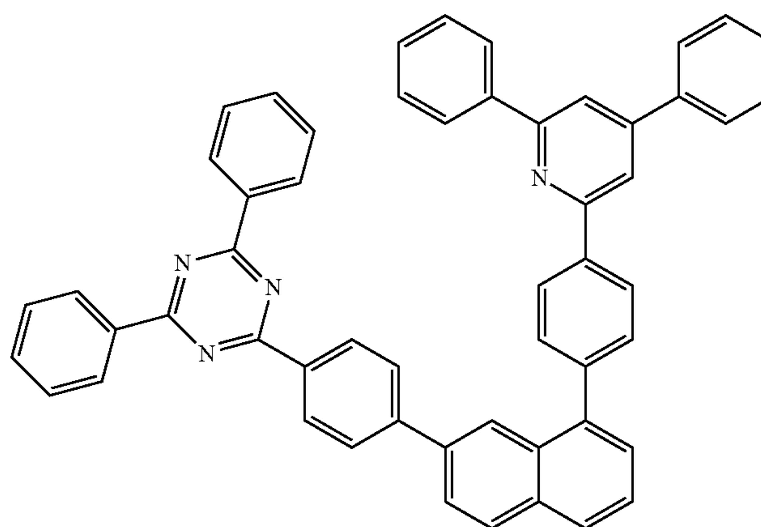
[Chemical Formula 2-2-1]
