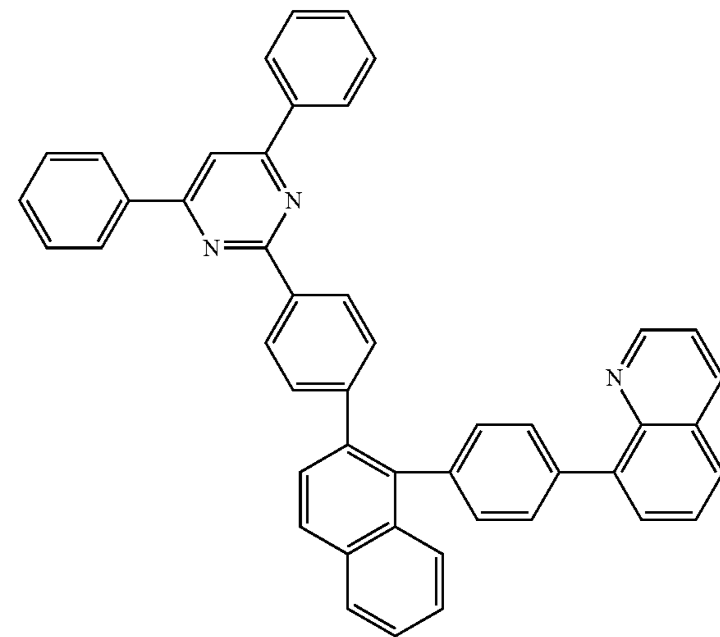
[formula 3-11-6]
