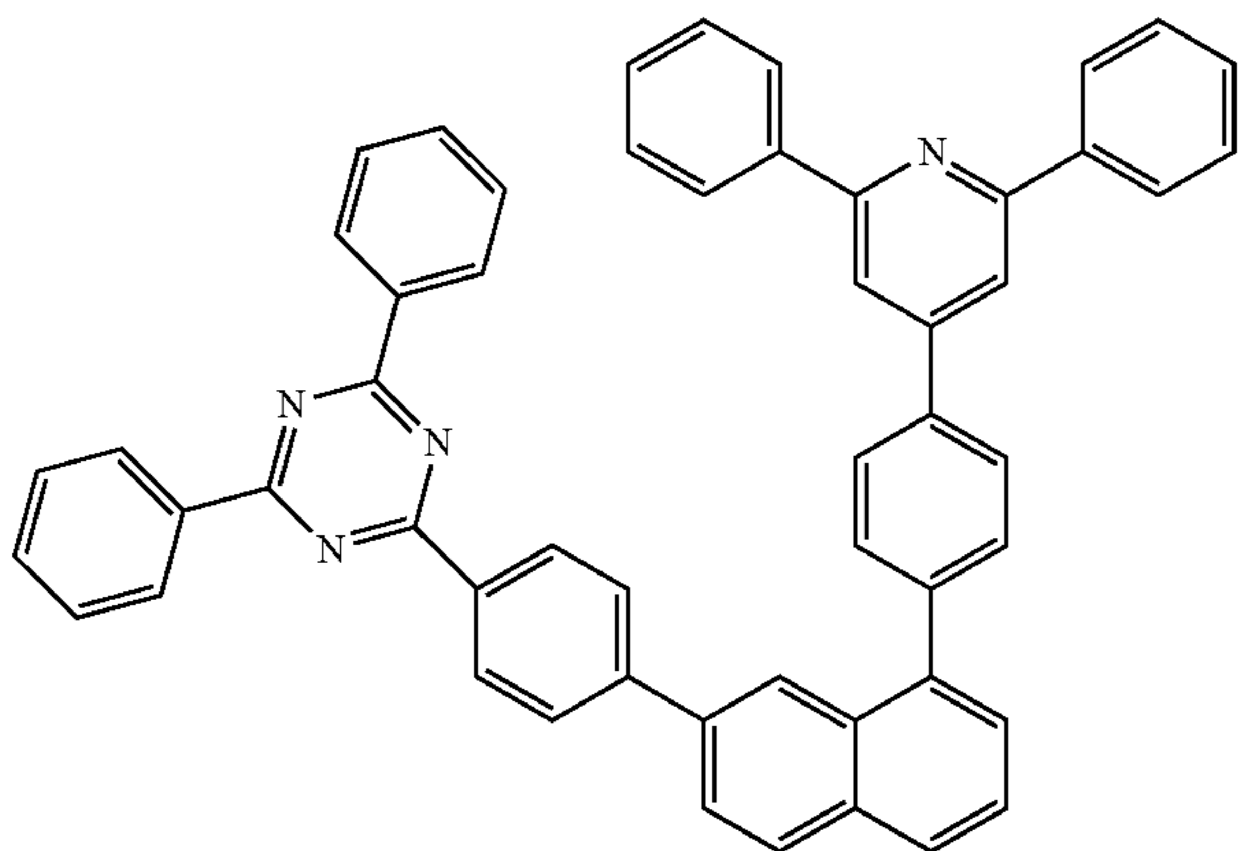
[formula 2-2-3]
