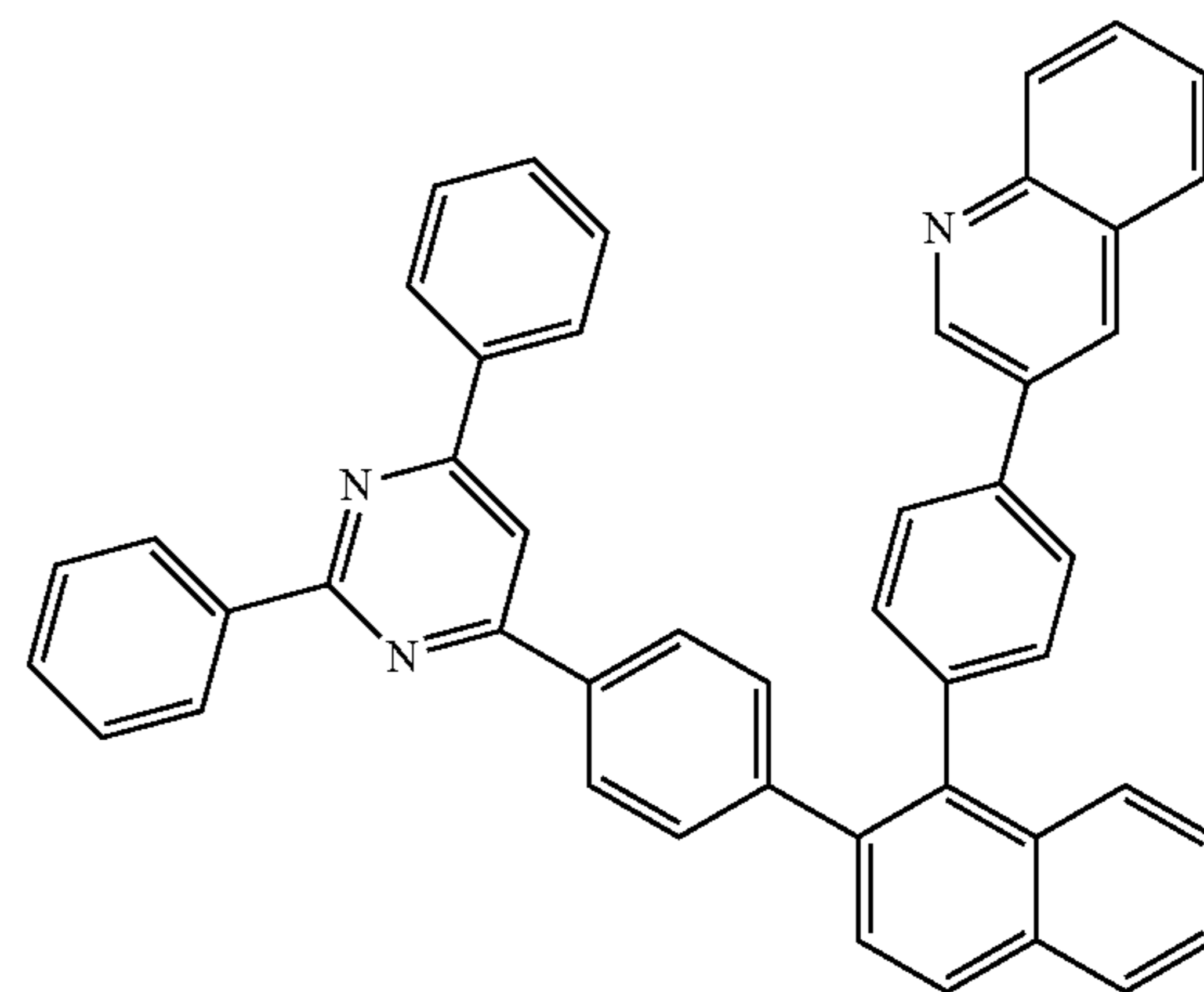
[formula 3-11-4]
