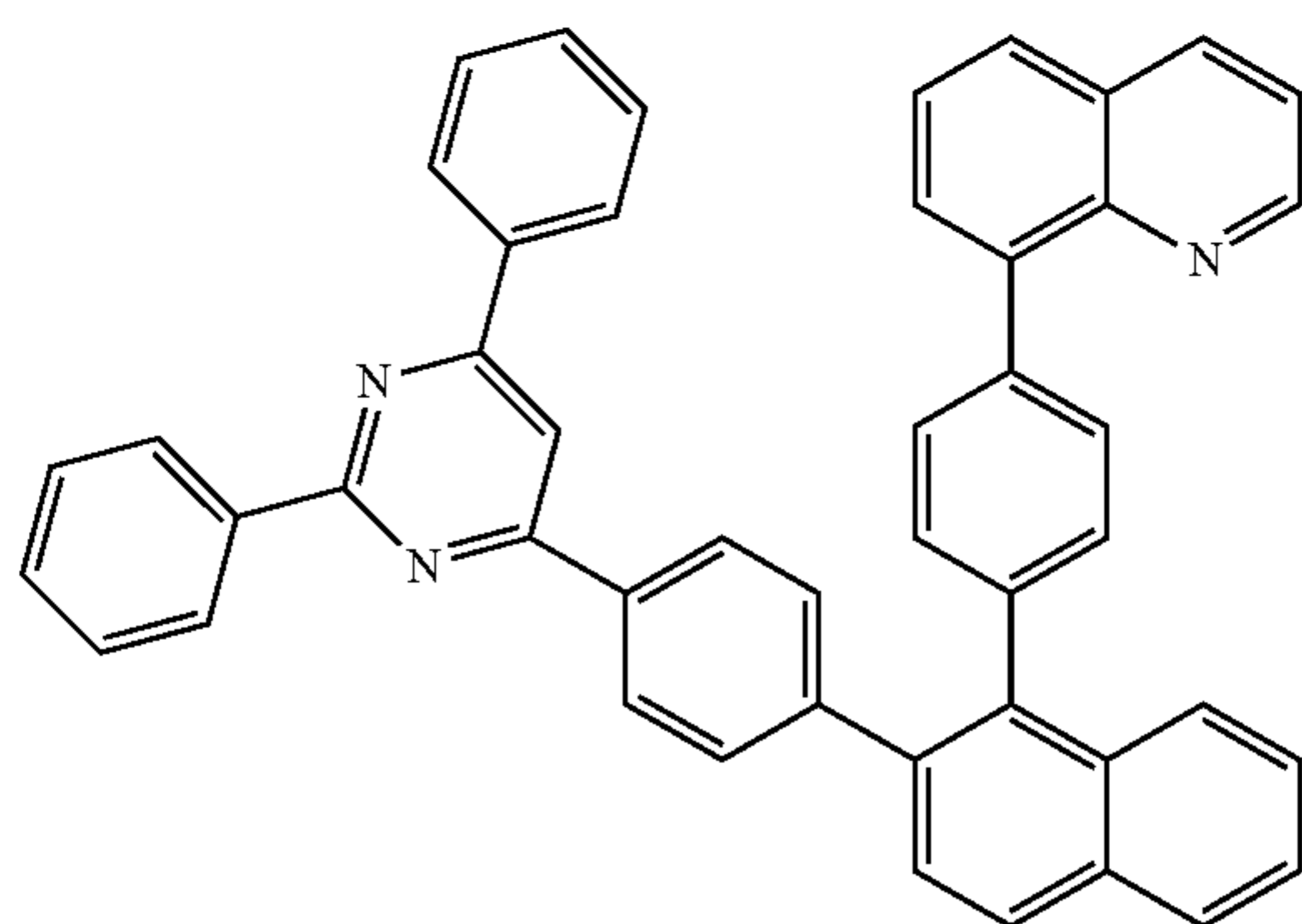
[formula 3-11-3]
