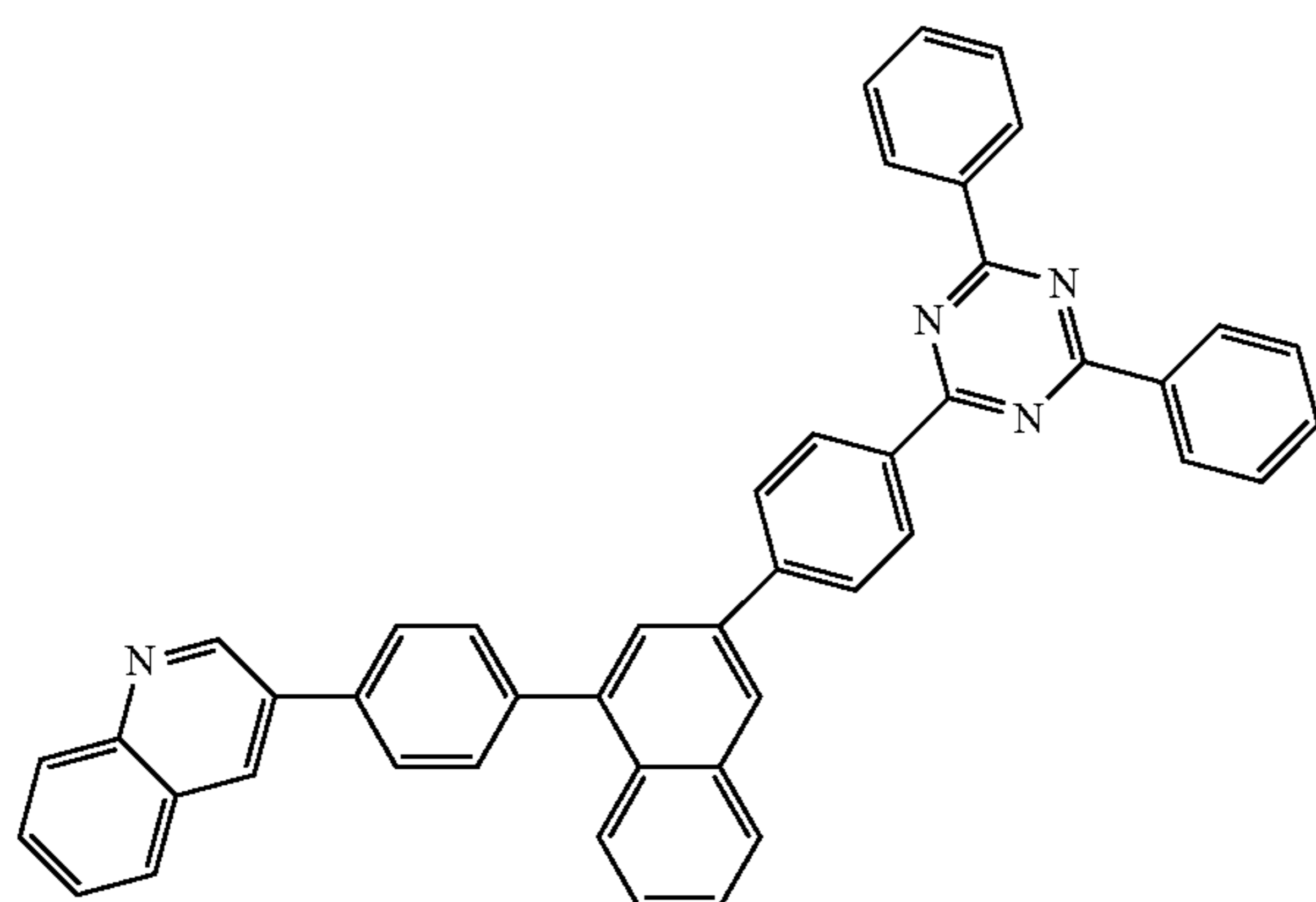
[formula 3-10-2]
