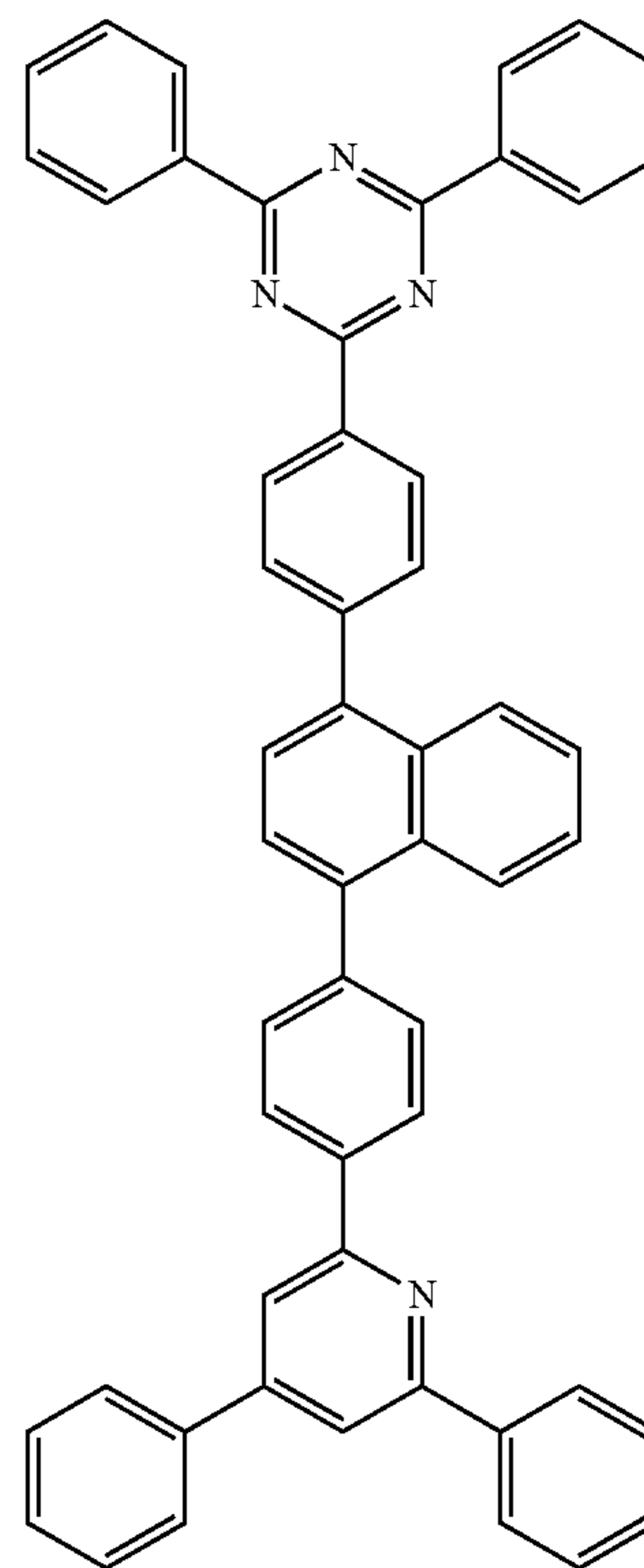
[Chemical Formula 2-12-1]
