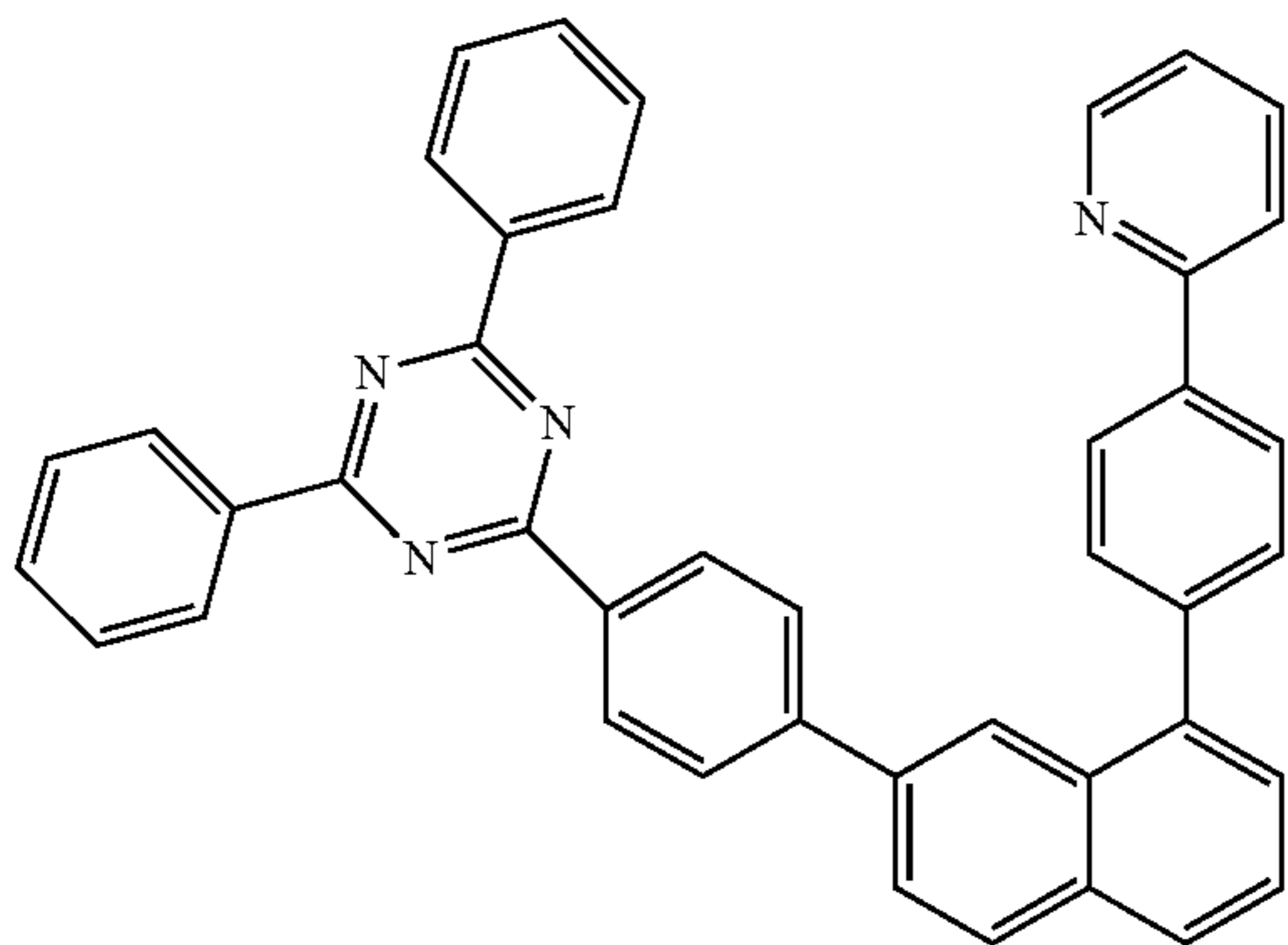
[formula 2-2-2]
