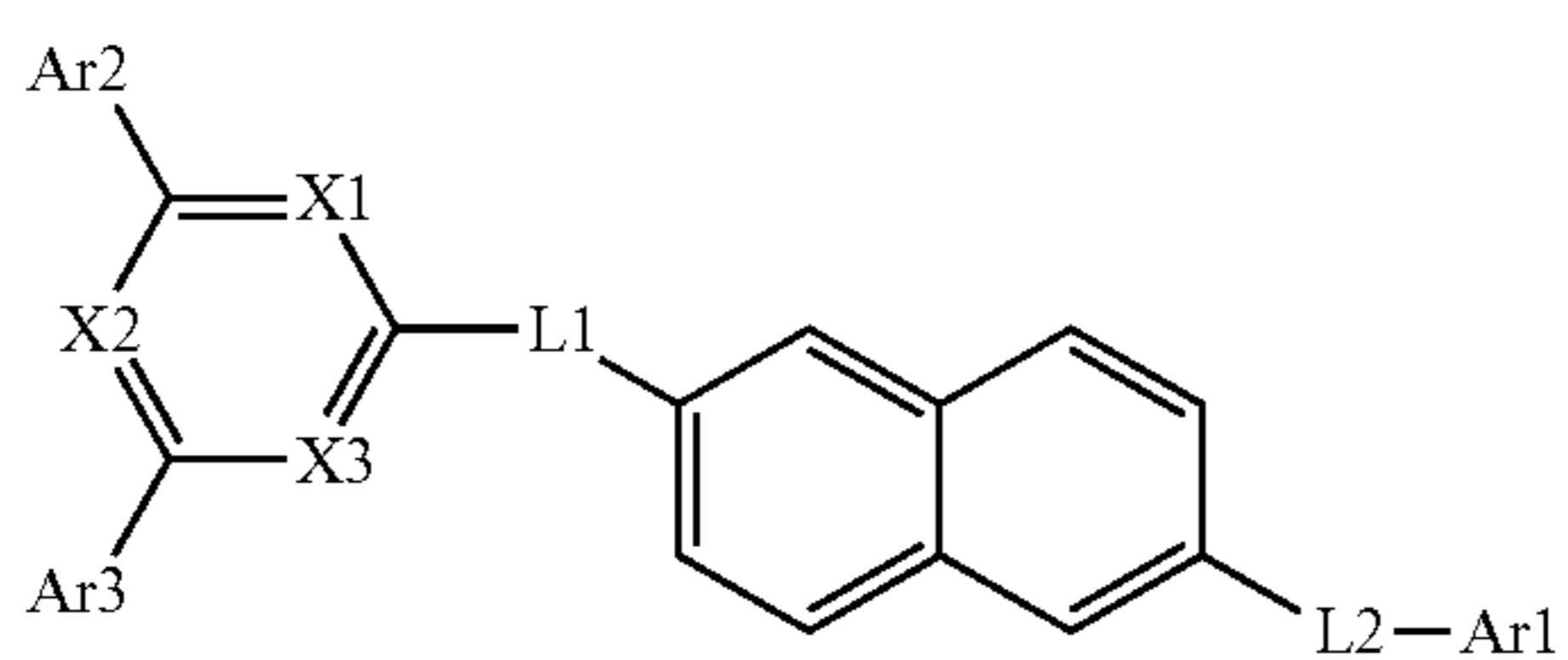
[Chemical Formula 1-4]
