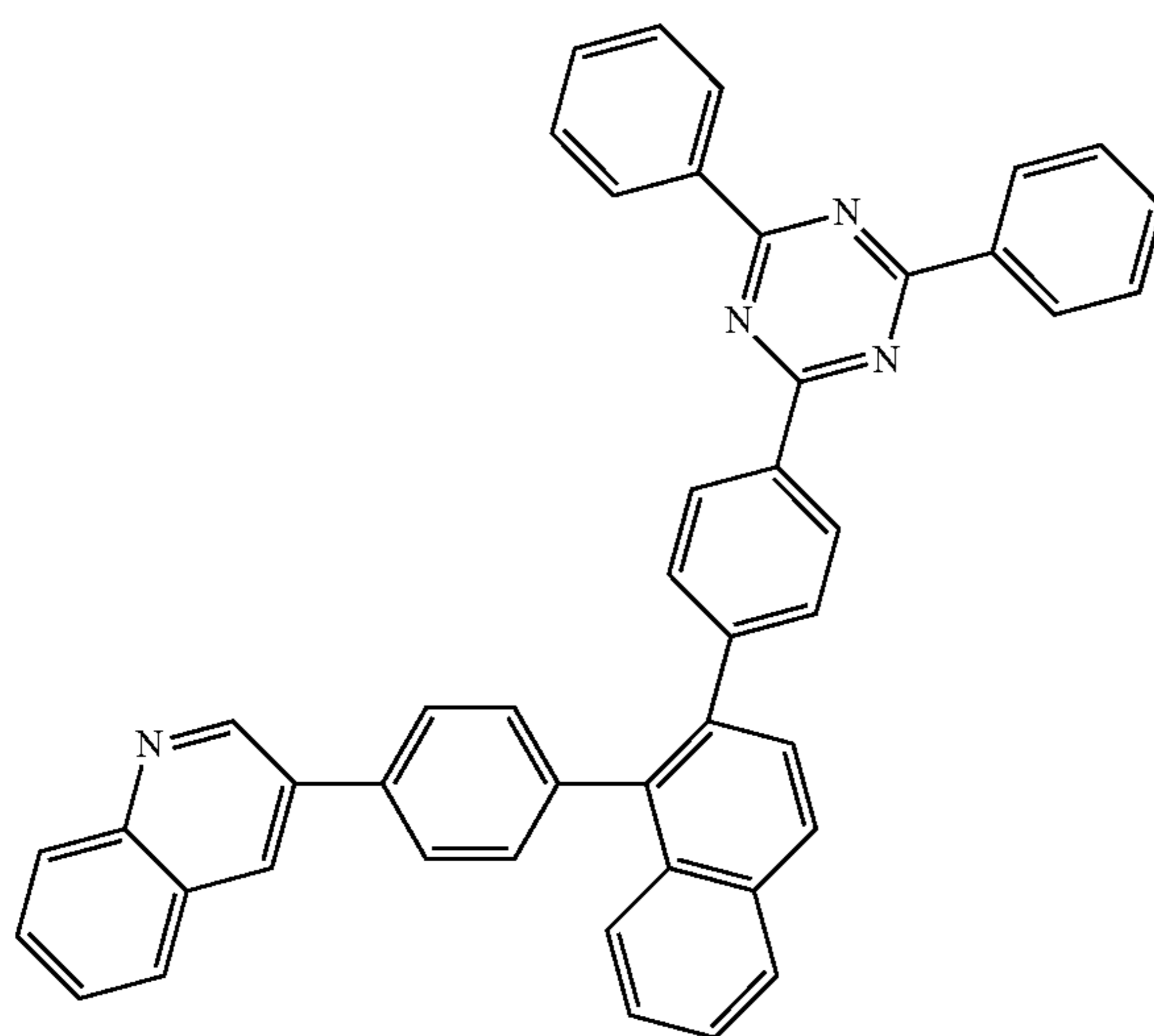
[formula 3-11-2]
