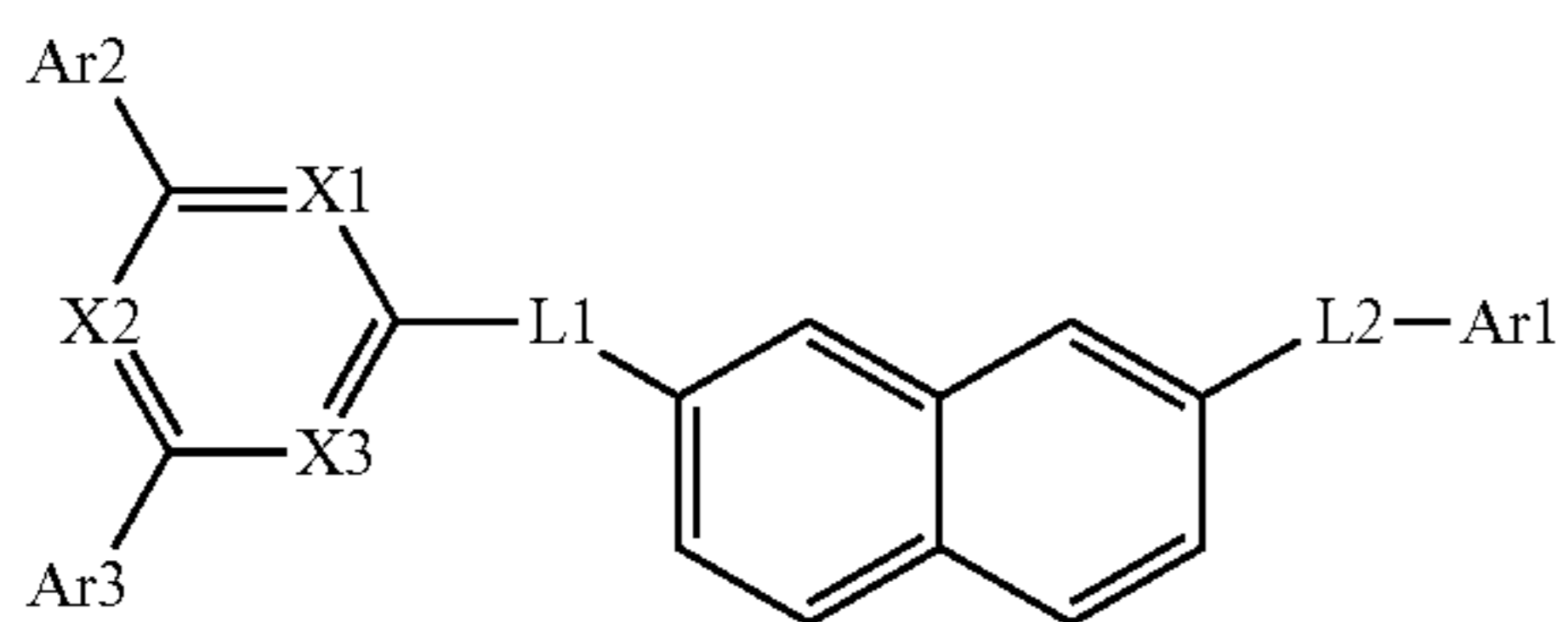
[Chemical Formula 1-1]
