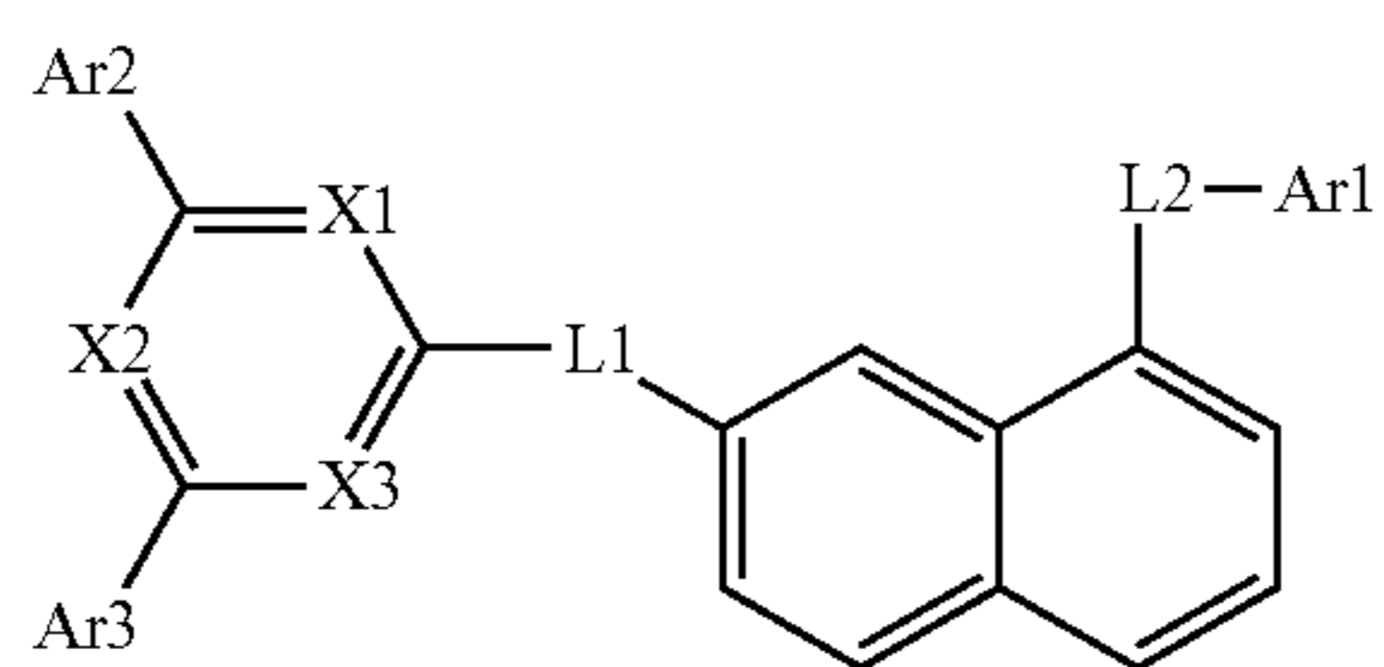
[Chemical Formula 1-2]
