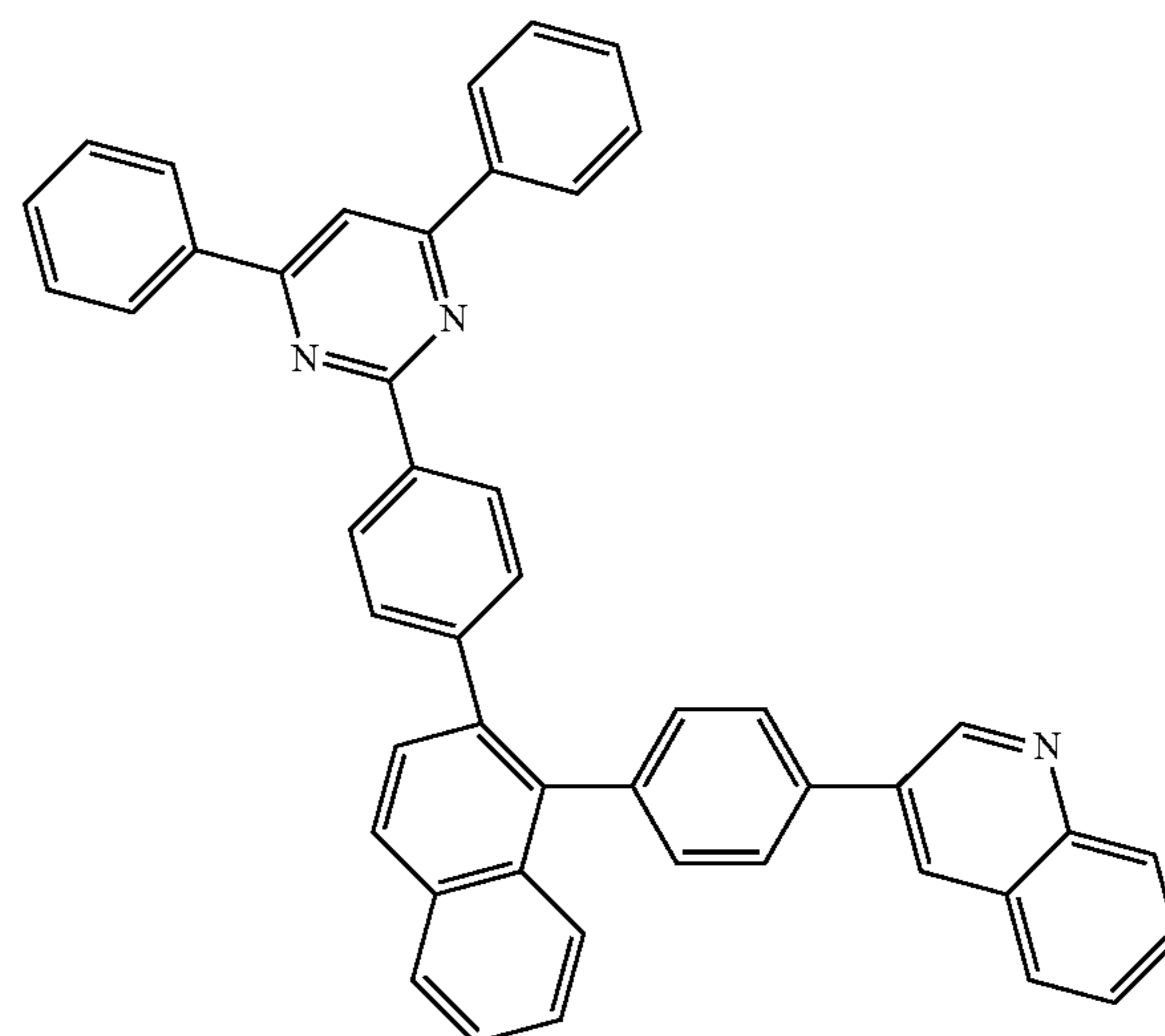
[formula 3-11-6]
