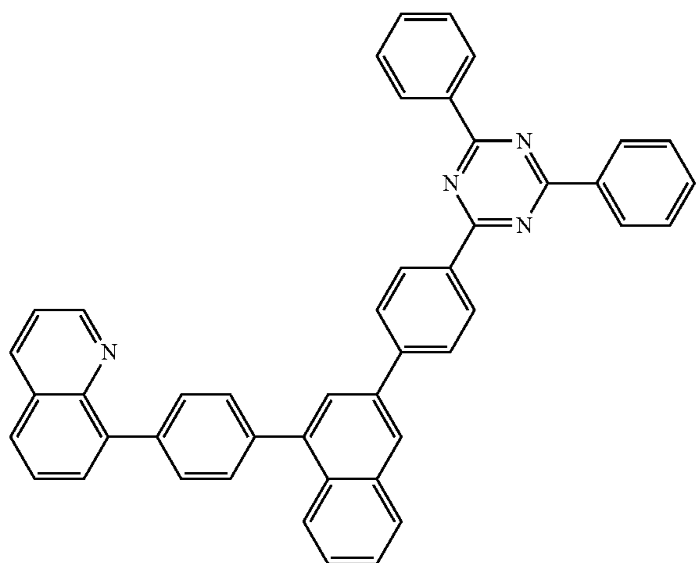
[formula 3-10-1]
