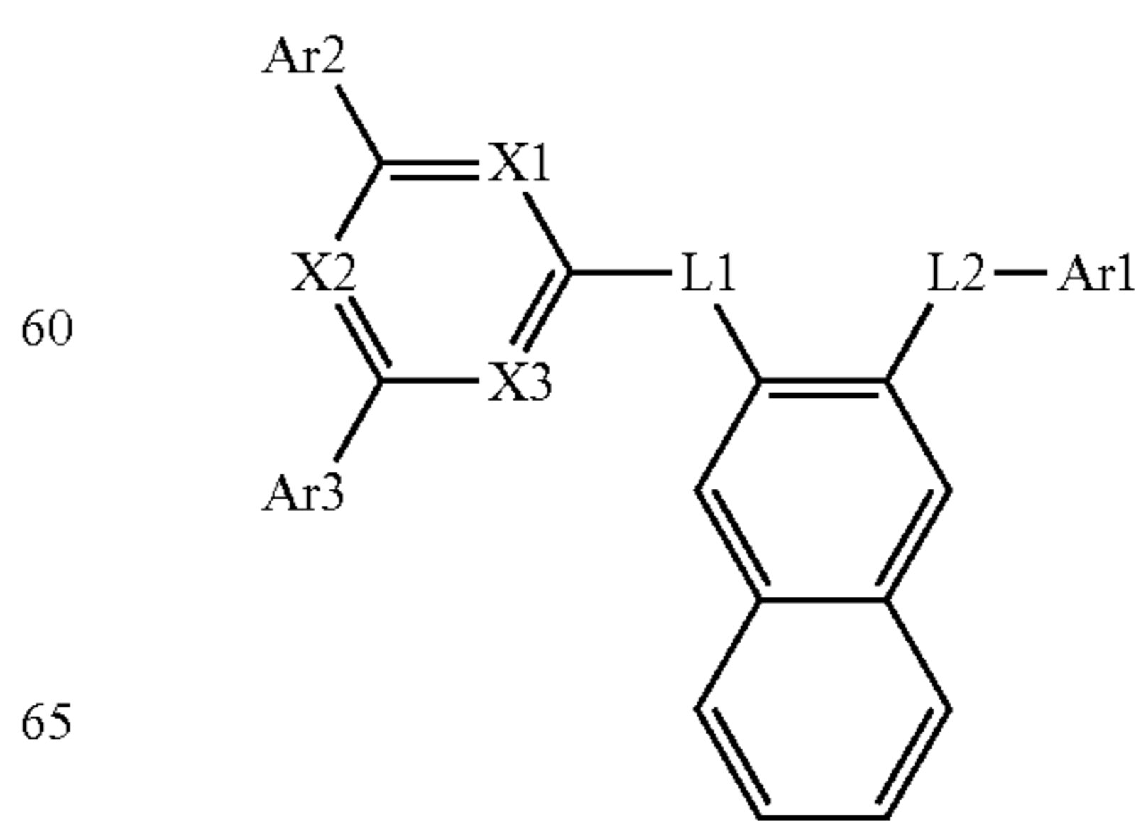
[Chemical Formula 1-4]
