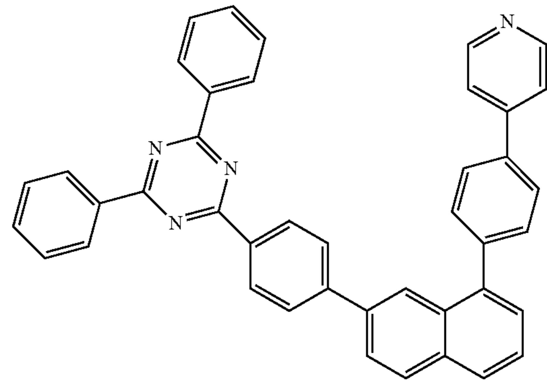
[formula 2-2-4]
