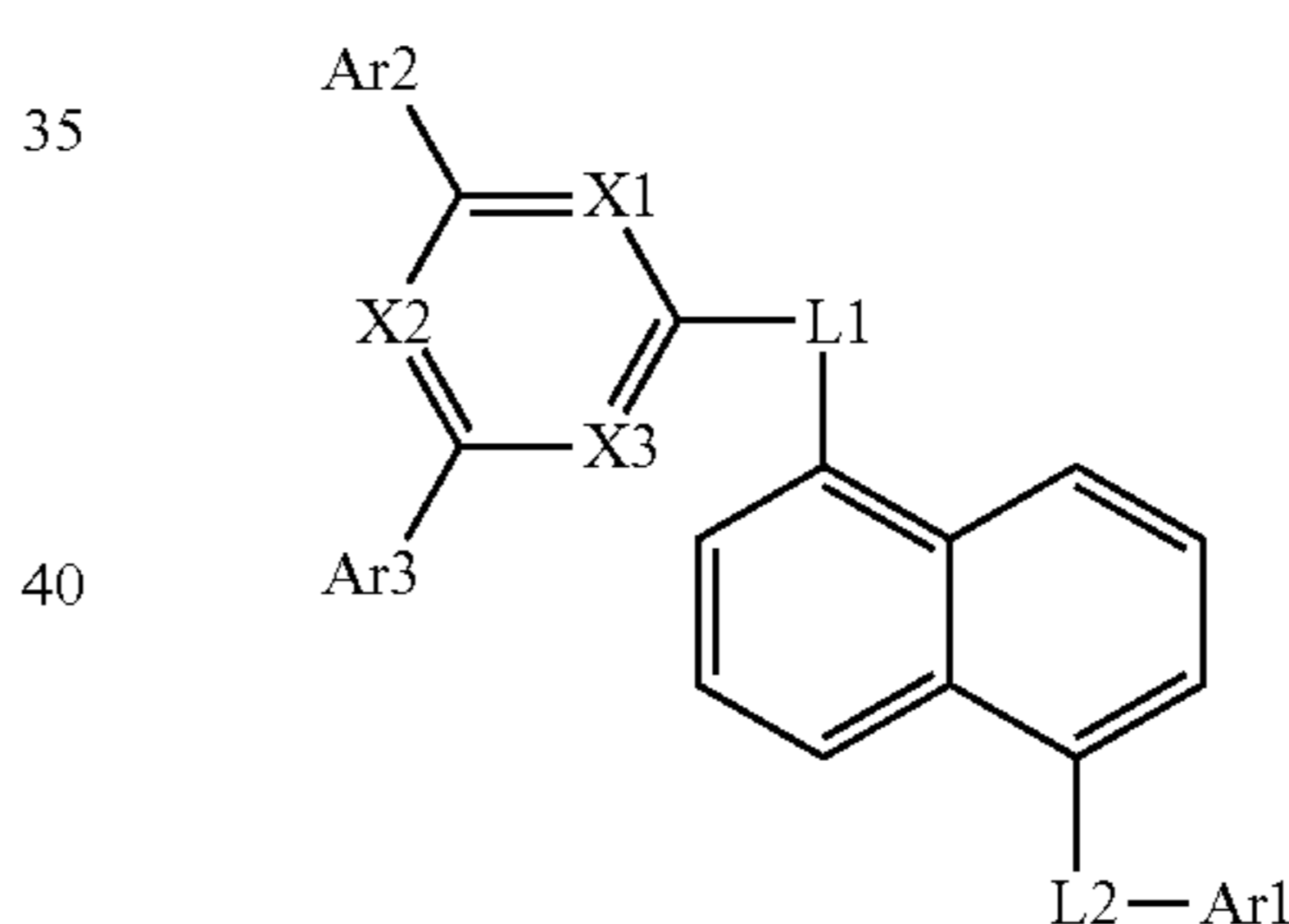
[Chemical Formula 1-2]
