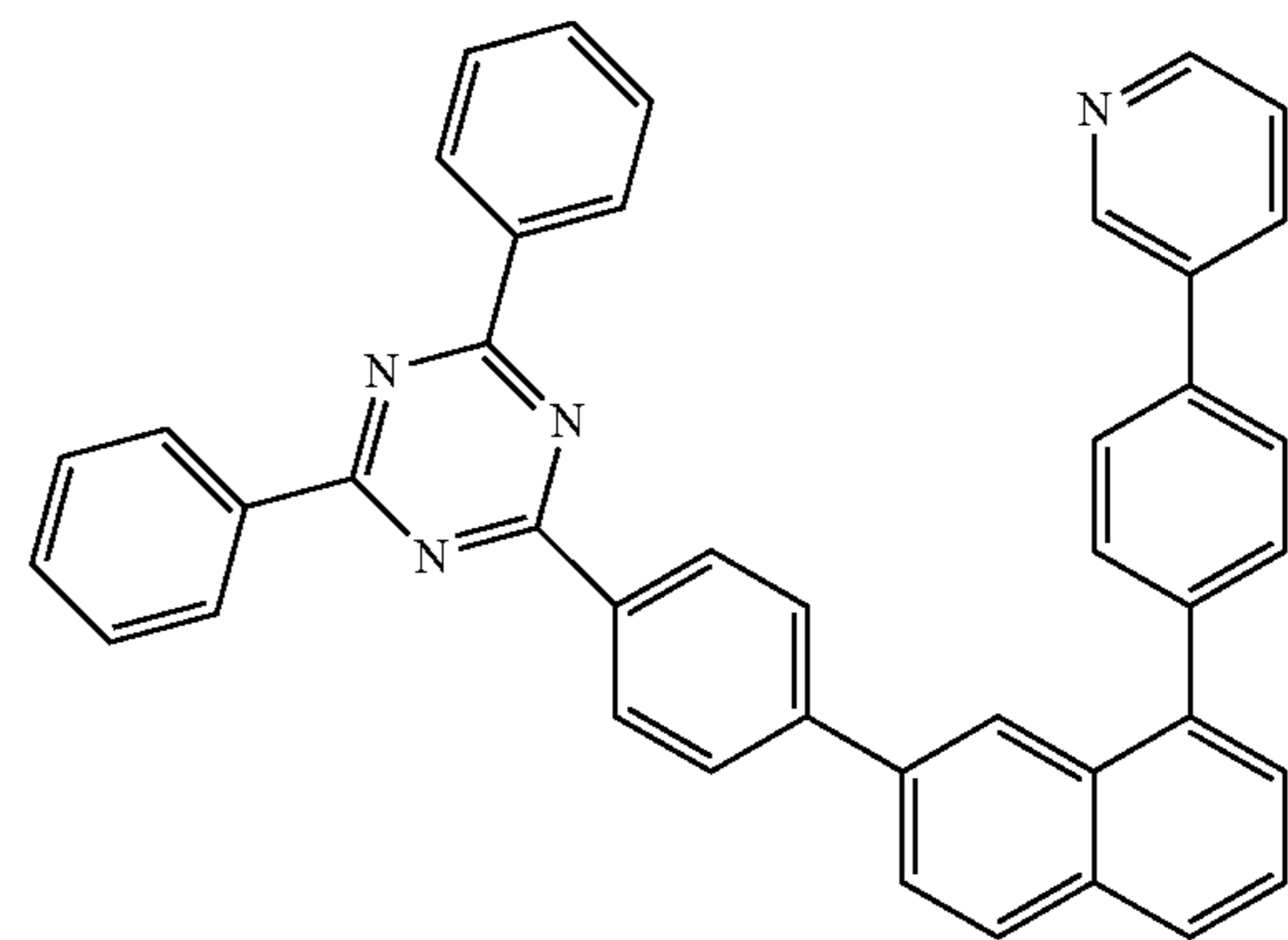
[formula 2-2-5]
