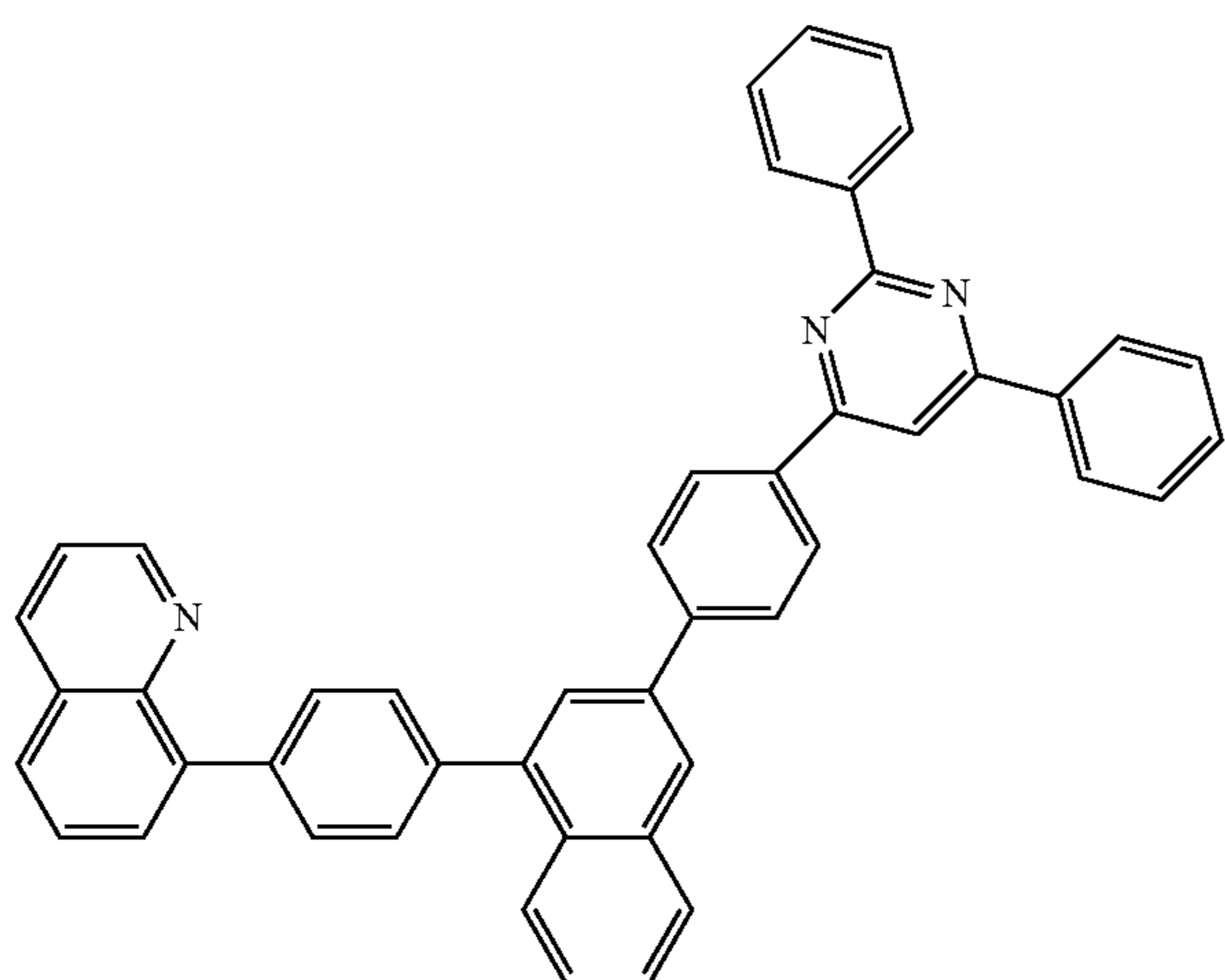
[formula 3-10-3]
