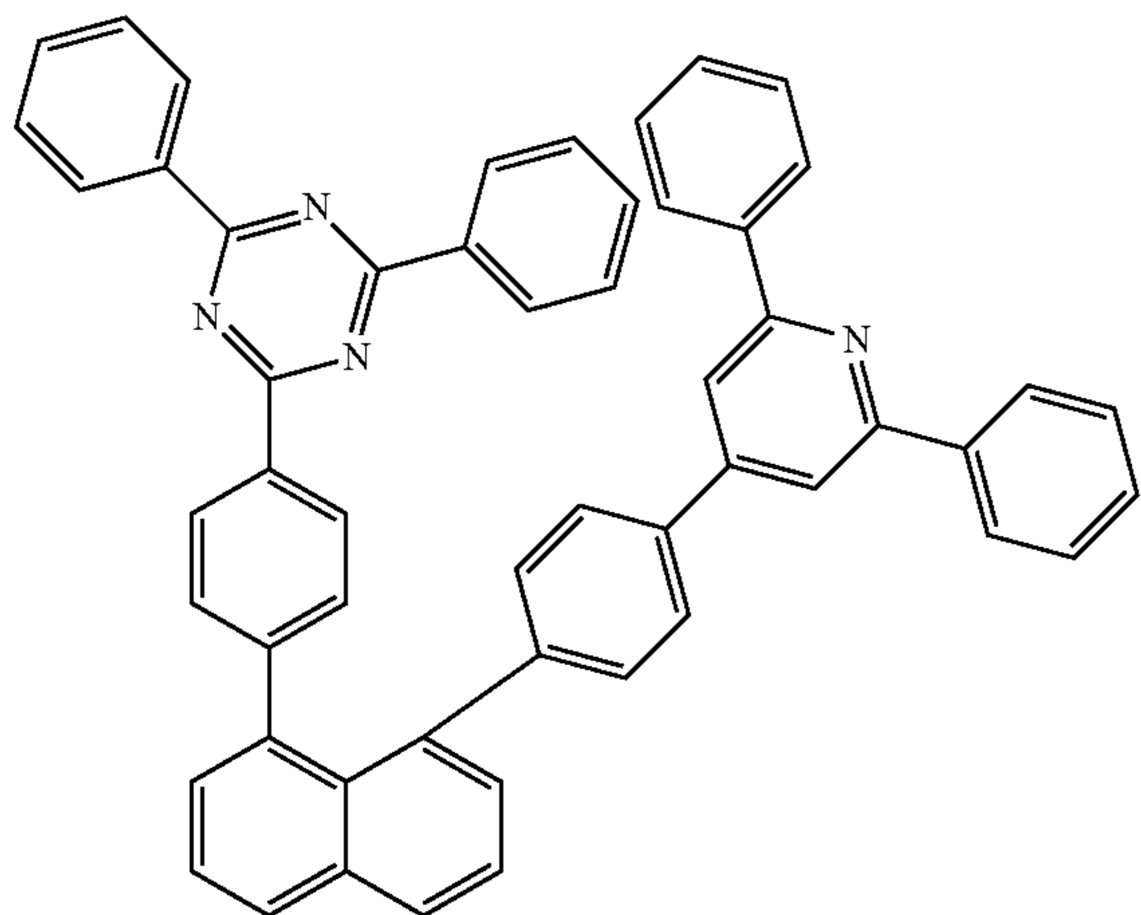
[formula 2-5-3]
