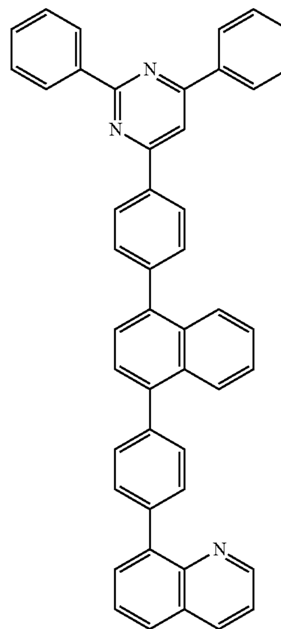
[Chemical Formula 3-12-3]
