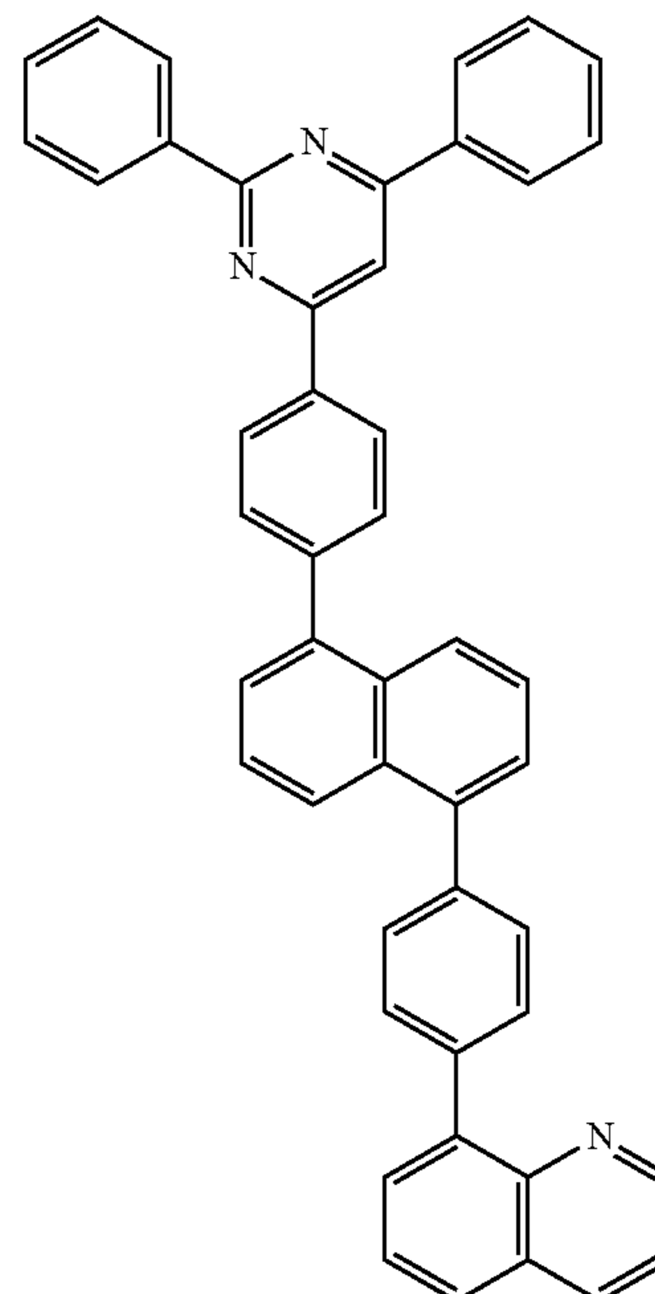
[Chemical Formula 3-8-3]
