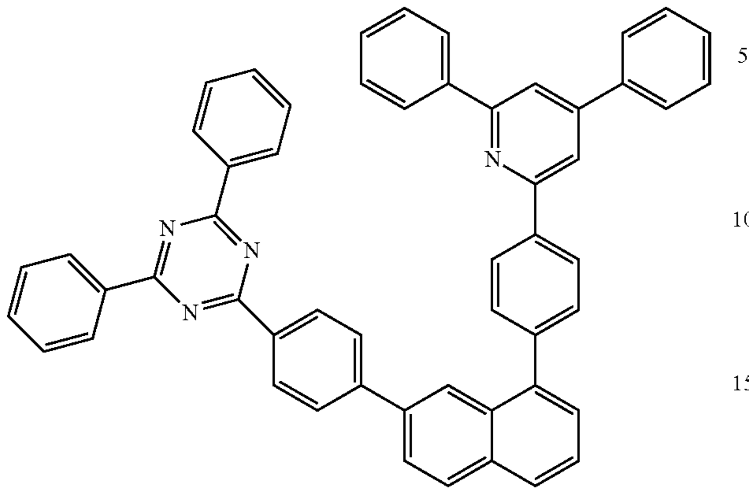
[formula 2-2-1]
