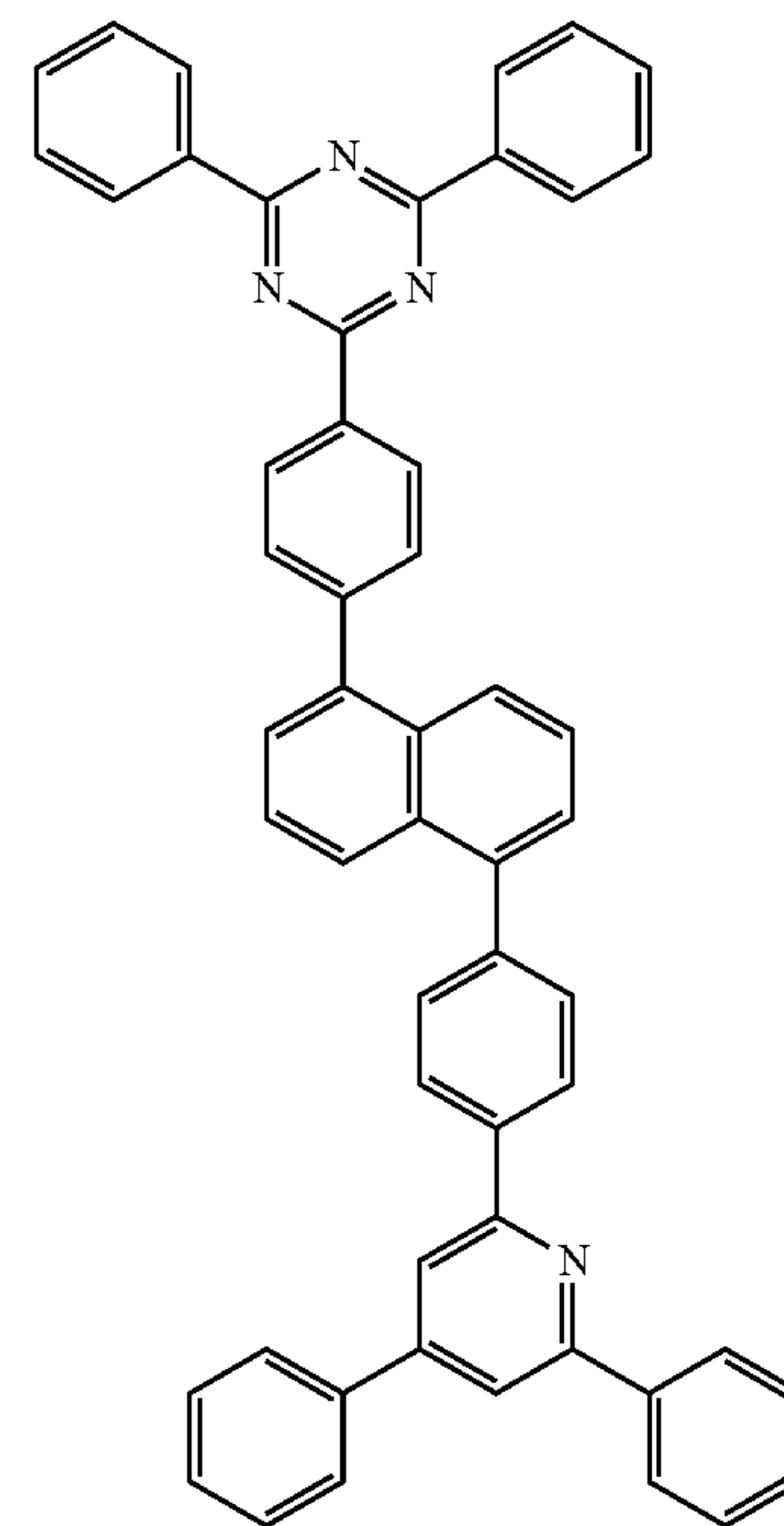
[Chemical Formula 2-8-1]
