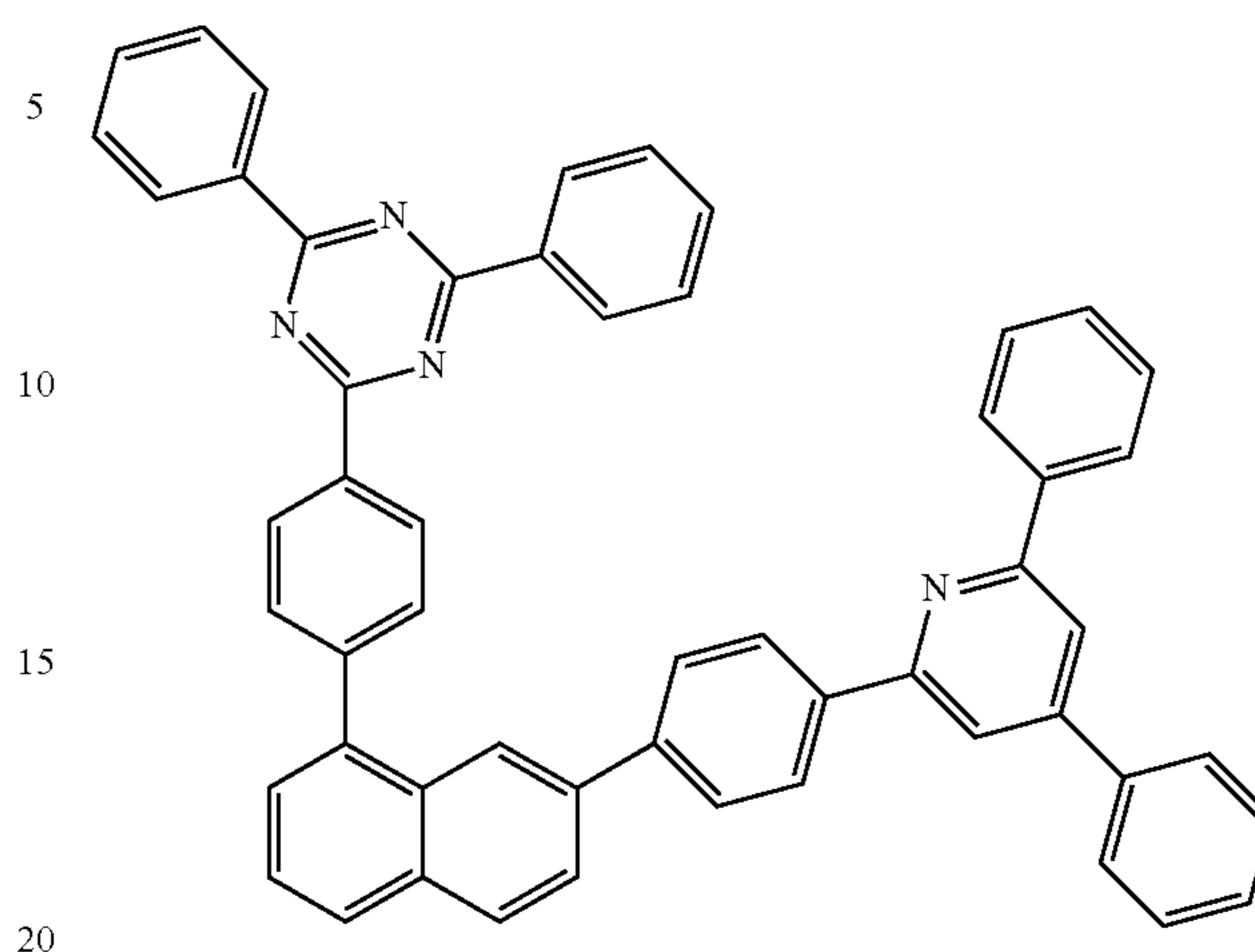
[formula 2-6-1]
