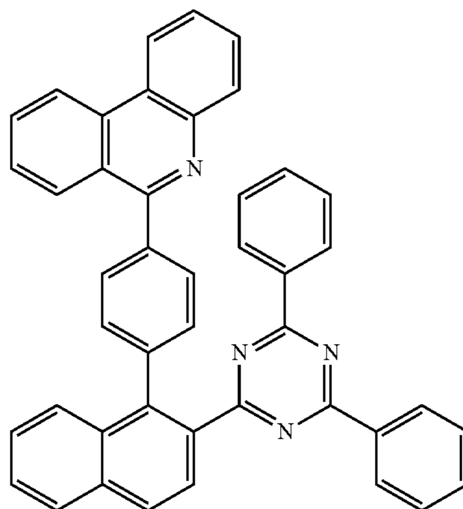
[Chemical Formula 6-11-1]
