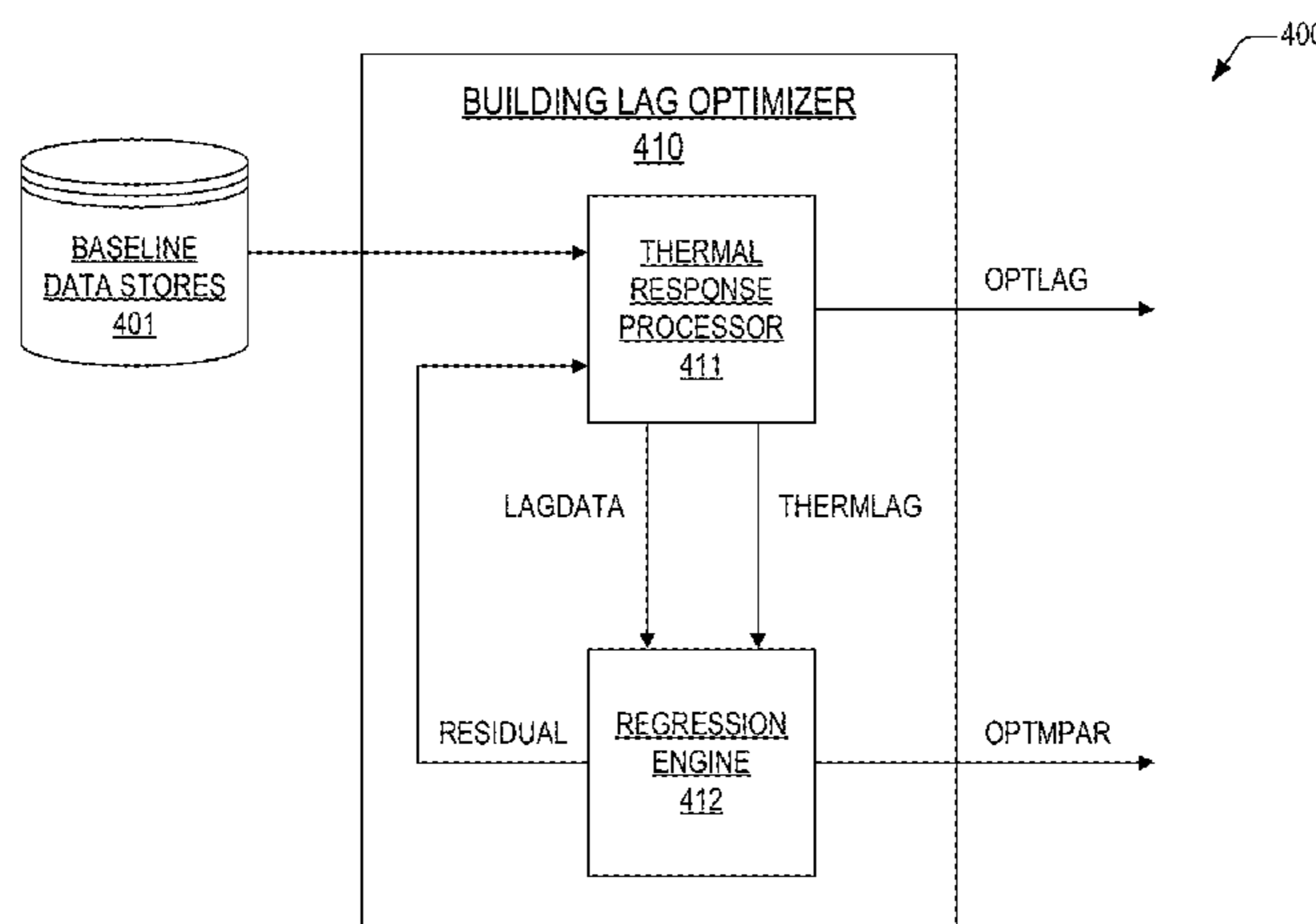
FINE-GRAINED BASELINE ENERGY DATA WEATHER NORMALIZATION APPARATUS
