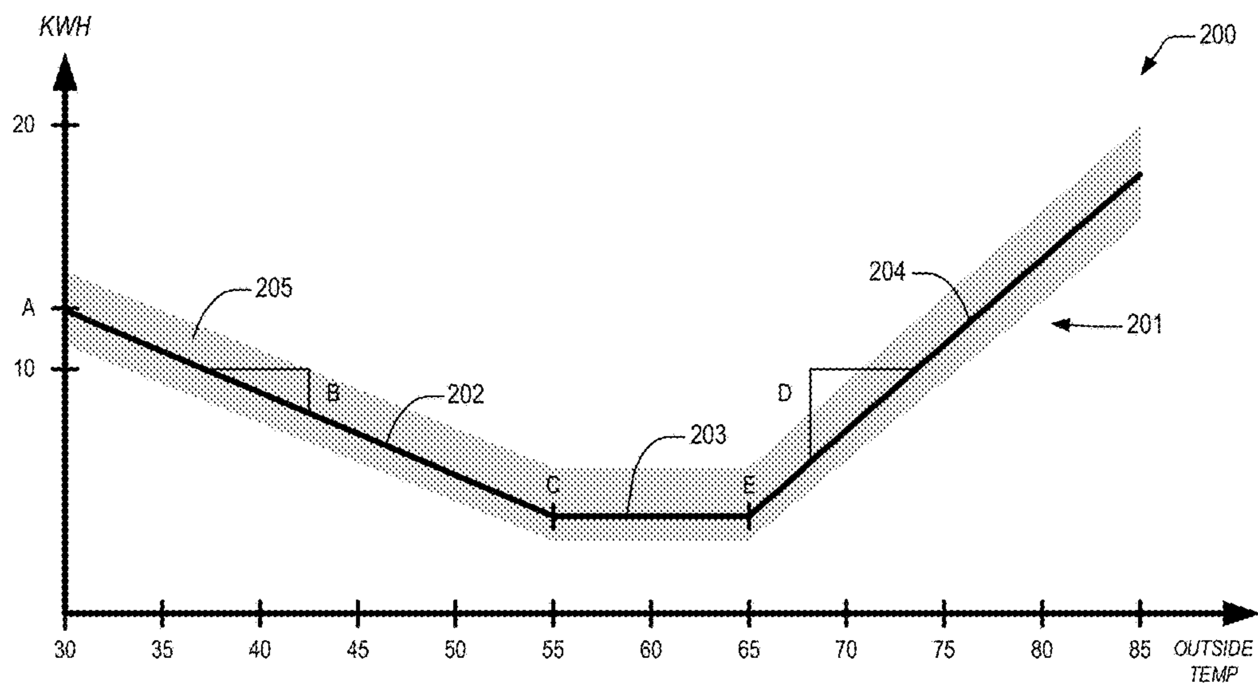
COARSE-GRAINED 5-PARAMETER REGRESSION BASELINE MODEL
