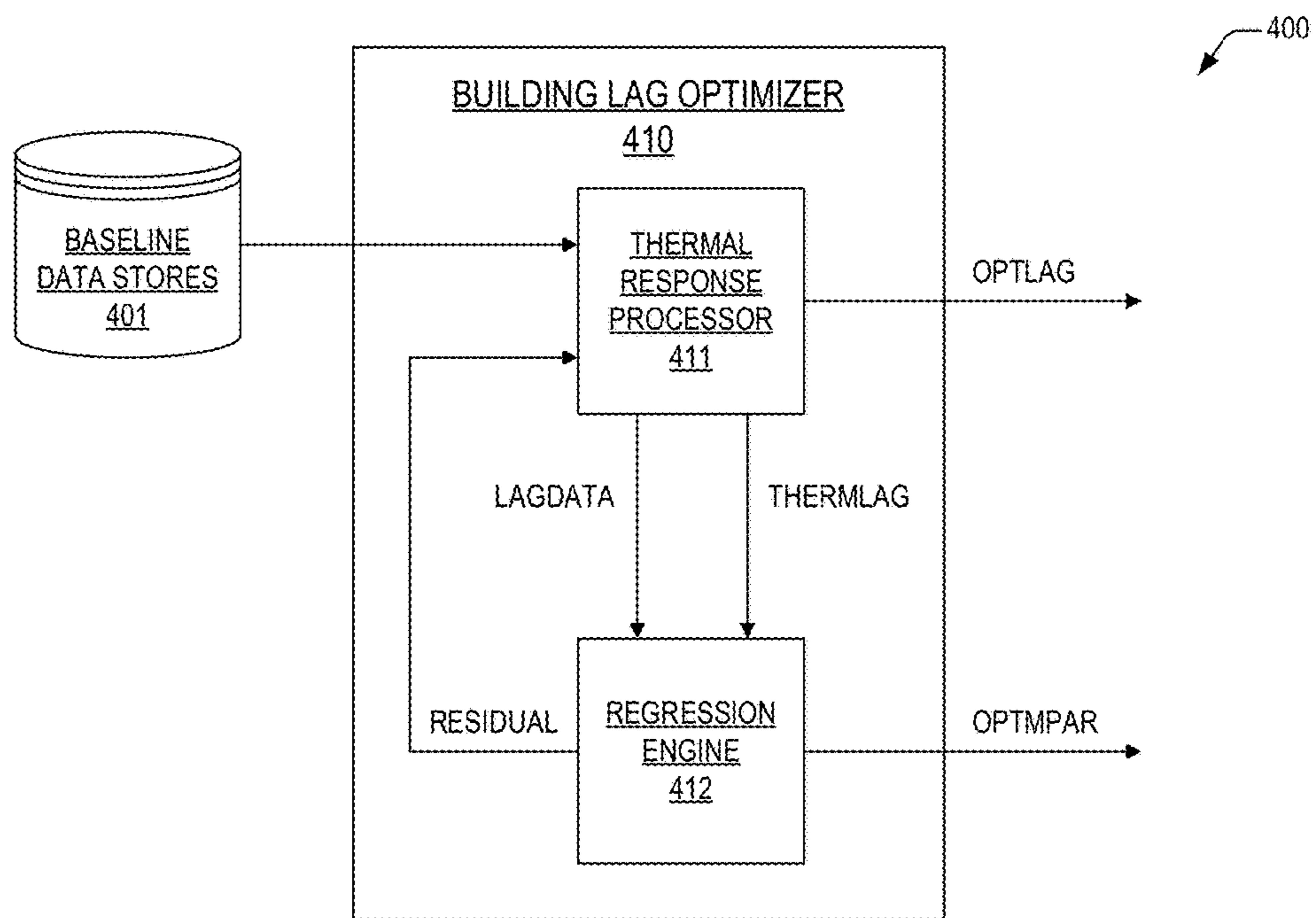
FIG. 4 FINE-GRAINED BASELINE ENERGY DATA WEATHER NORMALIZATION APPARATUS
