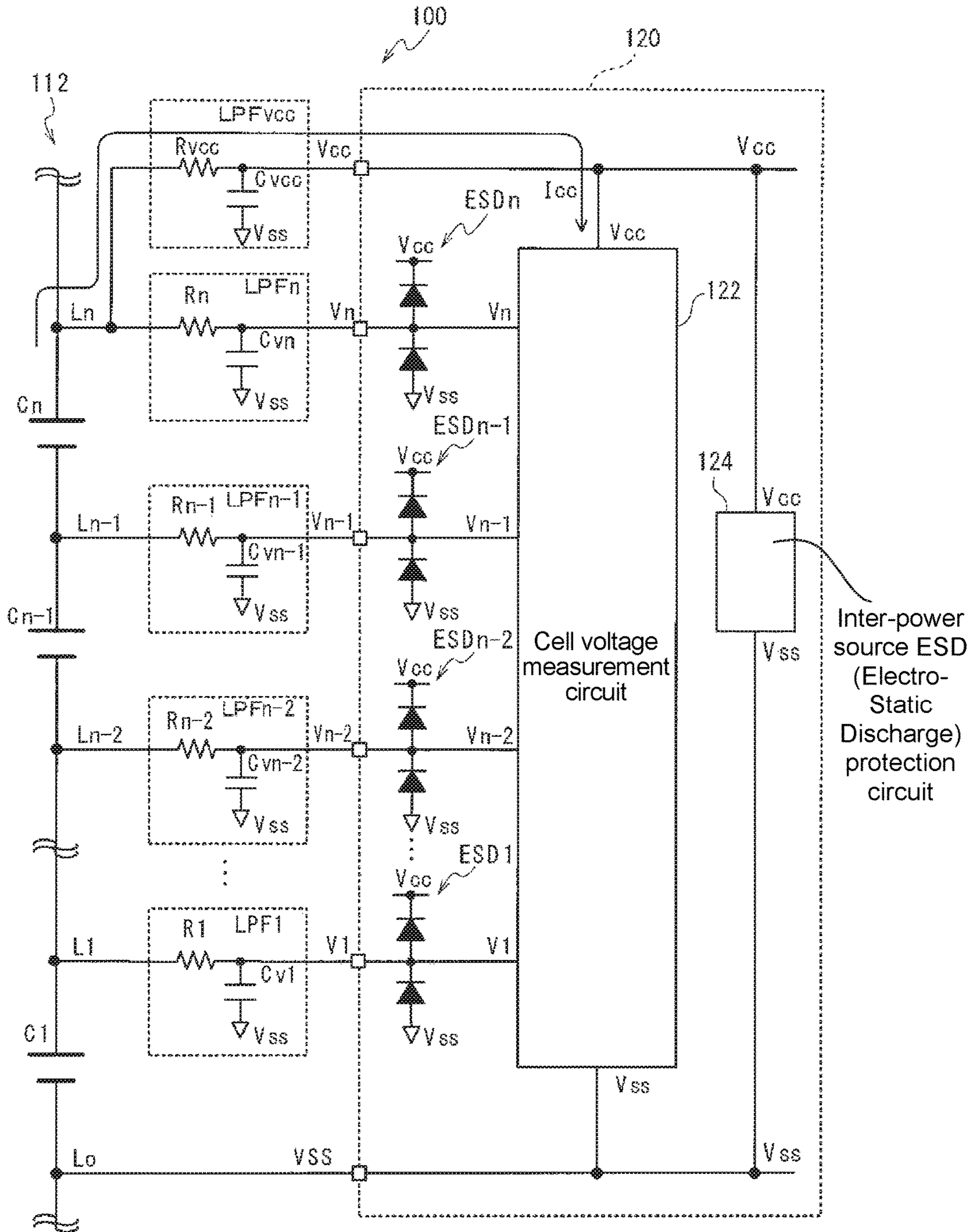
FIG. 5 PRIOR ART
