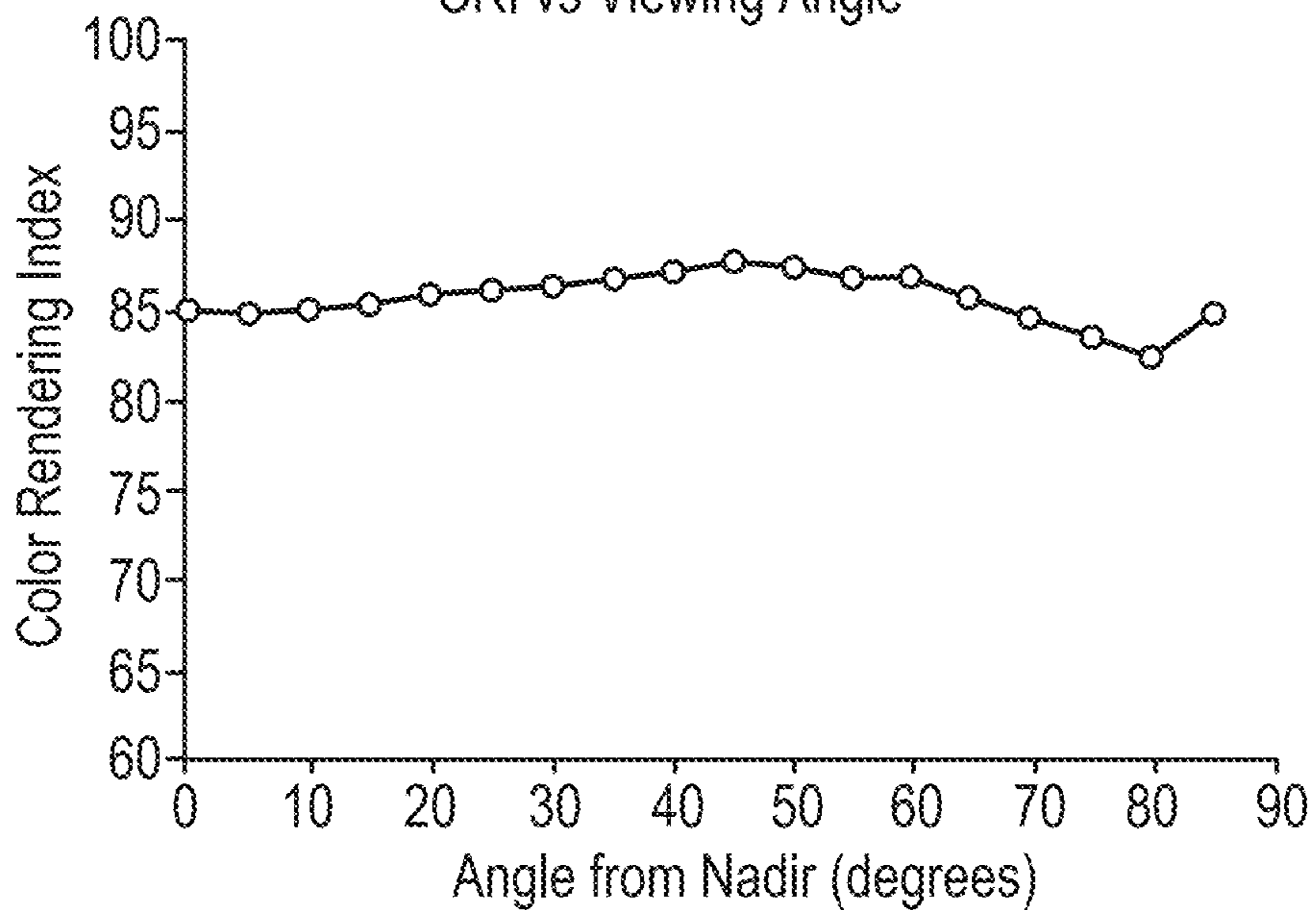
CRI vs Viewing Angle
