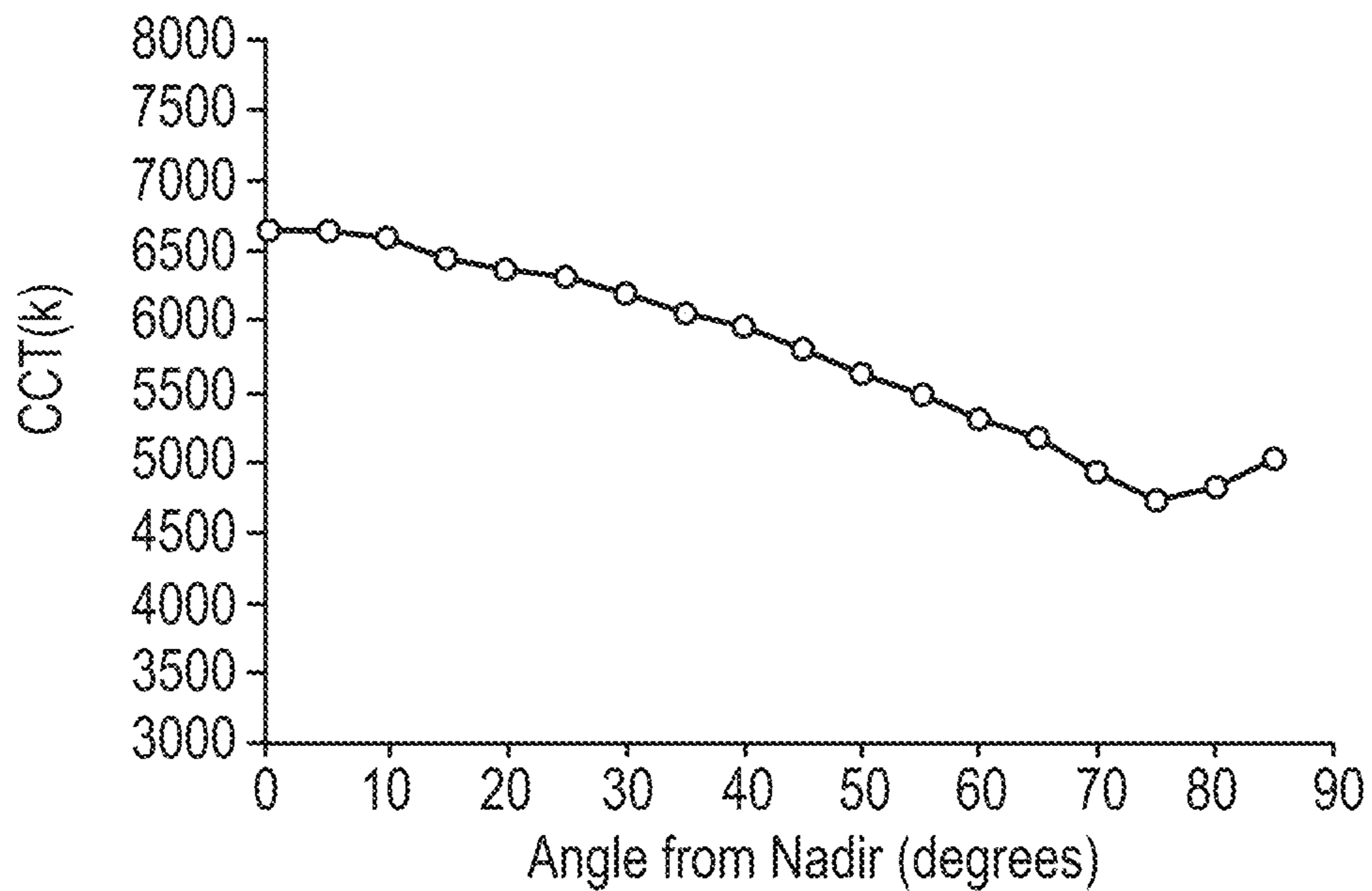
CCT vs Viewing Angle
