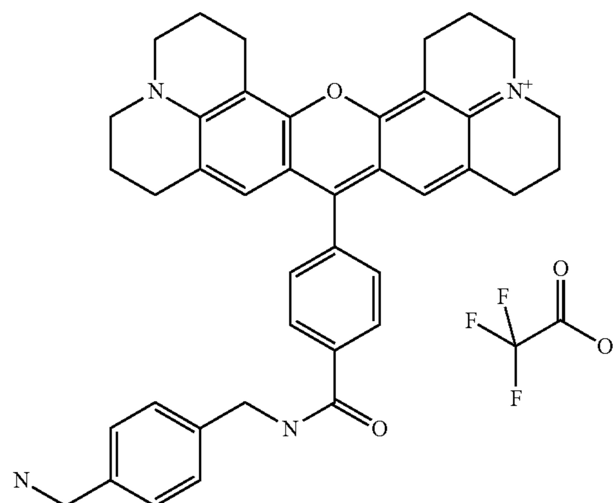
Compound 7
