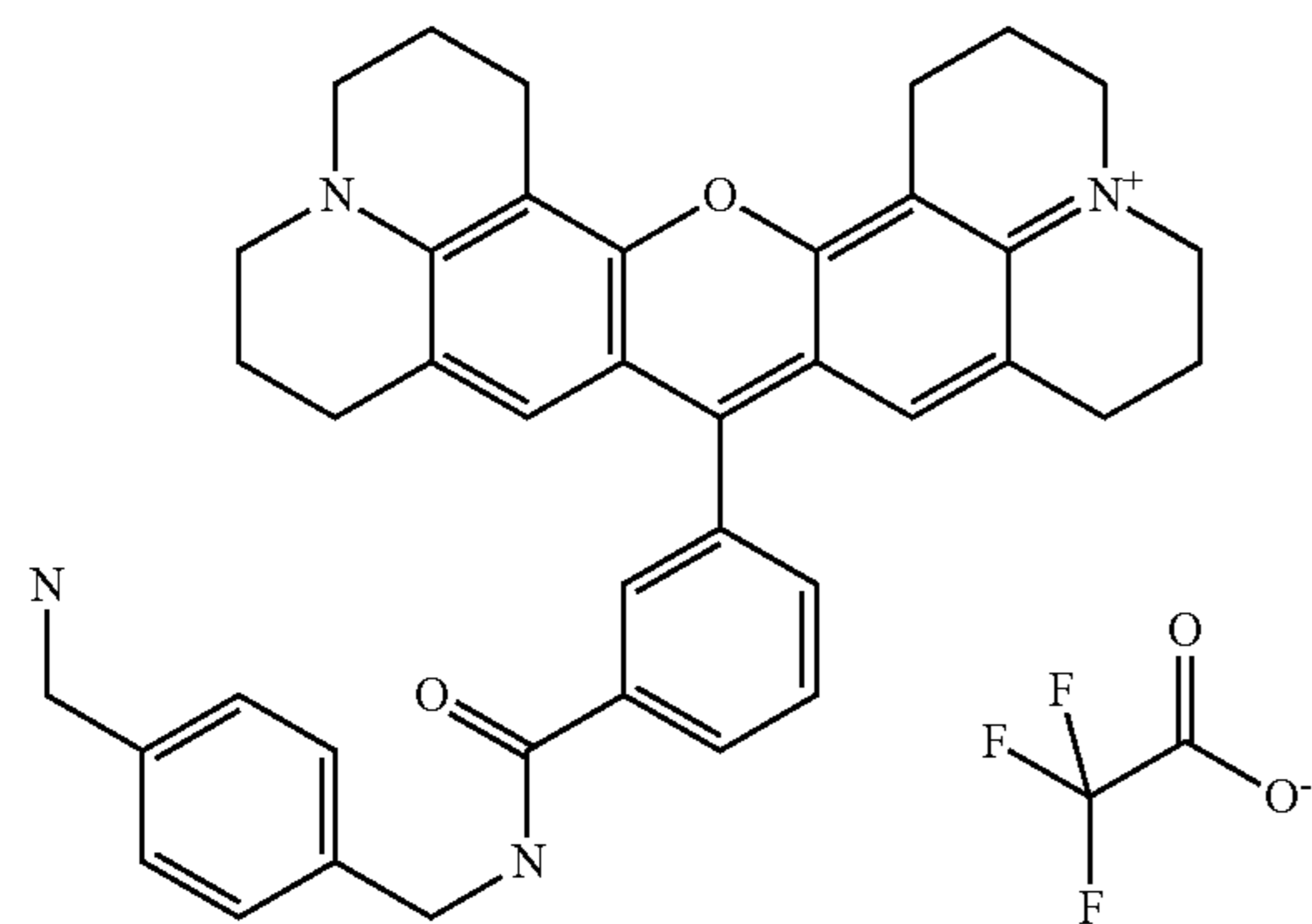
Compound 12
