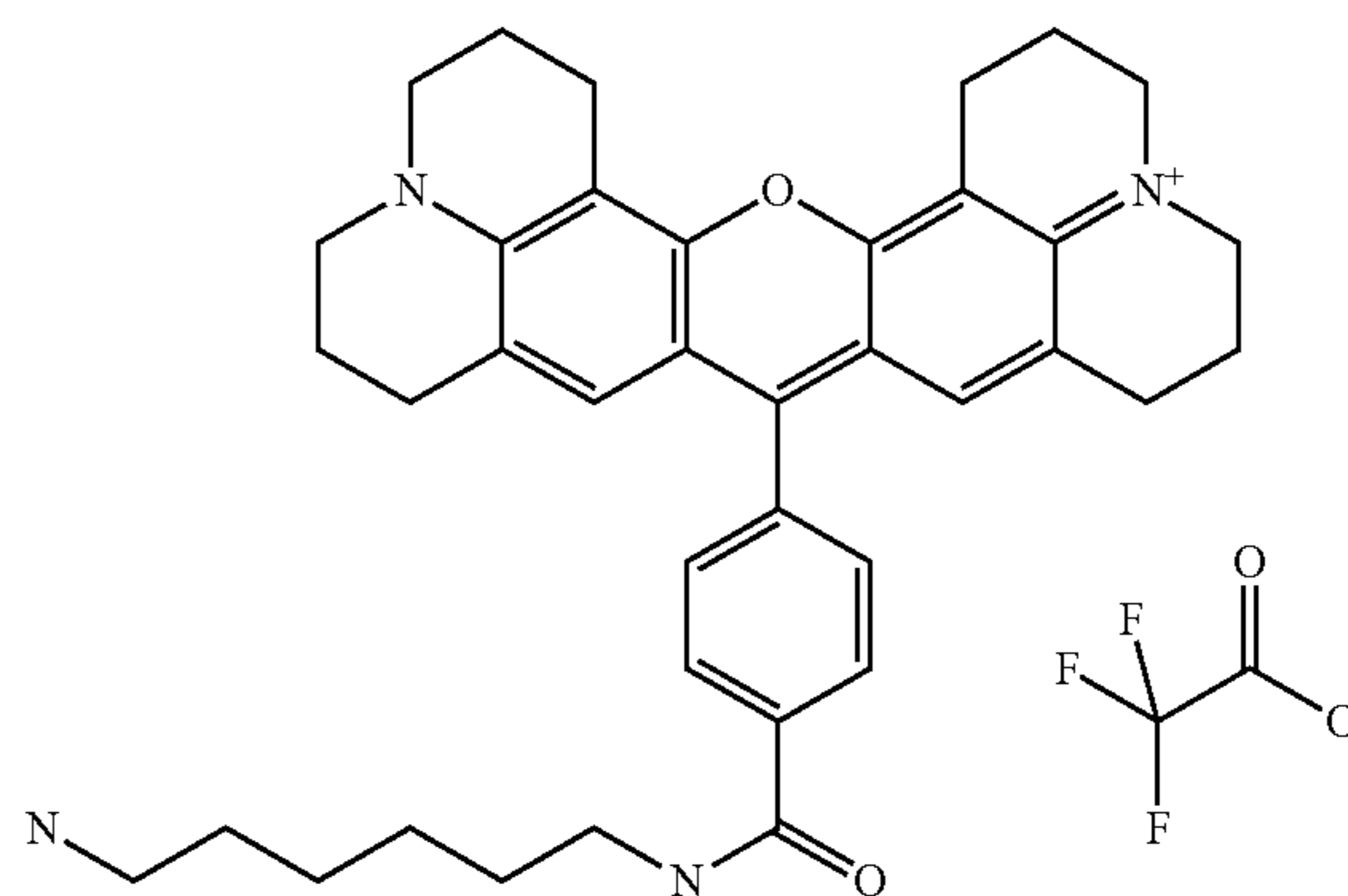
Compound 6
