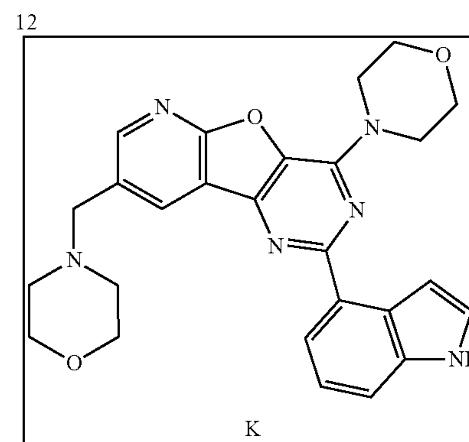
i. 2-Chloro-4-morpholin-4-yl-8-morpholin-4-ylmethyl-pyrido[3',2':4,5]furo[3,2-d]pyrimidine, 12
