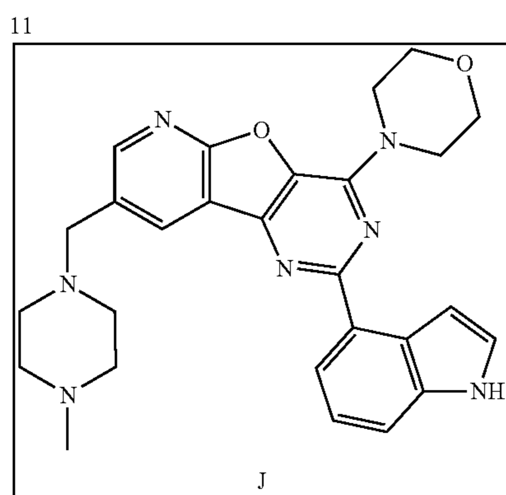
i. 2-Chloro-8-(4-methyl-piperazin-1-ylmethyl)-4-morpholin-4-yl-pyrido[3',2':4,5]furo[3,2-d]pyrimidine, 11
