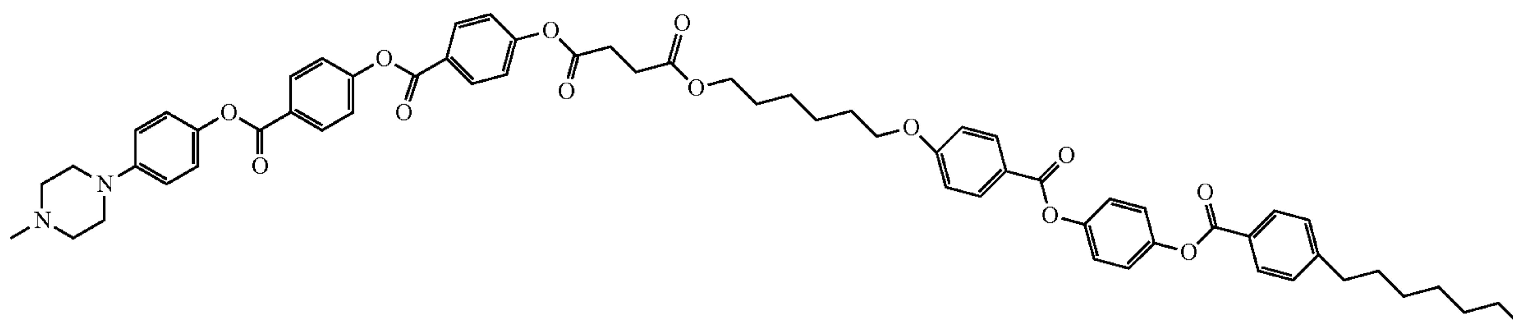
4-[4-(4-(4-[3-(6-(4[4-(4-nonyl-benzoyloxy)-phenoxy]-phenoxy)-hexyloxy)-propionyl]-benzoyloxy)-benzoyloxy)-phenyl]-piperazin-1-yl
