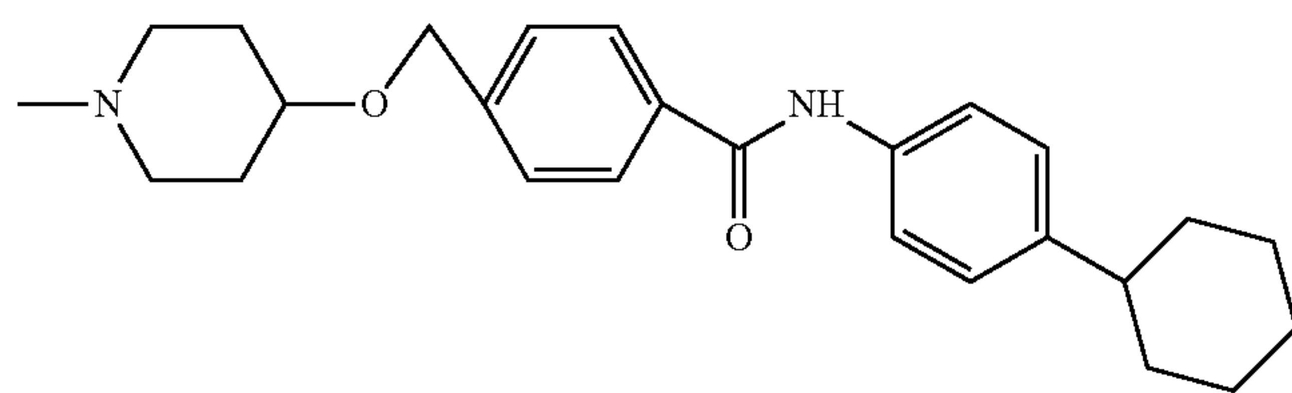
4-[4-(4-cyclohexyl-phenylcarbamoyl)-benzyloxy]-piperidin-1-yl
