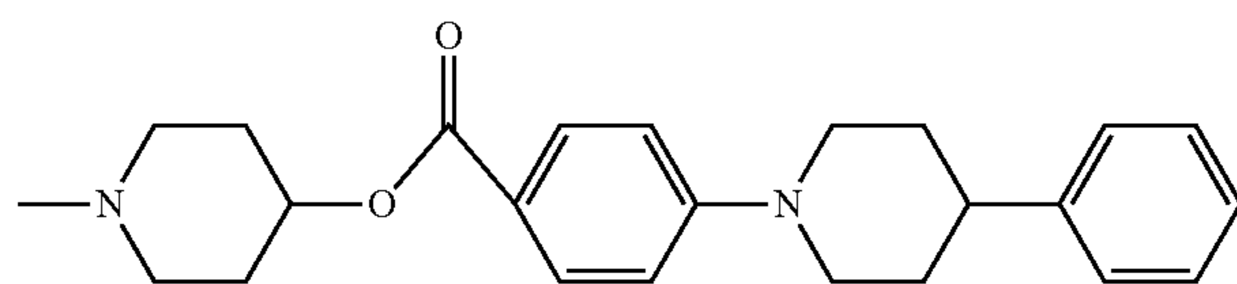
4-(4-(4-phenylpiperidin-1-yl)-benzoyloxy)-piperidin-1-yl
