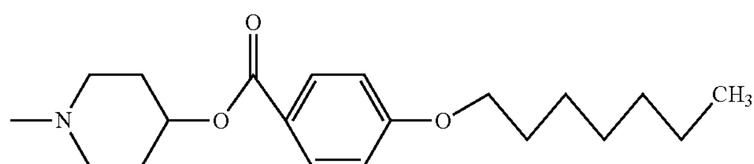
4-(4-hexyloxy-benzoyloxy)-piperidin-1-yl
