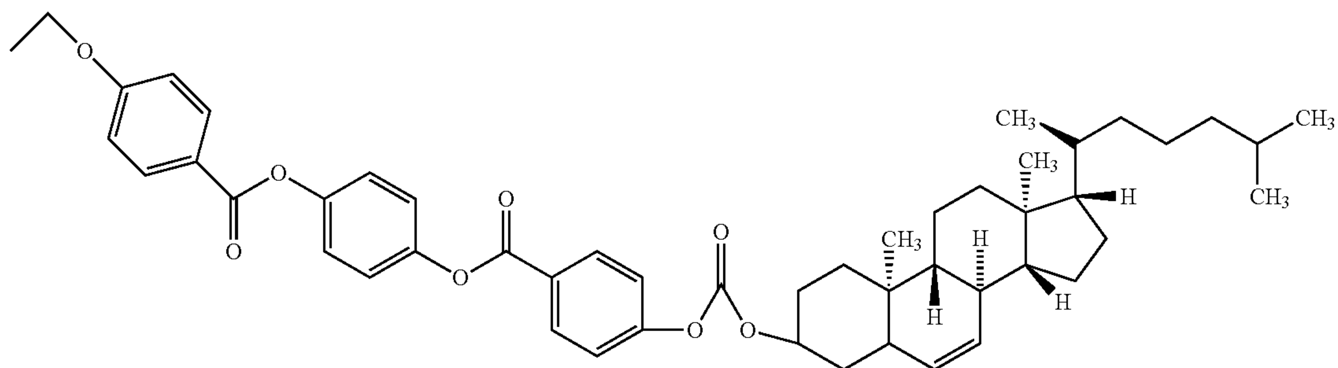
4-(4-(4-[17-(1,5-dimethyl-hexyl)-10,13-dimethyl-2,3,4,7,8,9,10,11,12,13,14,15,16,17-tetradecahydro-1H-cyclopenta[a]phenanthren-3-yloxy-carbonyloxy]-benzoyloxy)-phenoxycarbonyl)-phenoxy-methyl
