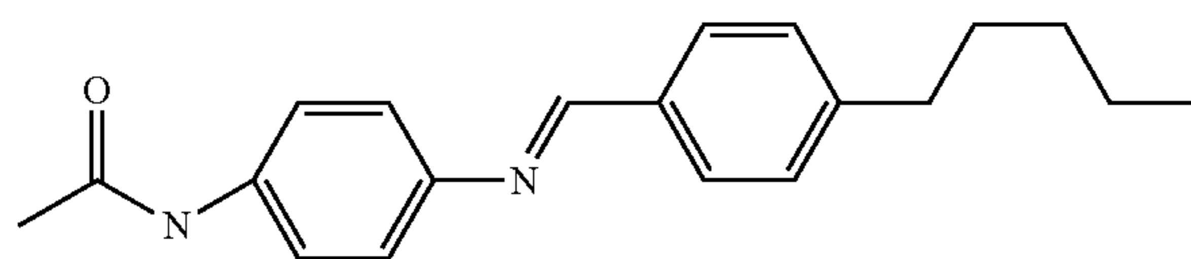
N-{4-[(4-pentyl-benzylidene)-amino]-phenyl}-acetamidyl
