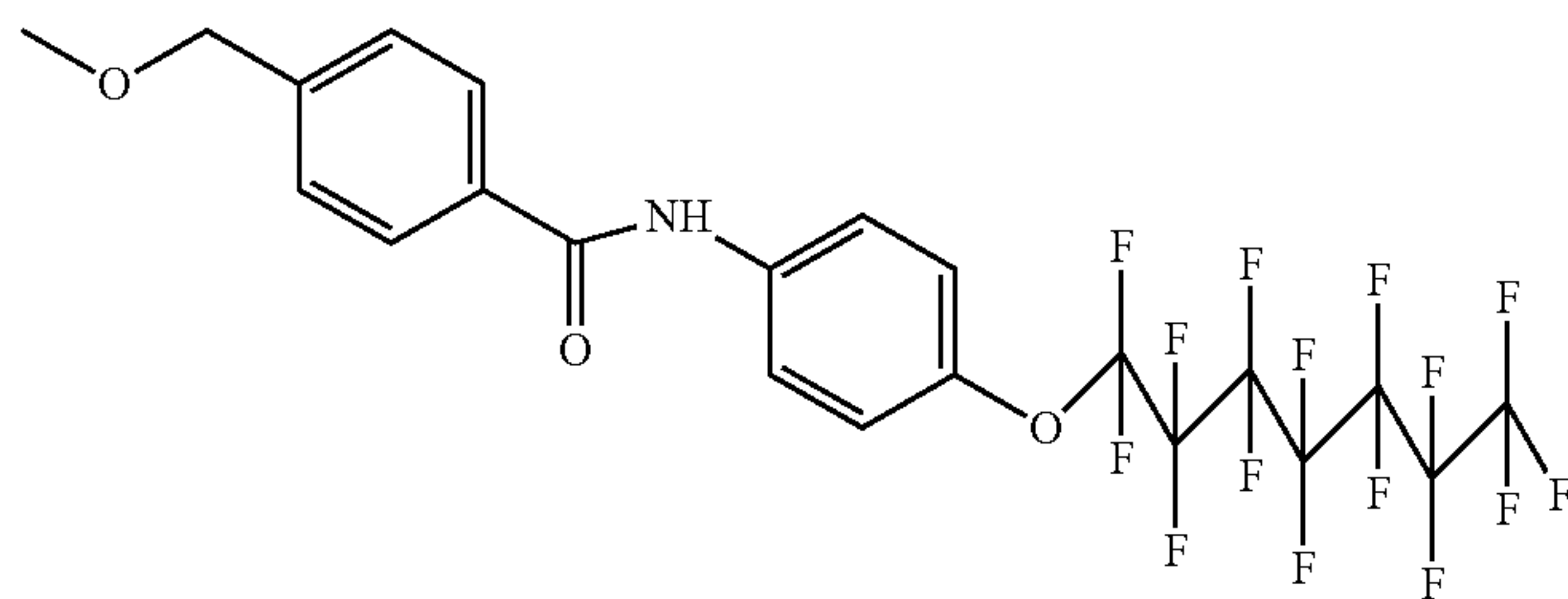
4-(4-pentadecafluoroheptyloxy-phenylcarbamoyl)-benzyloxy
