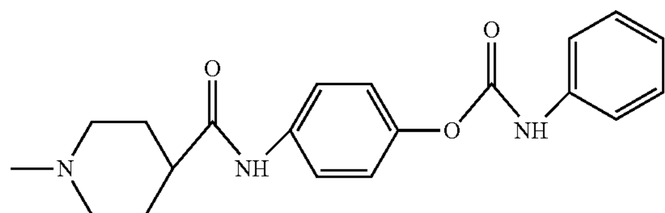
4-(4-phenylcarbamoyl-phenylcarbamoyl)-piperidin-1-yl
