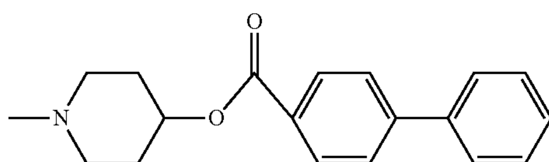
4-(biphenyl-4-carbonyloxy)-piperidin-1-yl
