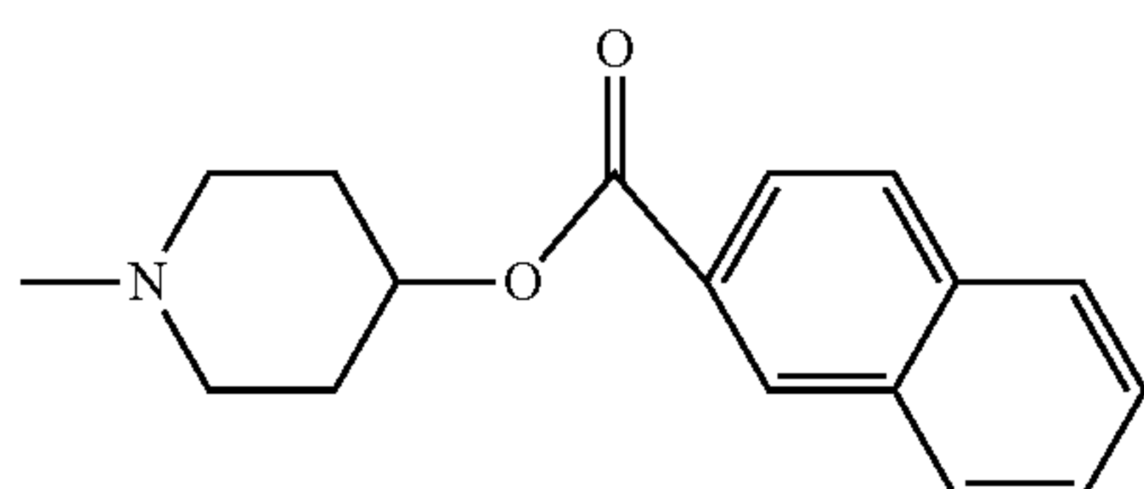
4-(naphthalene-2-carbonyloxy)- piperidin-1-yl
