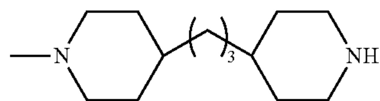
4-(3-piperidin-4-yl-propyl)-piperidin-1-yl
