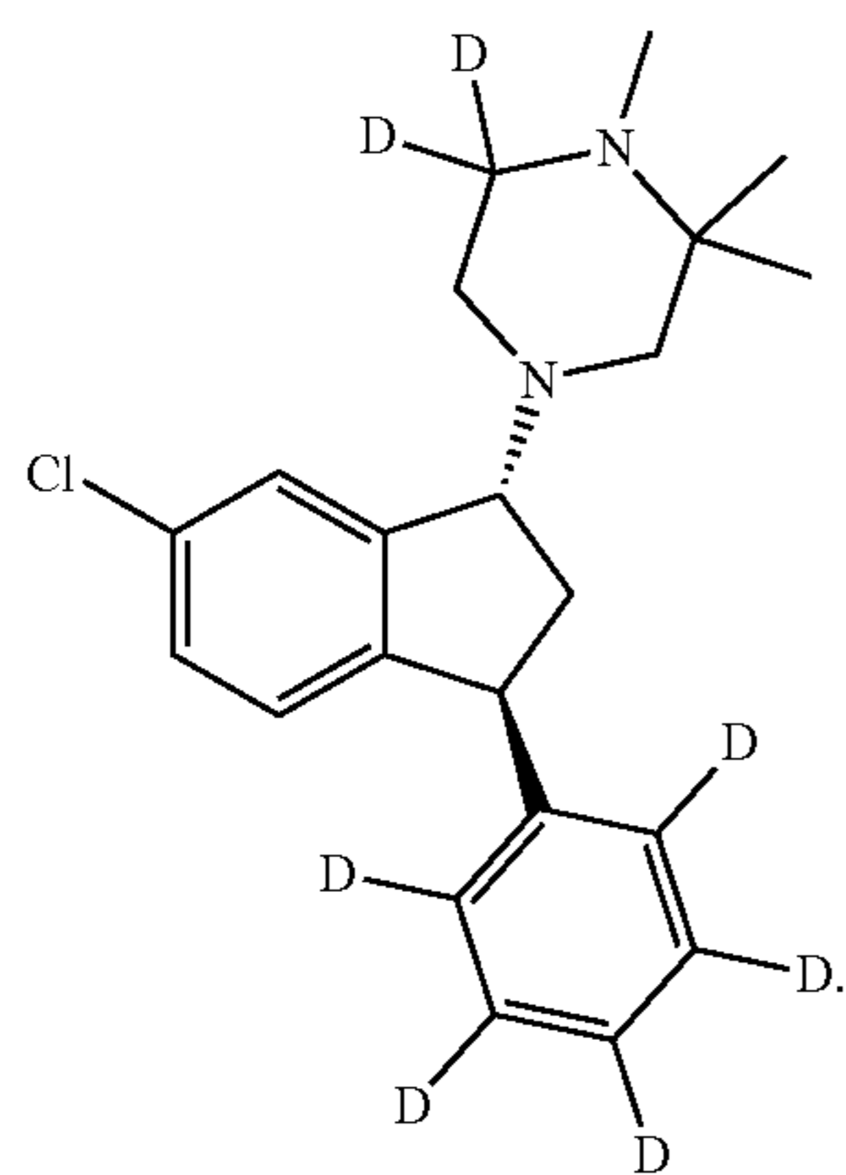
(1R,3S)-(VII)
