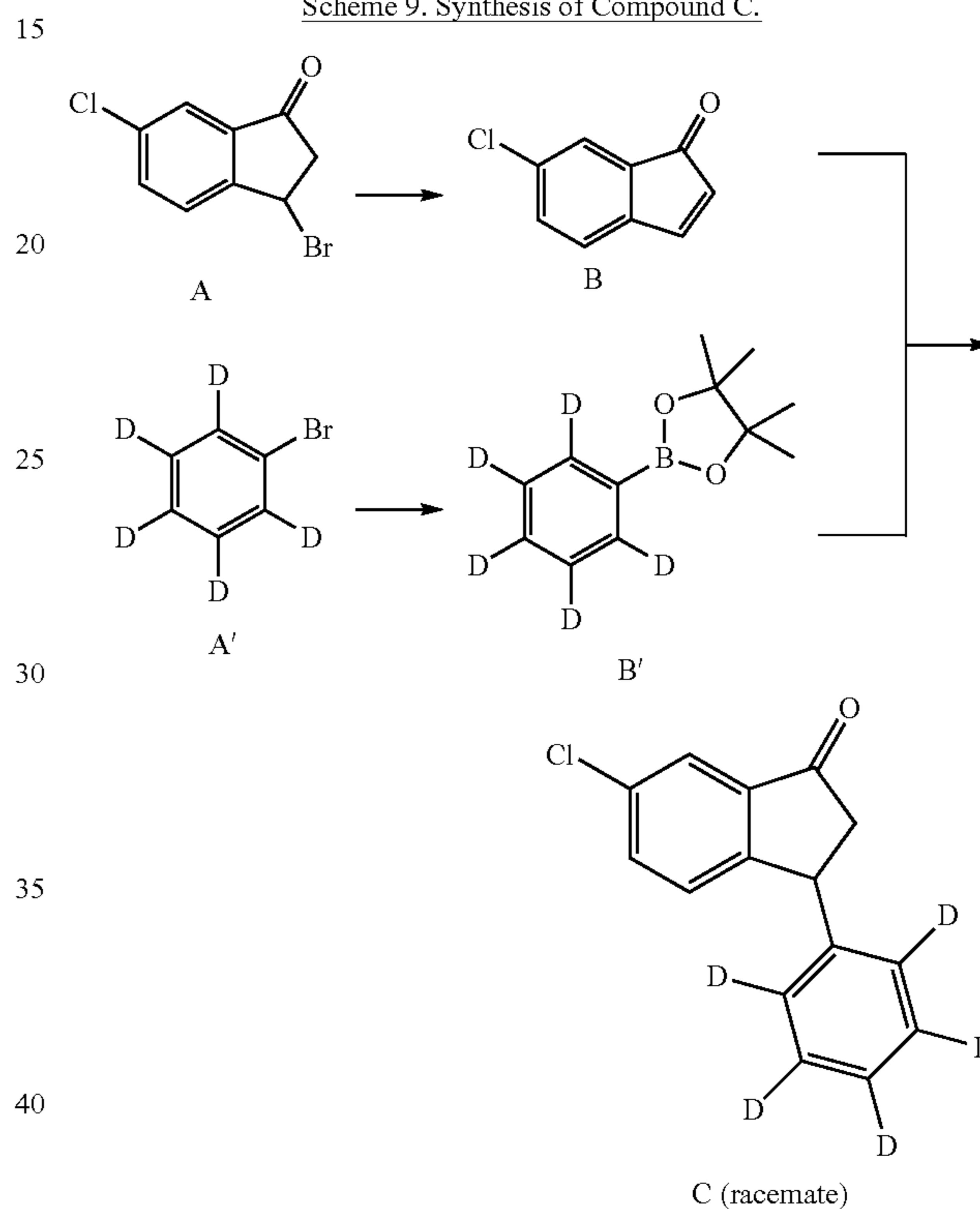
Scheme 9. Synthesis of Compound C.
