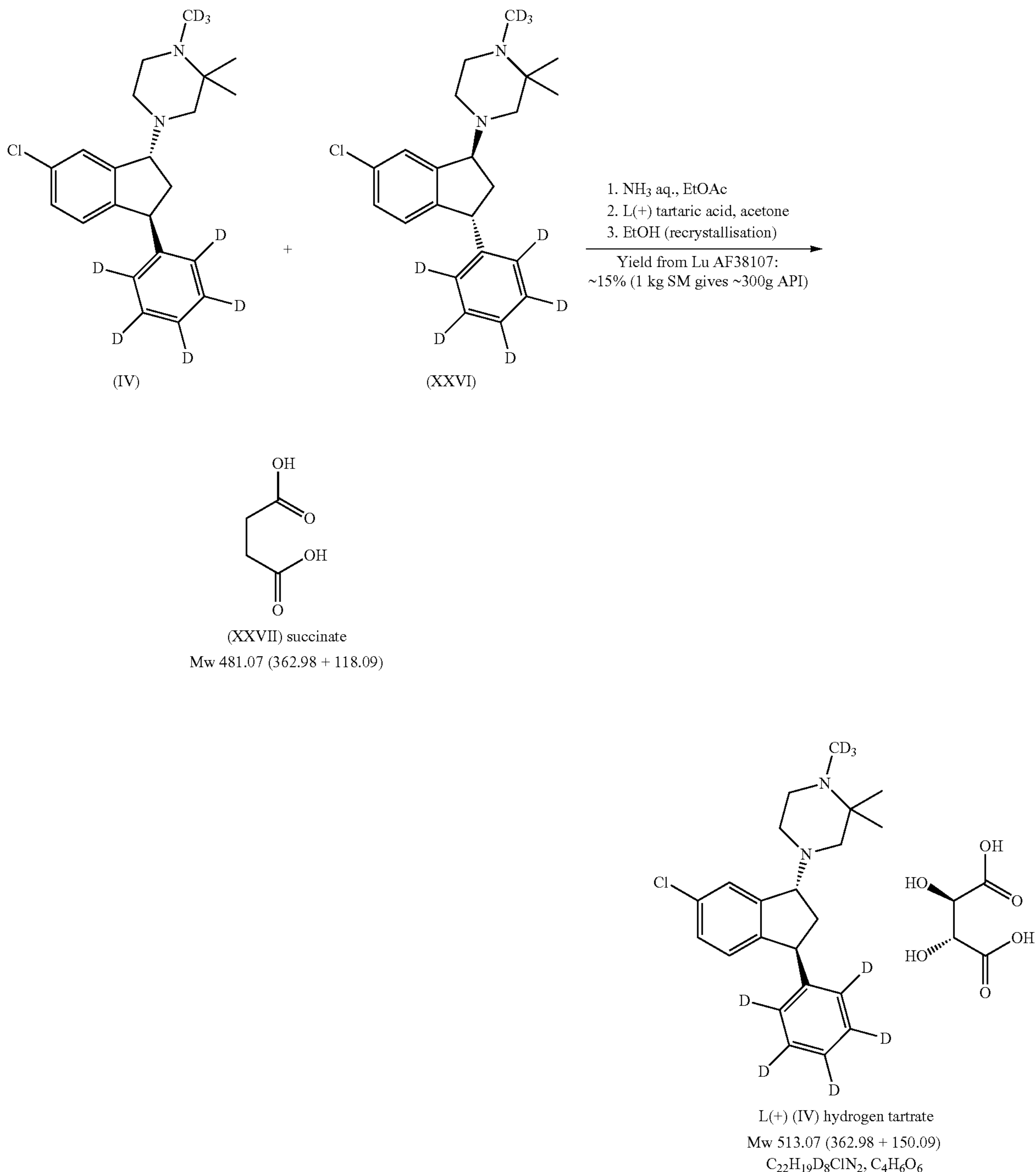
Scheme 18: Synthesis of 4-((1R, 3S)-6-chloro-3-phenyl( d 5 )-indan-1-yl)-1( d 3 ),2,2-trimethyl-piperazine L(+)-hydrogen tartrate.
