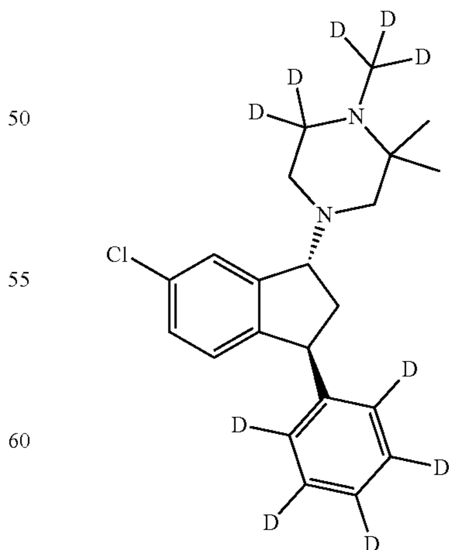
(1R, 3S)-(VI)
