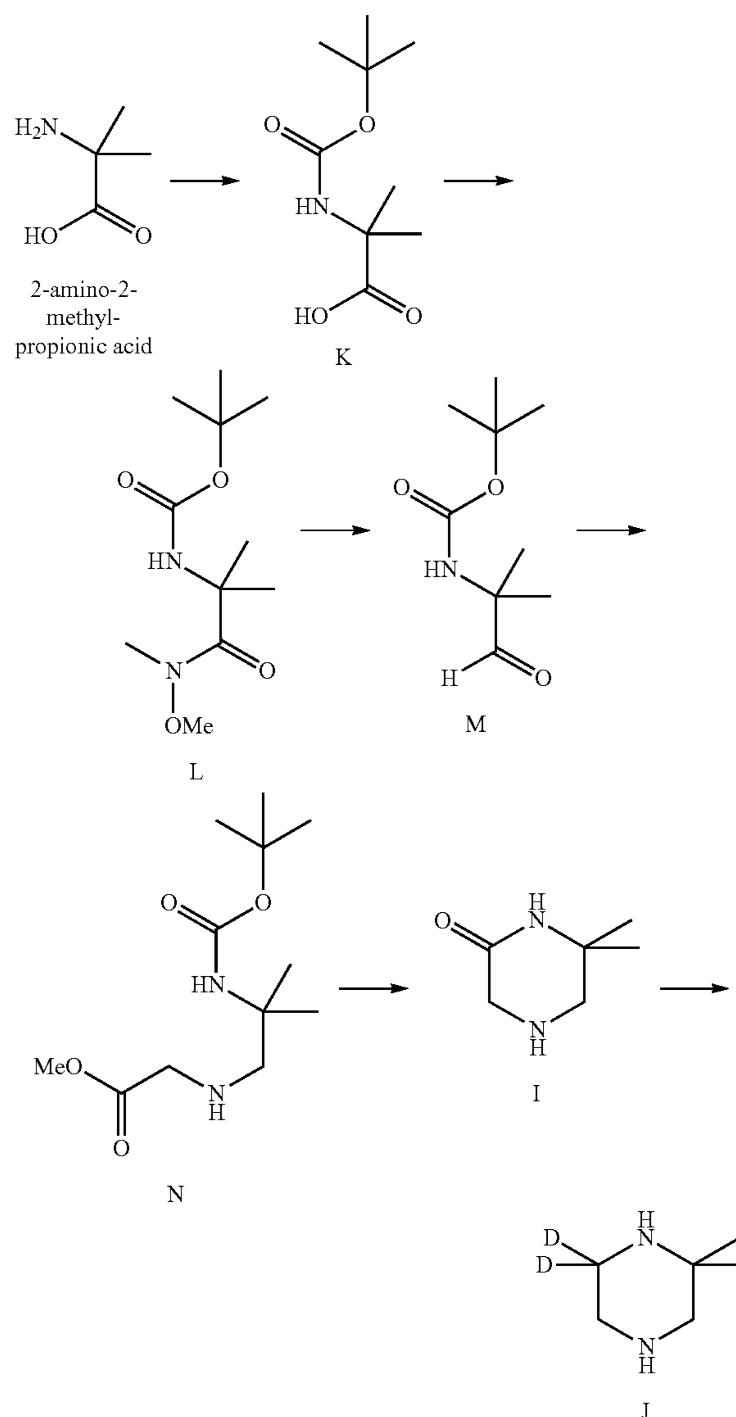
Scheme 11. Synthesis of intermediate J.
