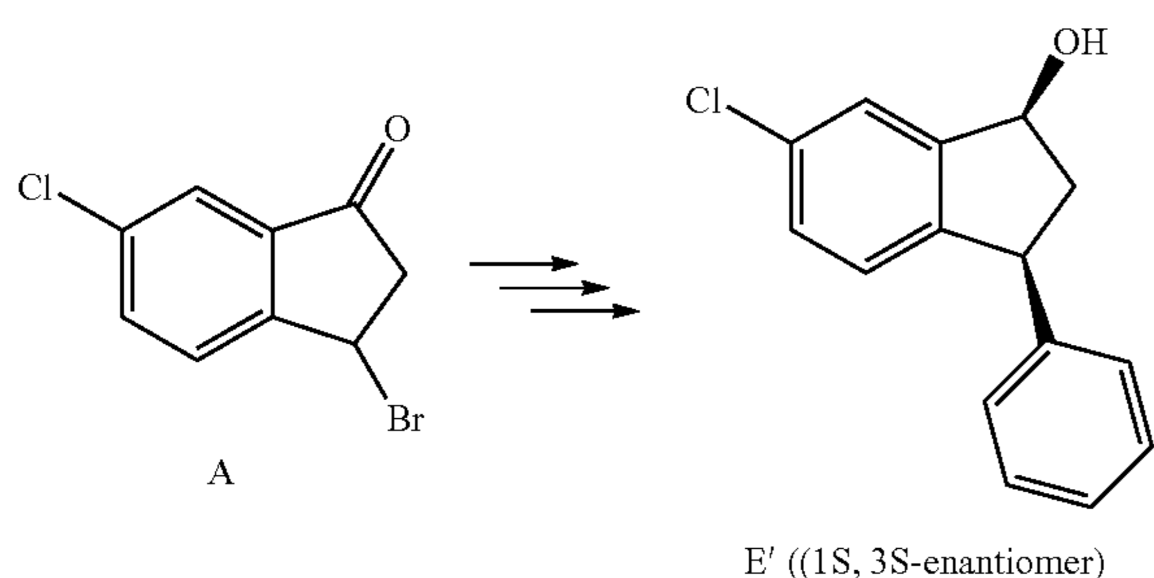
Scheme 3. Exemplary synthesis of intermediate E'.
