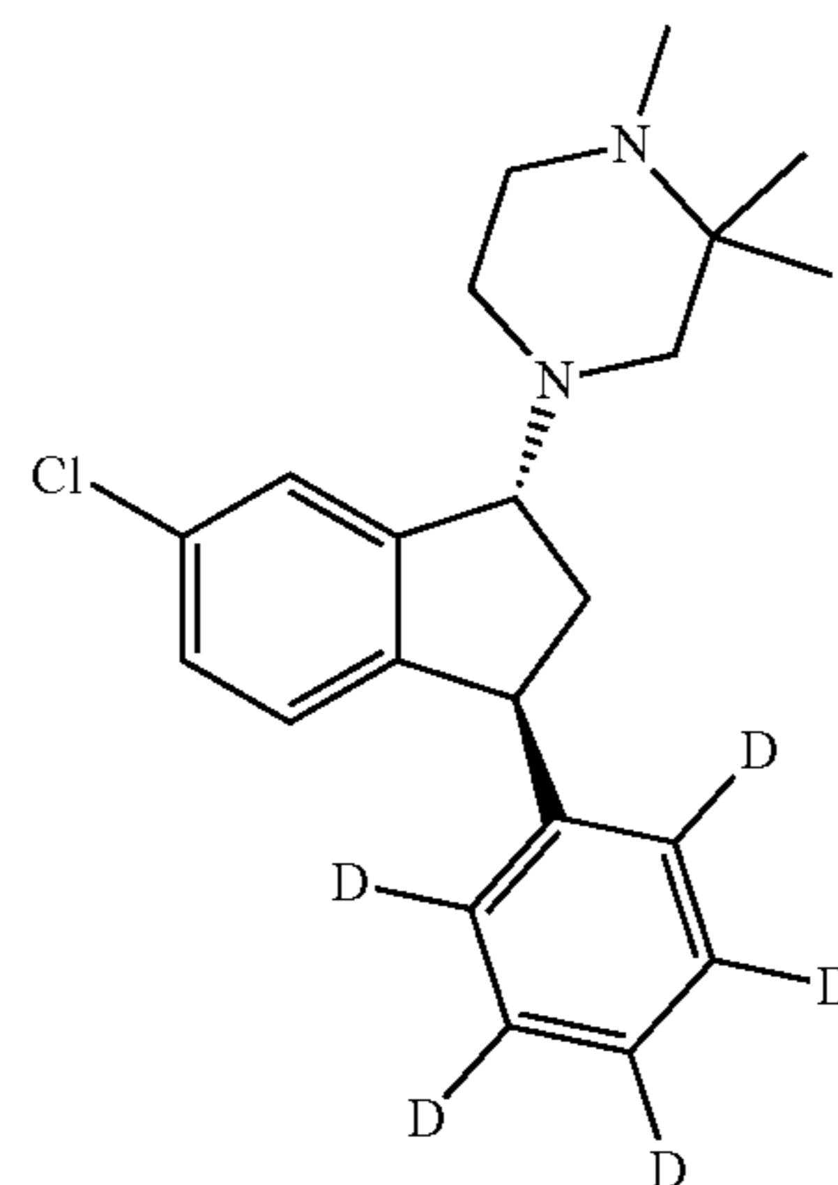
(1R, 3S)-(II)
