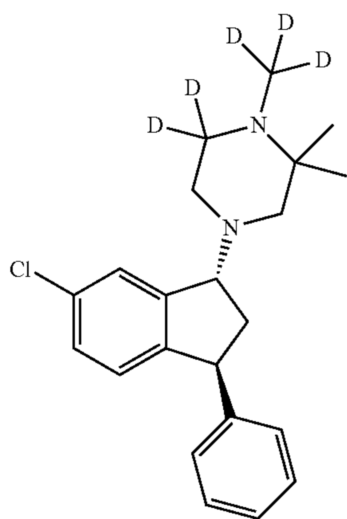
(1R, 3S)-(V)
