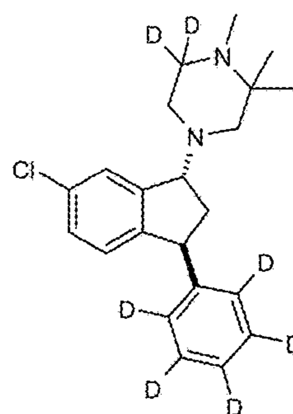
Compound (VII)
