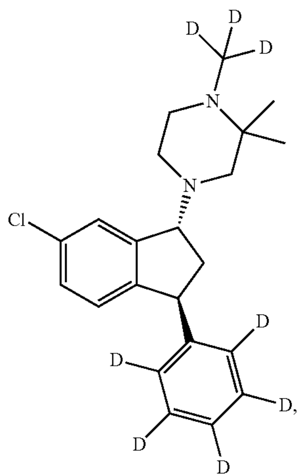
(1R, 3S)-(IV)
