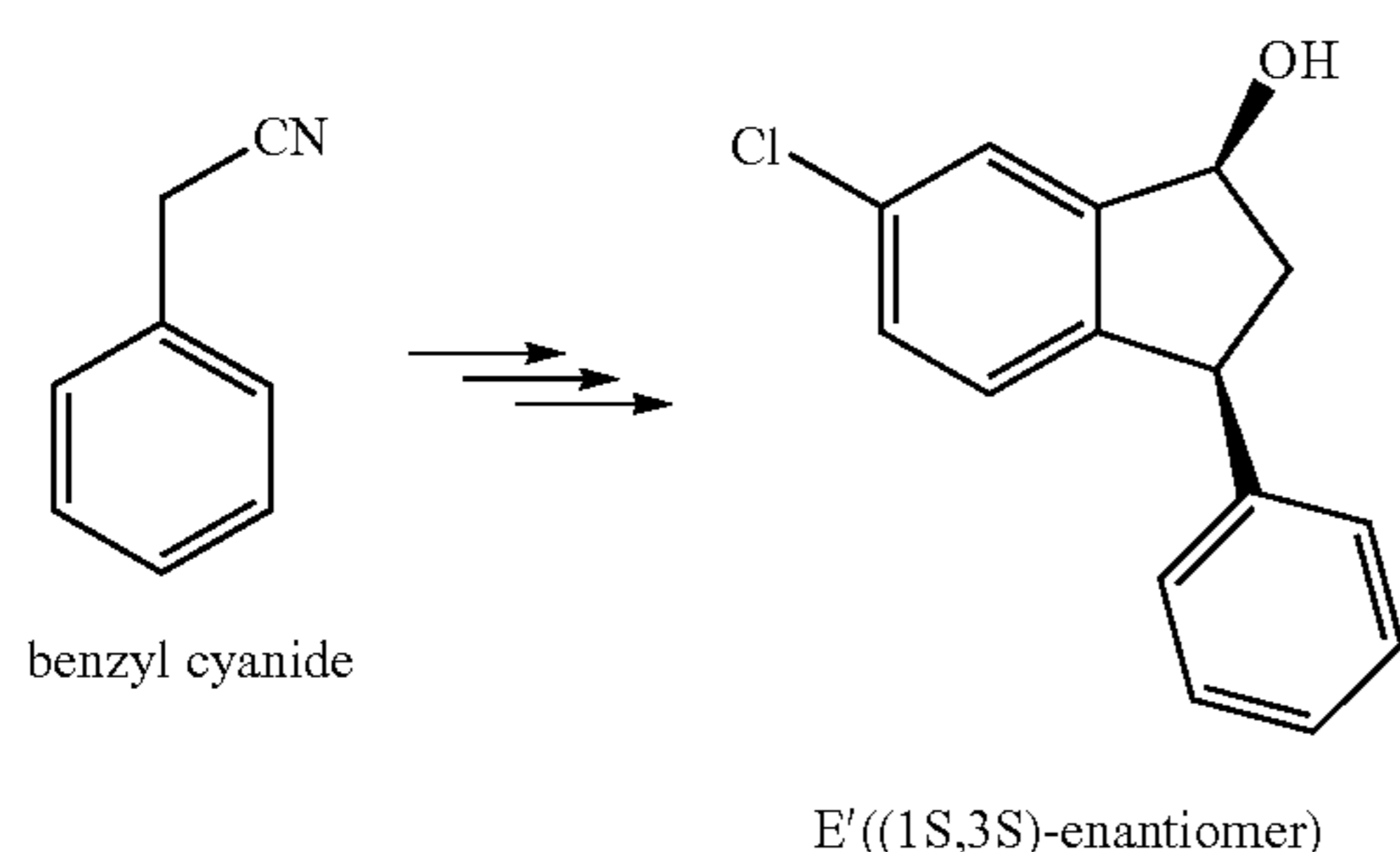
Scheme 4. Exemplary synthesis of intermediates E and E'.
