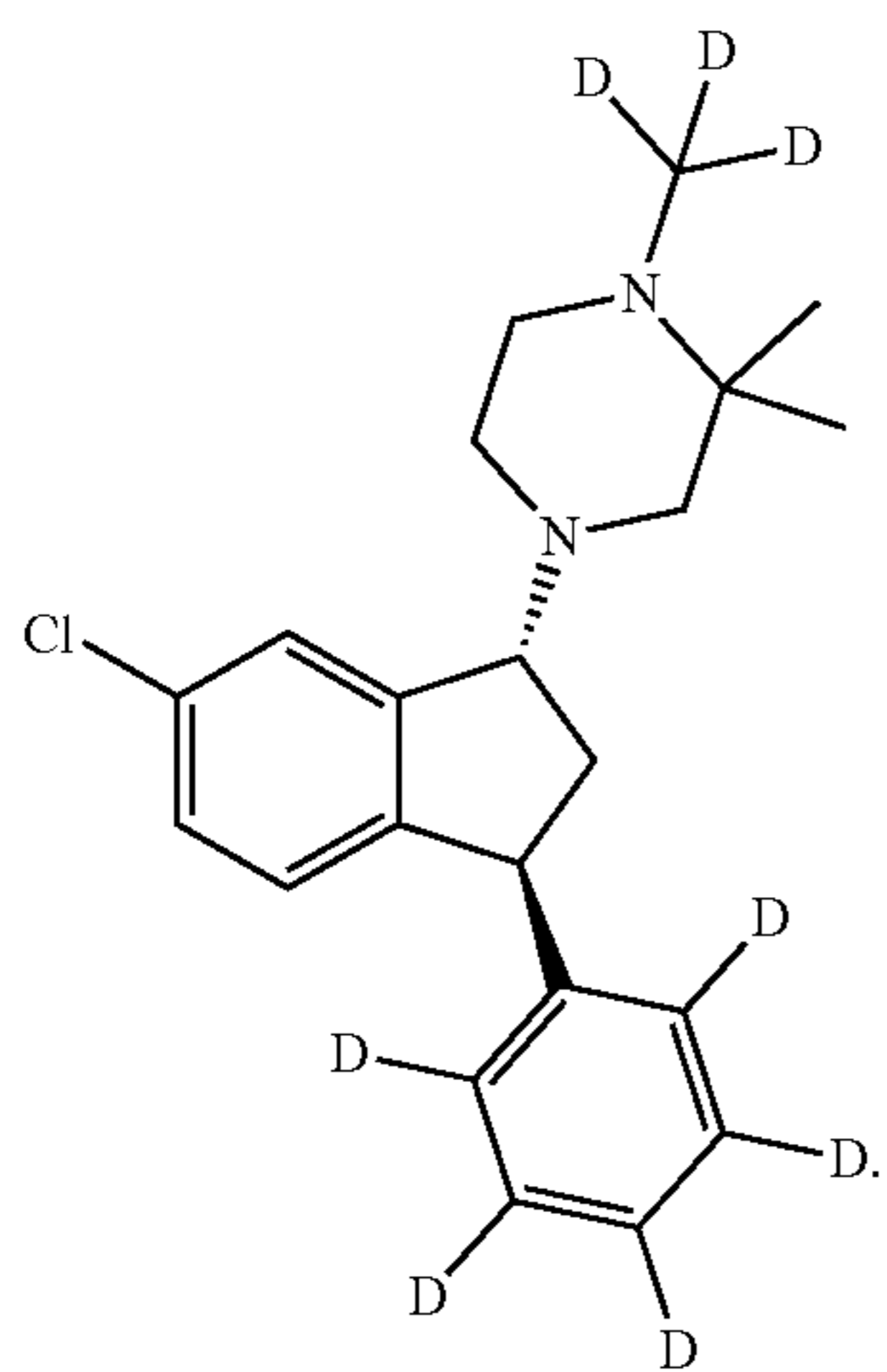
(1R, 3S)-(IV)
