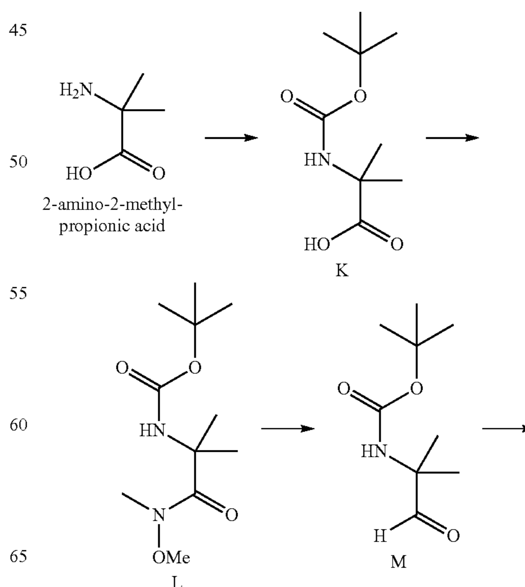
Scheme 7. Alternative exemplary synthesis of intermediate J.
