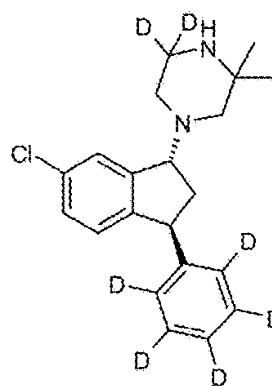
(XXI)
