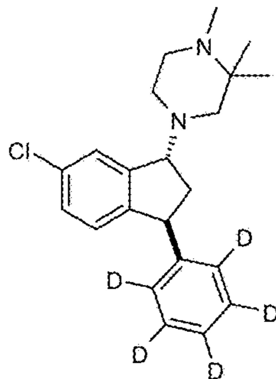
Compound (II)
