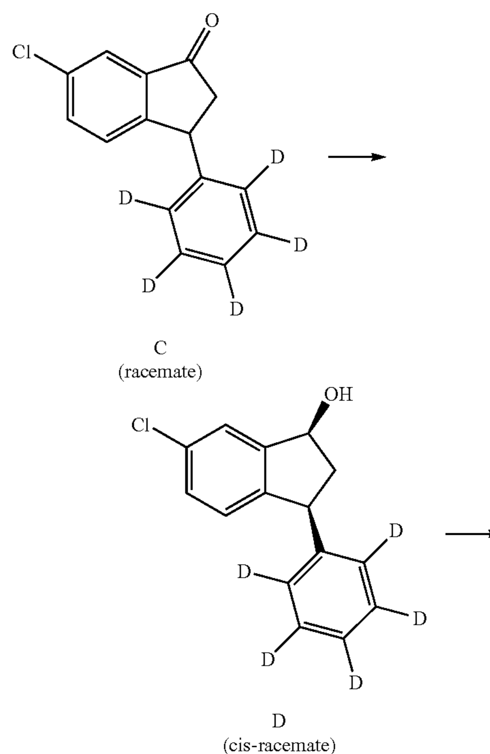
Scheme 2. Exemplary synthesis of intermediate E.
