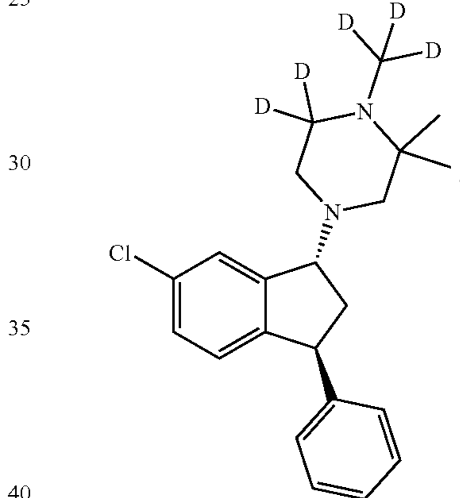
(1R, 3S)-(V)
