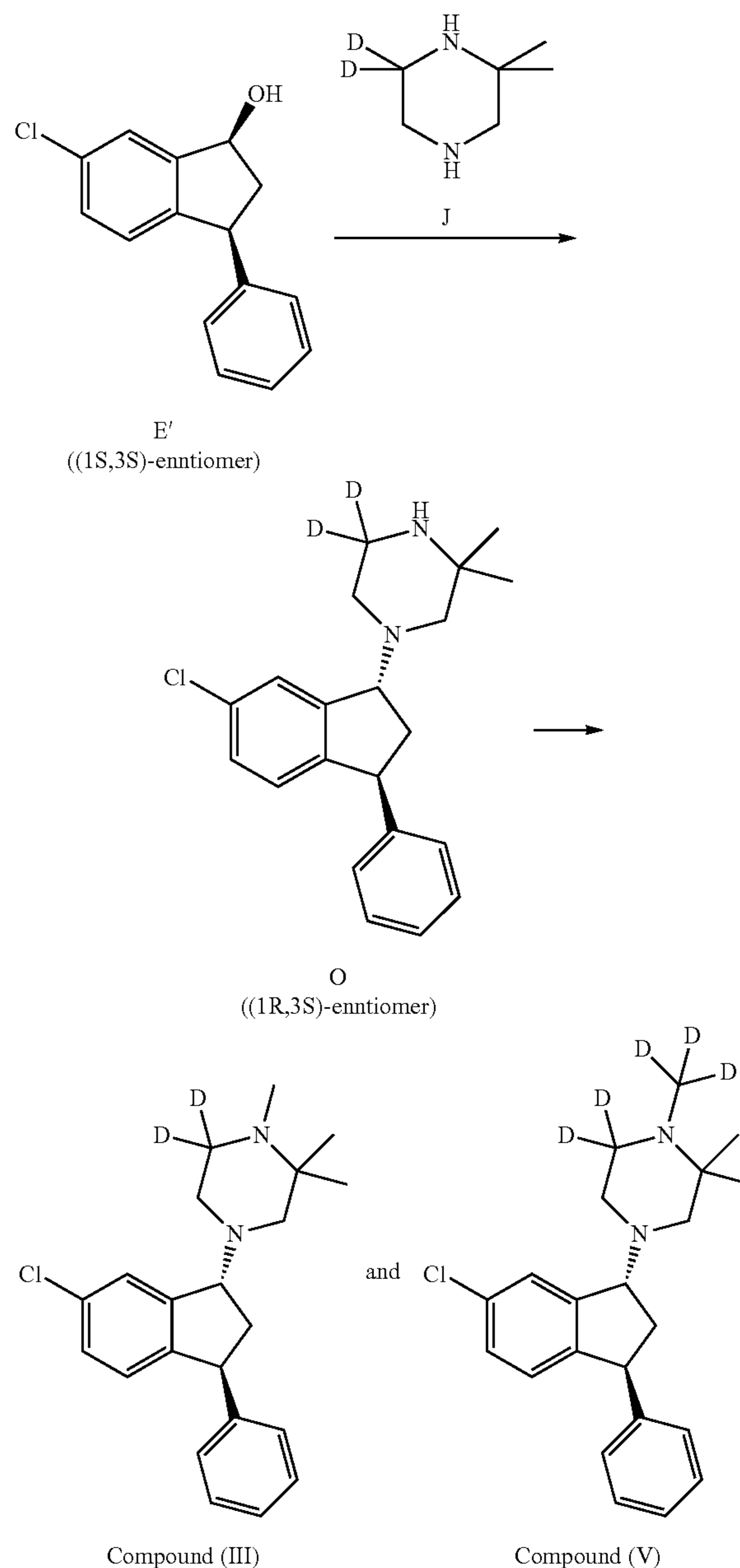
Scheme 12. Synthesis of Compound (III) and Compound (V).
