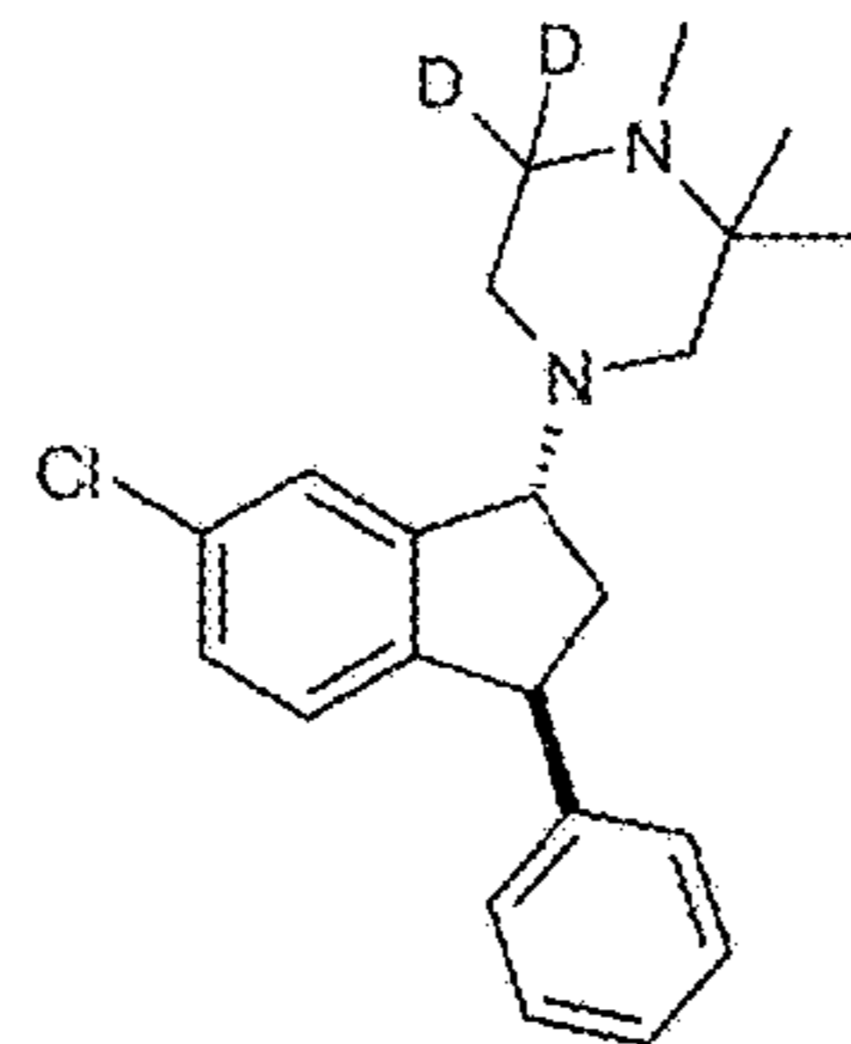
Compound (III)
