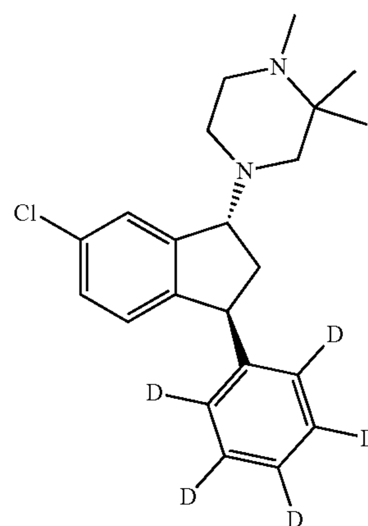
(1R, 3S)-(II)
