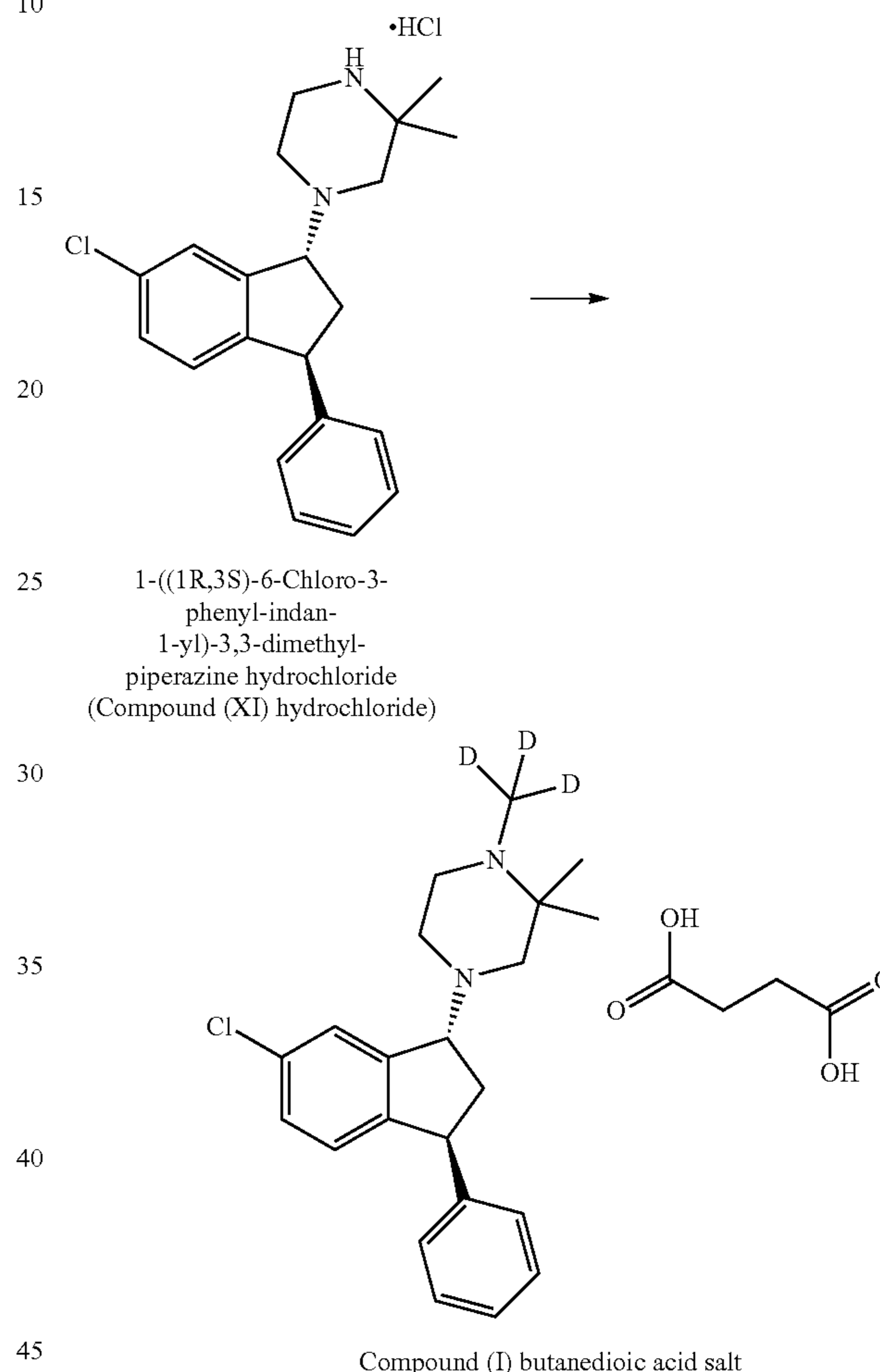
Scheme 8. Synthesis of Compound (I).
