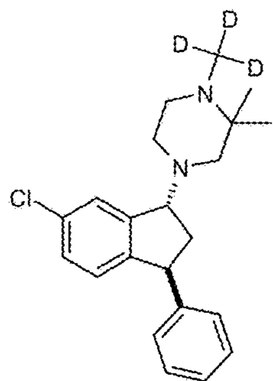
Compound (I)
