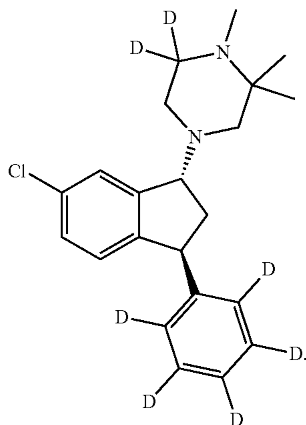
(1R, 3S)-(VII)
