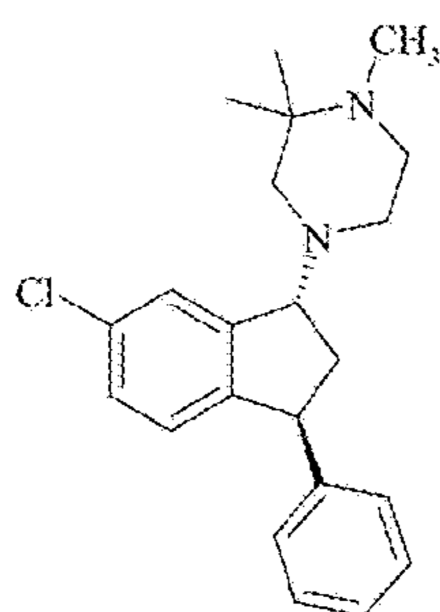
Compound (VI)
