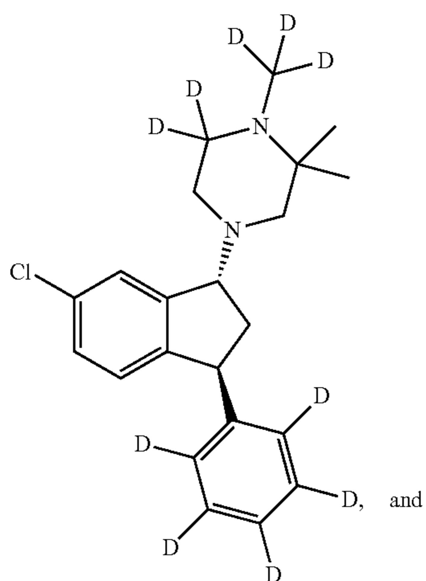
(1R, 3S)-(VI)
