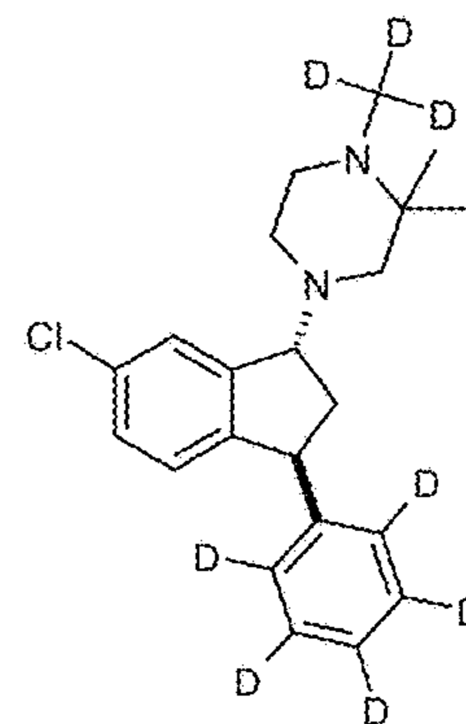
Compound (IV)
