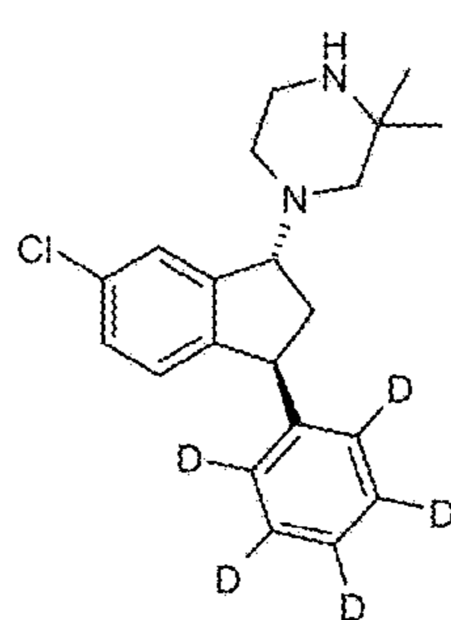
(XX)
