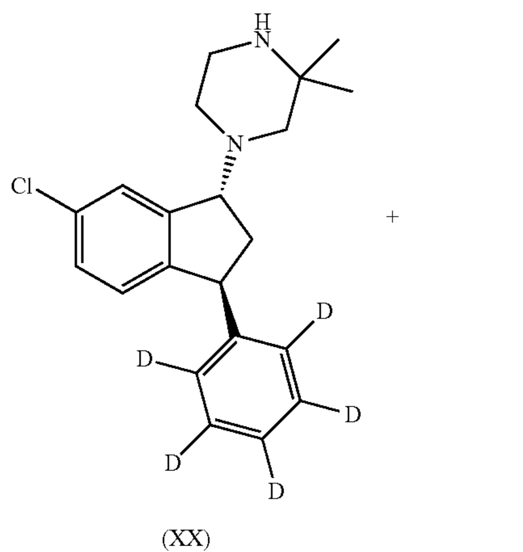
Scheme 17: Synthesis of rac-trans-1-(6-chloro-3-phenyl( d 5 )-indan-1-yl)-1( d 3 ), 2,2-trimethyl-piperazine succinate
