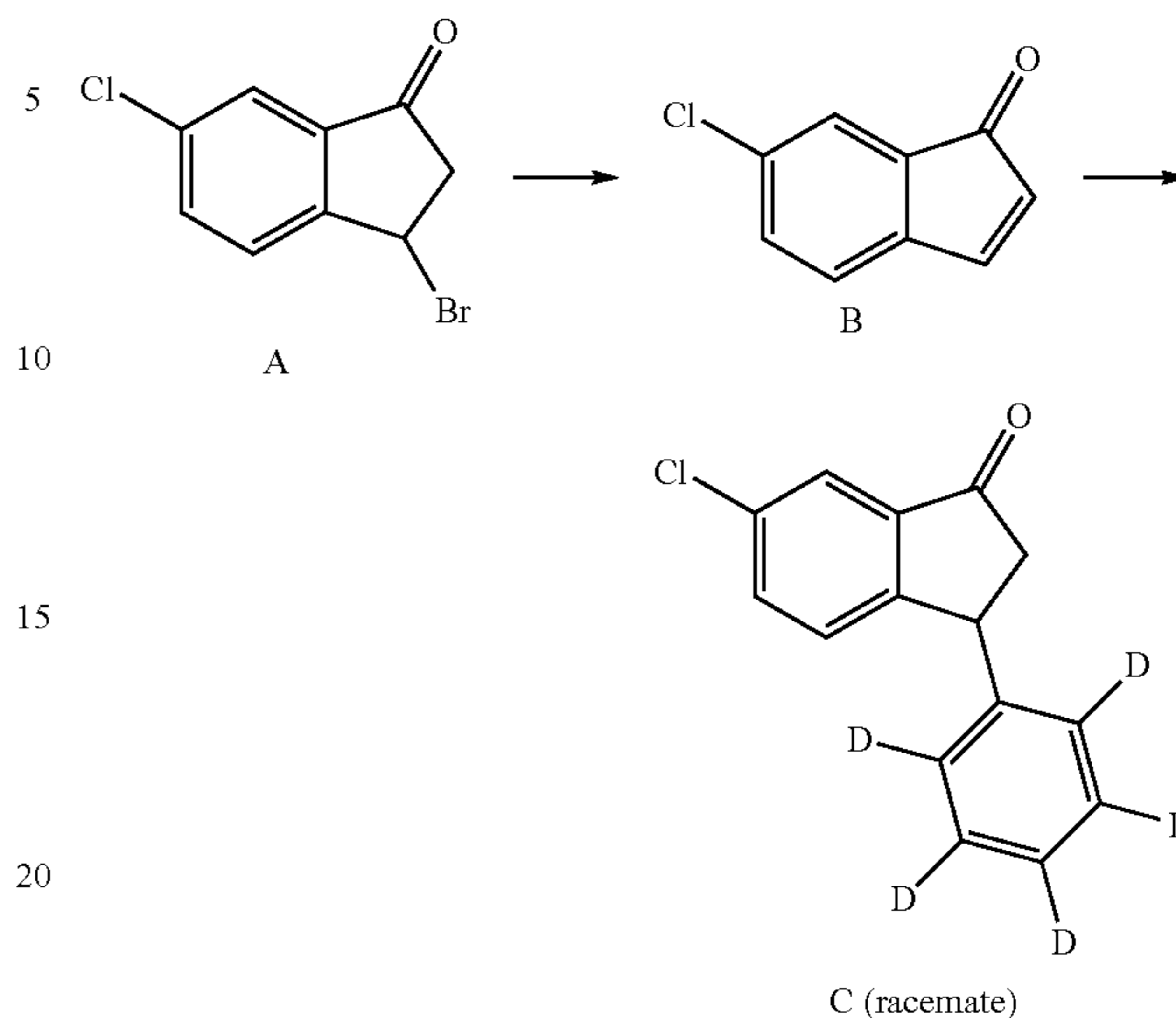
Scheme 1. Exemplary synthesis of intermediate C.
