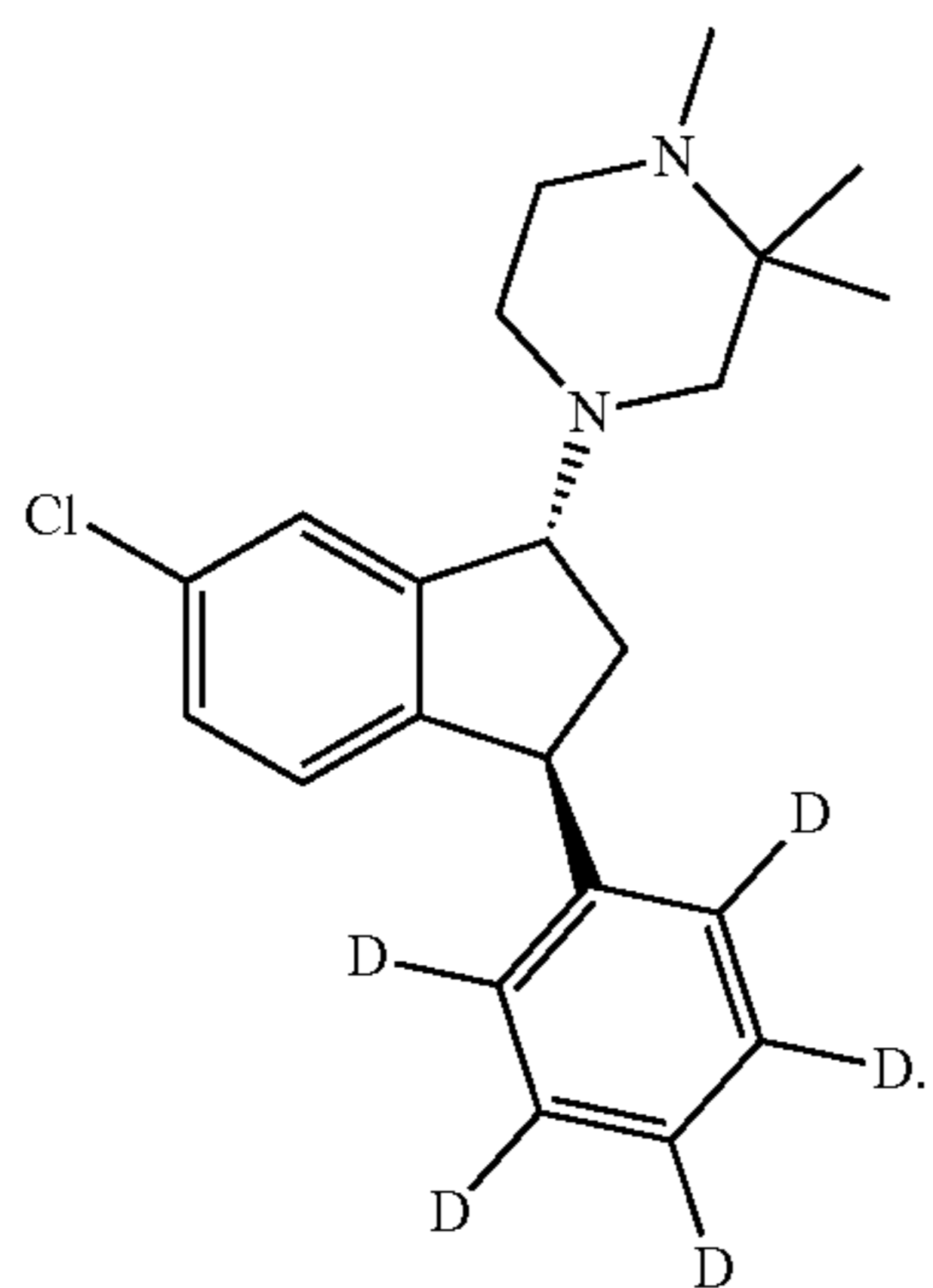
(1R, 3S)-(II)
