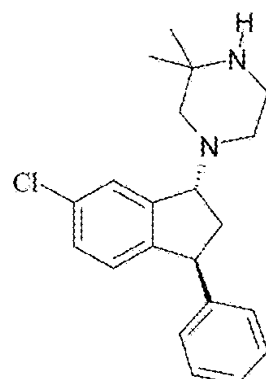
Compound (VII)
