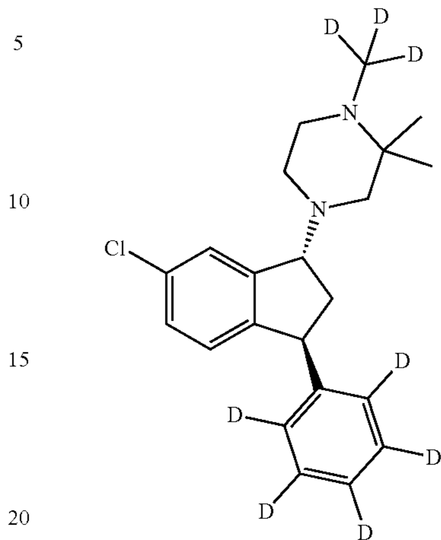
(1R, 3S)-(IV)
