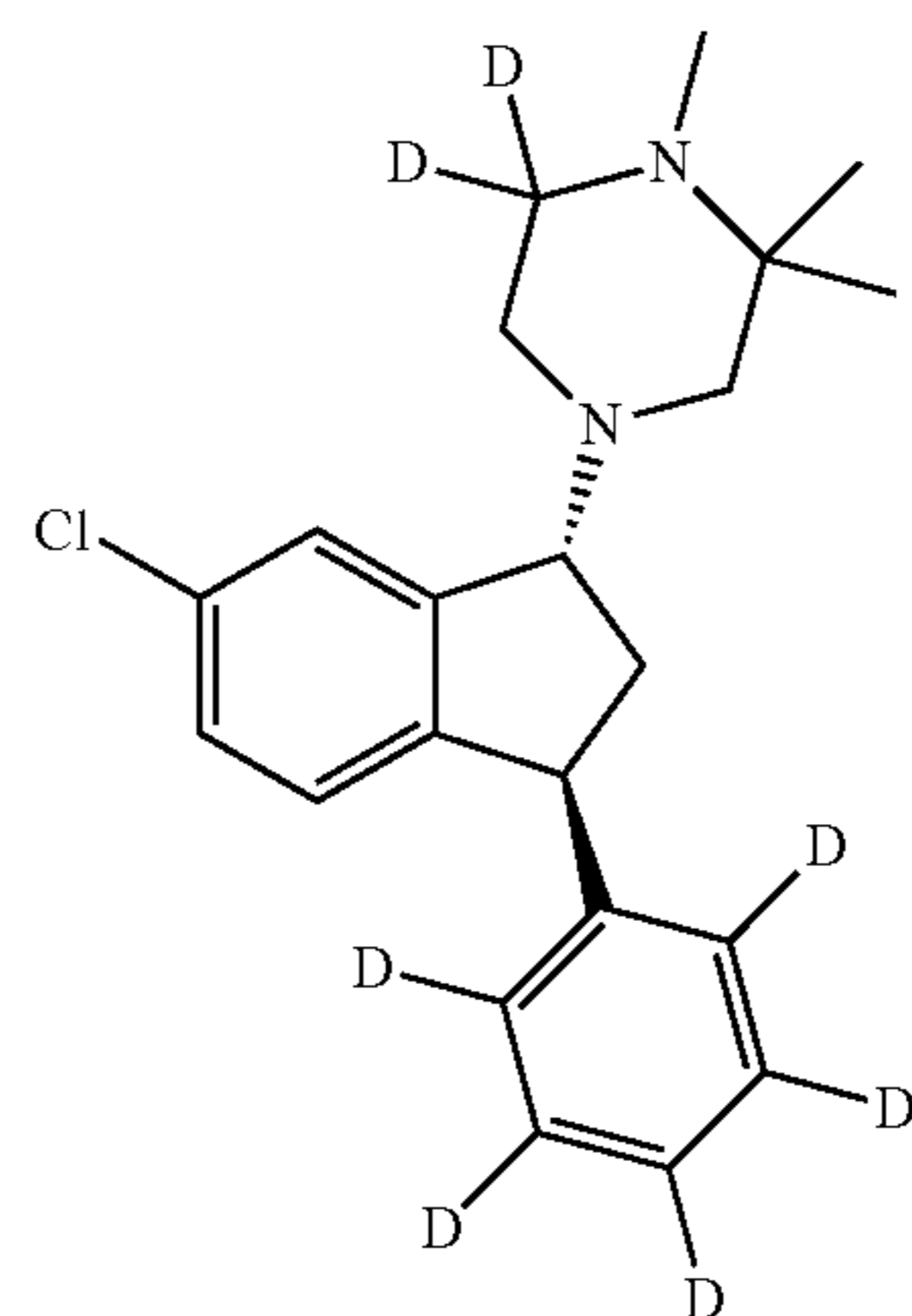
(1R, 3S)-(VII)
