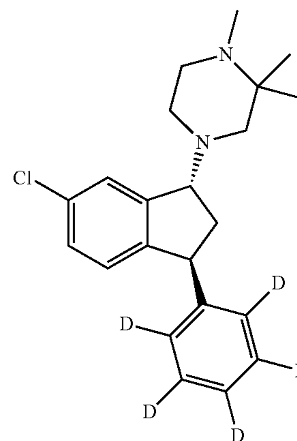
(1R, 3S)-(II)
