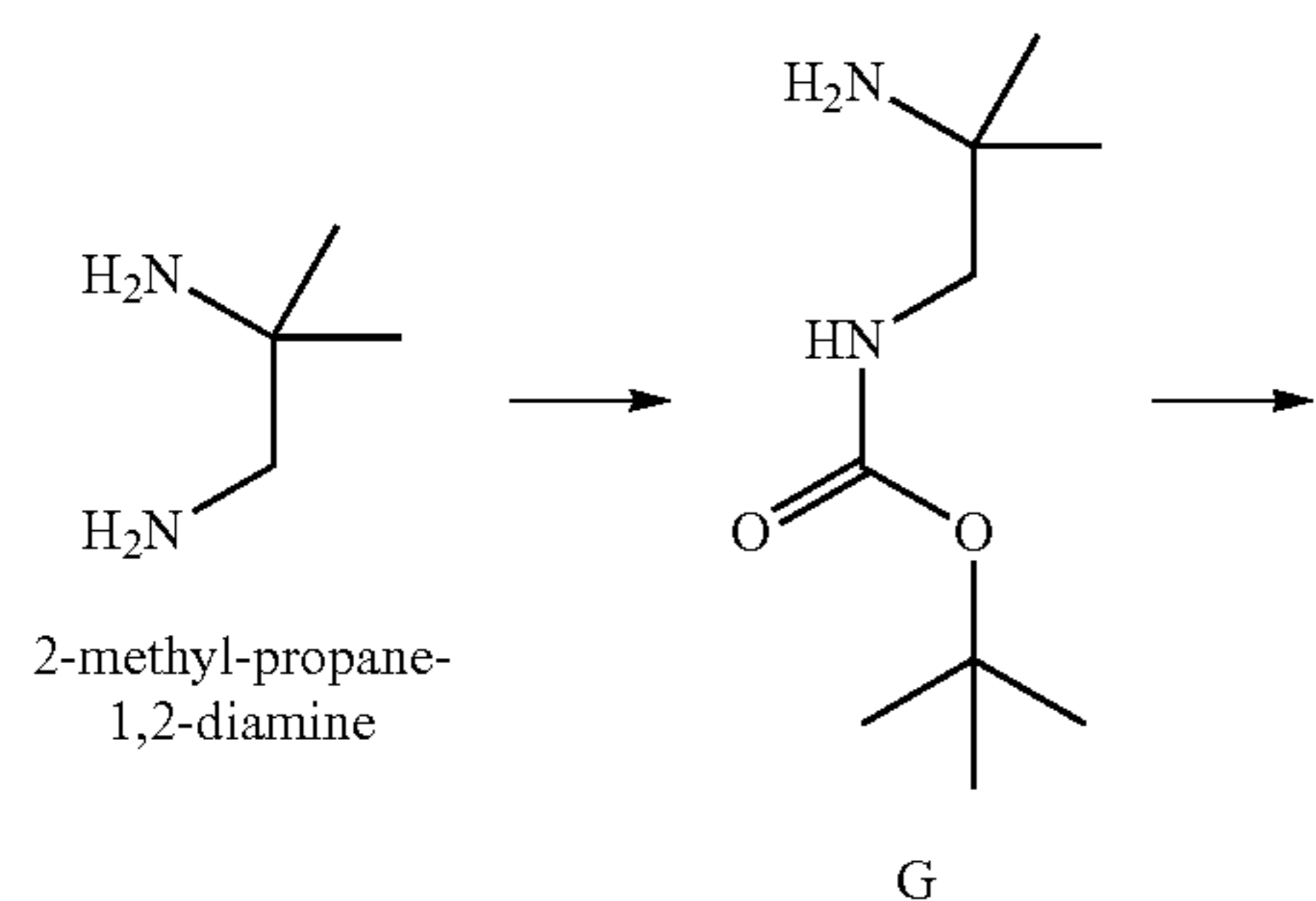
Scheme 6. Exemplary synthesis of intermediate J.
