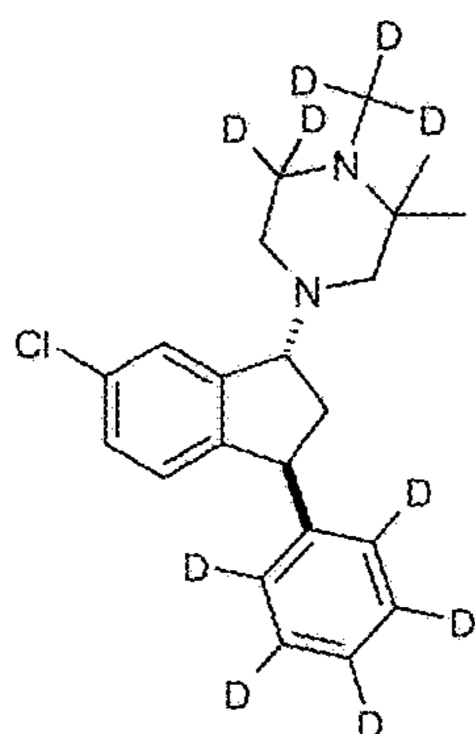
Compound (VI)
