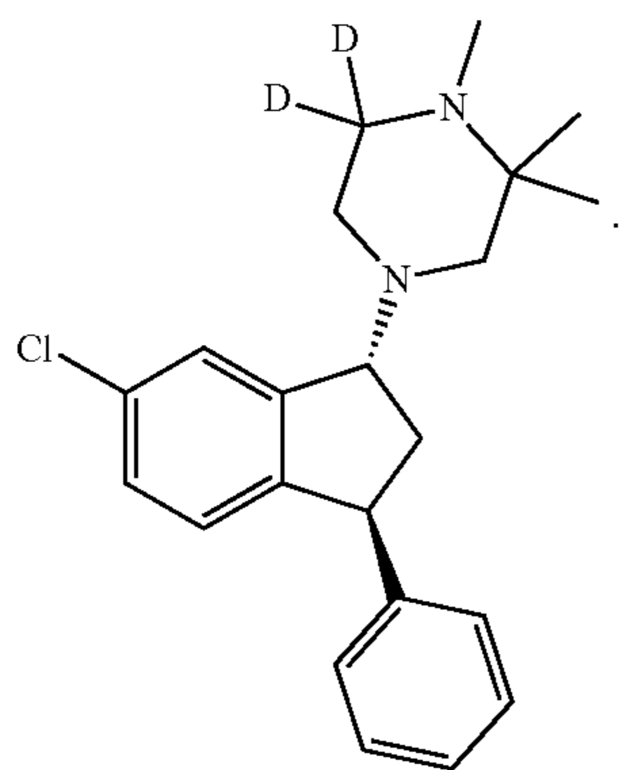
(1R, 3S)-(III)
