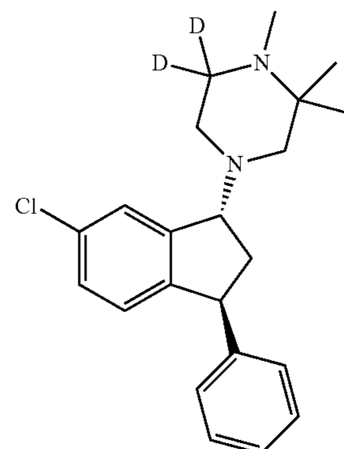
(1R, 3S)-(III)
