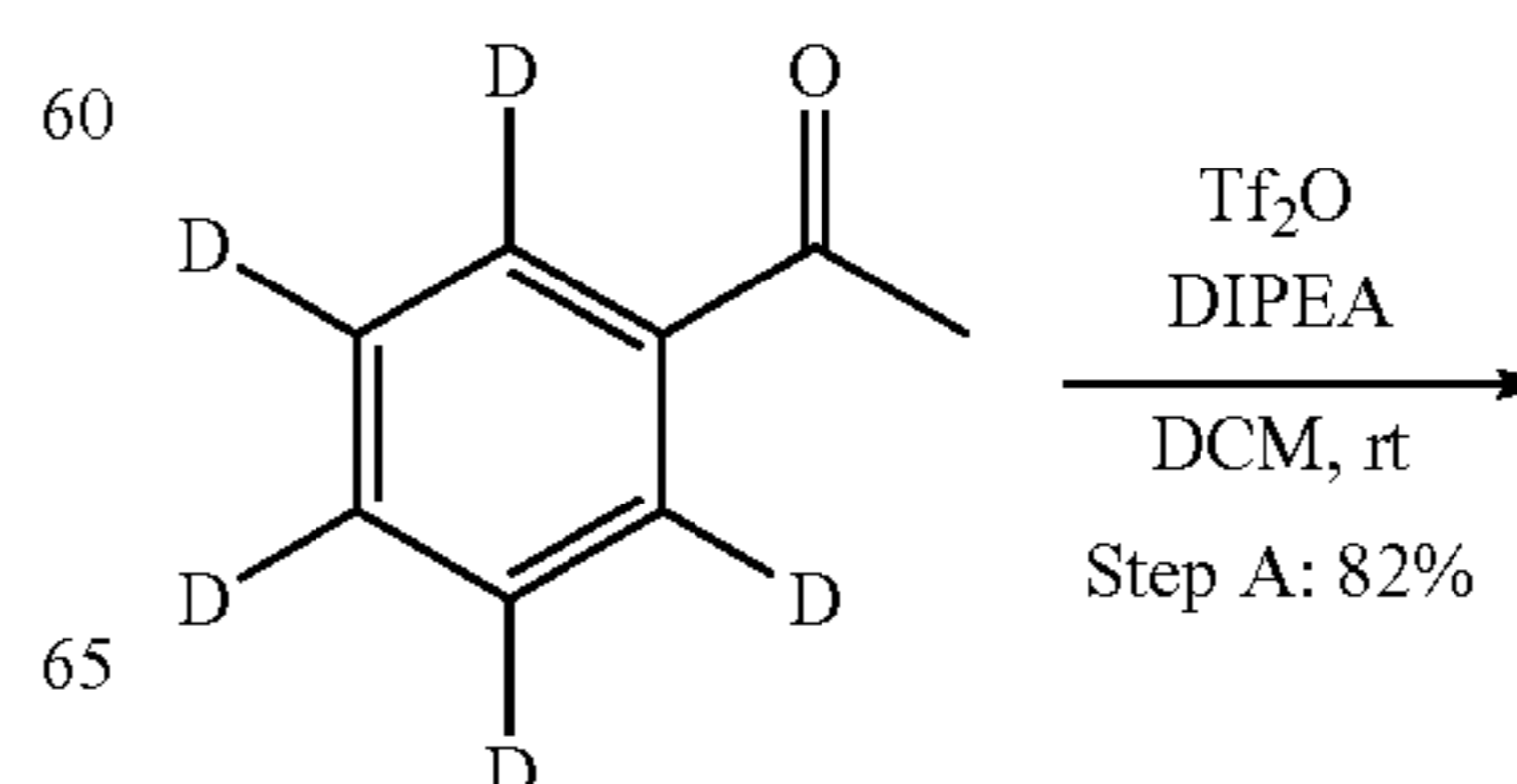
Scheme 14. Synthesis of Compound (XV)
