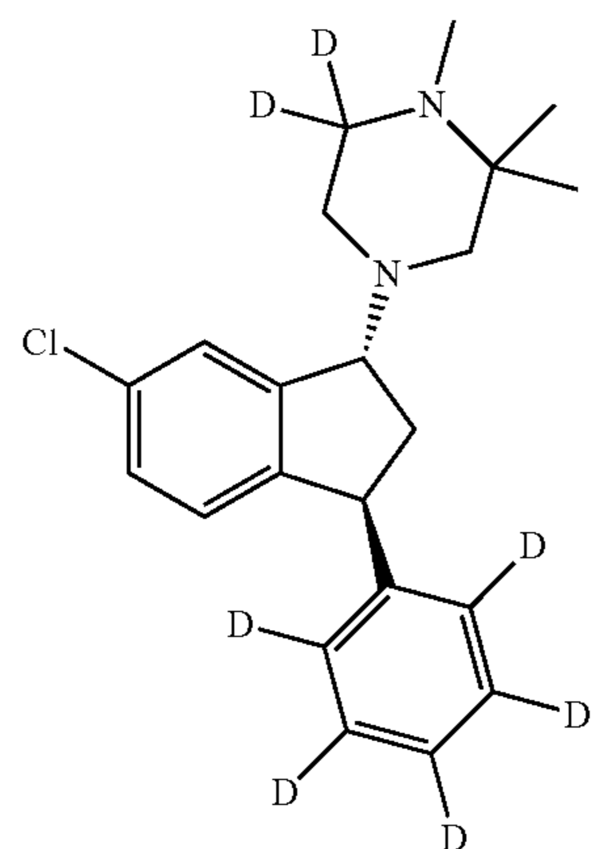
(1R, 3S)-(VII)
