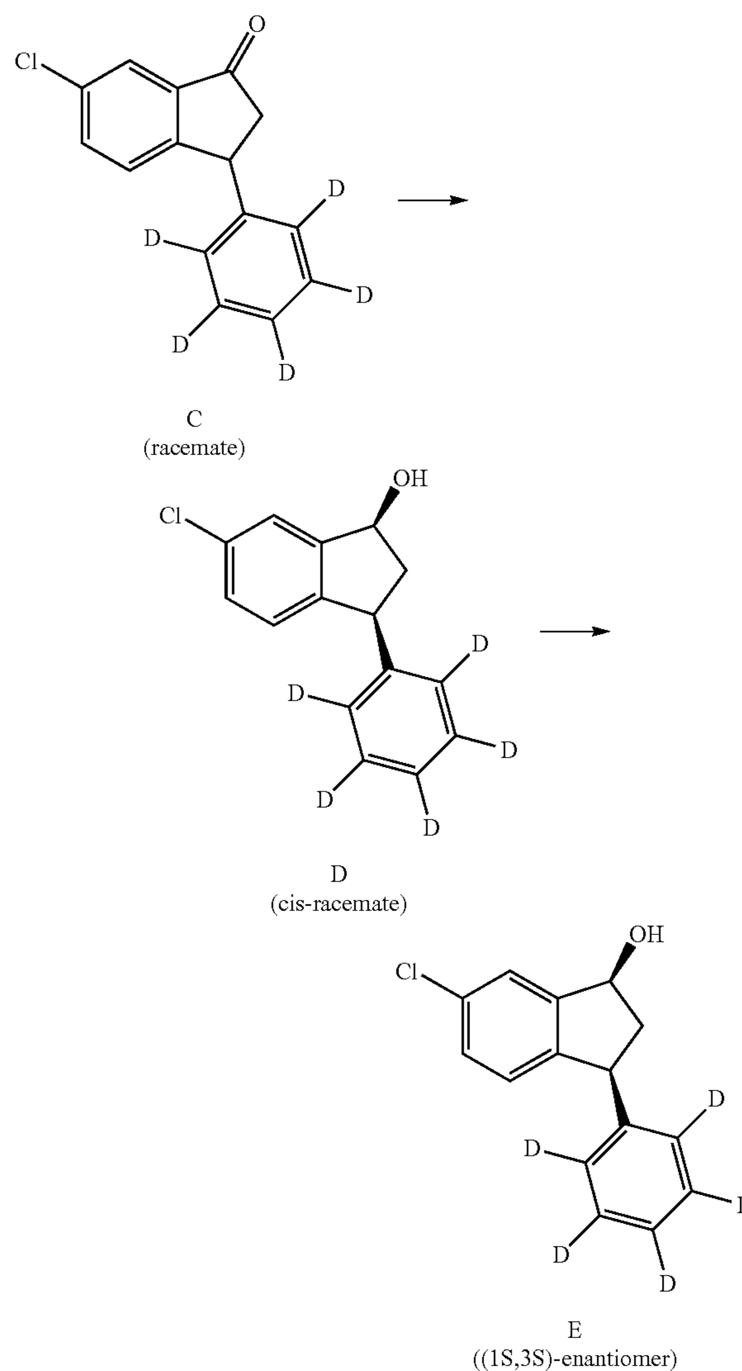
Scheme 10. Synthesis and resolutions of Compound E.
