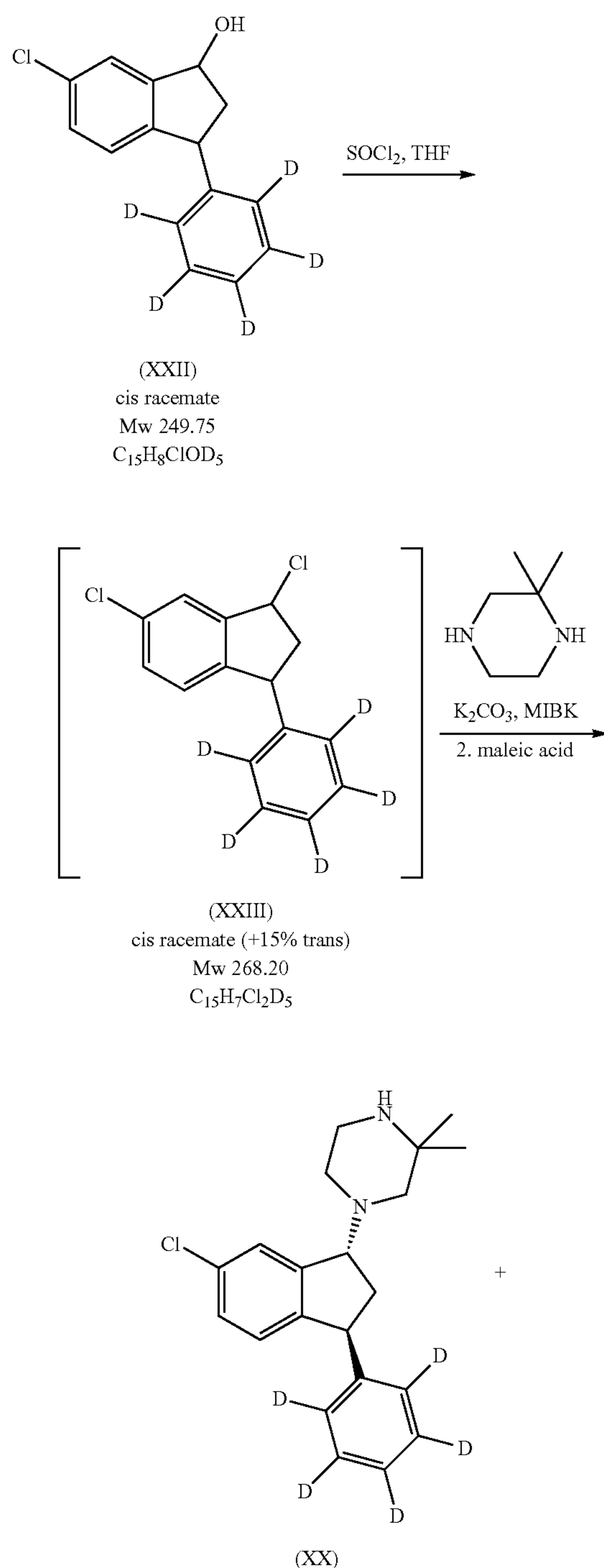
Scheme 16: Synthesis of rac-trans-1-(6-Chloro-3-phenyl(d 5 )-indan-1-yl)-3,3-dimethyl-piperazine maleate
