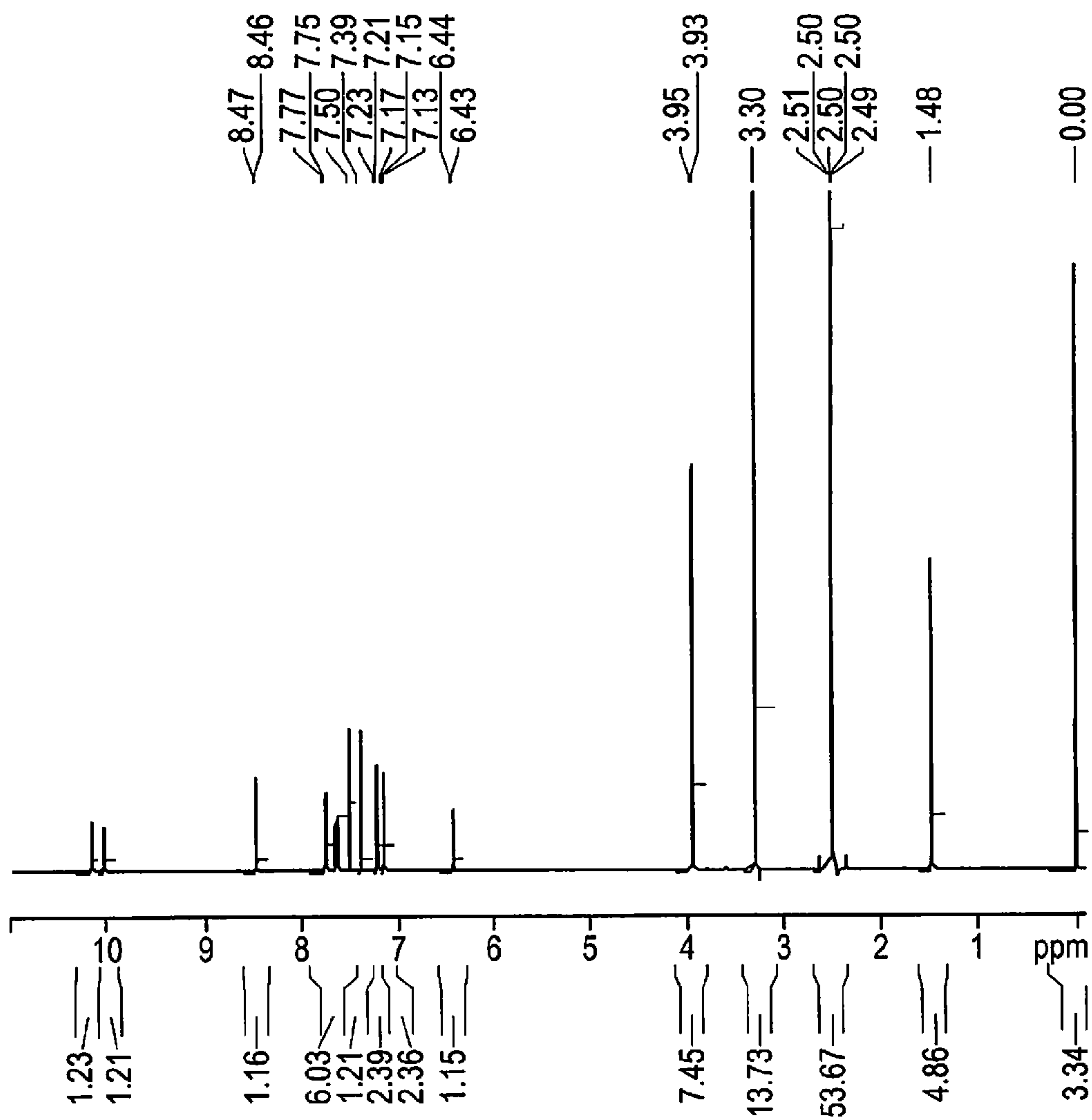
1 H NMR of Compound I Form I
