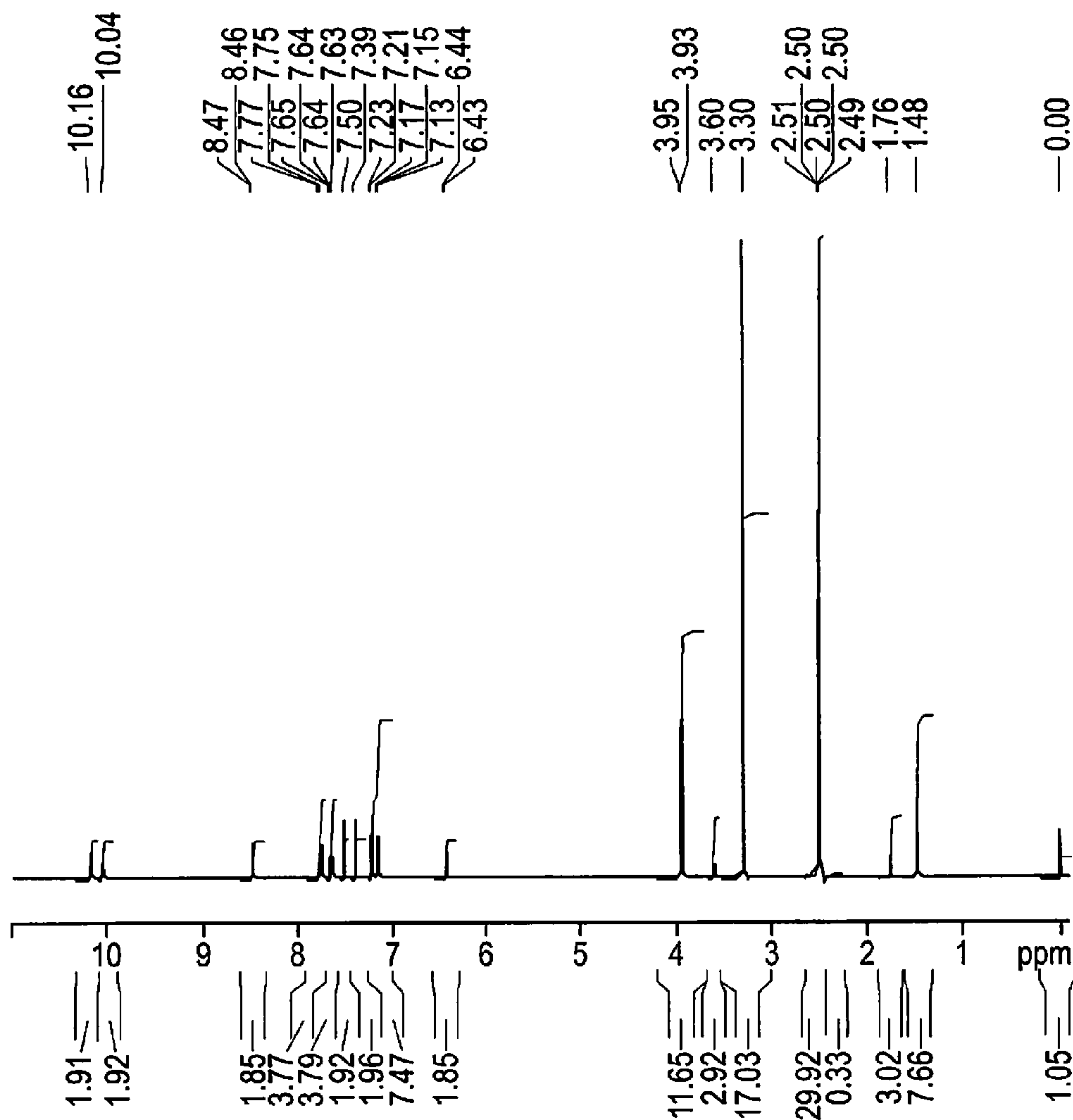
1 H NMR of Compound I Form II
