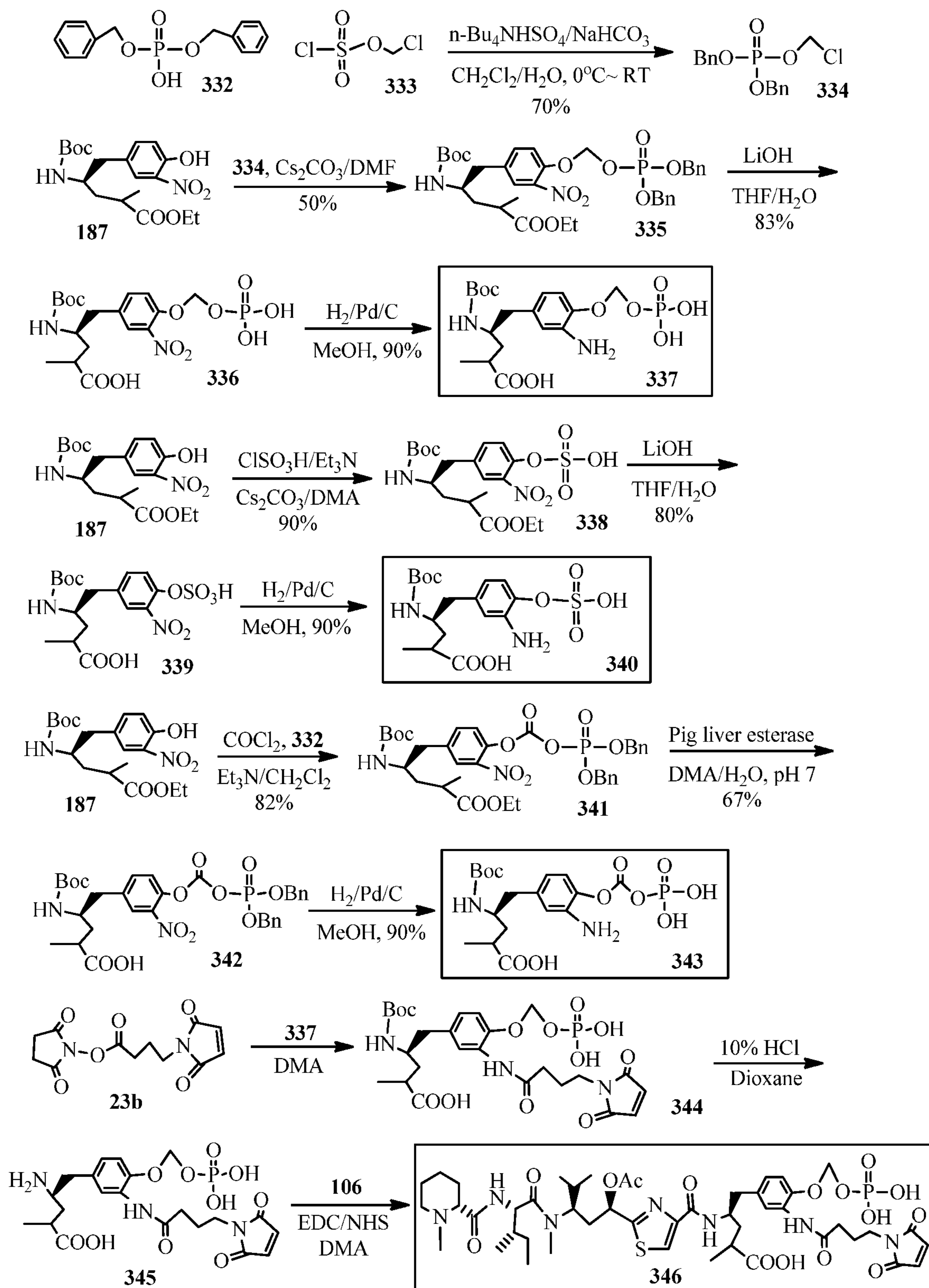
Fig. 29. Synthesis of hydrophilic Tut analogs for the synthesis of the hydrophilic prodrugs of antimetabolic agents
