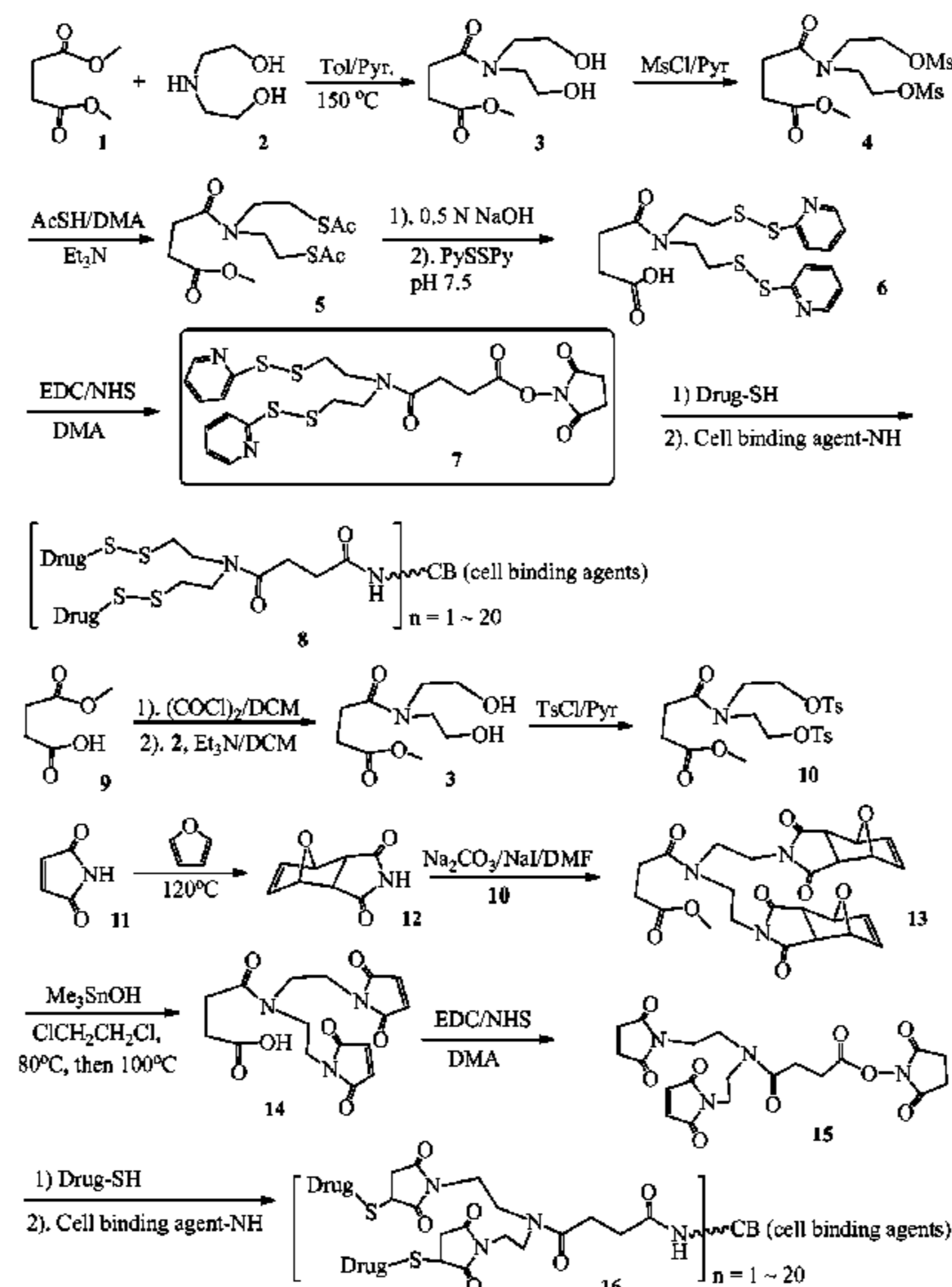
The synthesis of branched linkers for conjugation of drugs to cell binding agents.
