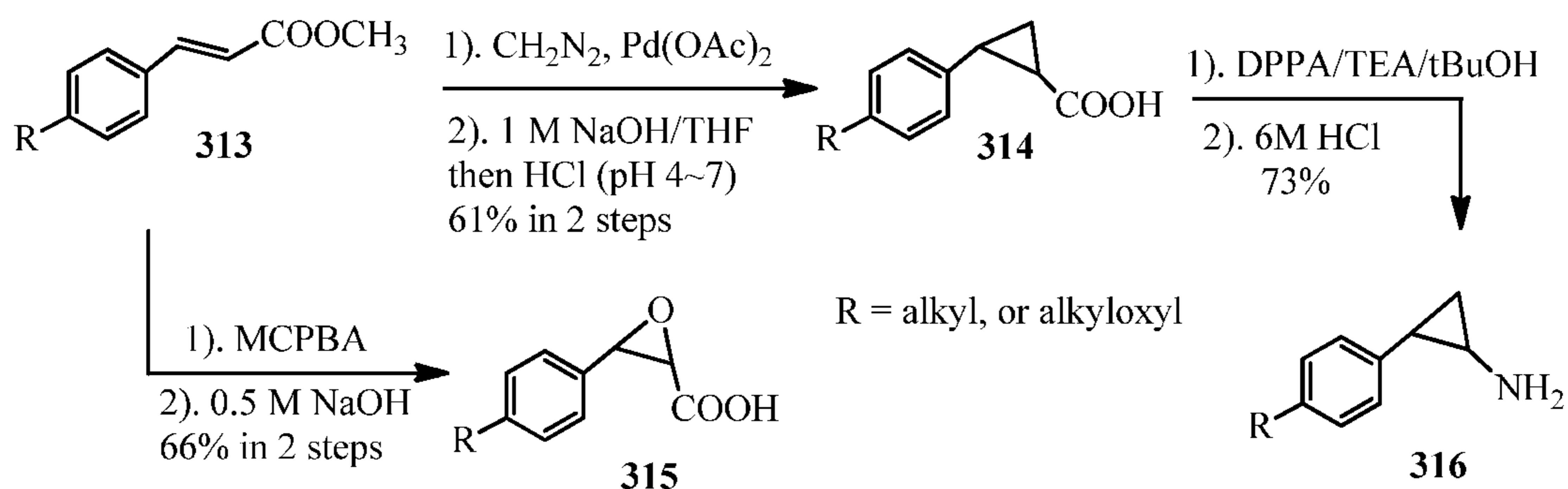
Figure 27. The synthesis of trans -2-arylcyclopropylamines, trans -2-arylcyclopropylcarboxyl acids and trans -2-arylethylepoxidyl carboxylic acids.
