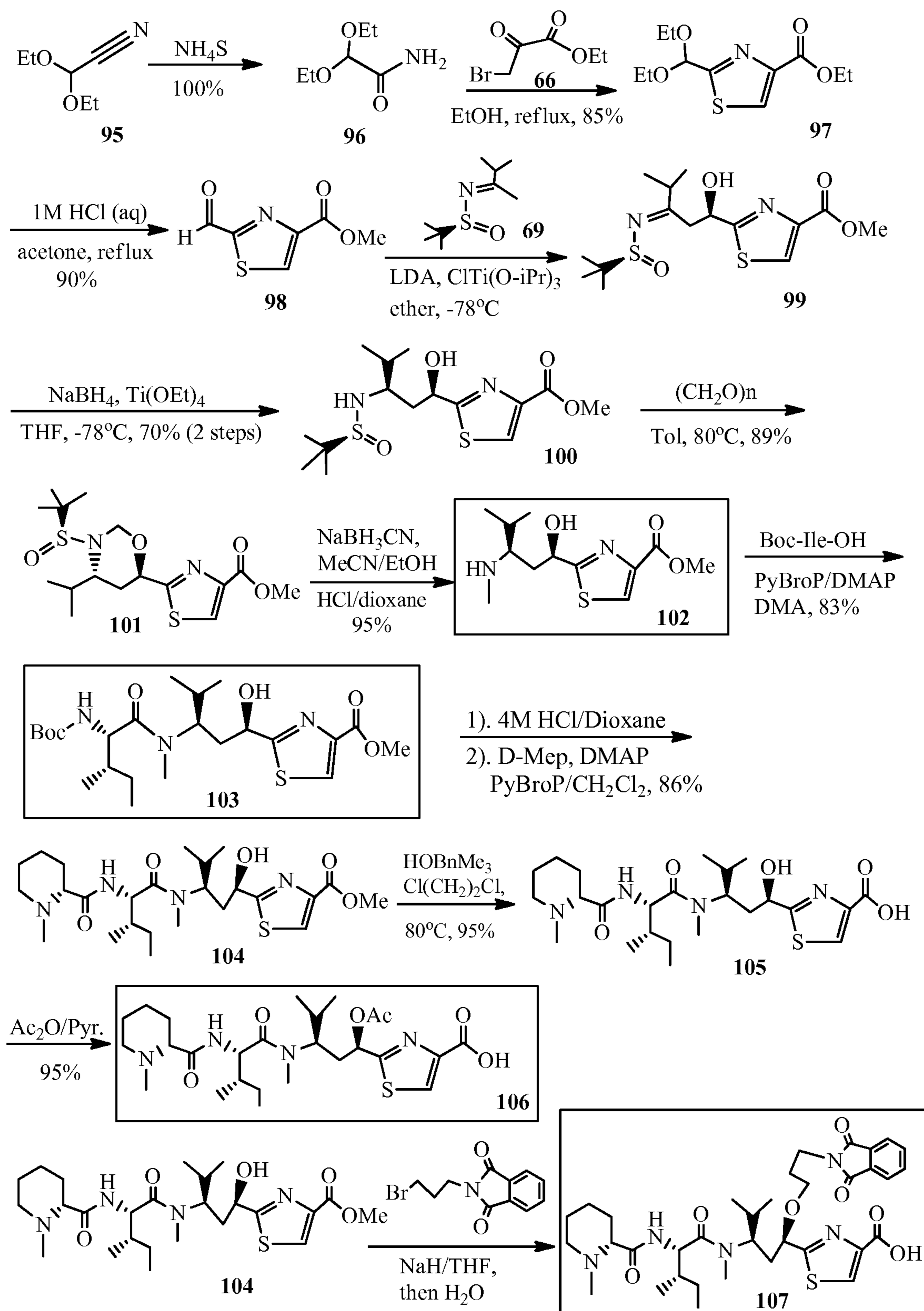
Figure 8. The synthesis of Tuv, Ile-Tuv and Mep-Ile-Tuv moieties of the antimetabolic agents.
