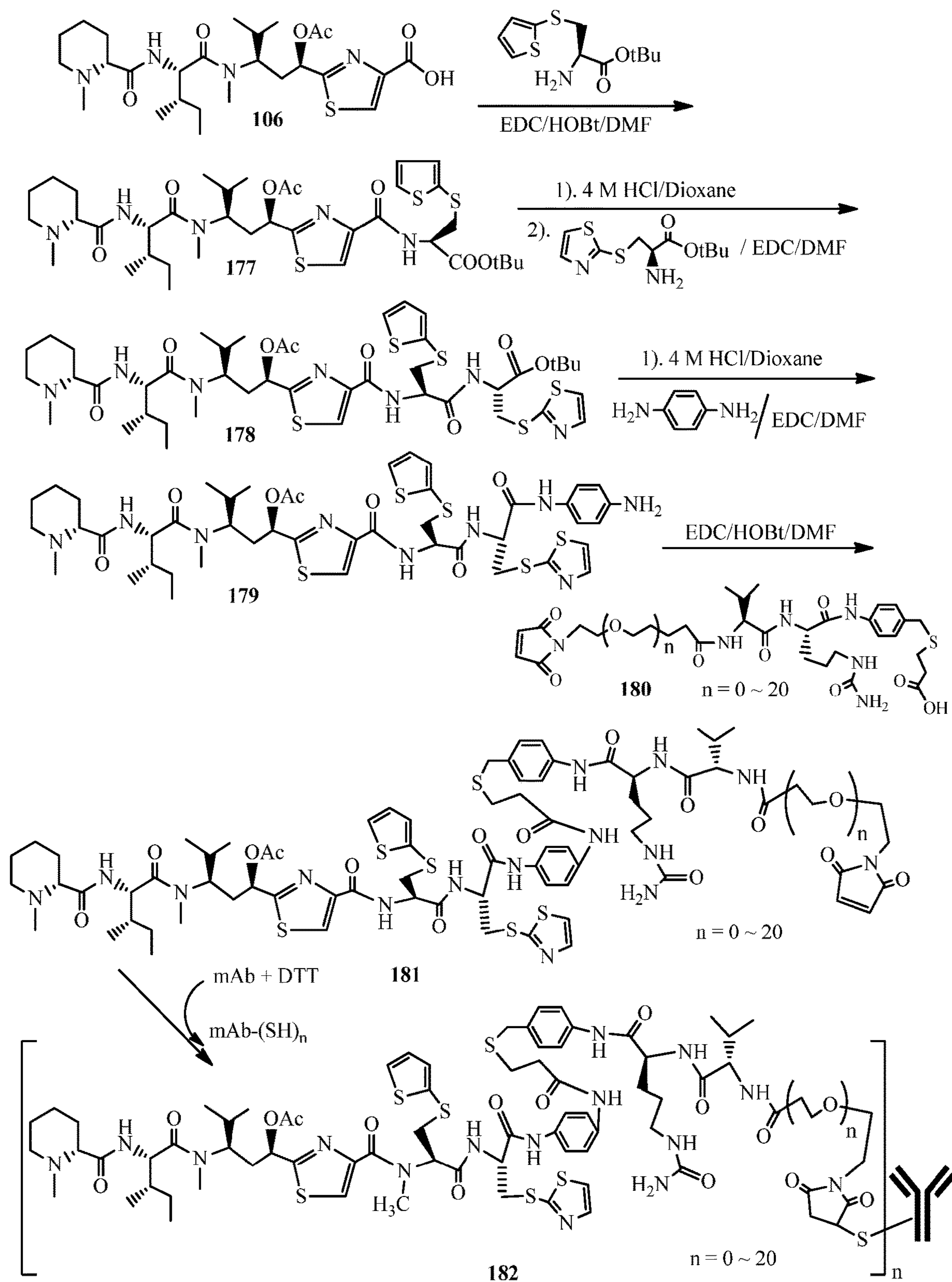
Figure 17. The synthesis of an antibody-antimitotic agent conjugates.
