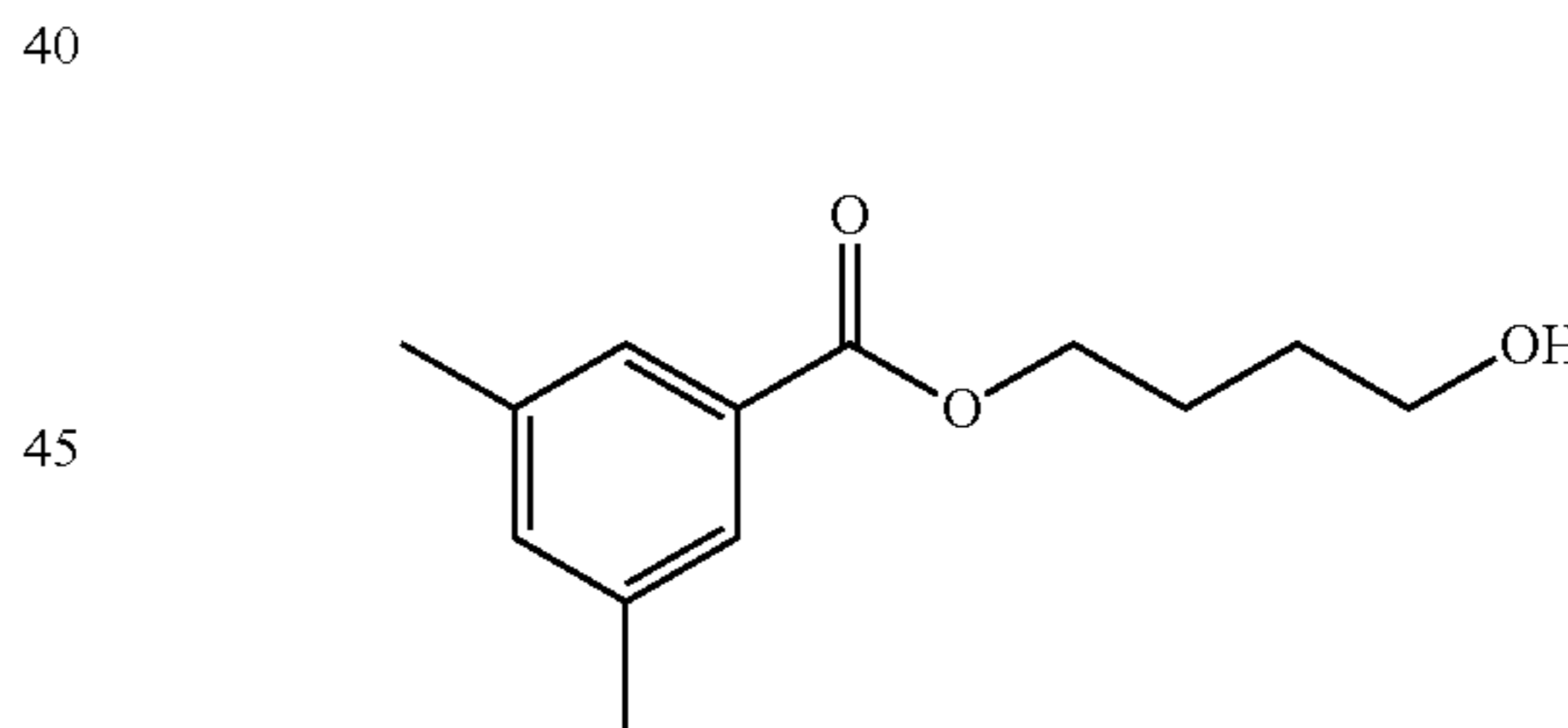
Intermediate Compound 19': 4-hydroxybutyl 3,5-dimethylbenzoate
