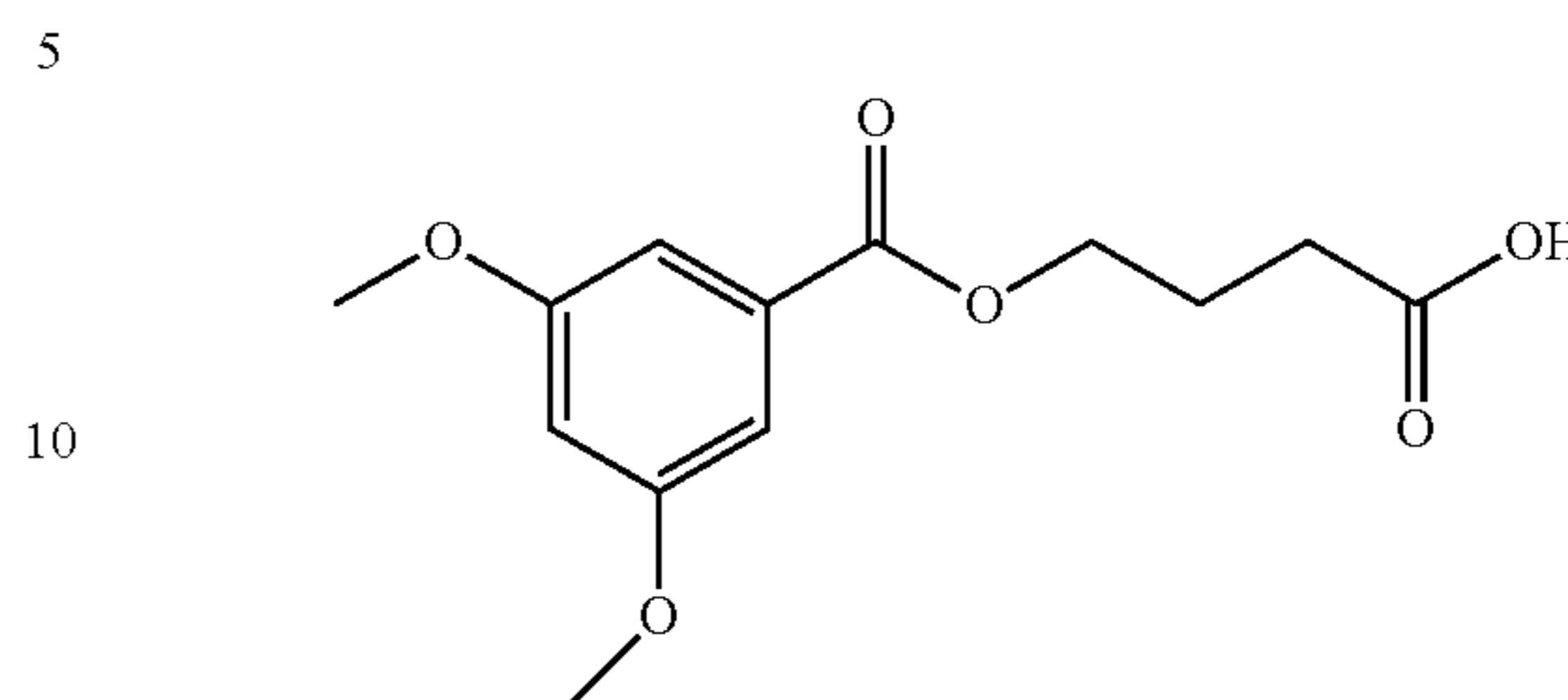
Compound 18: 4-(3,5-dimethoxybenzoyloxy)butanoic Acid
