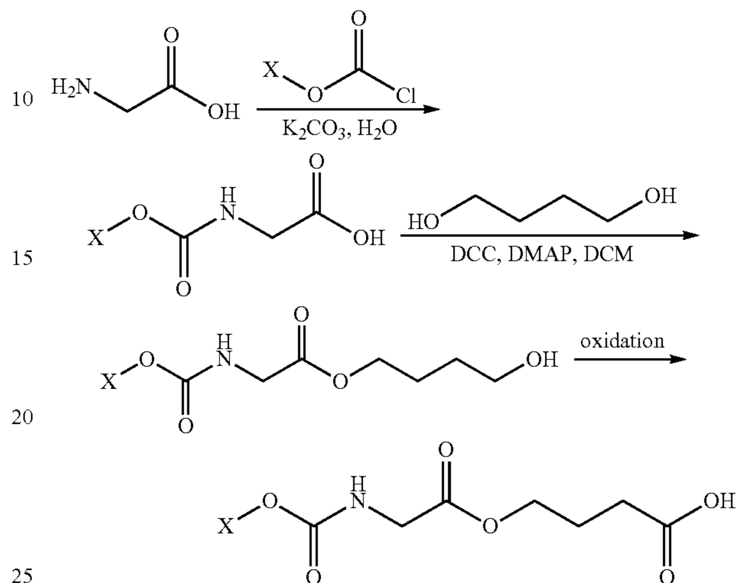
Scheme 6:
