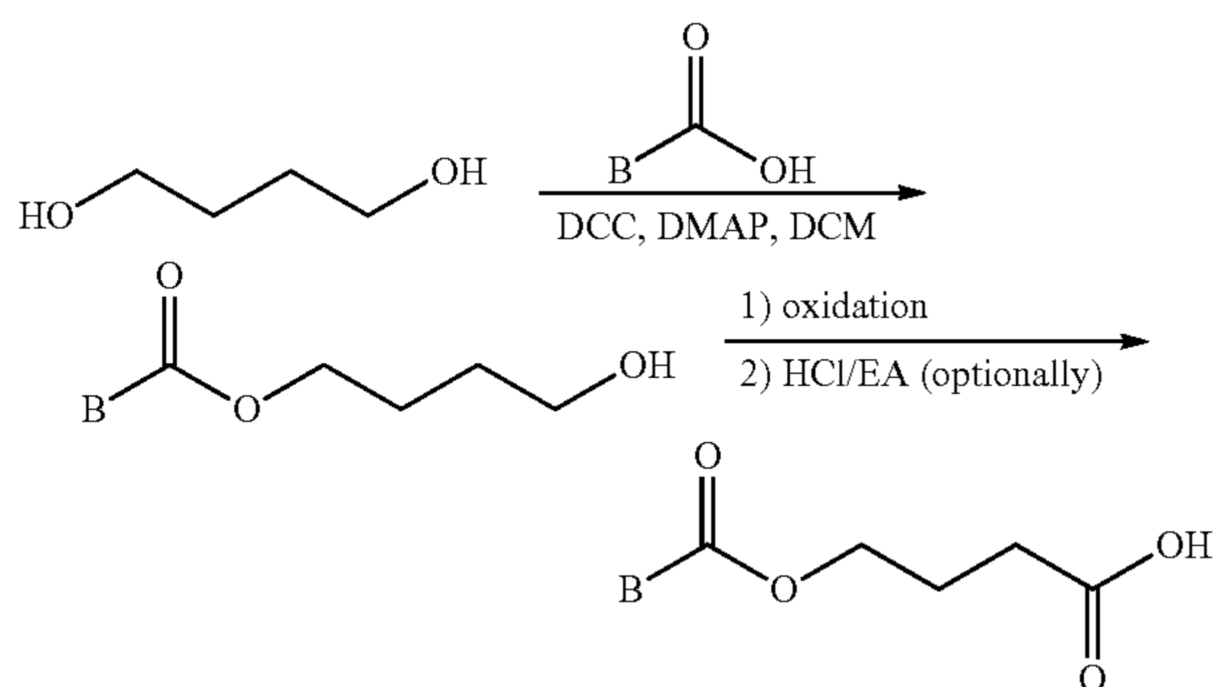
Scheme 2
