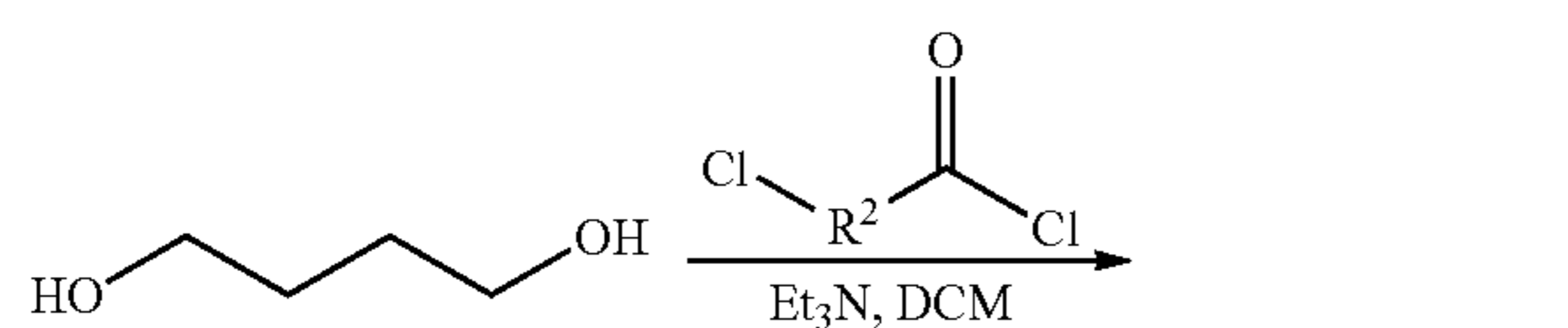
Scheme 13
