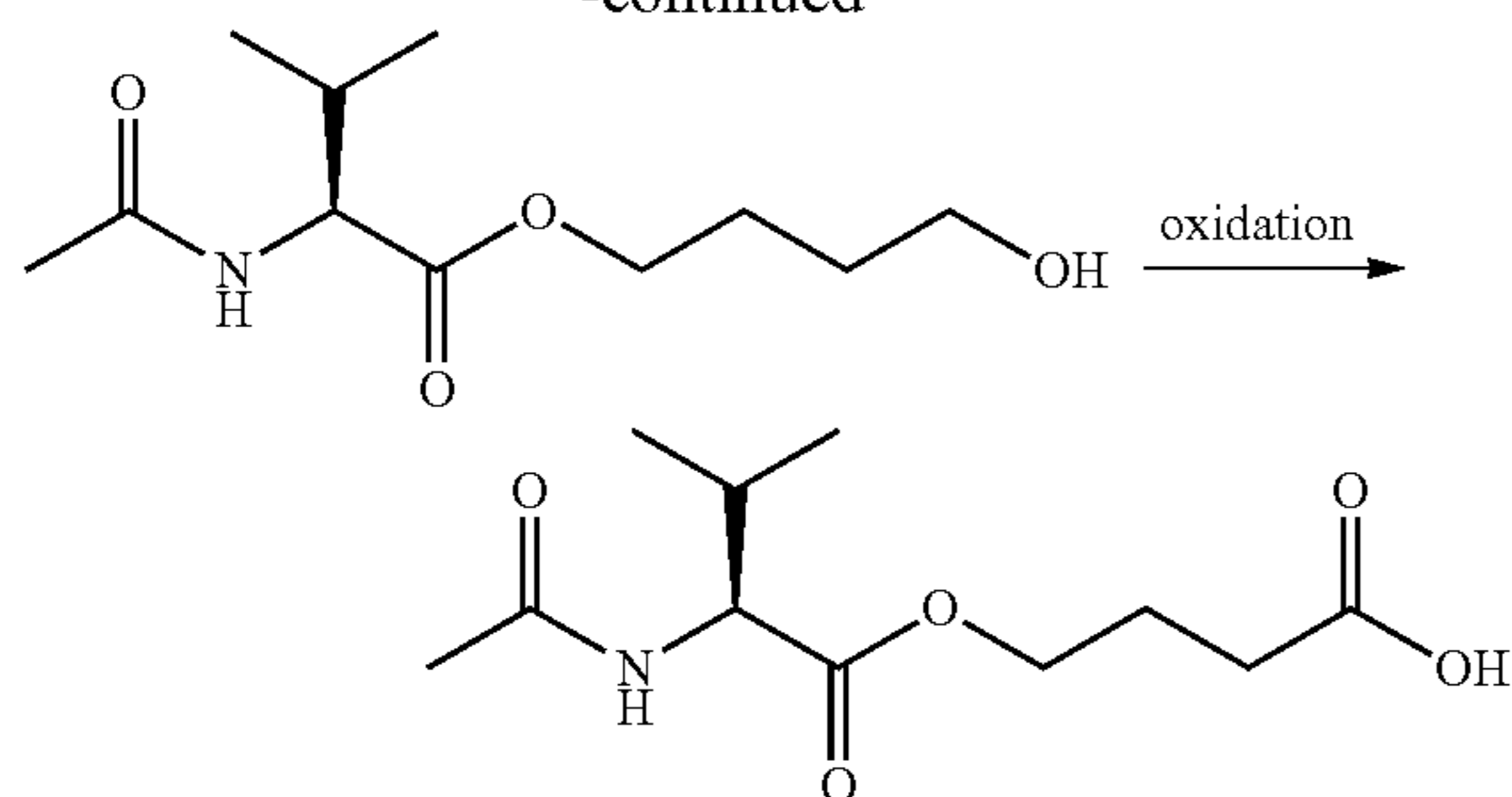
Intermediate Compound 67': (S)-4-hydroxybutyl 2-acetamido-3-methylbutanoate
