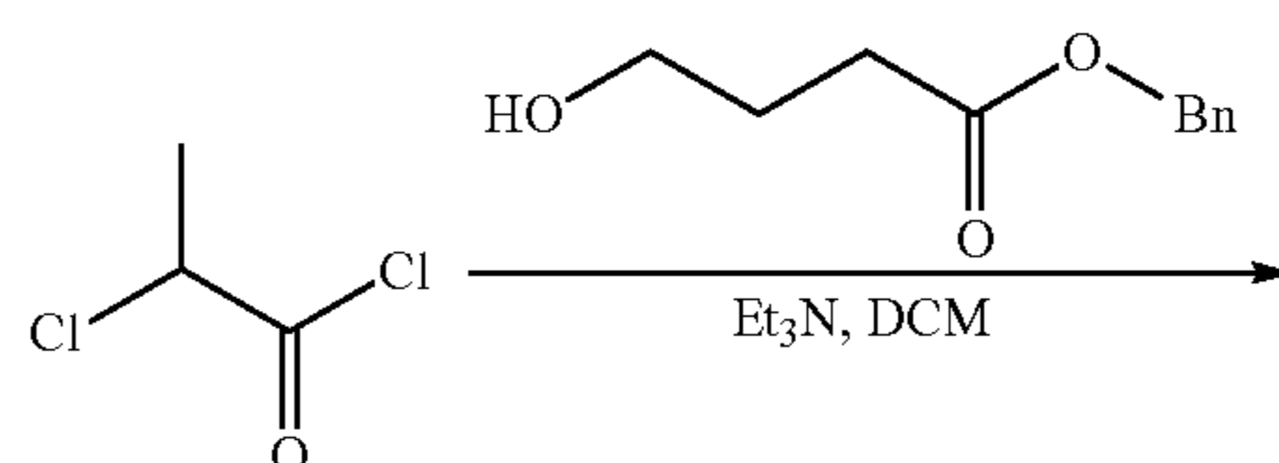
Scheme 15
