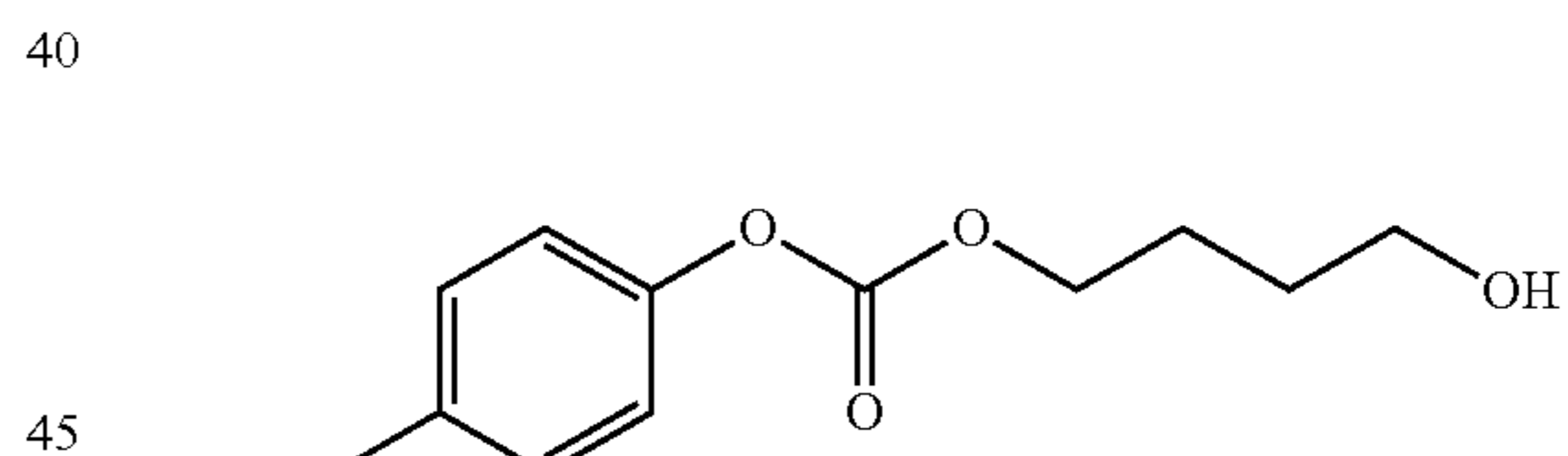
Intermediate Compound 34': 4-hydroxybutyl p-tolyl carbonate
