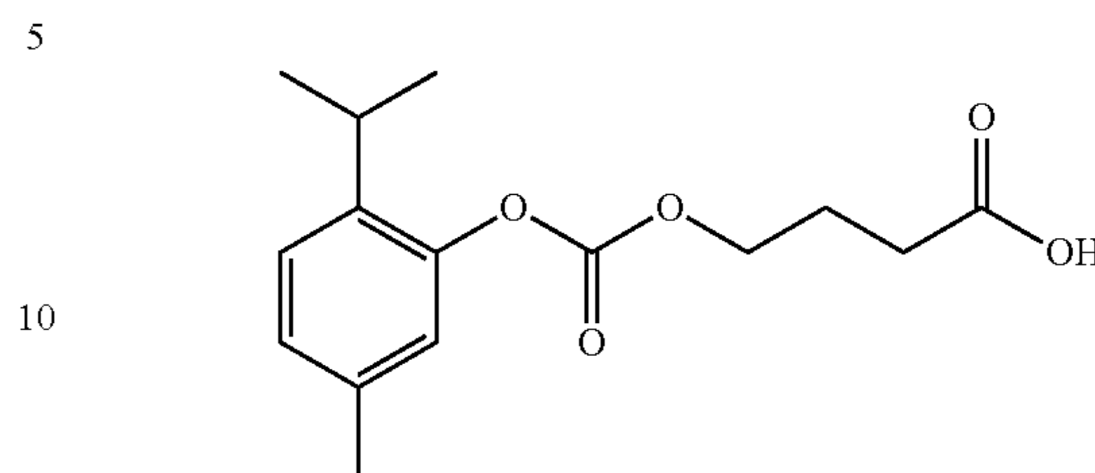
Compound 74: 4-((2-isopropyl-1-methylphenoxy) carbonyloxy)butanoic Acid
