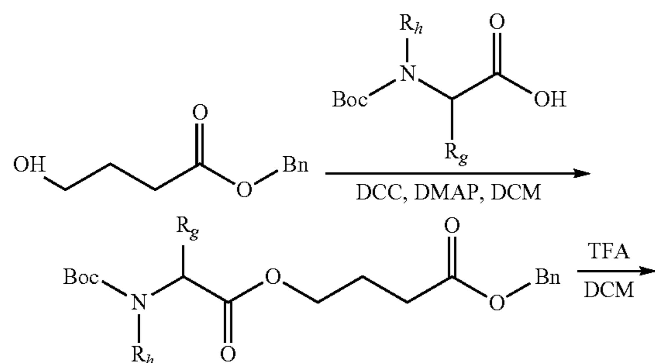
Scheme 3:
