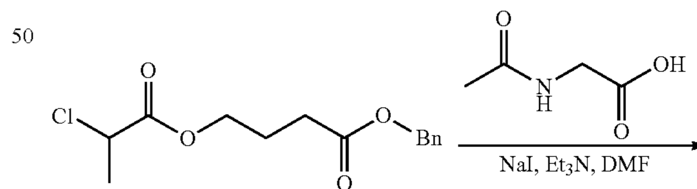
Scheme 16
