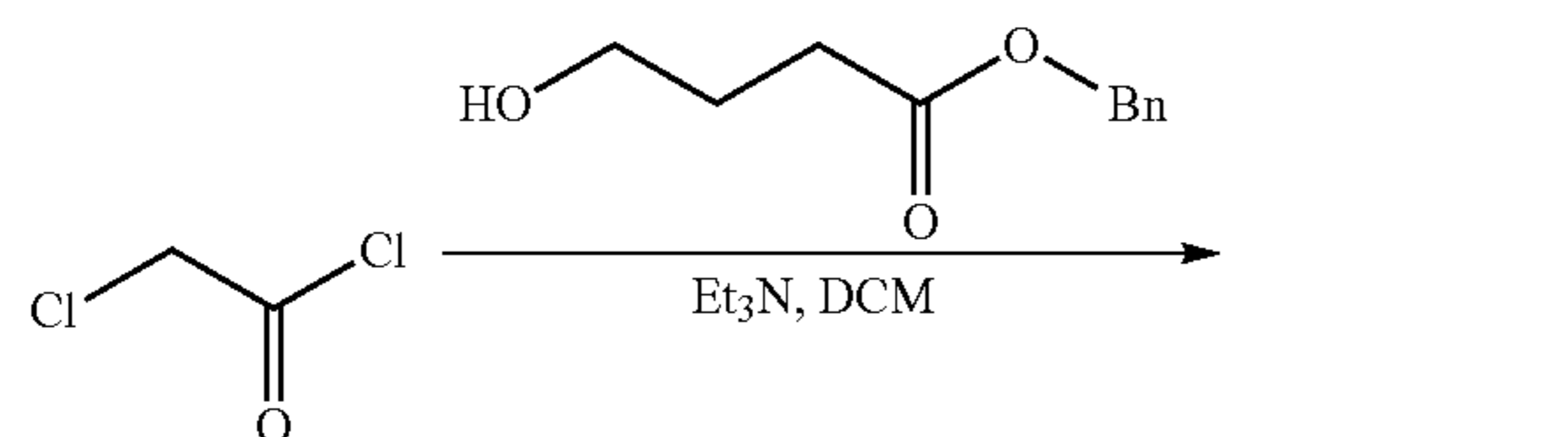
Scheme 14
