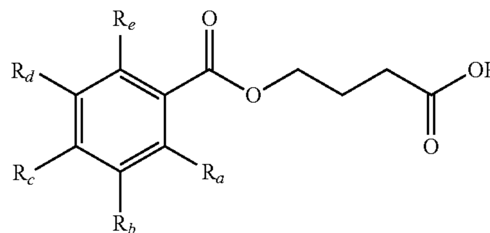
Formula (IA-2) 20
