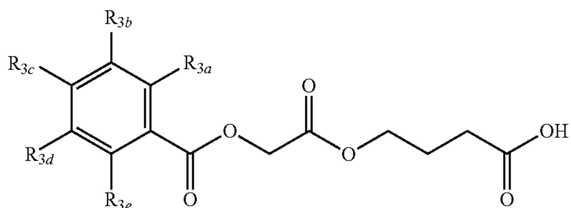
Formula (ID-1) 5
