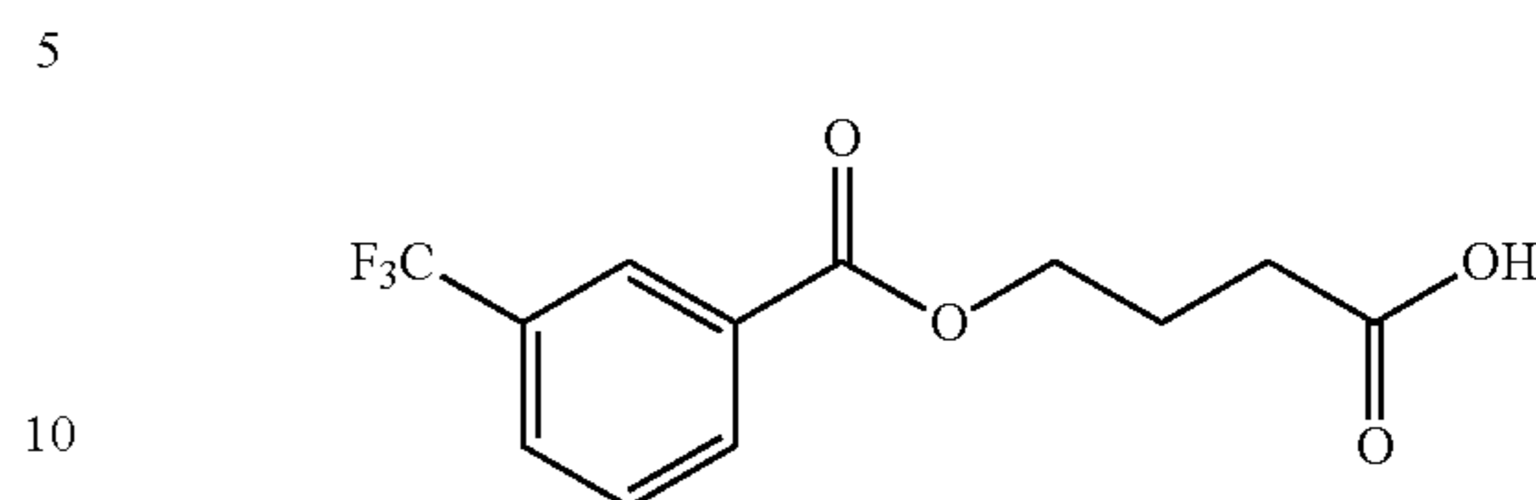
Compound 14: 4-(3-(trifluoromethyl)benzyloxy)butanoic Acid
