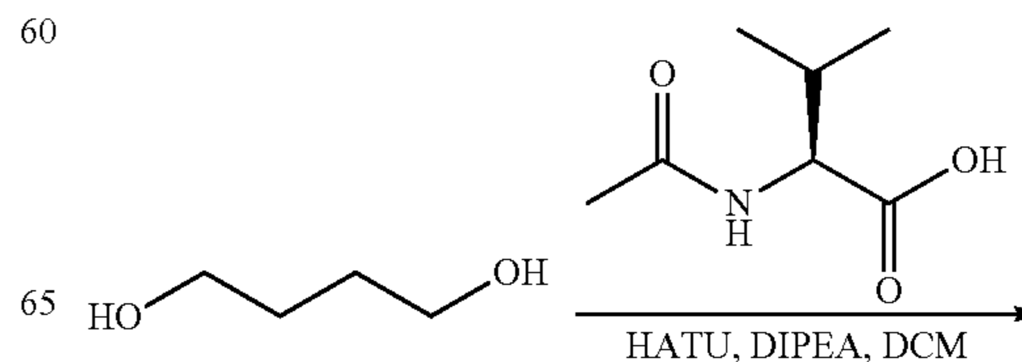
Scheme 5:
