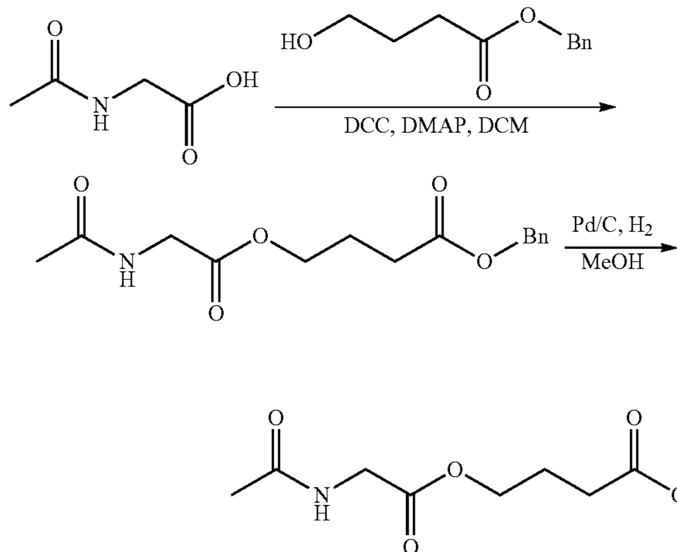
Scheme 4:
