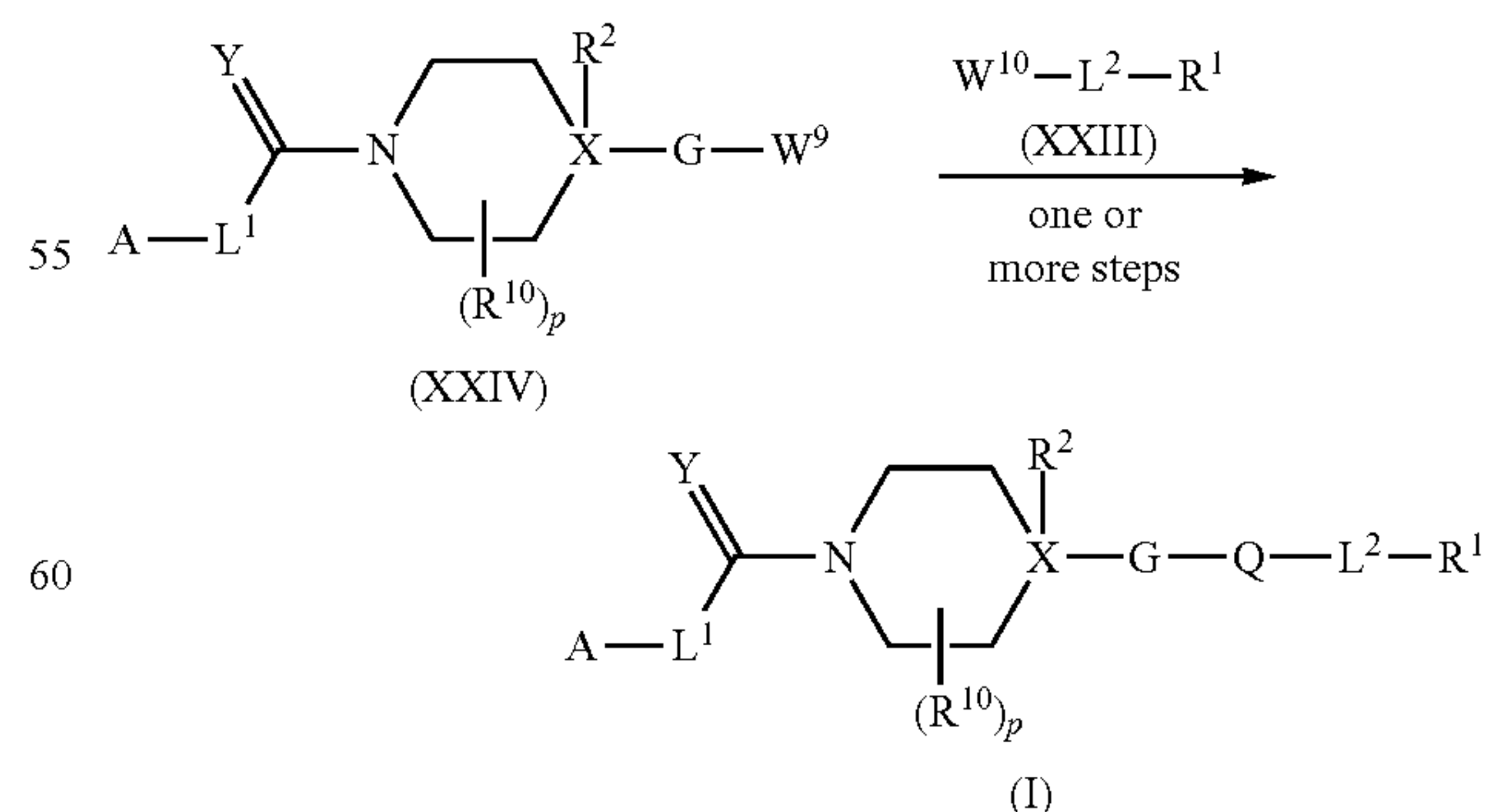
Scheme 1: Process A
