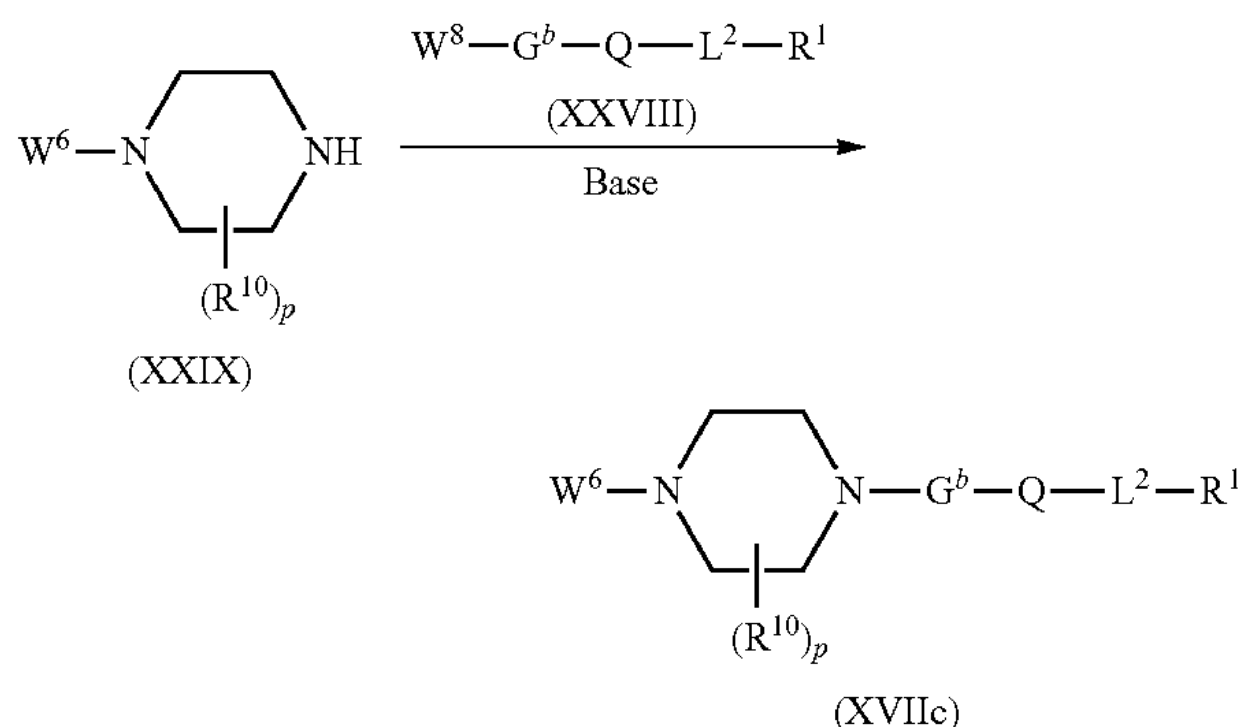
Scheme 16: Process O
