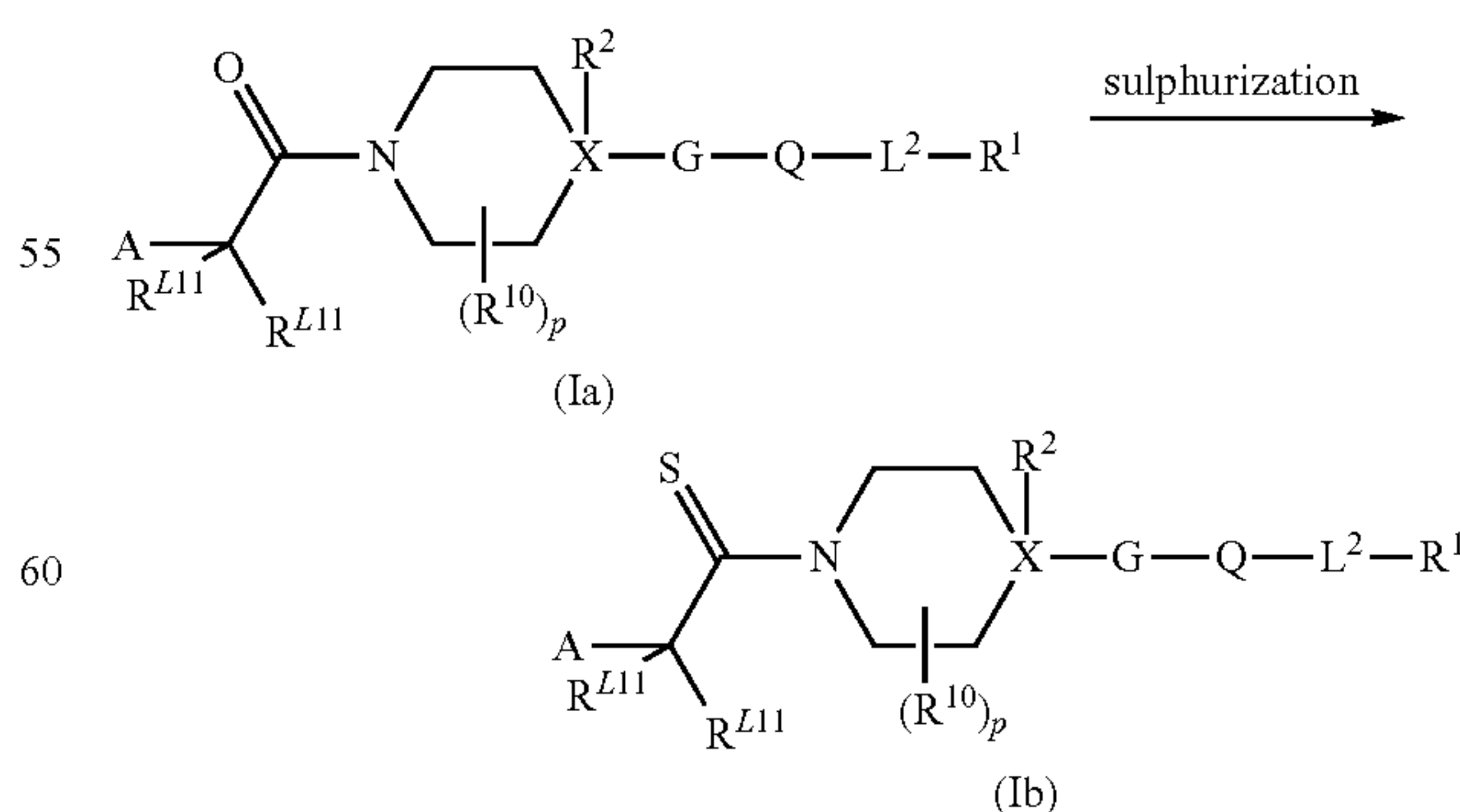
Scheme 7: Process F
