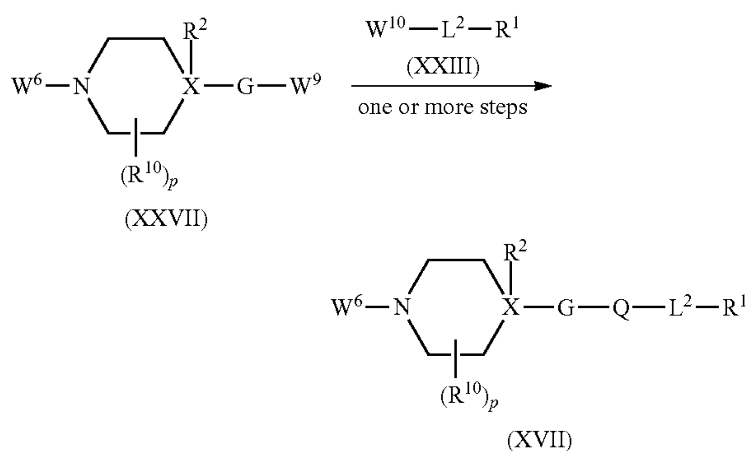
Scheme 17: Process P
