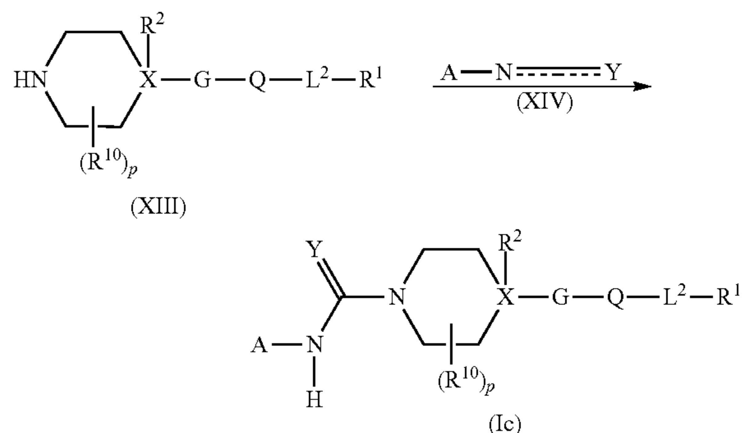
Scheme 10: Process I
