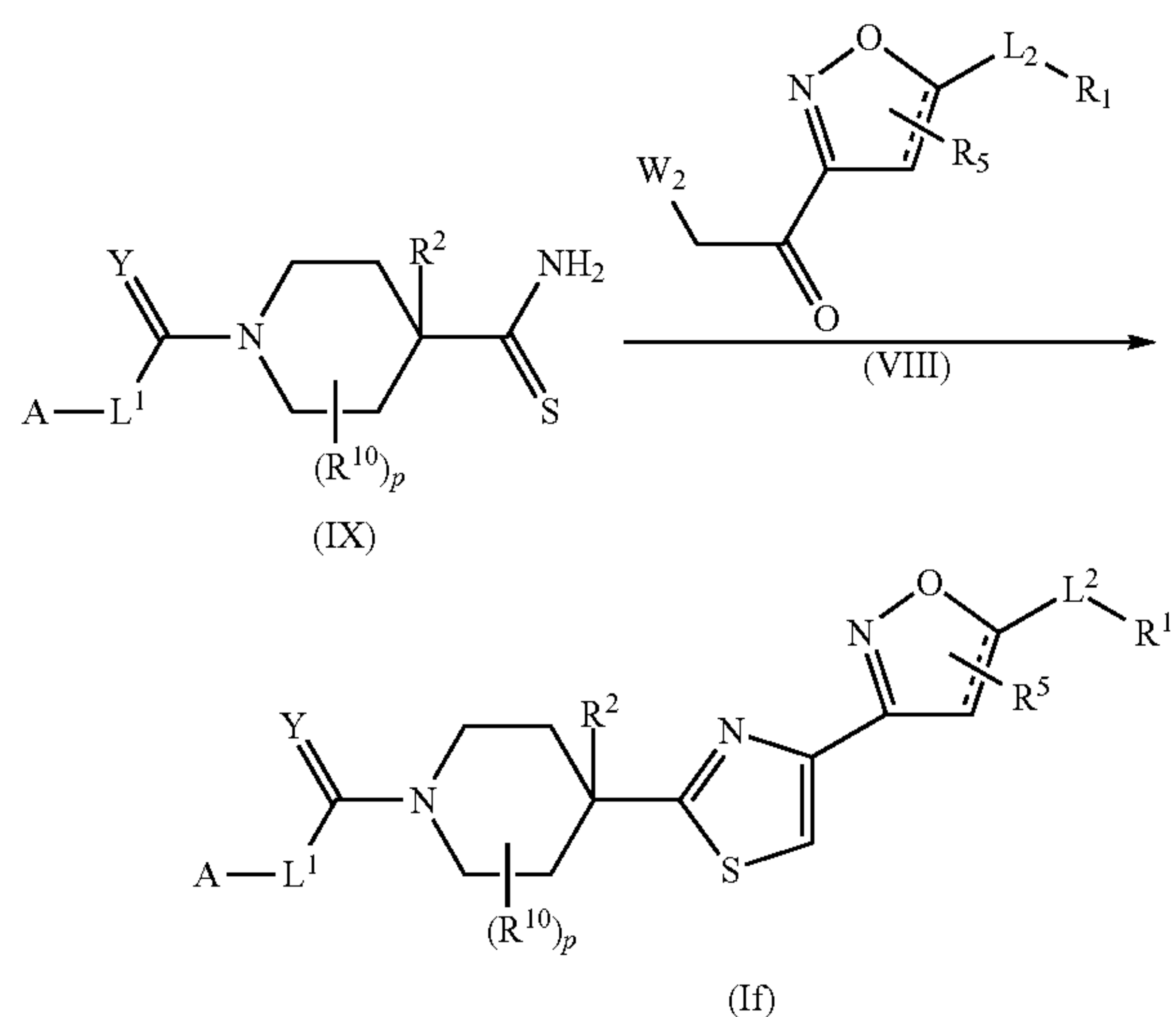
Scheme 5: Process E
