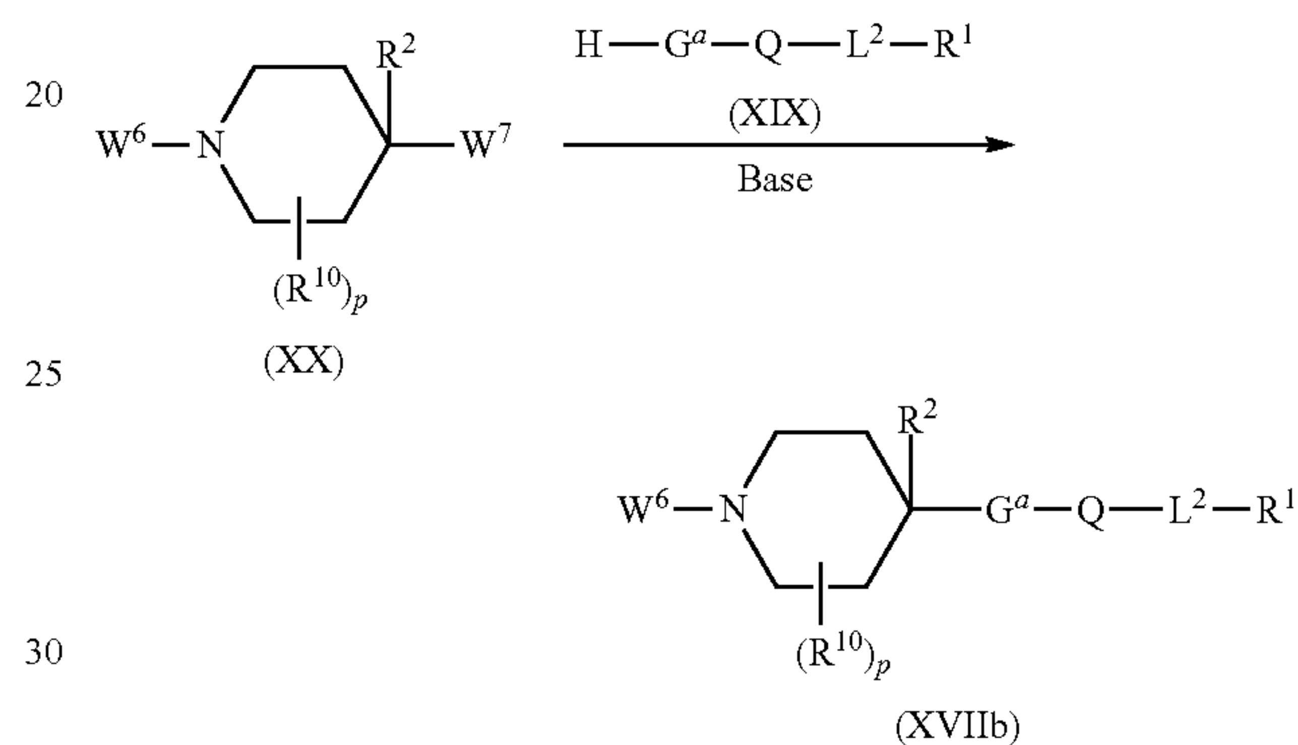
Scheme 15: Process N
