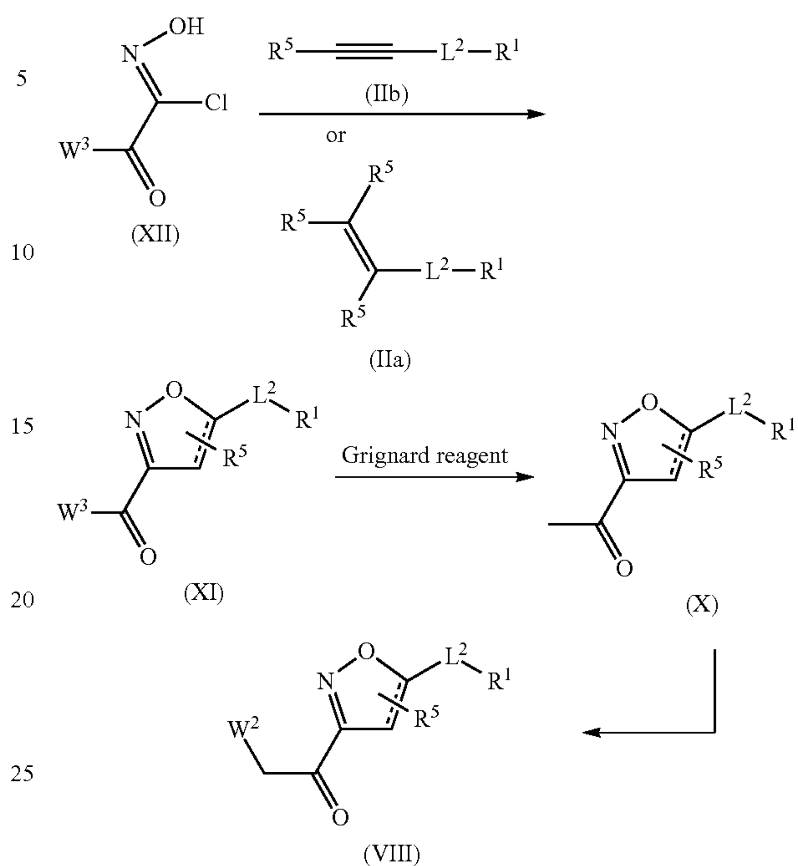
Scheme 6
