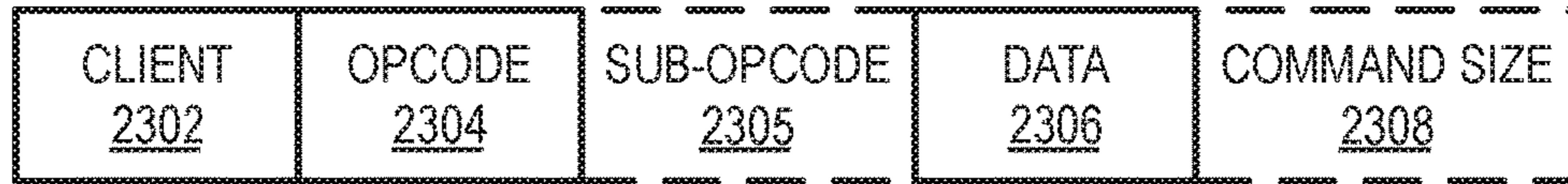
FIG. 23A GRAPHICS PROCESSOR COMMAND FORMAT 2300
