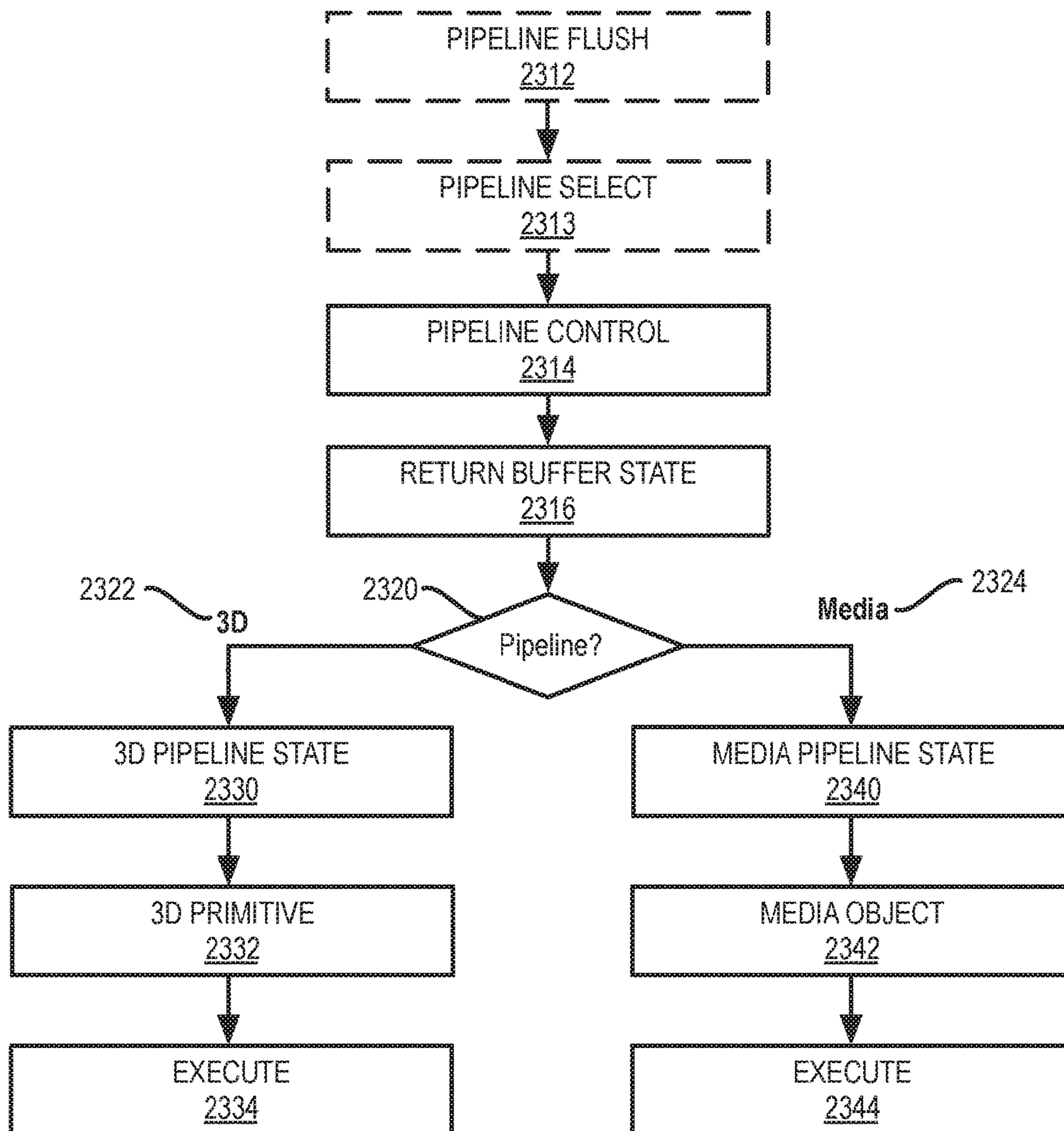
FIG. 23B GRAPHICS PROCESSOR COMMAND SEQUENCE 2310
