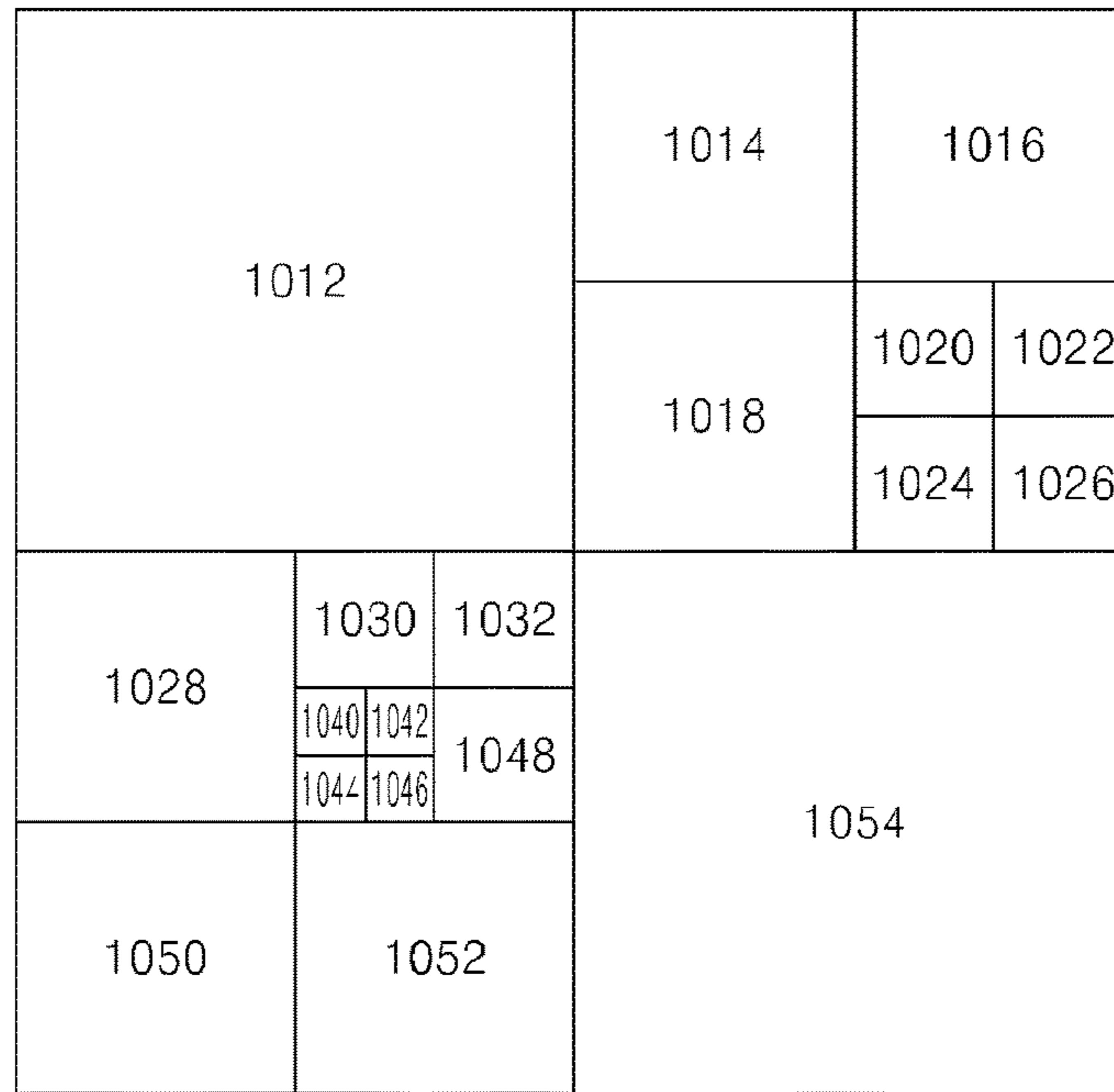
CODING UNIT (1010)
