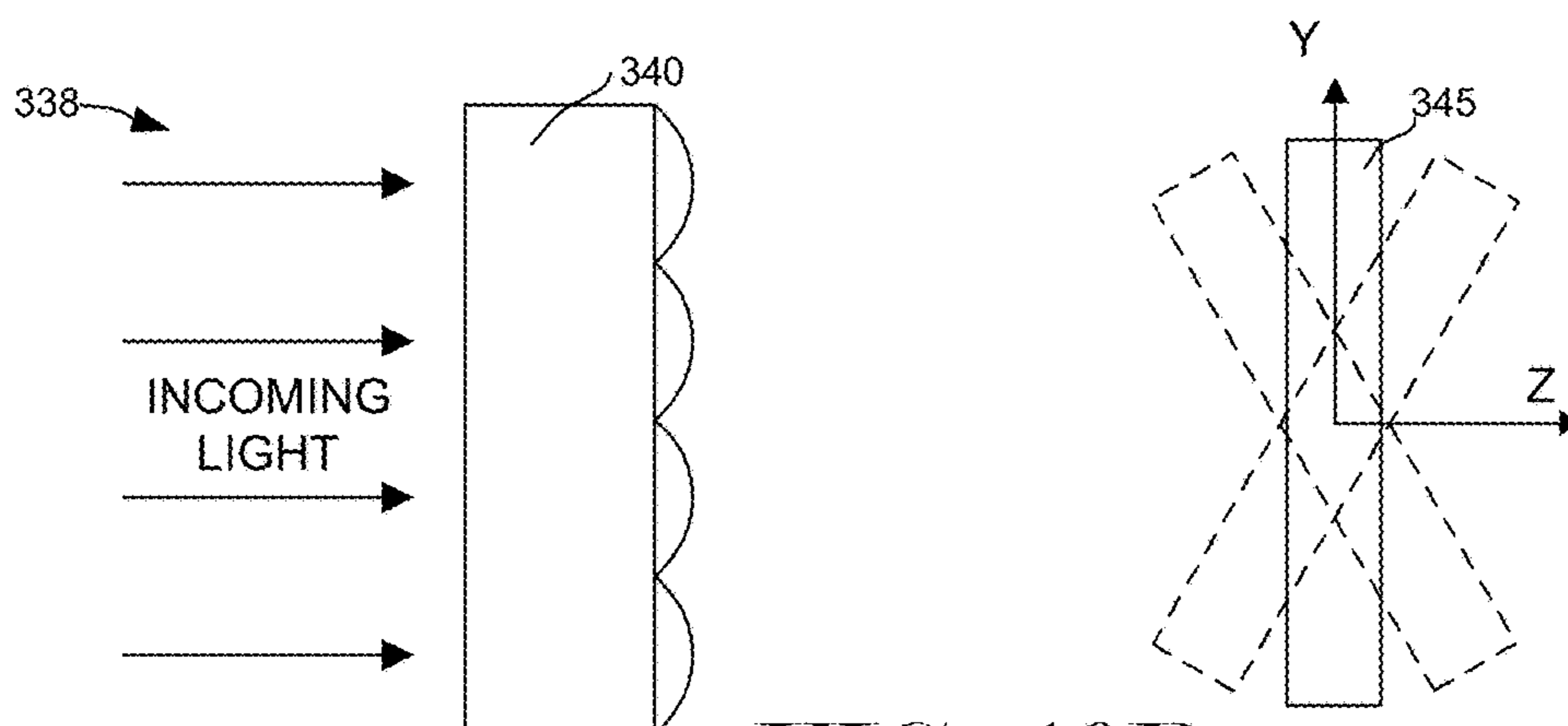
FIG. 10B (SIDE VIEW)
