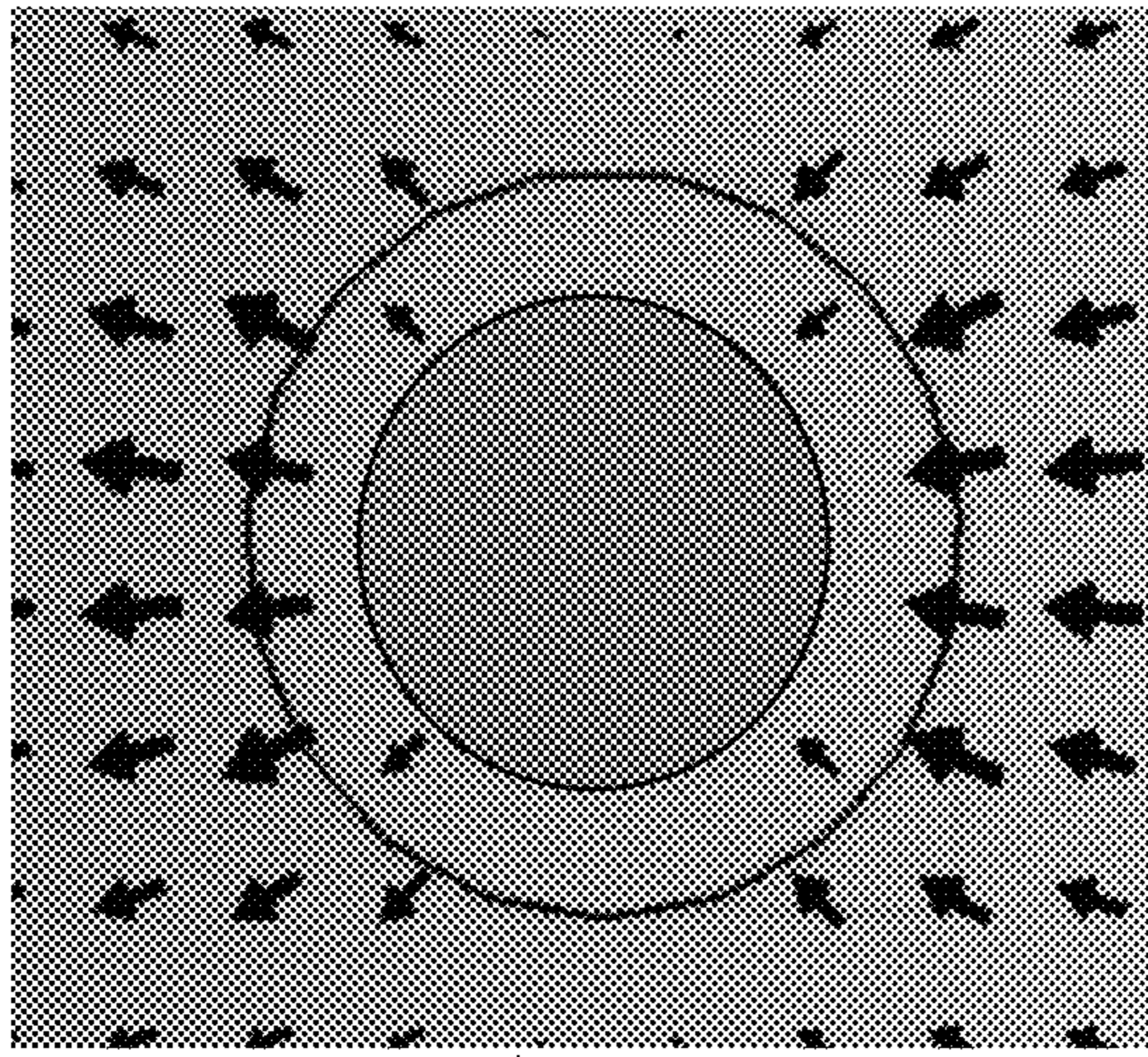
Conductor mode (HE11) 2157
