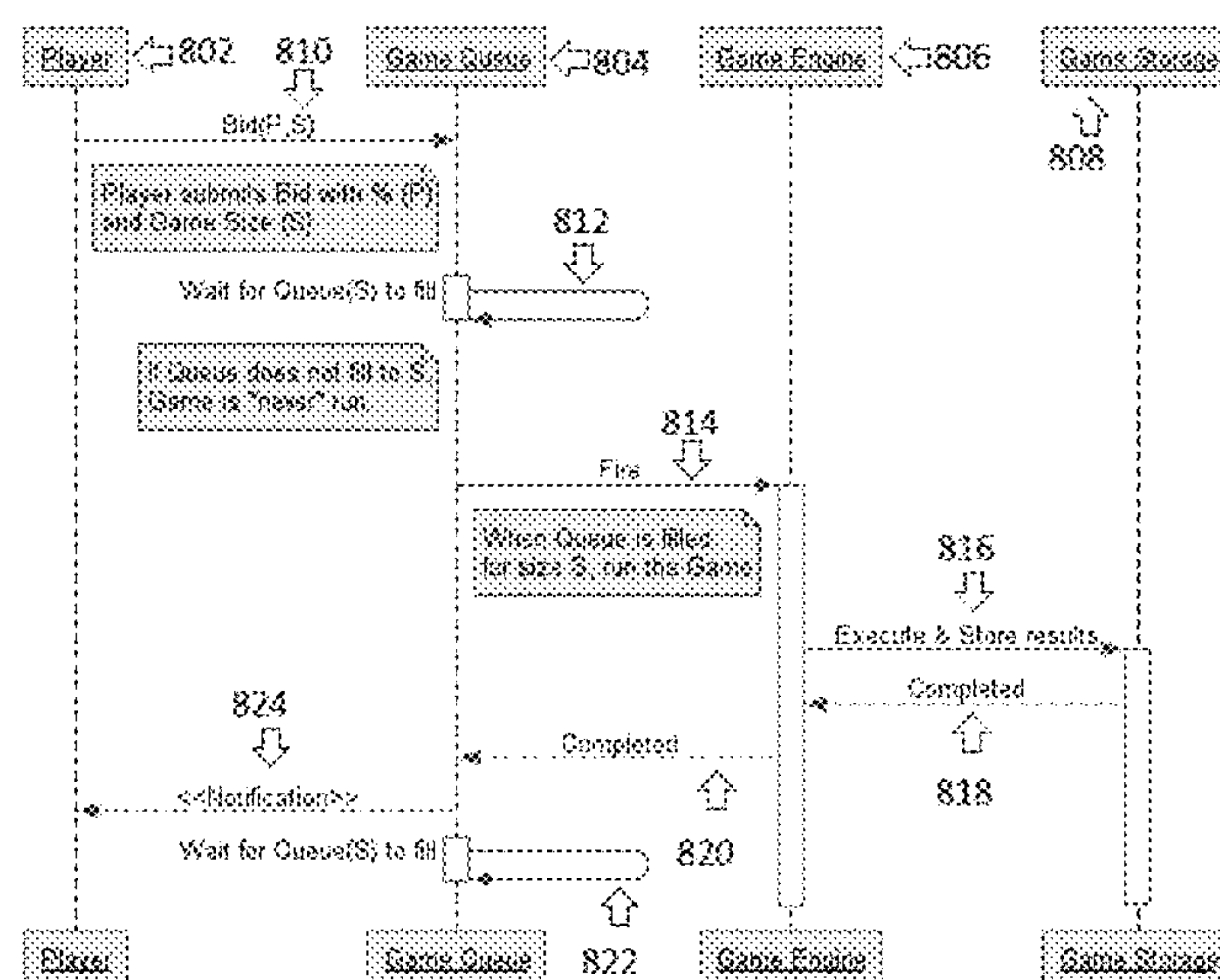
Player/Game Sequence Diagram
