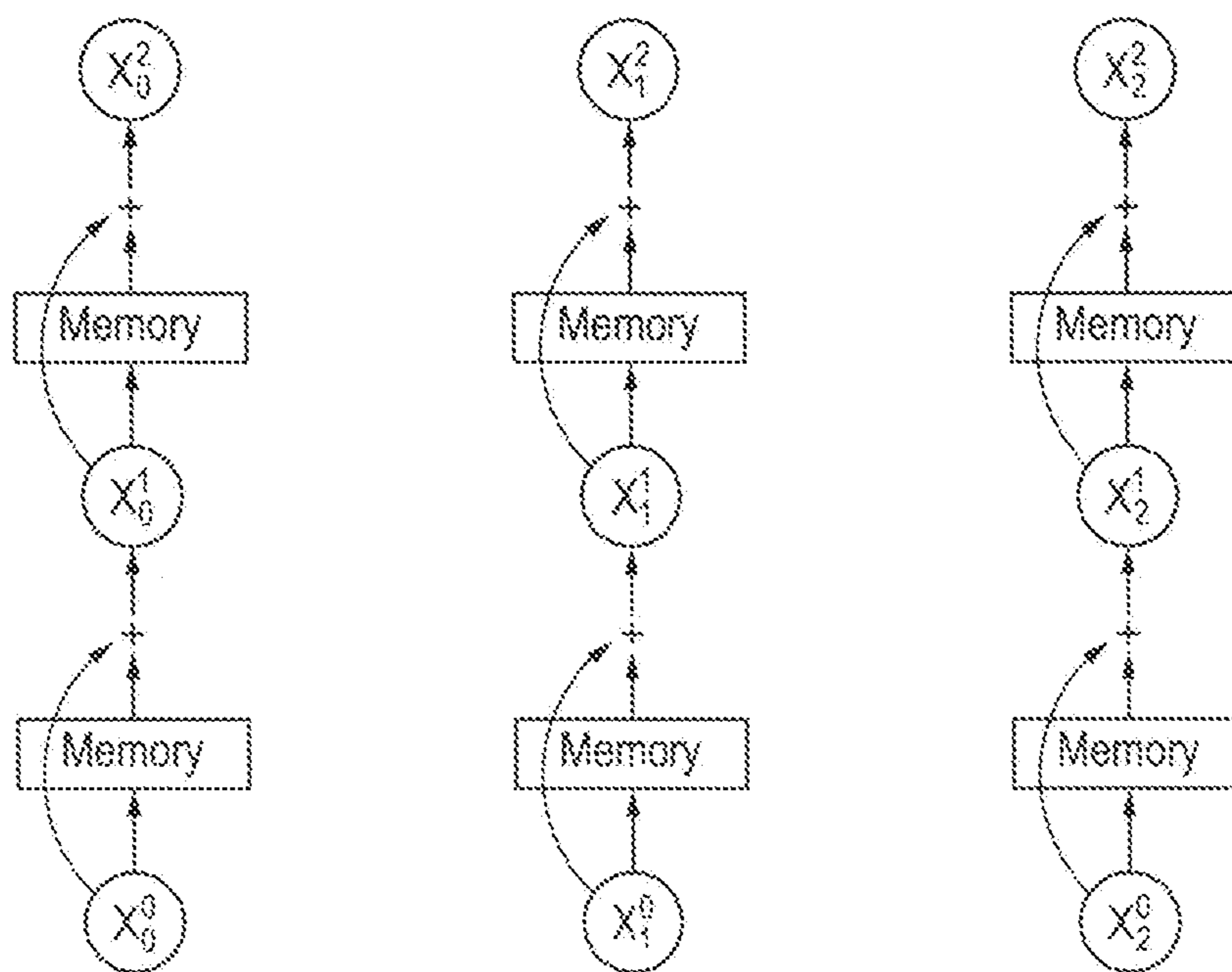
Neural Network
