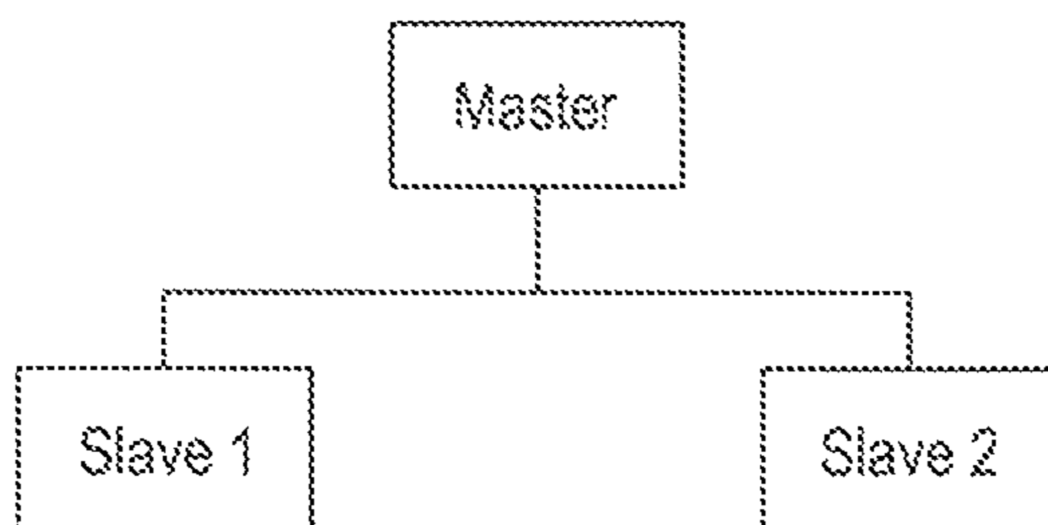
Hierarchical Systems
