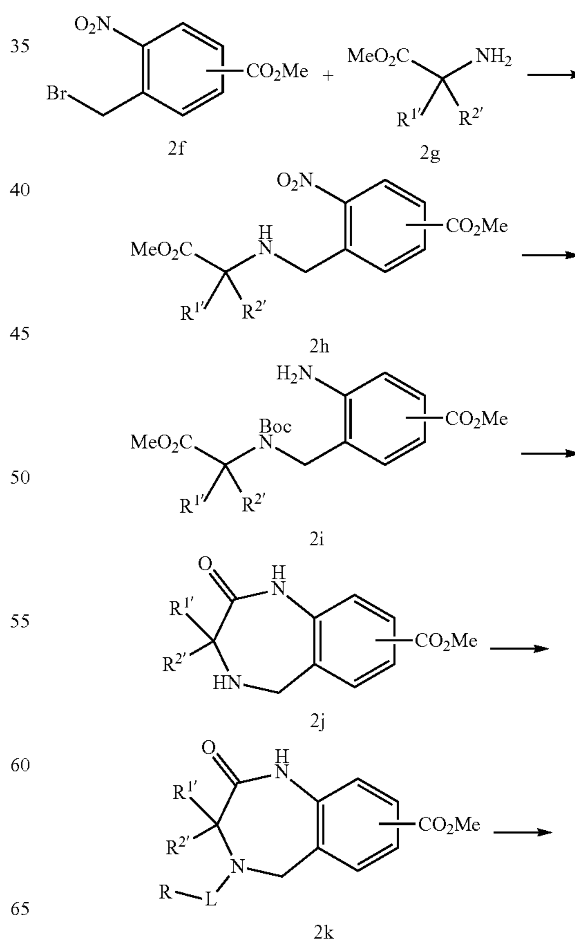
Scheme 2. General synthesis of amides described in the disclosure.
