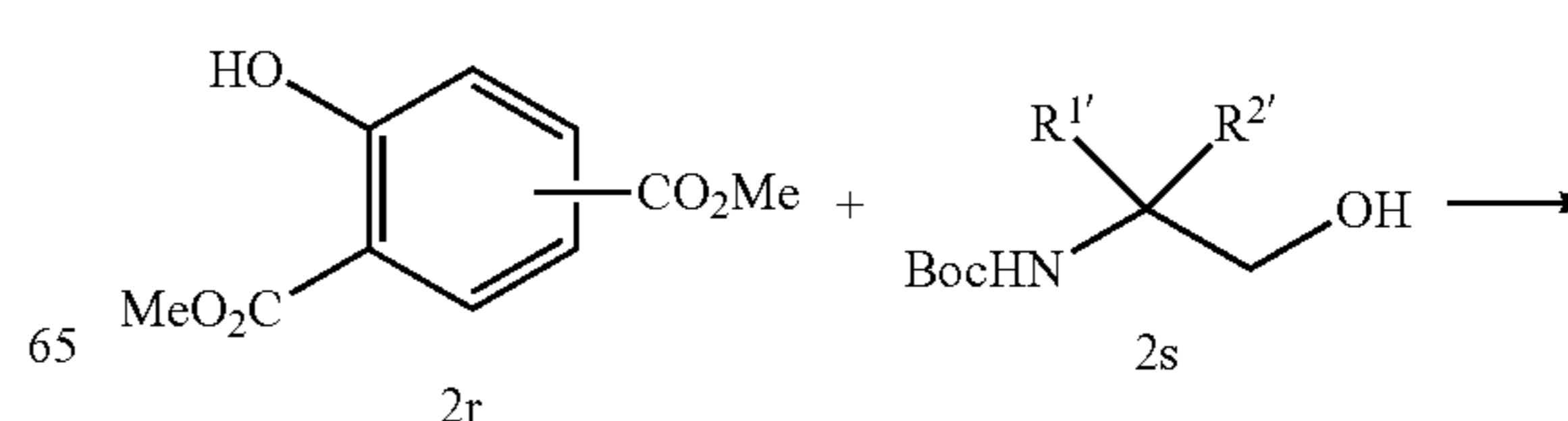
Scheme 4. General synthesis of amides described in the disclosure.
