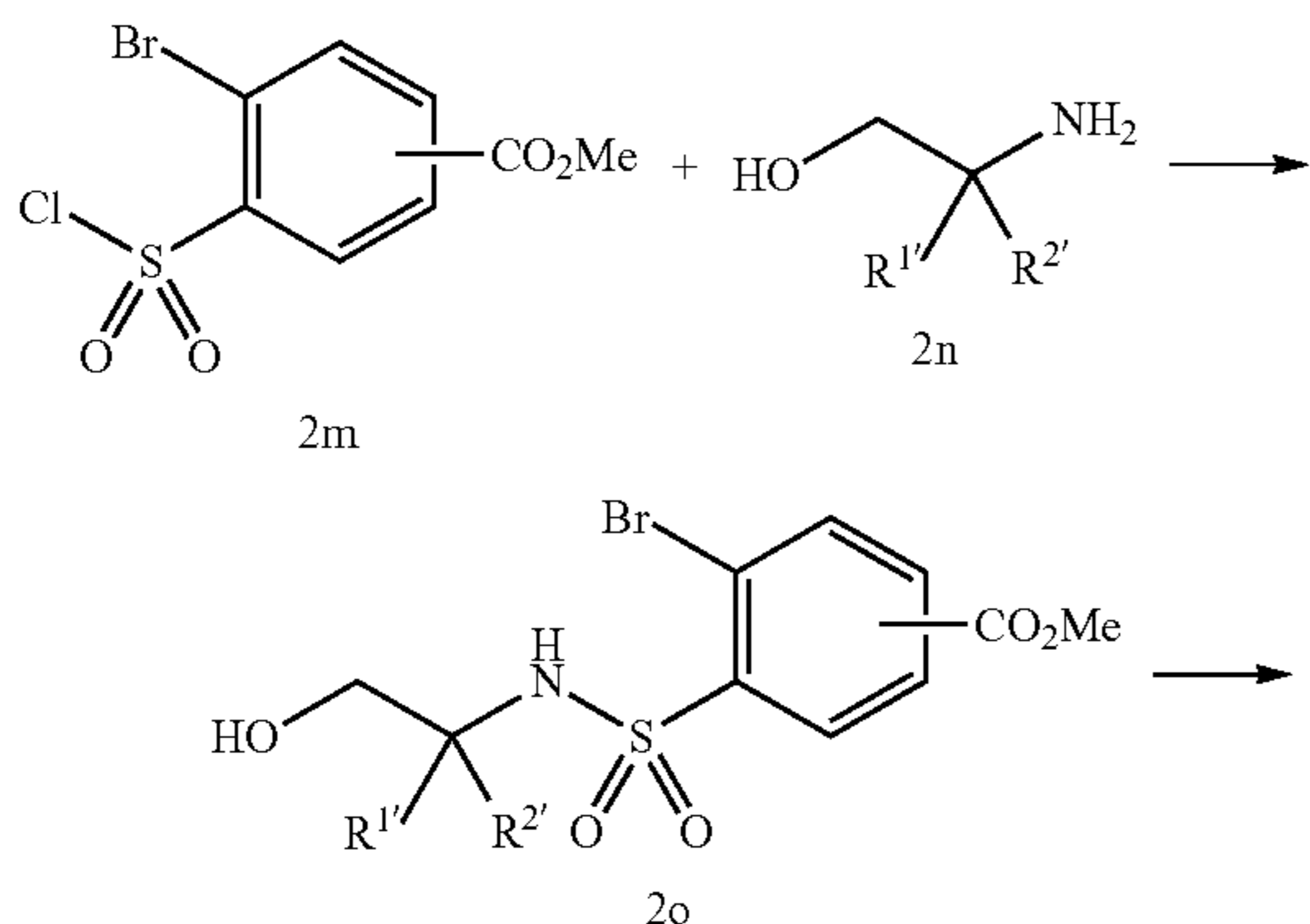
Scheme 3. General synthesis of sulfonamides described in the disclosure.
