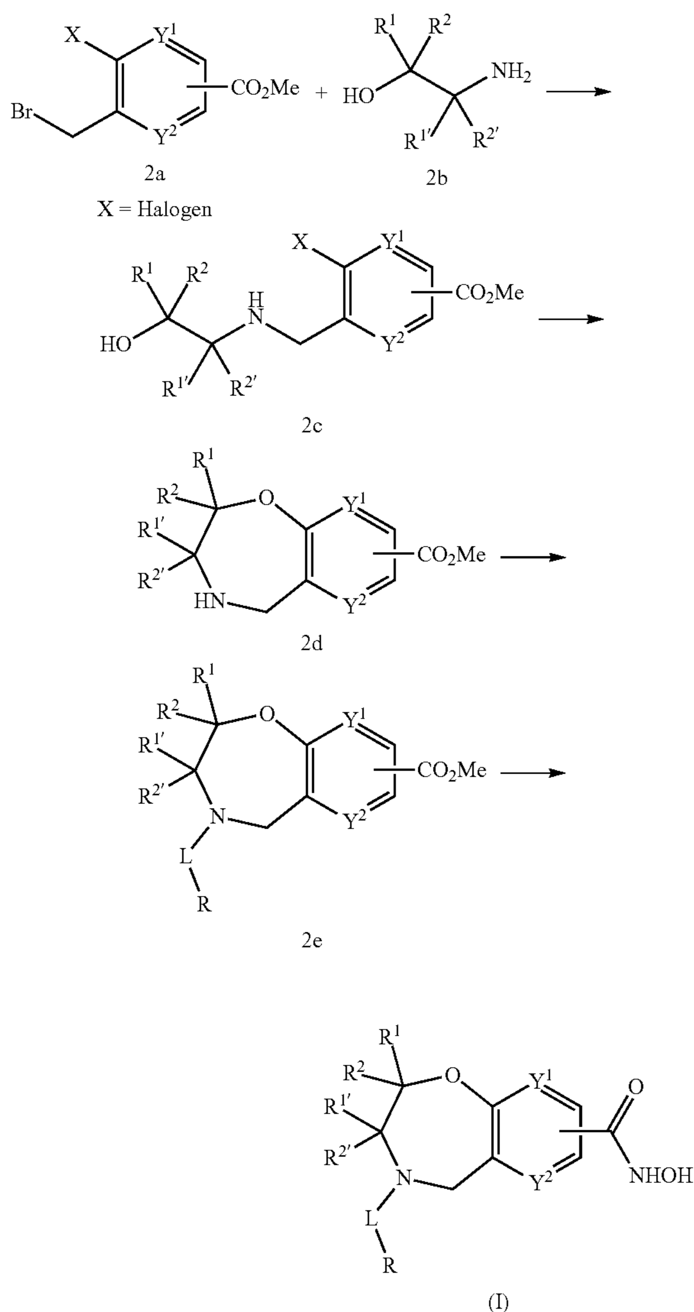
Scheme 1. General synthesis of ethers, thioethers, or sulfones described in the disclosure.
